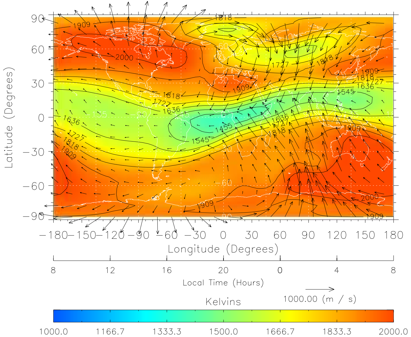
TIME-GCM MAP Temperature with Neutral Wind vectors ZP = 2.00 UT = 20.00 DOY = 324
