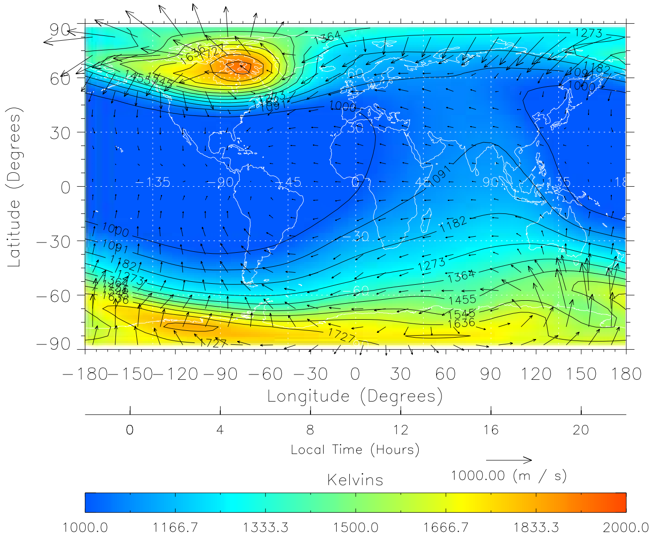
TIME-GCM MAP Temperature with Neutral Wind vectors ZP = 2.00 UT = 10.00 DOY = 324
