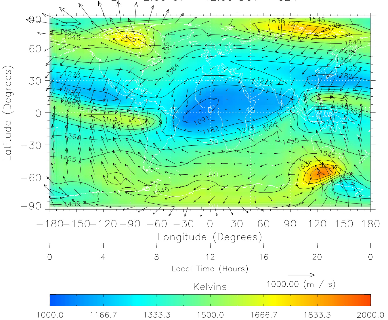
TIME-GCM MAP Temperature with Neutral Wind vectors ZP = 2.00 UT = 12.00 DOY = 324
