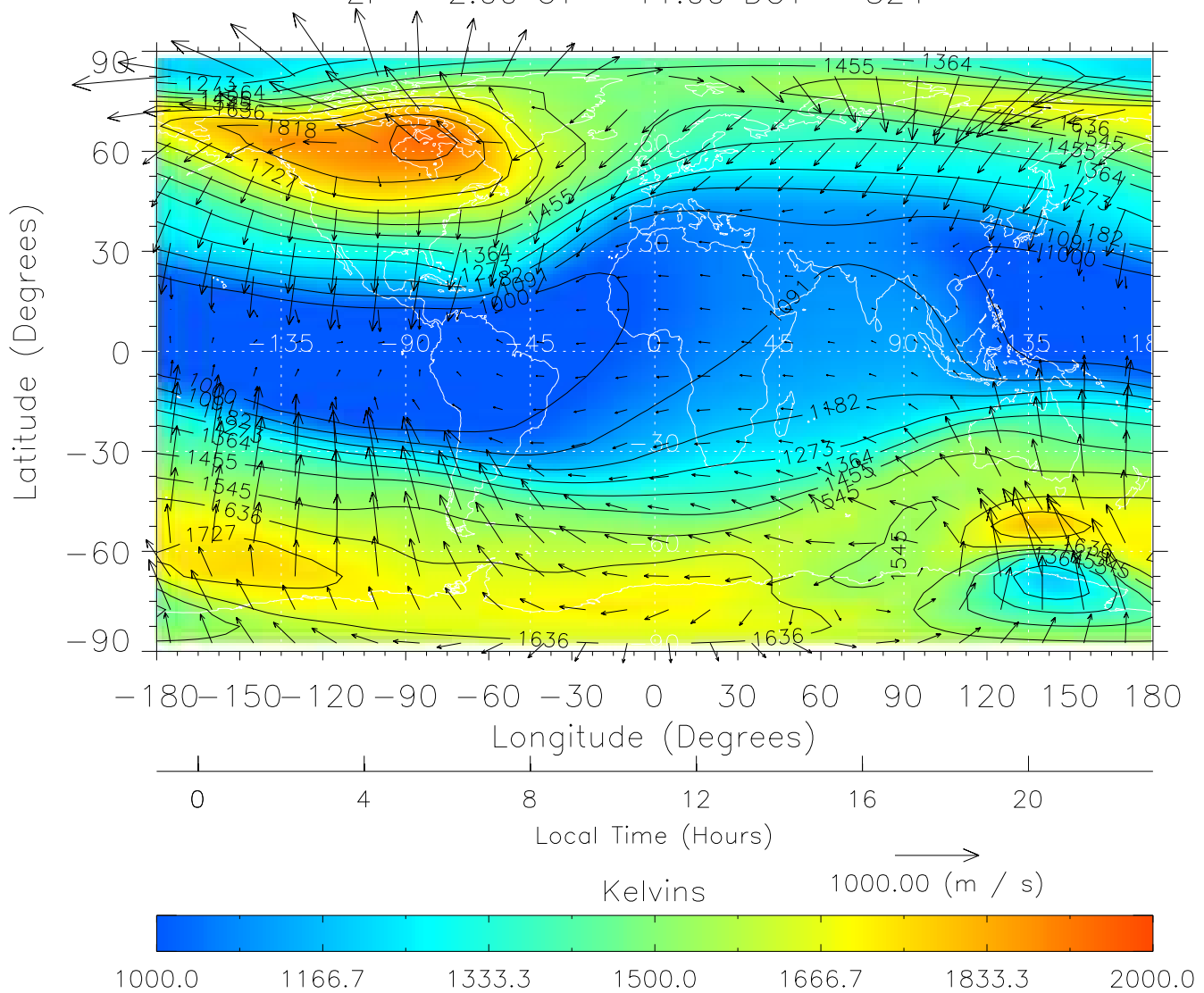
TIME-GCM MAP Temperature with Neutral Wind vectors ZP = 2.00 UT = 11.00 DOY = 324
