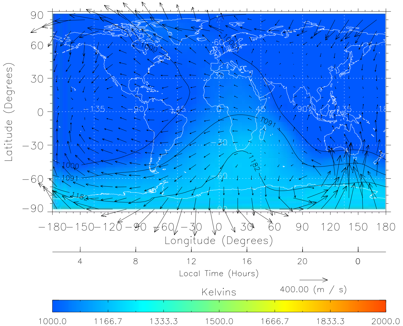
TIME-GCM MAP Temperature with Neutral Wind vectors ZP = 2.00 UT = 14.00 DOY = 323
