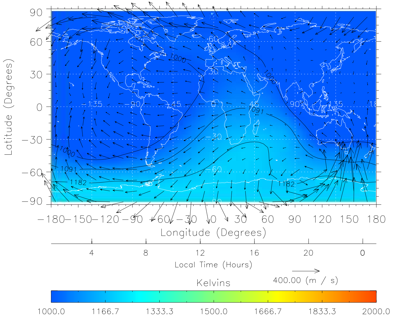
TIME-GCM MAP Temperature with Neutral Wind vectors ZP = 2.00 UT = 13.00 DOY = 323
