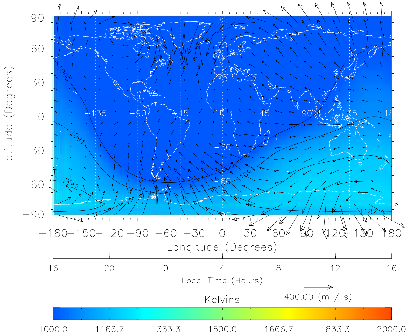
TIME-GCM MAP Temperature with Neutral Wind vectors ZP = 2.00 UT = 4.00 DOY = 323
