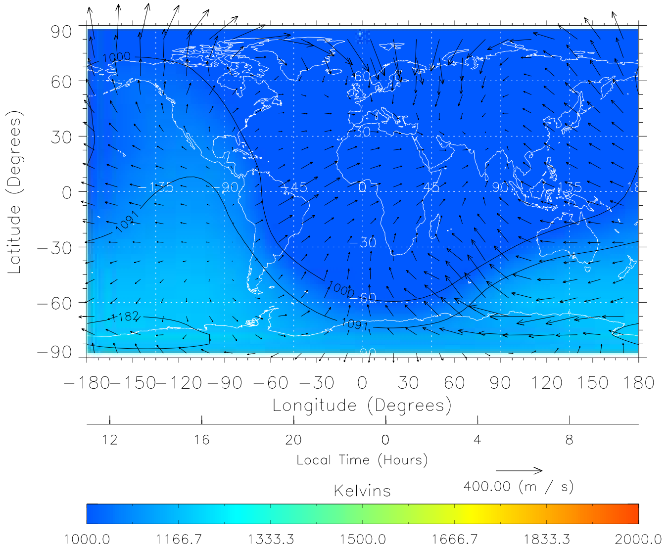
TIME-GCM MAP Temperature with Neutral Wind vectors ZP = 2.00 UT = 23.00 DOY = 323
