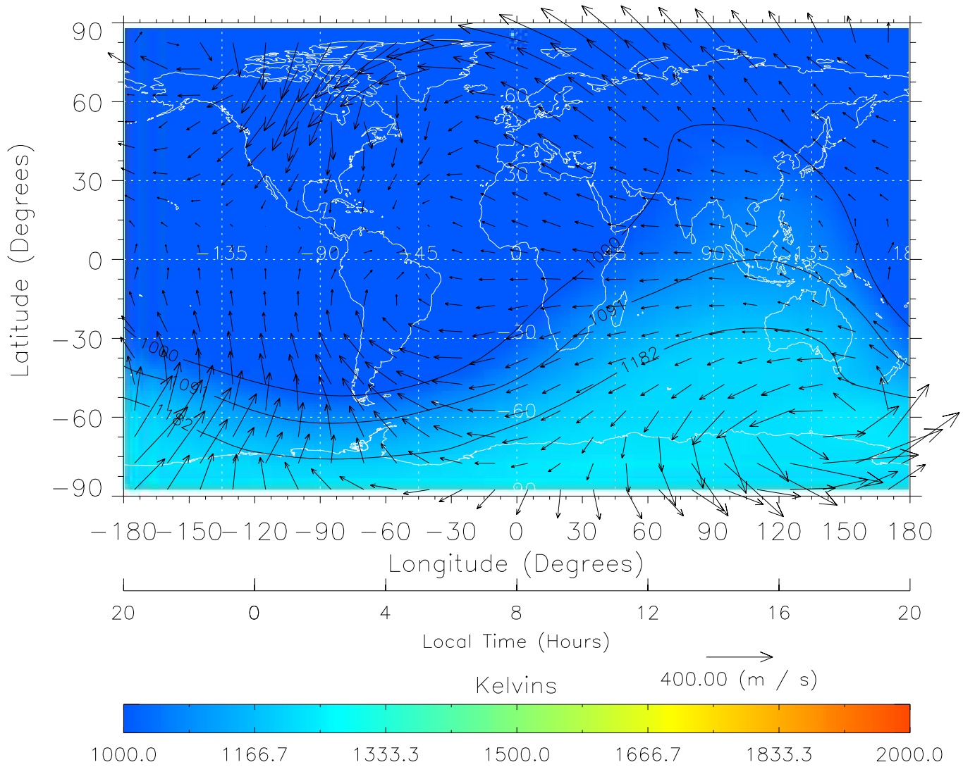
TIME-GCM MAP Temperature with Neutral Wind vectors ZP = 2.00 UT = 8.00 DOY = 323
