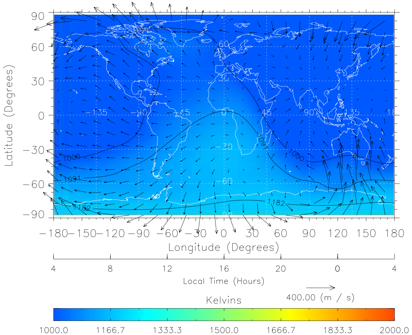
TIME-GCM MAP Temperature with Neutral Wind vectors ZP = 2.00 UT = 16.00 DOY = 323
