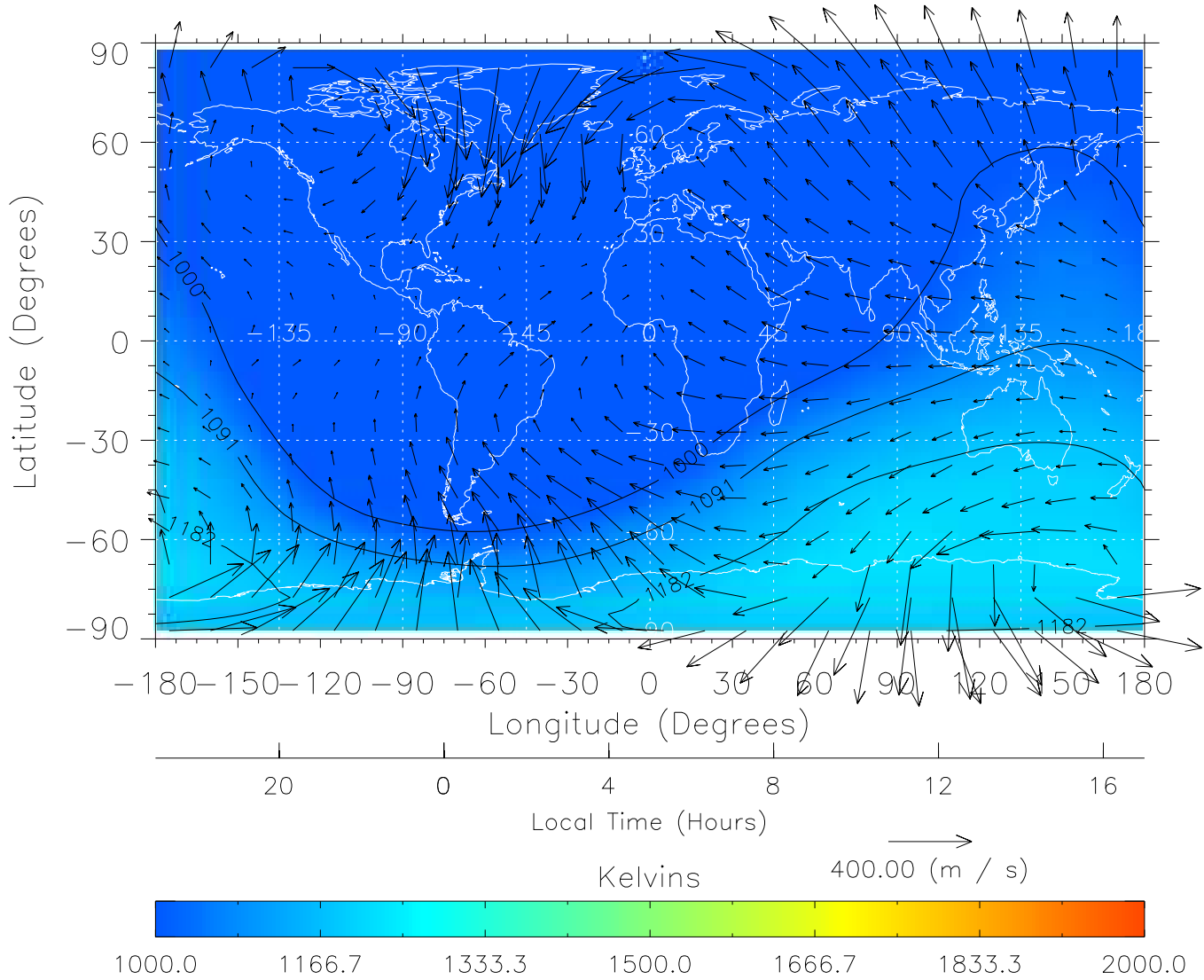
TIME-GCM MAP Temperature with Neutral Wind vectors ZP = 2.00 UT = 5.00 DOY = 323
