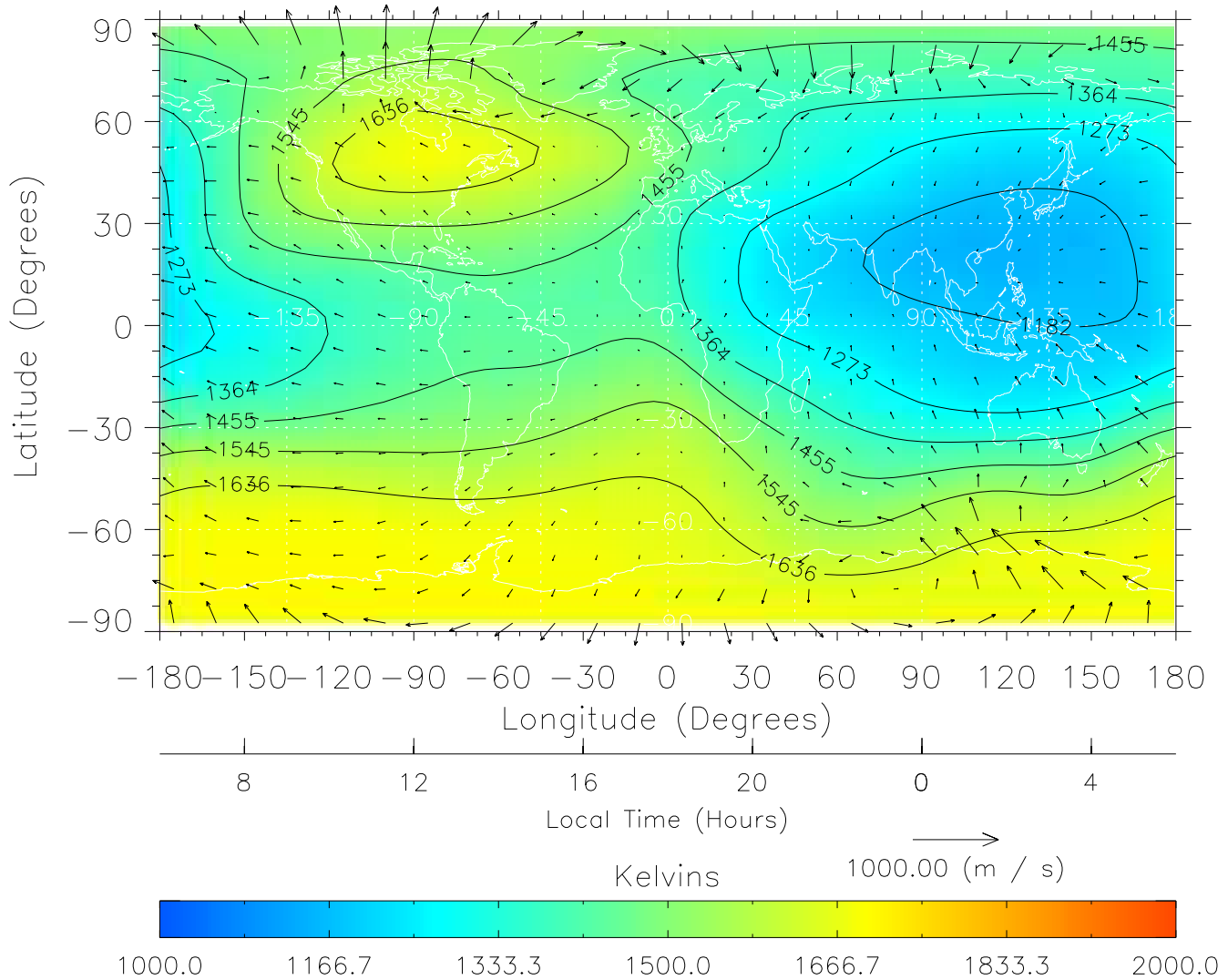
TIME-GCM MAP Temperature with Neutral Wind vectors ZP = 2.00 UT = 18.00 DOY = 303
