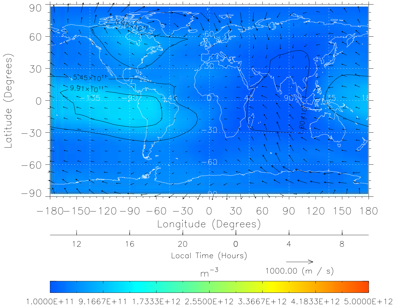
TIME-GCM MAP NmF2 with Neutral Wind vectors ZP = 2.00 UT = 22.00 DOY = 304
