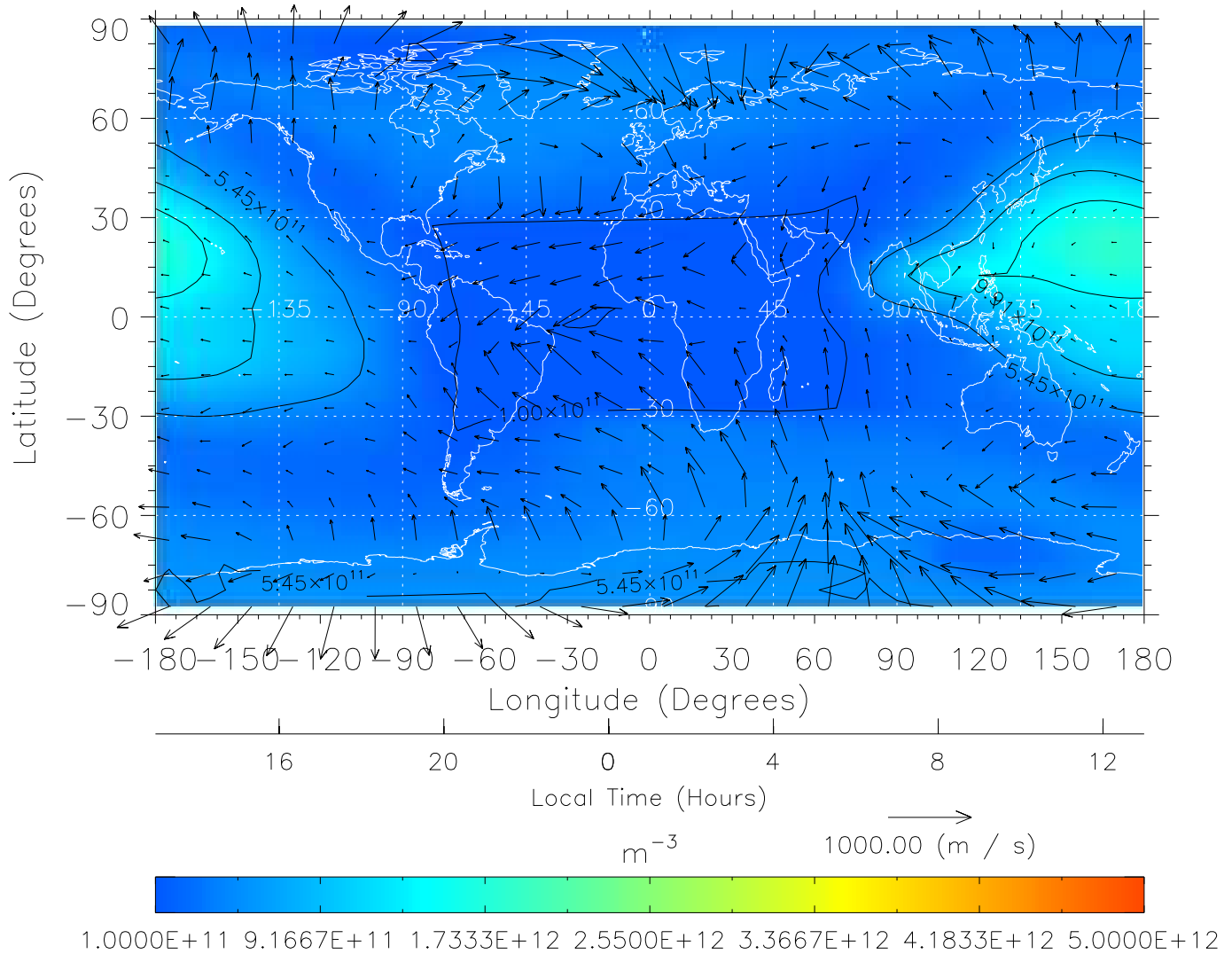
TIME-GCM MAP NmF2 with Neutral Wind vectors ZP = 2.00 UT = 1.00 DOY = 304
