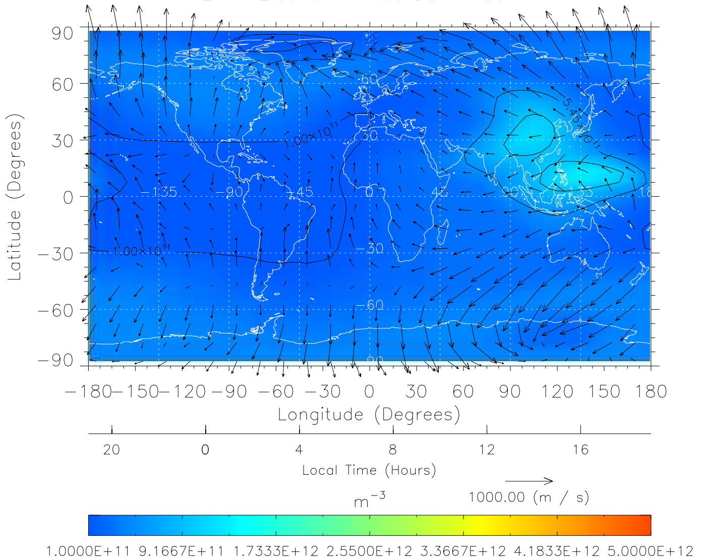
TIME-GCM MAP NmF2 with Neutral Wind vectors ZP = 2.00 UT = 7.00 DOY = 304
