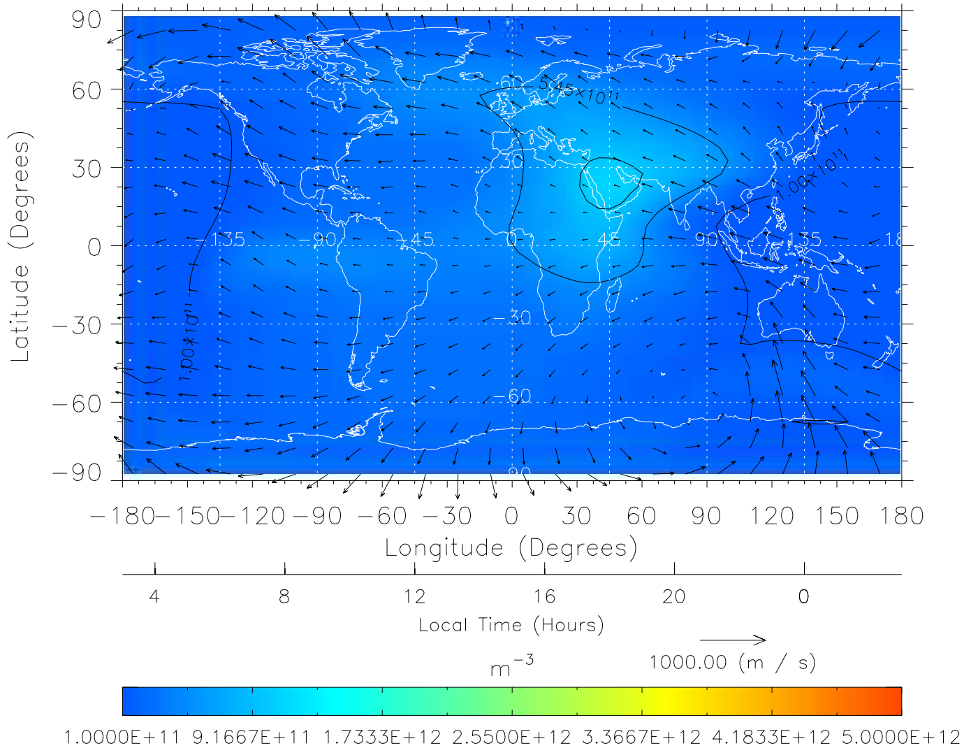
TIME-GCM MAP NmF2 with Neutral Wind vectors ZP = 2.00 UT = 15.00 DOY = 304
