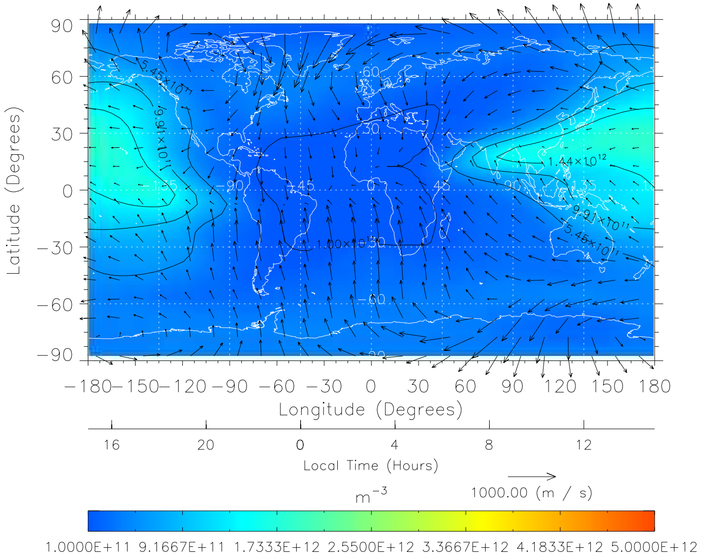
TIME-GCM MAP NmF2 with Neutral Wind vectors ZP = 2.00 UT = 3.00 DOY = 303
