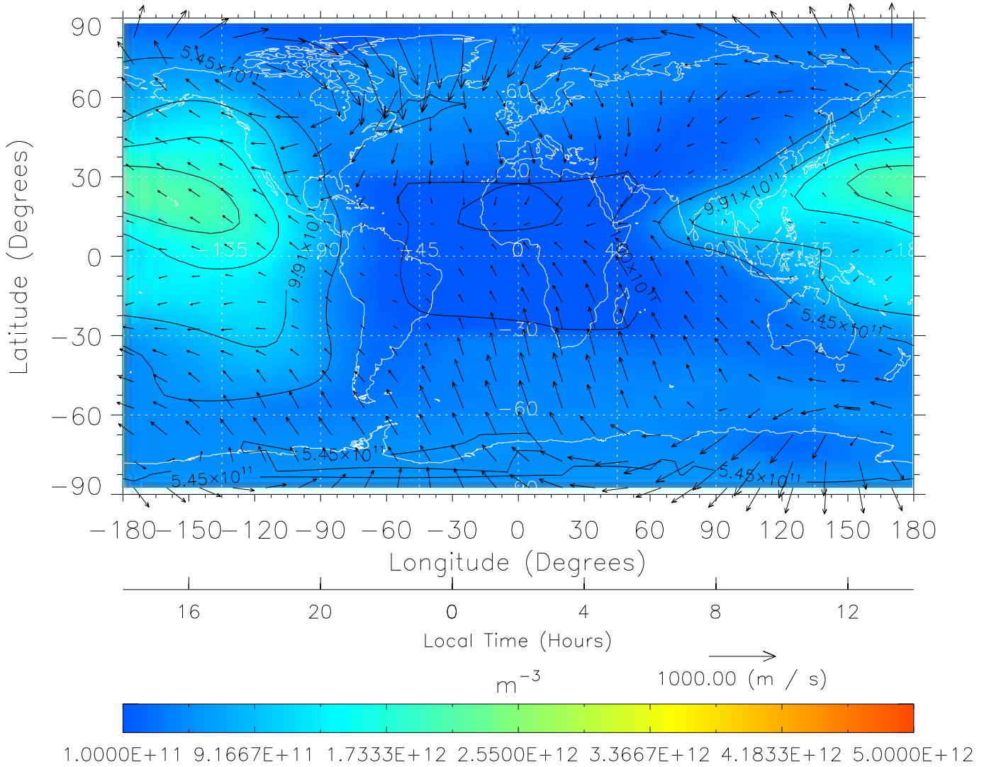
TIME-GCM MAP NmF2 with Neutral Wind vectors ZP = 2.00 UT = 2.00 DOY = 303
