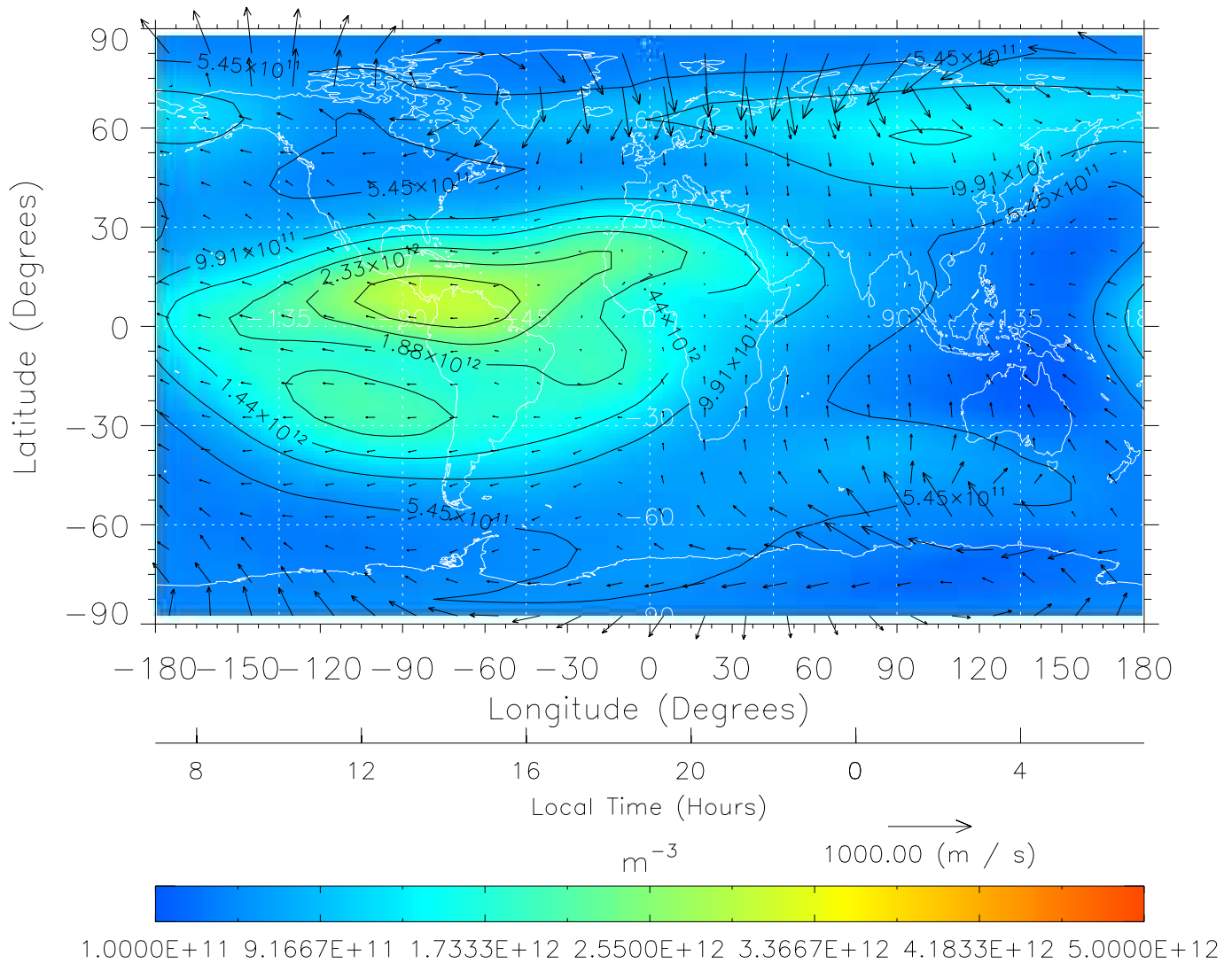
TIME-GCM MAP NmF2 with Neutral Wind vectors ZP = 2.00 UT = 19.00 DOY = 303
