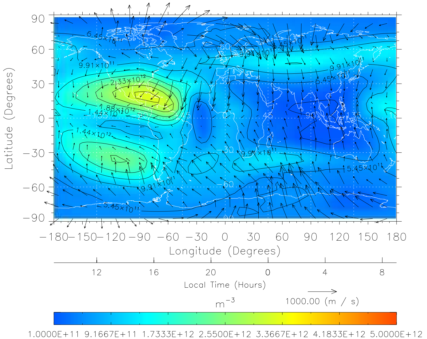
TIME-GCM MAP NmF2 with Neutral Wind vectors ZP = 2.00 UT = 21.00 DOY = 303
