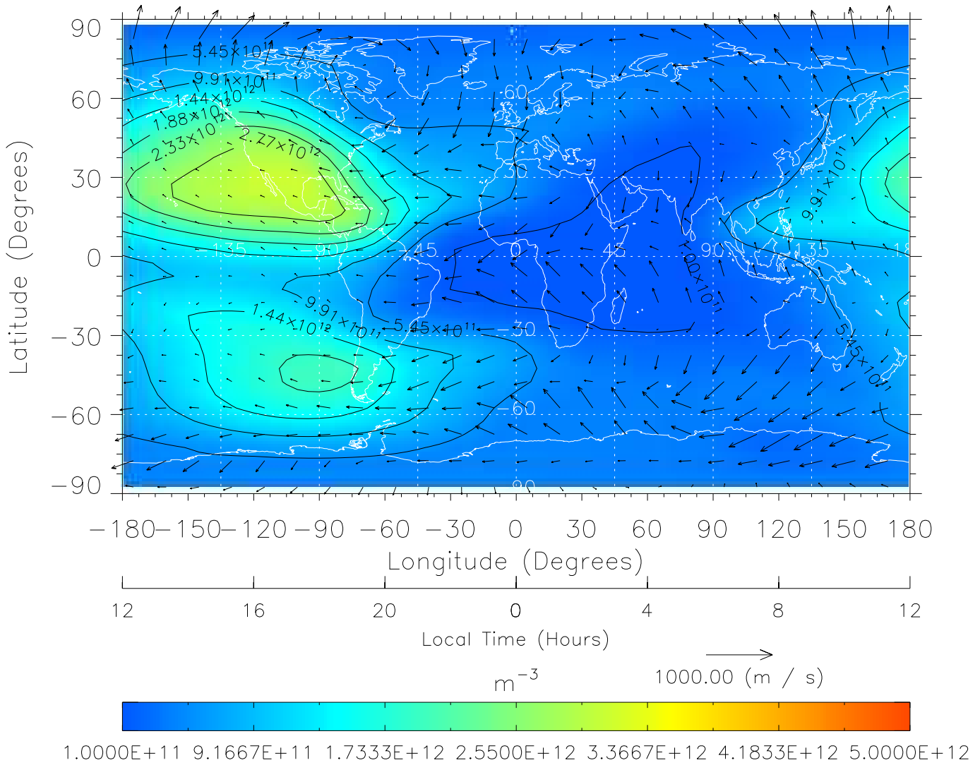
TIME-GCM MAP NmF2 with Neutral Wind vectors ZP = 2.00 UT = 0.00 DOY = 303
