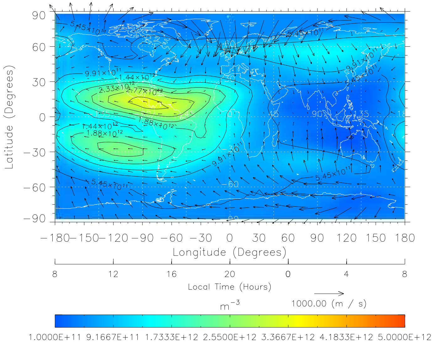
TIME-GCM MAP NmF2 with Neutral Wind vectors ZP = 2.00 UT = 20.00 DOY = 303
