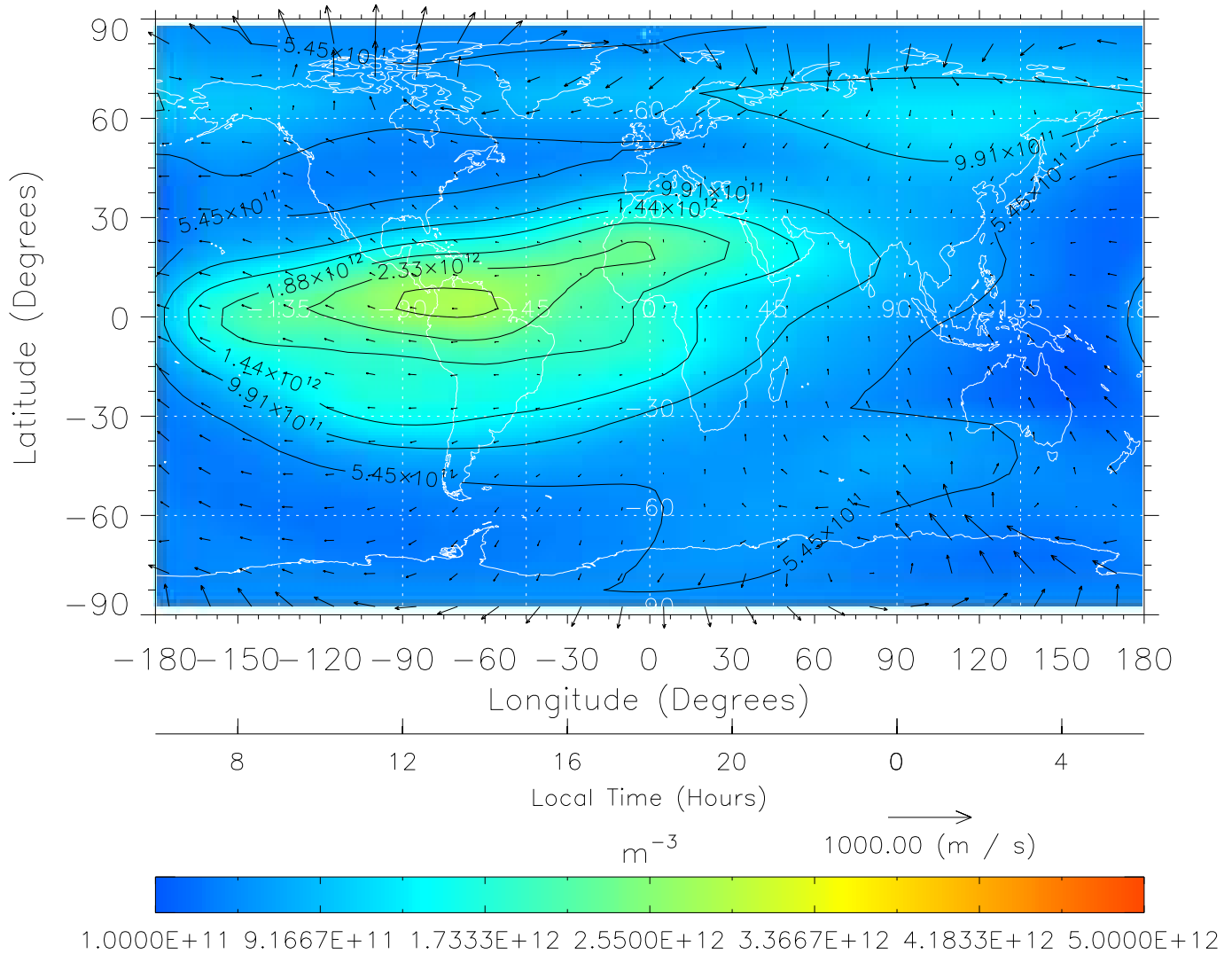
TIME-GCM MAP NmF2 with Neutral Wind vectors ZP = 2.00 UT = 18.00 DOY = 303
