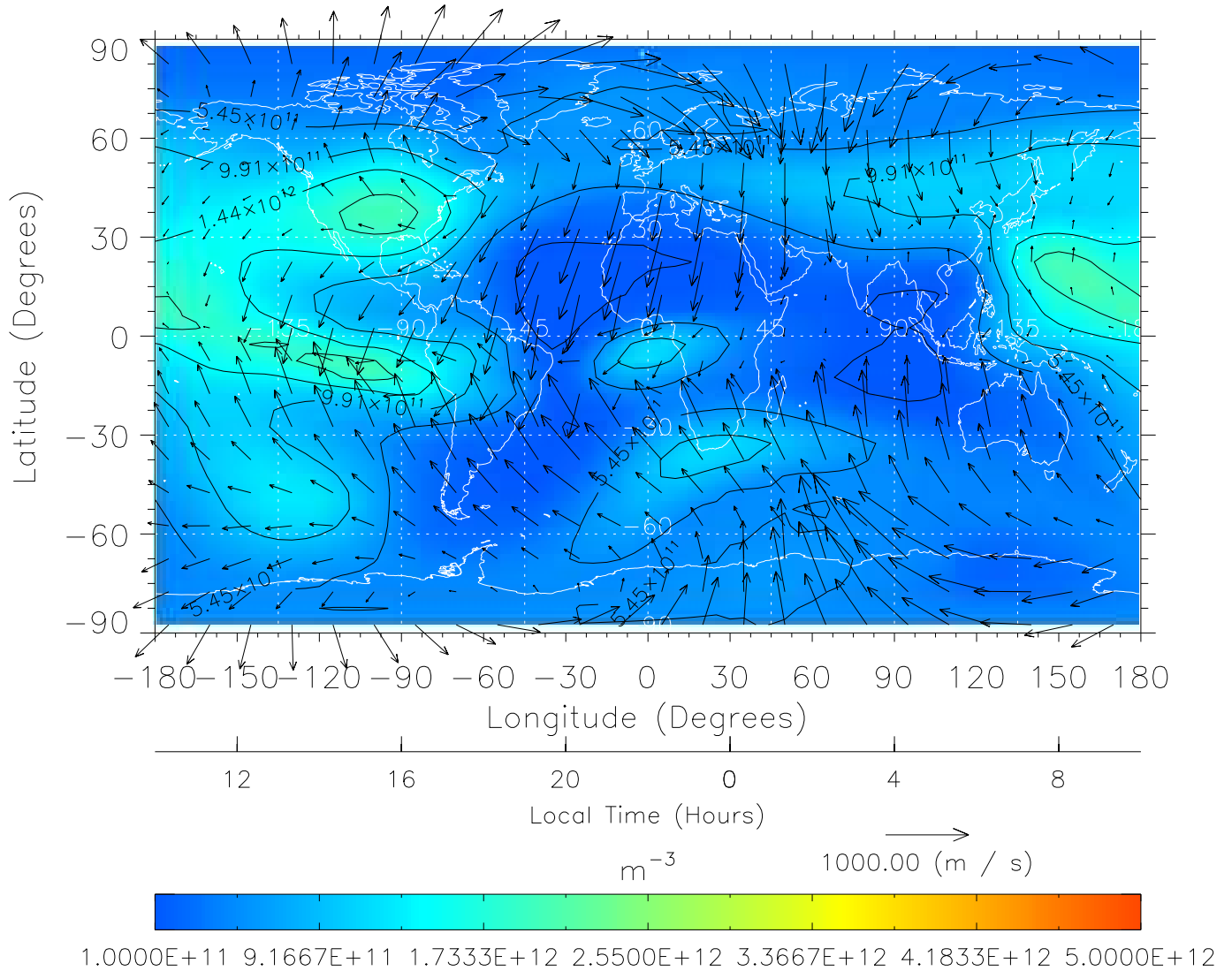
TIME-GCM MAP NmF2 with Neutral Wind vectors ZP = 2.00 UT = 22.00 DOY = 303
