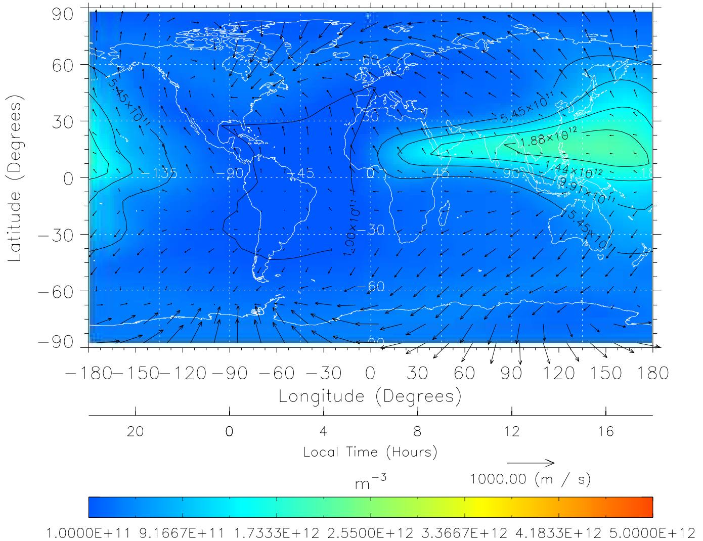
TIME-GCM MAP NmF2 with Neutral Wind vectors ZP = 2.00 UT = 6.00 DOY = 303
