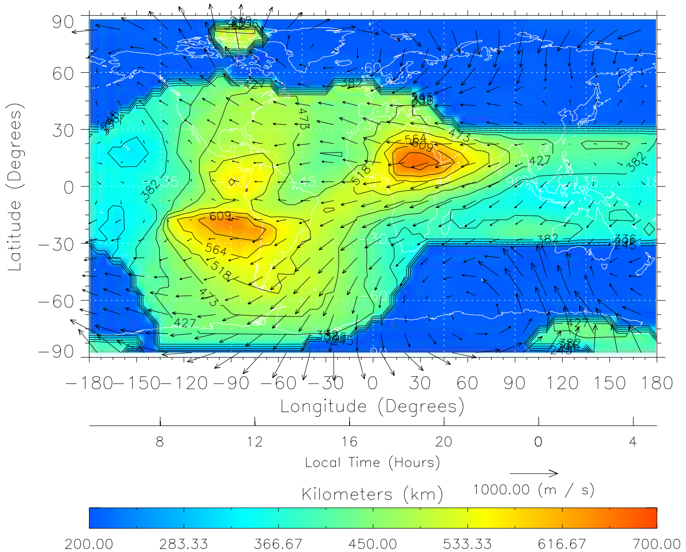
TIME-GCM MAP hmF2 with Neutral Wind vectors ZP = 2.00 UT = 17.00 DOY = 324
