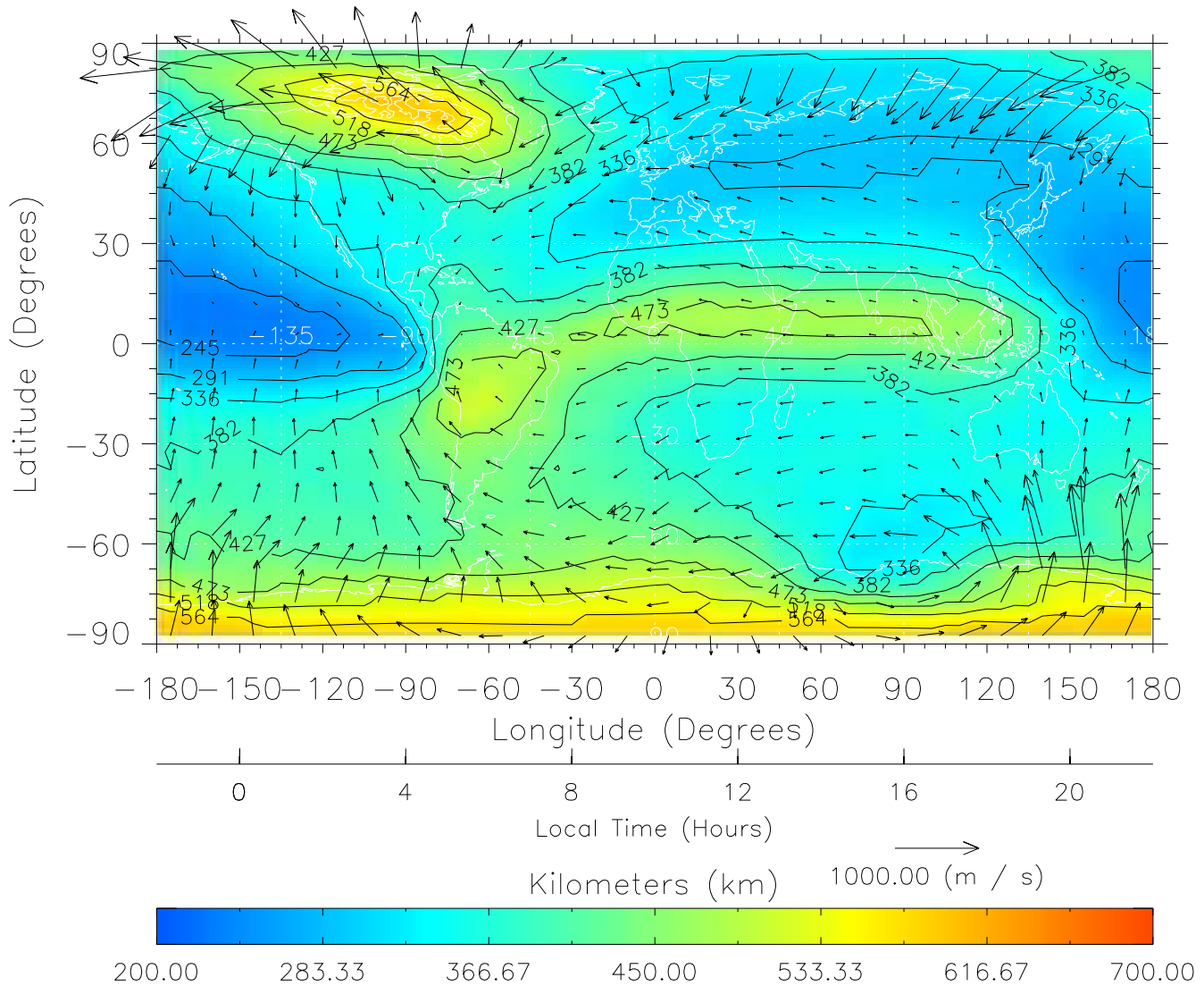
TIME-GCM MAP hmF2 with Neutral Wind vectors ZP = 2.00 UT = 10.00 DOY = 324
