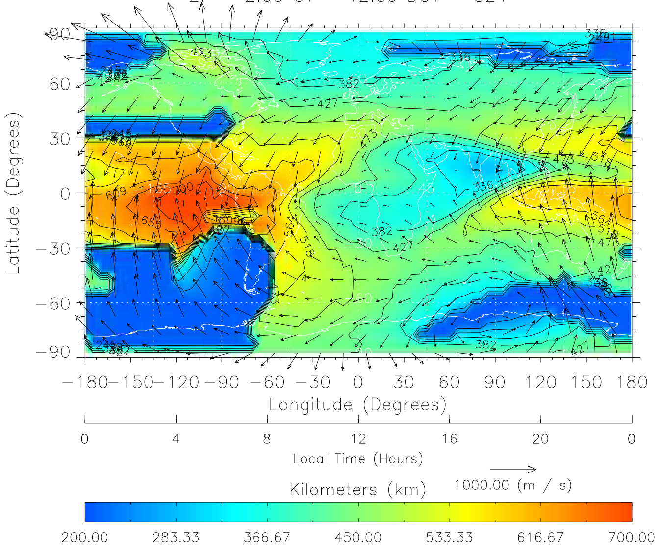
TIME-GCM MAP hmF2 with Neutral Wind vectors ZP = 2.00 UT = 12.00 DOY = 324
