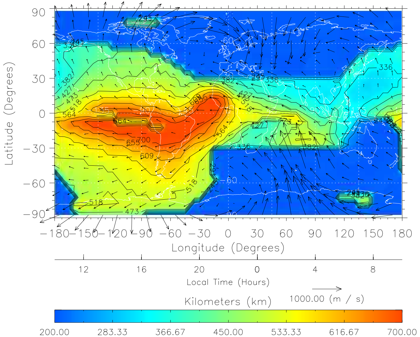
TIME-GCM MAP hmF2 with Neutral Wind vectors ZP = 2.00 UT = 22.00 DOY = 324
