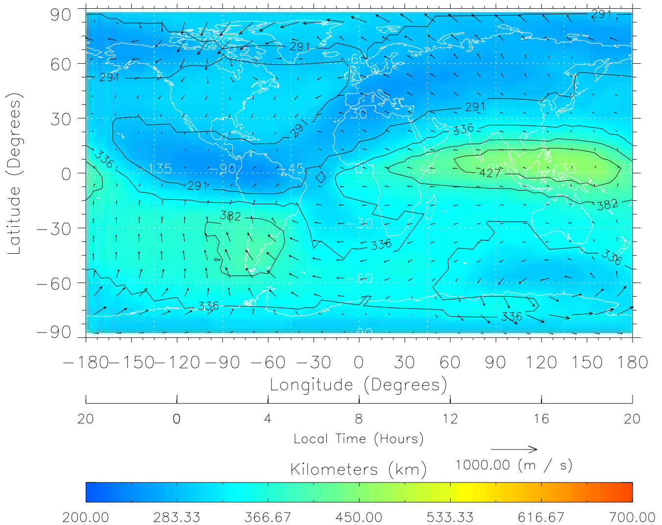
TIME-GCM MAP hmF2 with Neutral Wind vectors ZP = 2.00 UT = 8.00 DOY = 324
