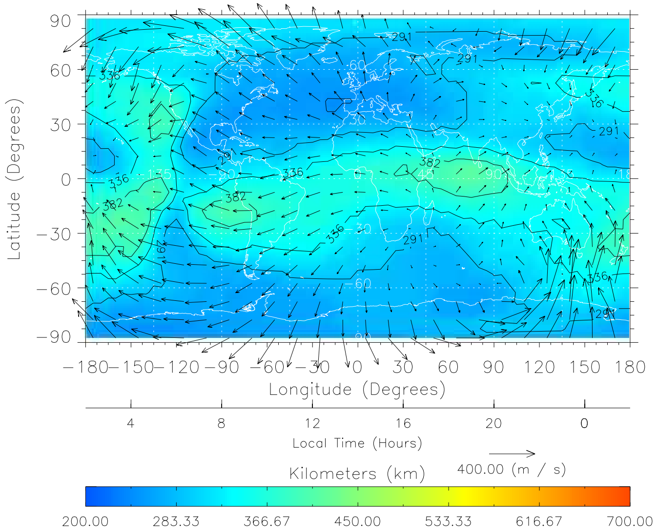
TIME-GCM MAP hmF2 with Neutral Wind vectors ZP = 2.00 UT = 14.00 DOY = 305
