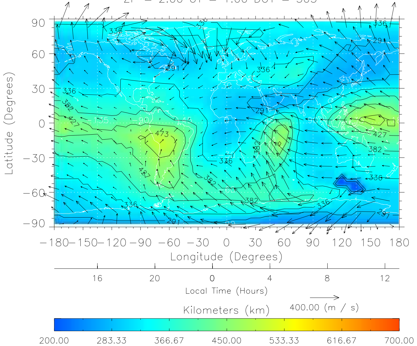
TIME-GCM MAP hmF2 with Neutral Wind vectors ZP = 2.00 UT = 1.00 DOY = 305
