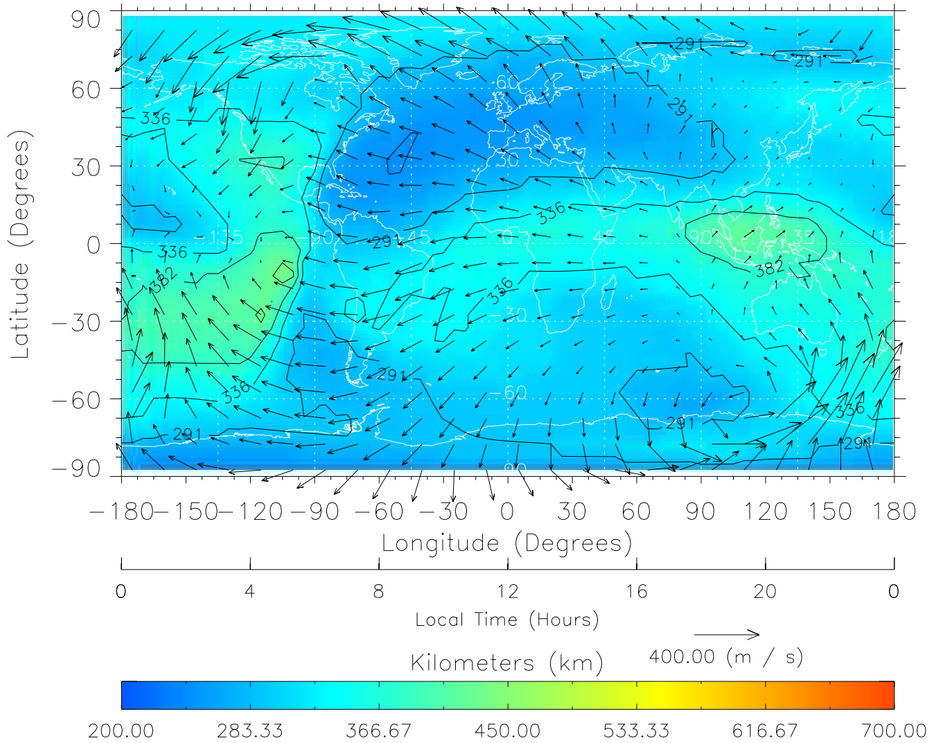
TIME-GCM MAP hmF2 with Neutral Wind vectors ZP = 2.00 UT = 12.00 DOY = 305
