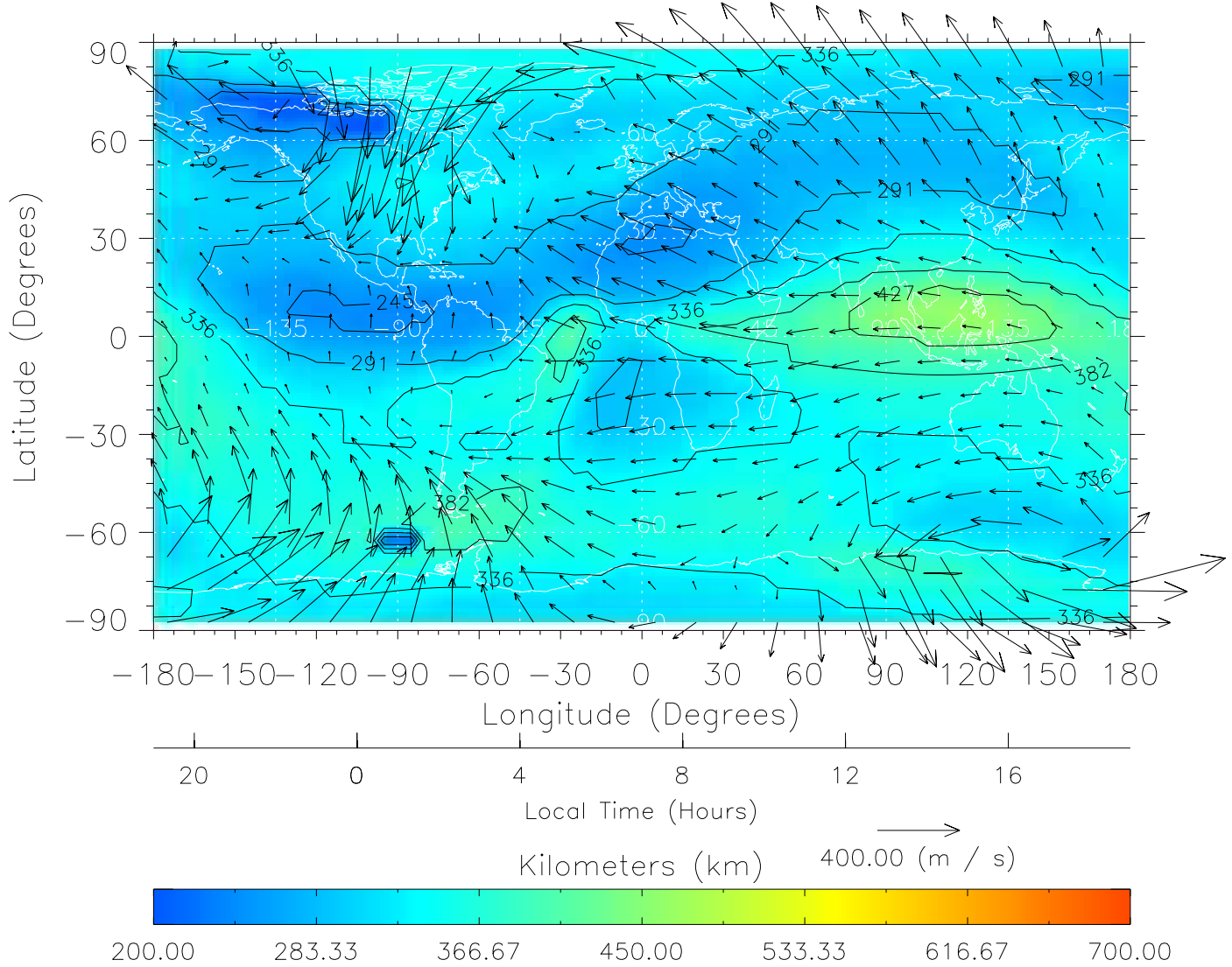
TIME-GCM MAP hmF2 with Neutral Wind vectors ZP = 2.00 UT = 7.00 DOY = 305
