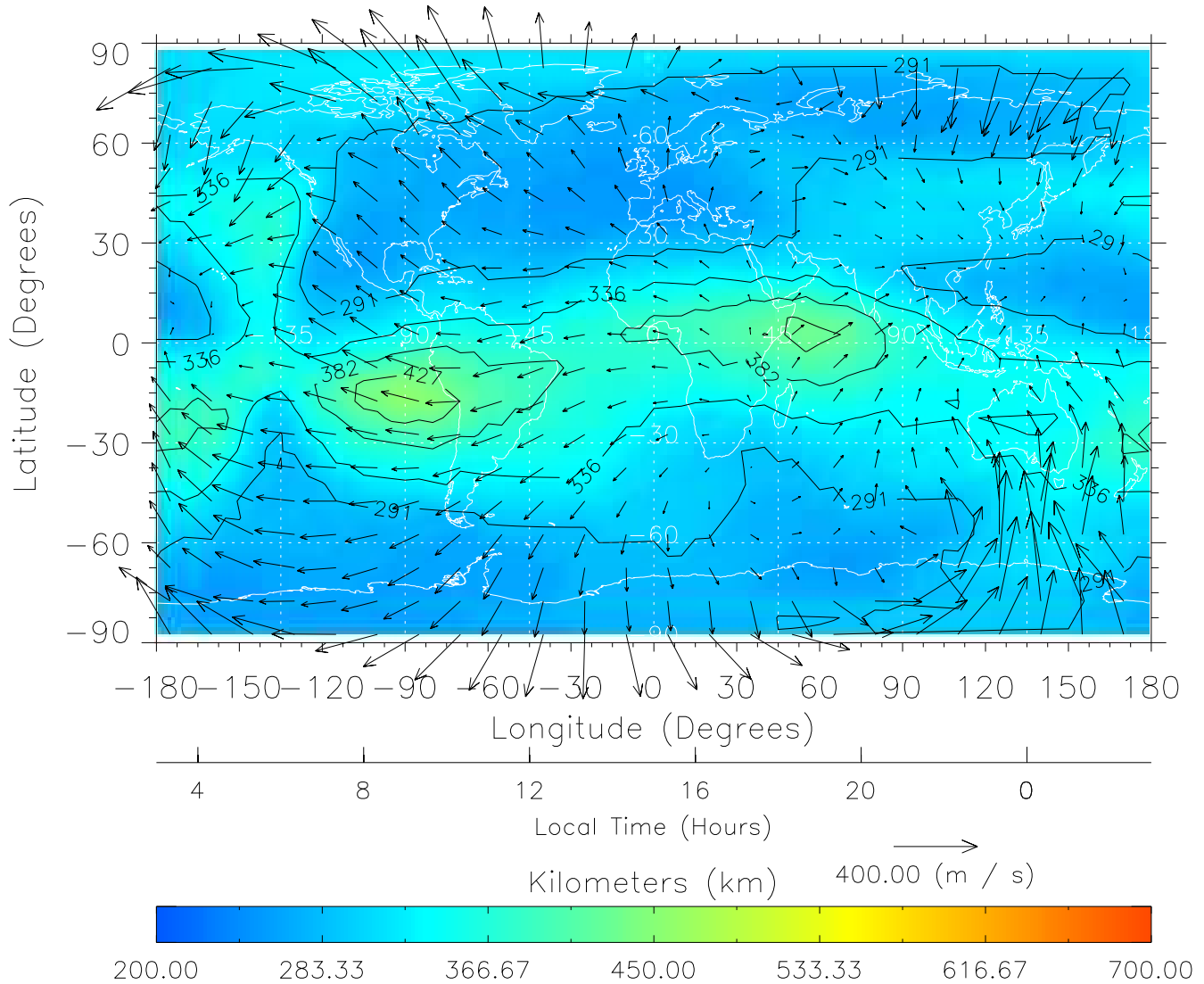
TIME-GCM MAP hmF2 with Neutral Wind vectors ZP = 2.00 UT = 15.00 DOY = 305
