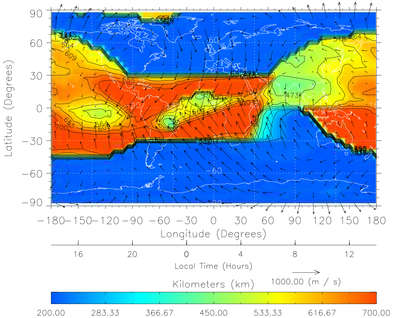
TIME-GCM MAP hmF2 with Neutral Wind vectors ZP = 2.00 UT = 2.00 DOY = 304
