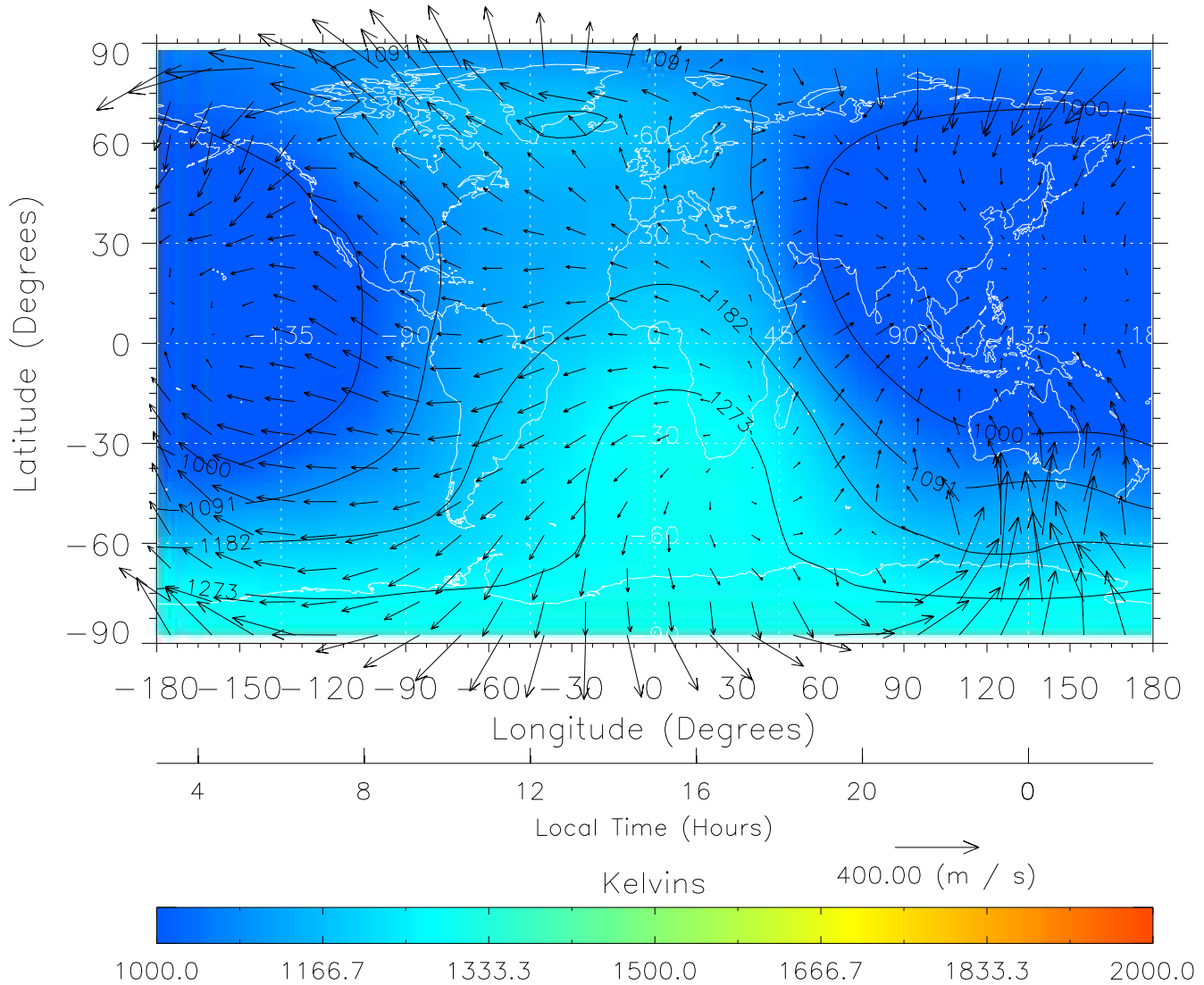
TIME-GCM MAP Temperature with Neutral Wind vectors ZP = 2.00 UT = 15.00 DOY = 305
