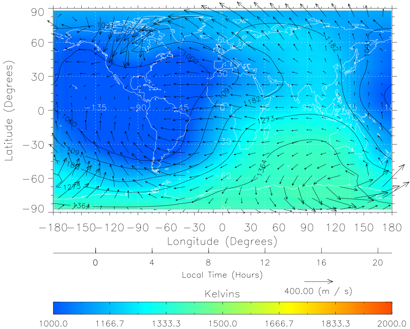
TIME-GCM MAP Temperature with Neutral Wind vectors ZP = 2.00 UT = 9.00 DOY = 305
