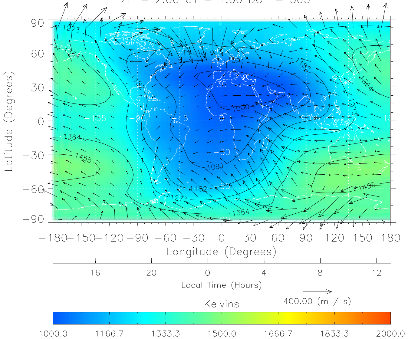
TIME-GCM MAP Temperature with Neutral Wind vectors ZP = 2.00 UT = 1.00 DOY = 305
