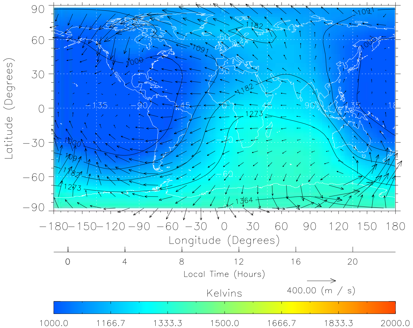
TIME-GCM MAP Temperature with Neutral Wind vectors ZP = 2.00 UT = 11.00 DOY = 305
