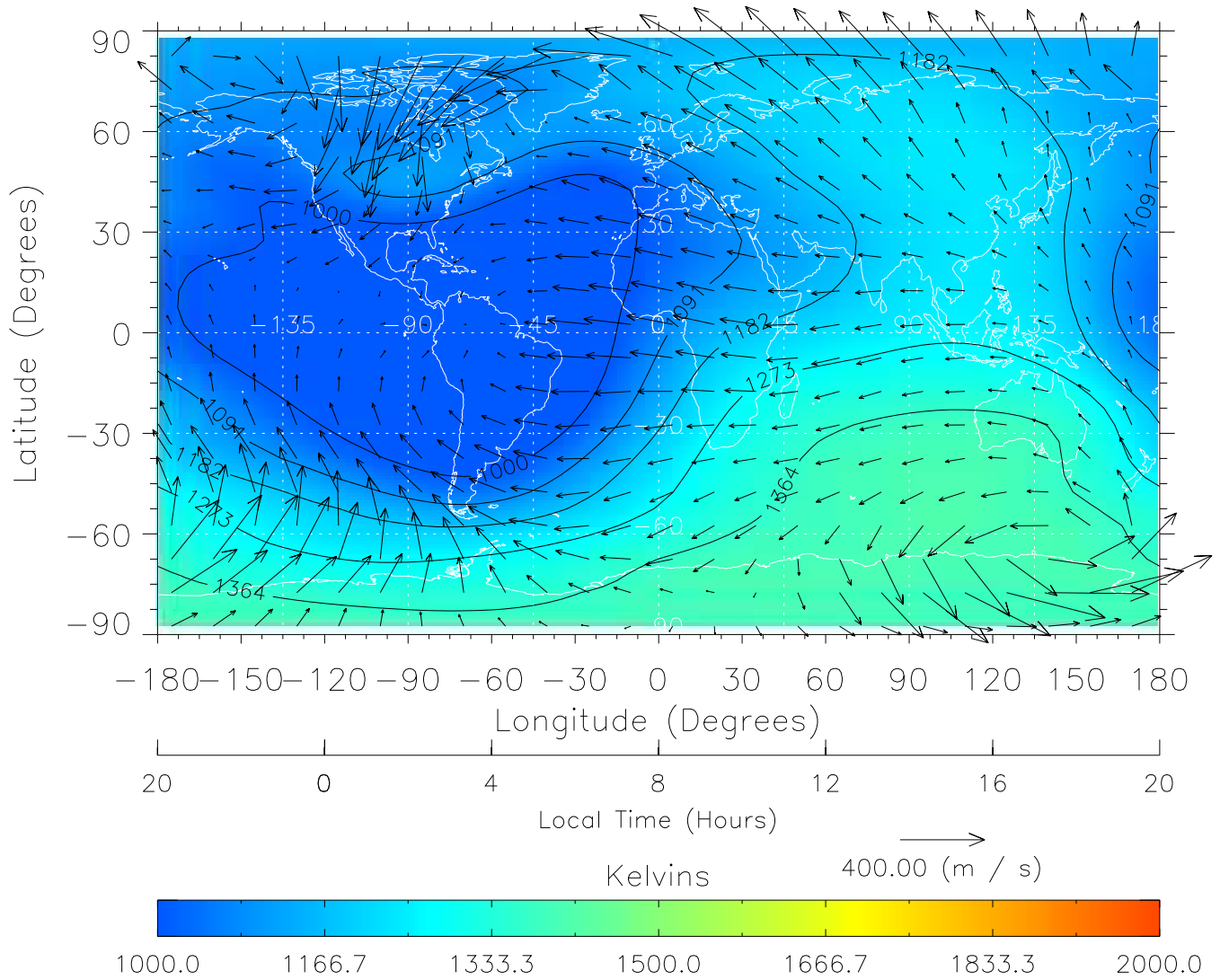
TIME-GCM MAP Temperature with Neutral Wind vectors ZP = 2.00 UT = 8.00 DOY = 305
