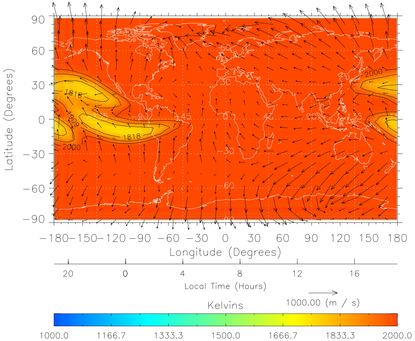
TIME-GCM MAP Temperature with Neutral Wind vectors ZP = 2.00 UT = 7.00 DOY = 304
