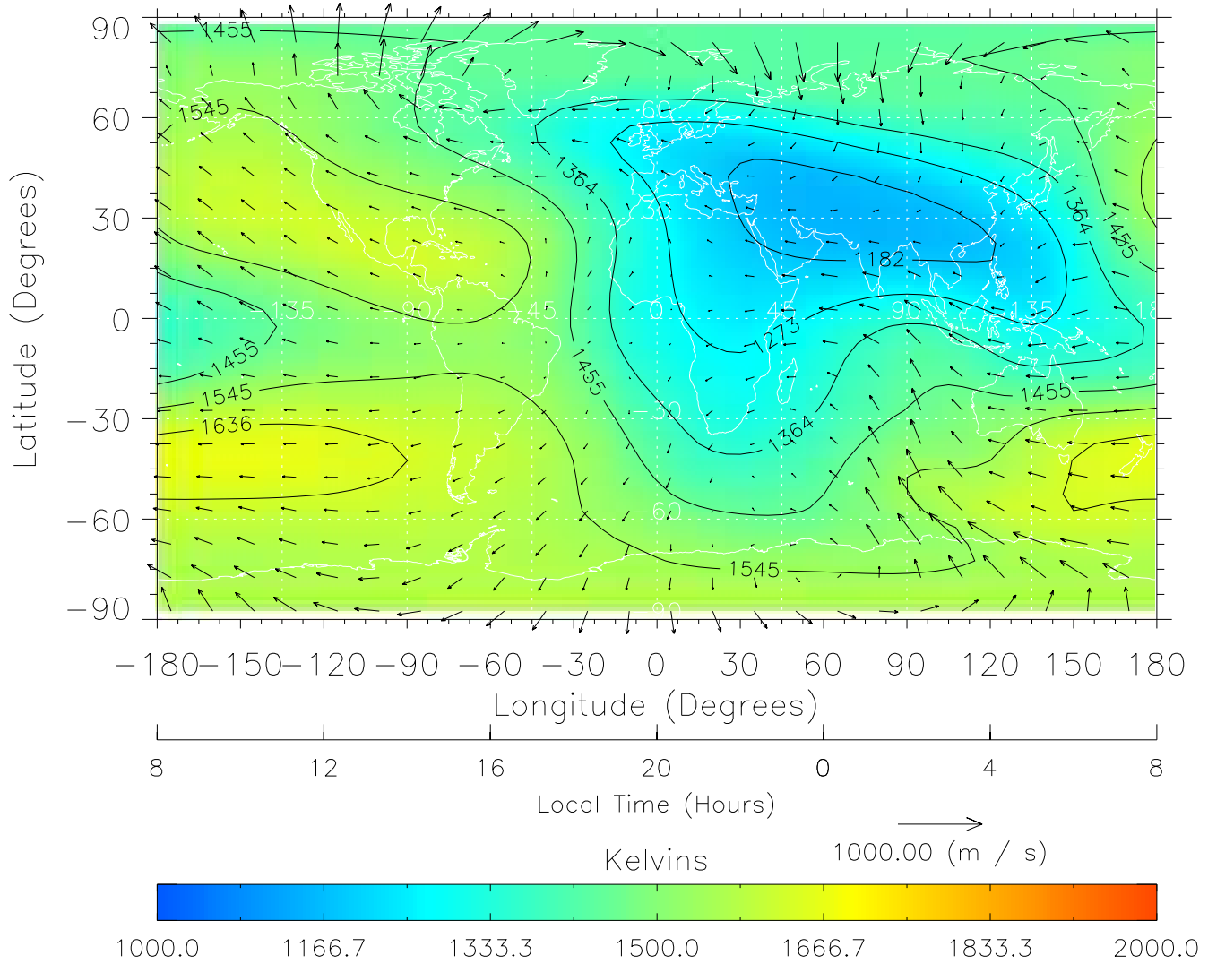
TIME-GCM MAP Temperature with Neutral Wind vectors ZP = 2.00 UT = 20.00 DOY = 304
