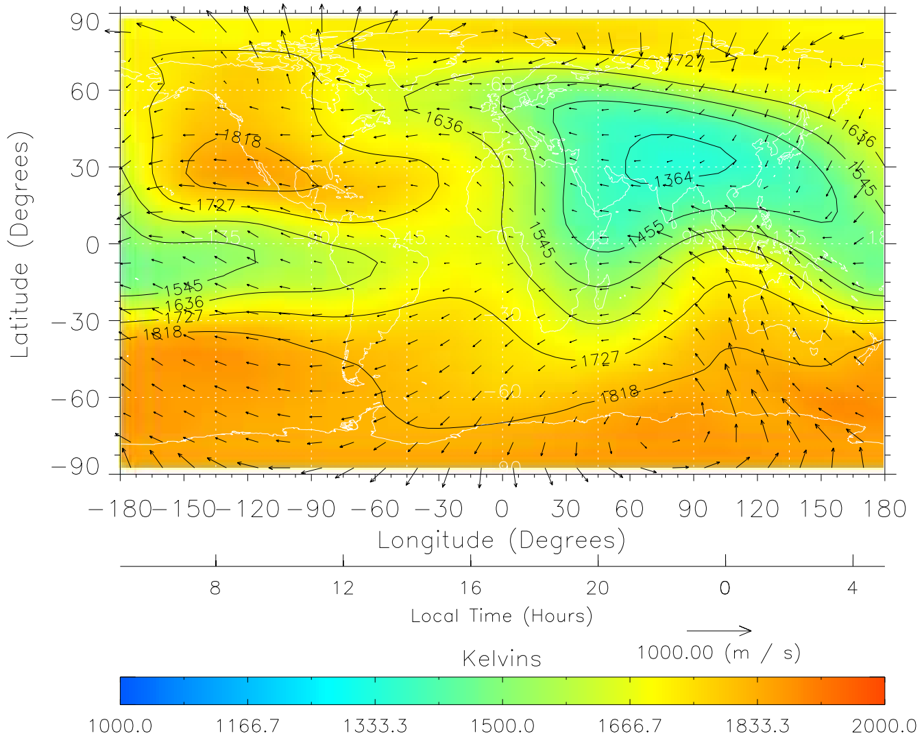
TIME-GCM MAP Temperature with Neutral Wind vectors ZP = 2.00 UT = 17.00 DOY = 304
