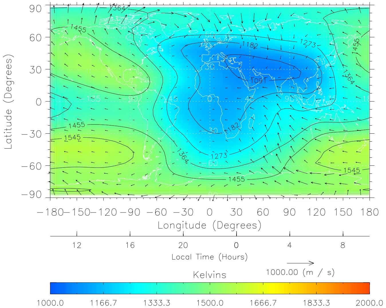
TIME-GCM MAP Temperature with Neutral Wind vectors ZP = 2.00 UT = 22.00 DOY = 304
