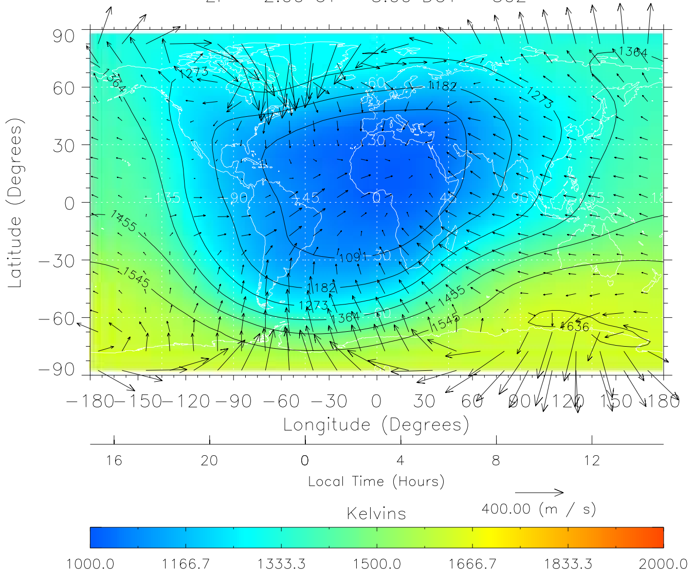
TIME-GCM MAP Temperature with Neutral Wind vectors ZP = 2.00 UT = 3.00 DOY = 302
