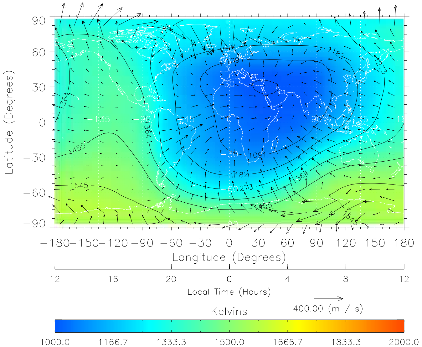
TIME-GCM MAP Temperature with Neutral Wind vectors ZP = 2.00 UT = 0.00 DOY = 302
