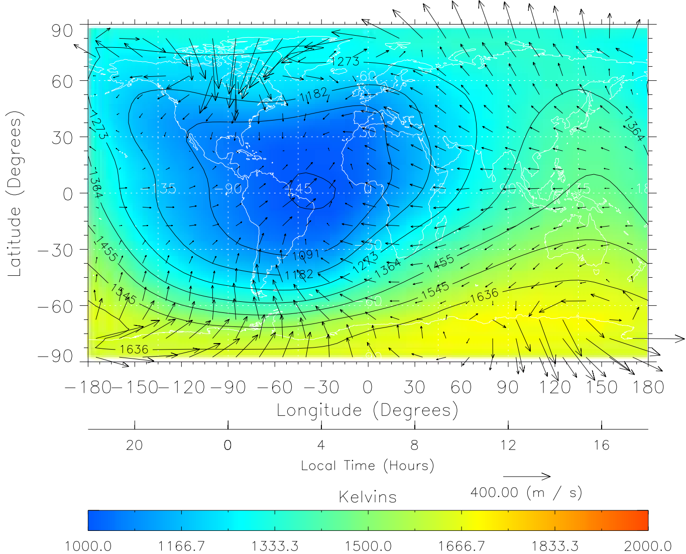
TIME-GCM MAP Temperature with Neutral Wind vectors ZP = 2.00 UT = 6.00 DOY = 302
