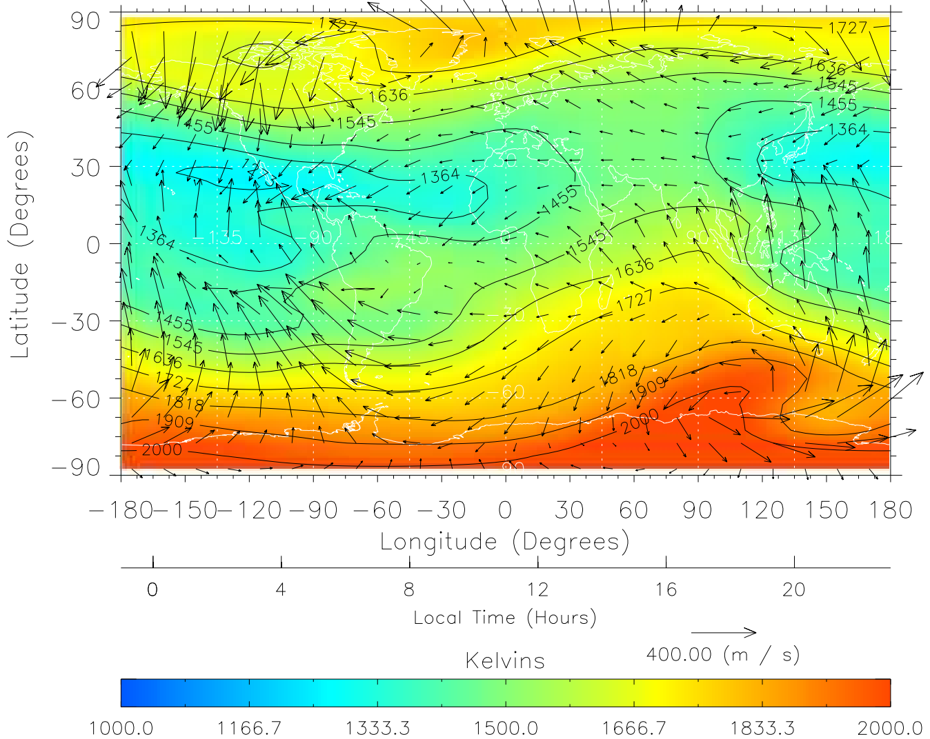
TIME-GCM MAP Temperature with Neutral Wind vectors ZP = 2.00 UT = 11.00 DOY = 302
