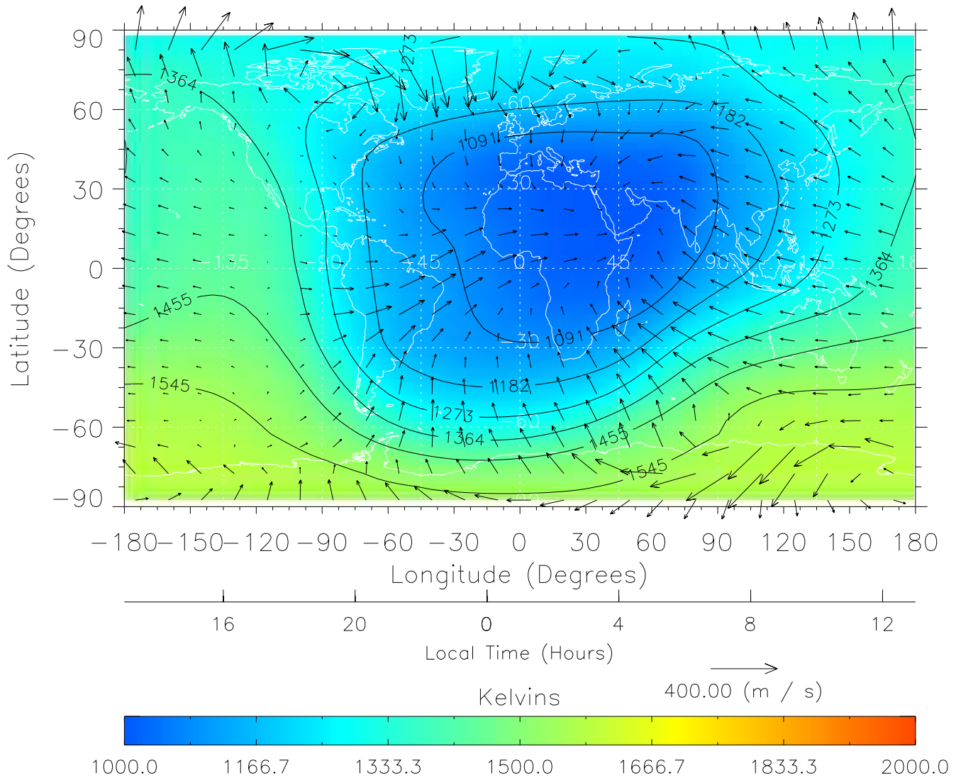
TIME-GCM MAP Temperature with Neutral Wind vectors ZP = 2.00 UT = 1.00 DOY = 302
