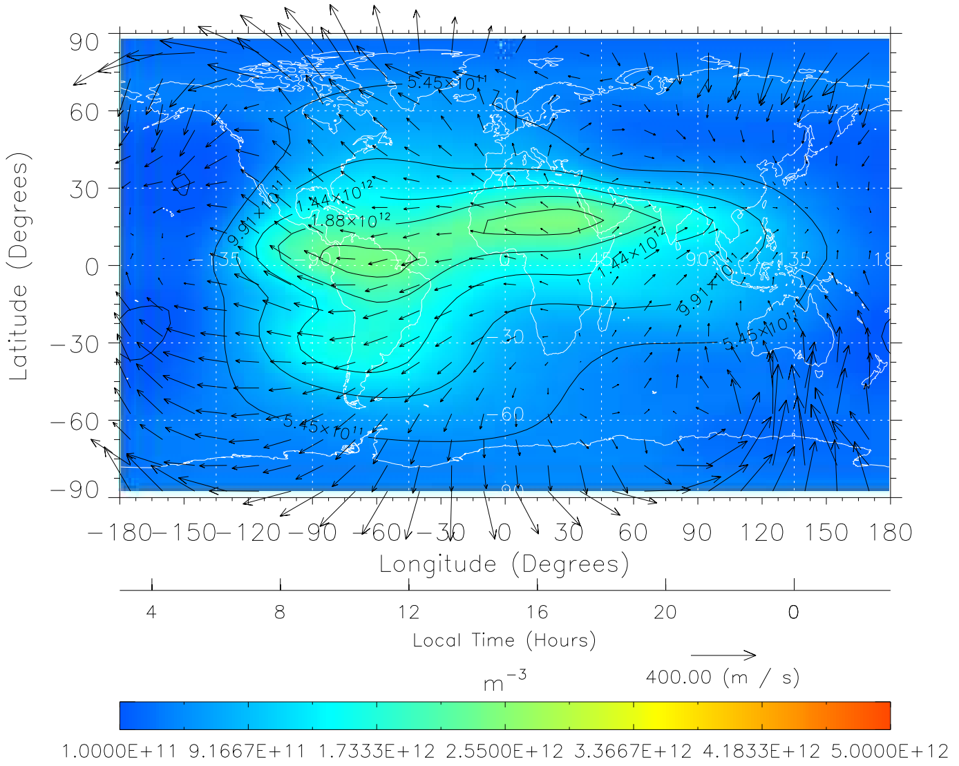
TIME-GCM MAP NmF2 with Neutral Wind vectors ZP = 2.00 UT = 15.00 DOY = 305
