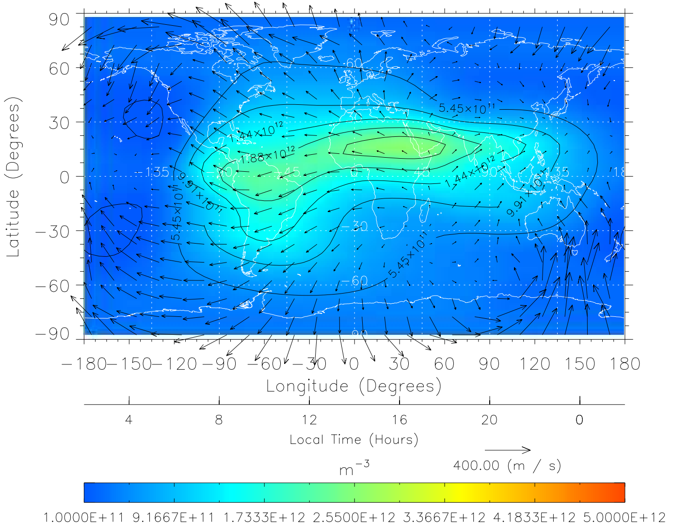
TIME-GCM MAP NmF2 with Neutral Wind vectors ZP = 2.00 UT = 14.00 DOY = 305
