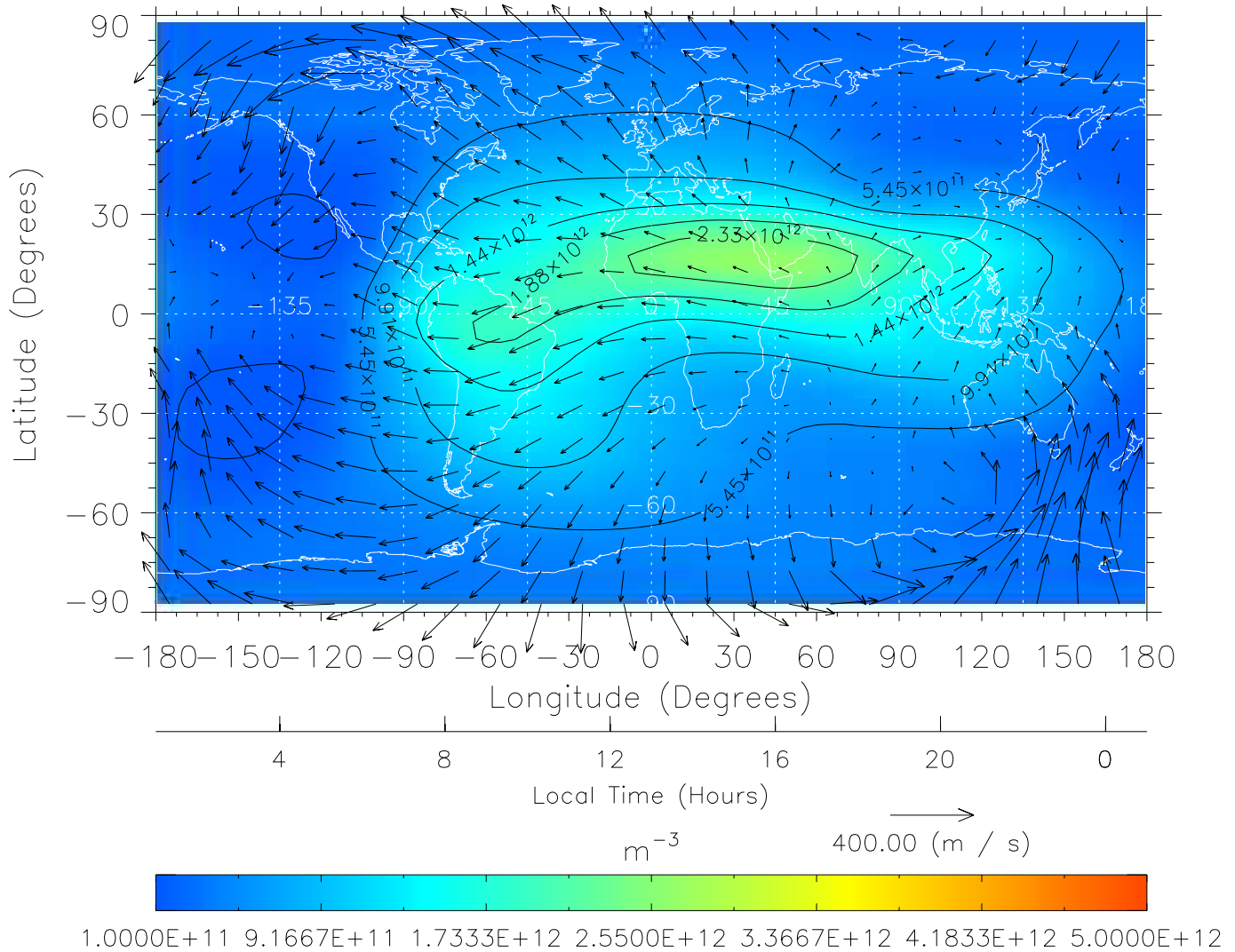
TIME-GCM MAP NmF2 with Neutral Wind vectors ZP = 2.00 UT = 13.00 DOY = 305
