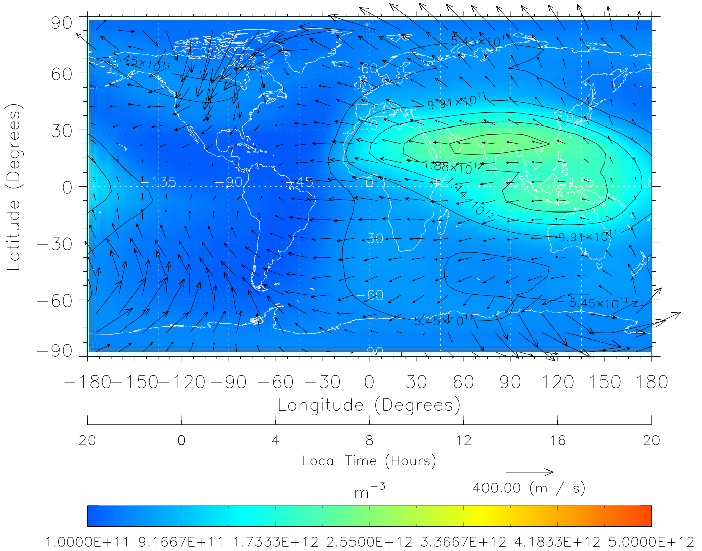
TIME-GCM MAP NmF2 with Neutral Wind vectors ZP = 2.00 UT = 8.00 DOY = 305
