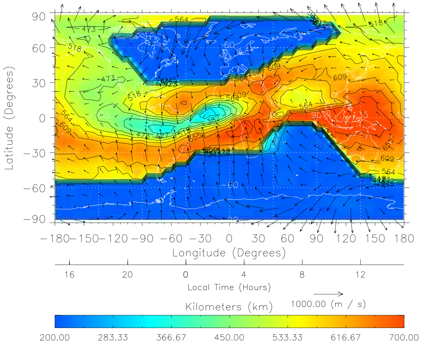
TIME-GCM MAP hmF2 with Neutral Wind vectors ZP = 2.00 UT = 3.00 DOY = 303
