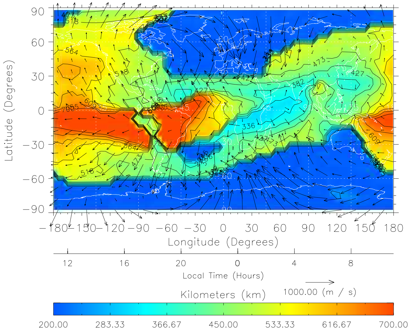
TIME-GCM MAP hmF2 with Neutral Wind vectors ZP = 2.00 UT = 23.00 DOY = 303
