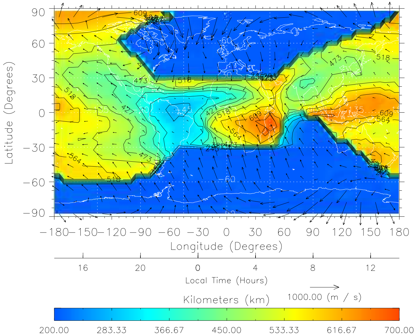
TIME-GCM MAP hmF2 with Neutral Wind vectors ZP = 2.00 UT = 2.00 DOY = 303
