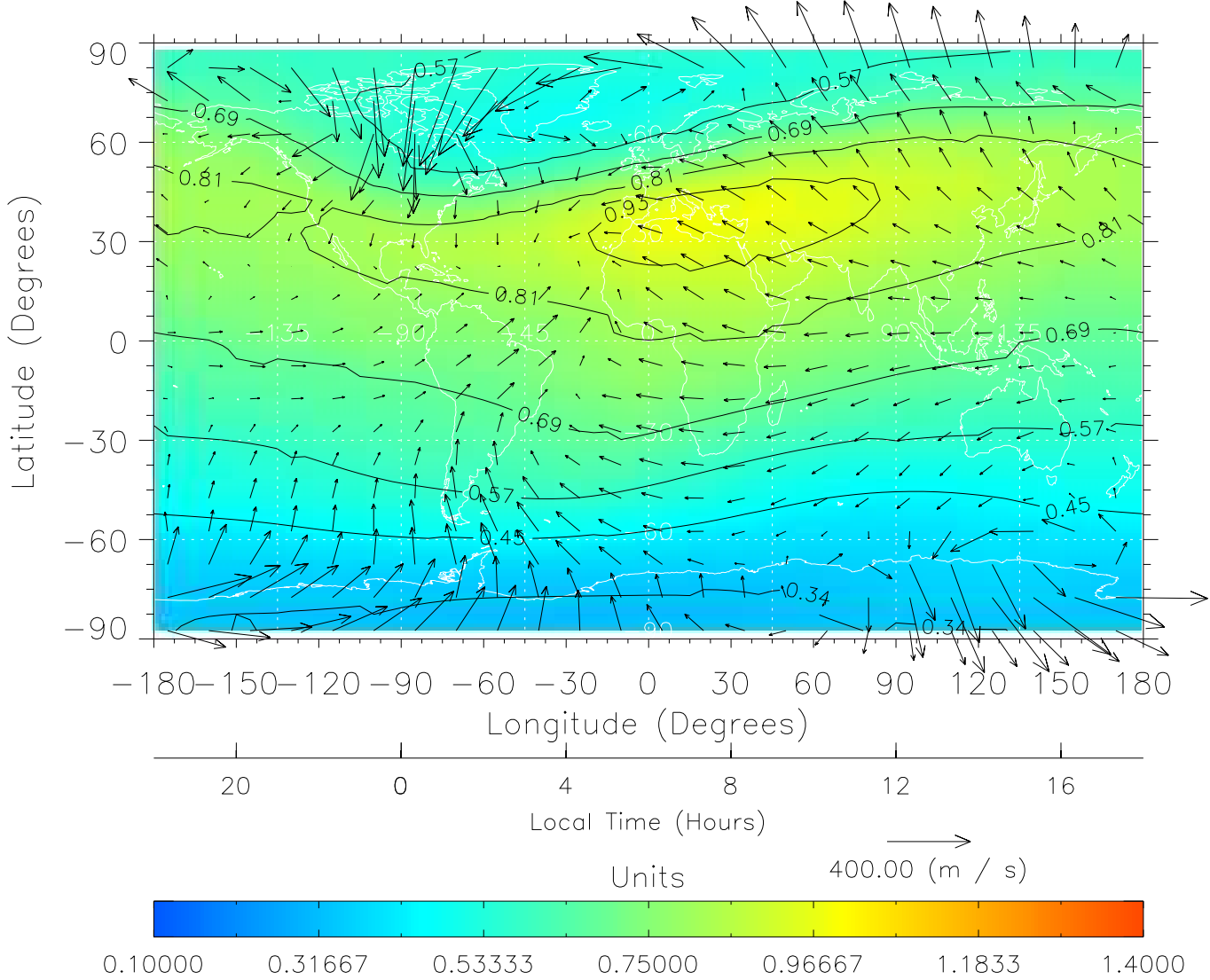
TIME-GCM MAP \Sigma O/N_2 with Neutral Wind vectors ZP = 2.00 UT = 6.00 DOY = 302
