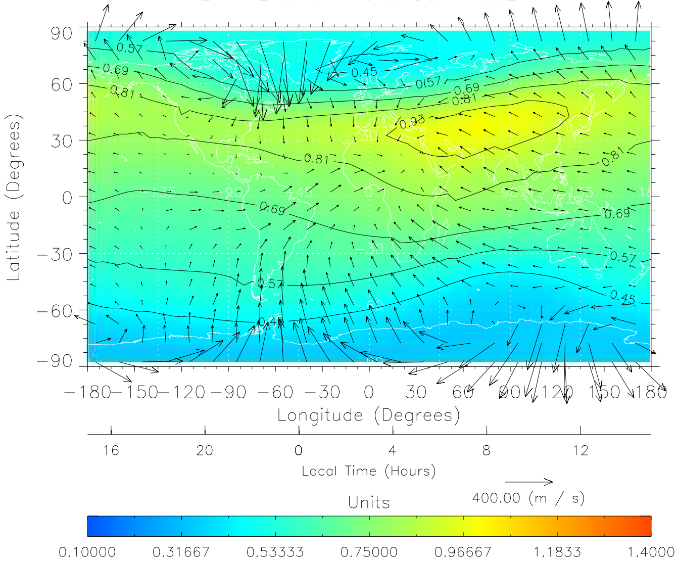
TIME-GCM MAP \Sigma O/N_2 with Neutral Wind vectors ZP = 2.00 UT = 3.00 DOY = 302
