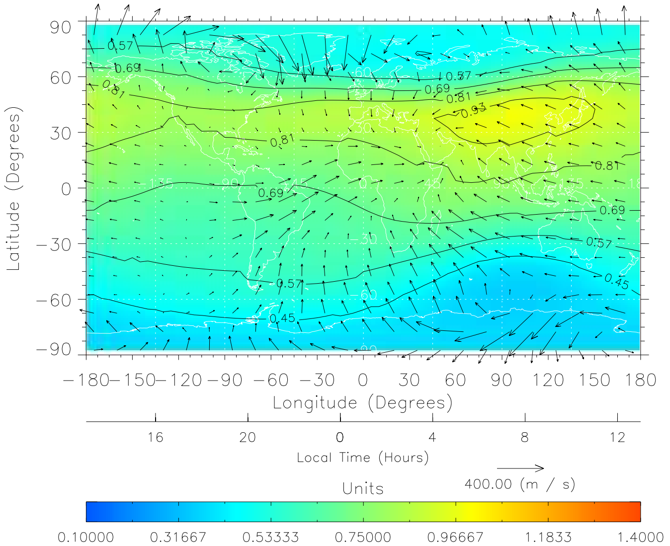
TIME-GCM MAP \Sigma O/N_2 with Neutral Wind vectors ZP = 2.00 UT = 1.00 DOY = 302
