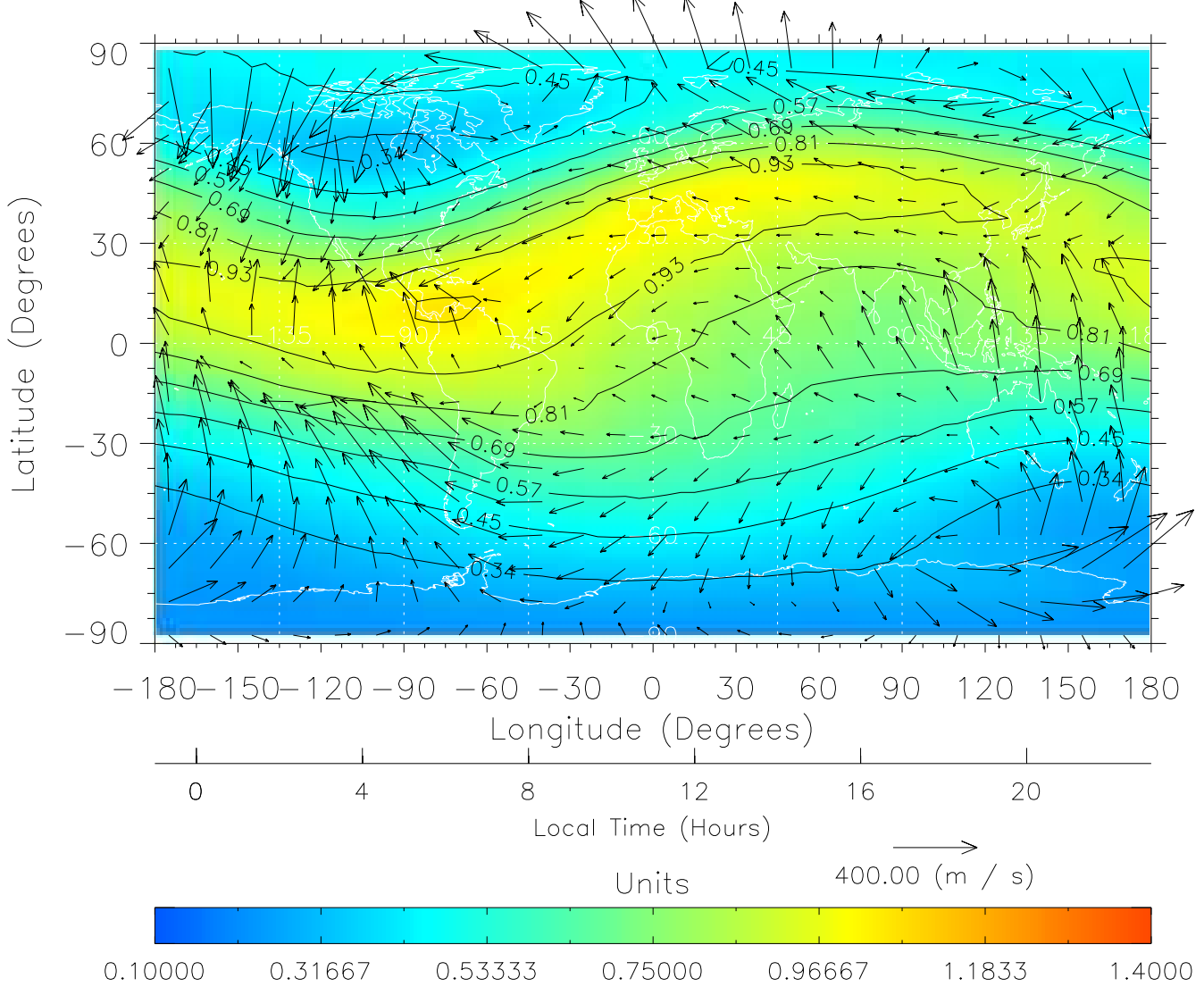
TIME-GCM MAP \Sigma O/N_2 with Neutral Wind vectors ZP = 2.00 UT = 11.00 DOY = 302
