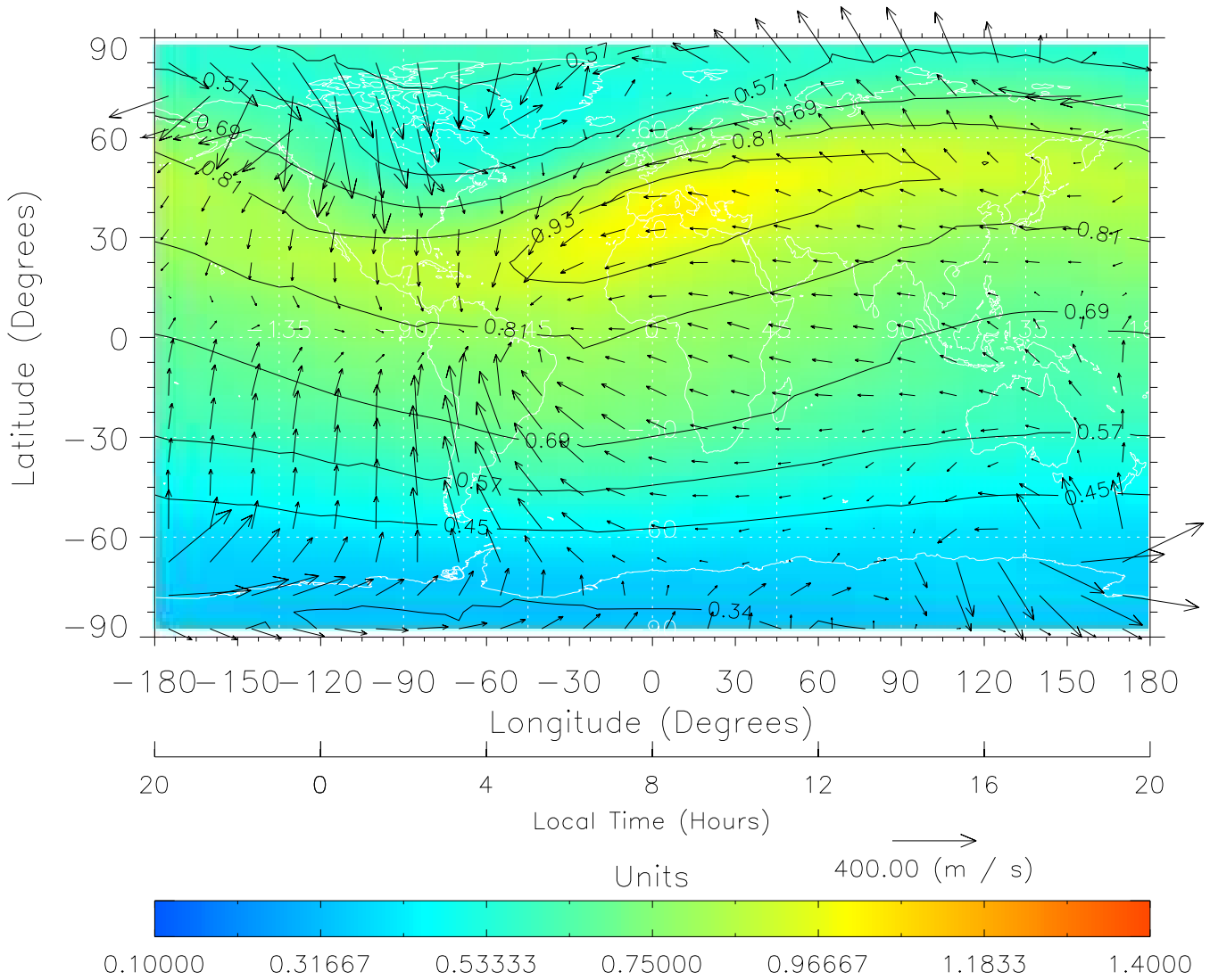
TIME-GCM MAP \Sigma O/N_2 with Neutral Wind vectors ZP = 2.00 UT = 8.00 DOY = 302
