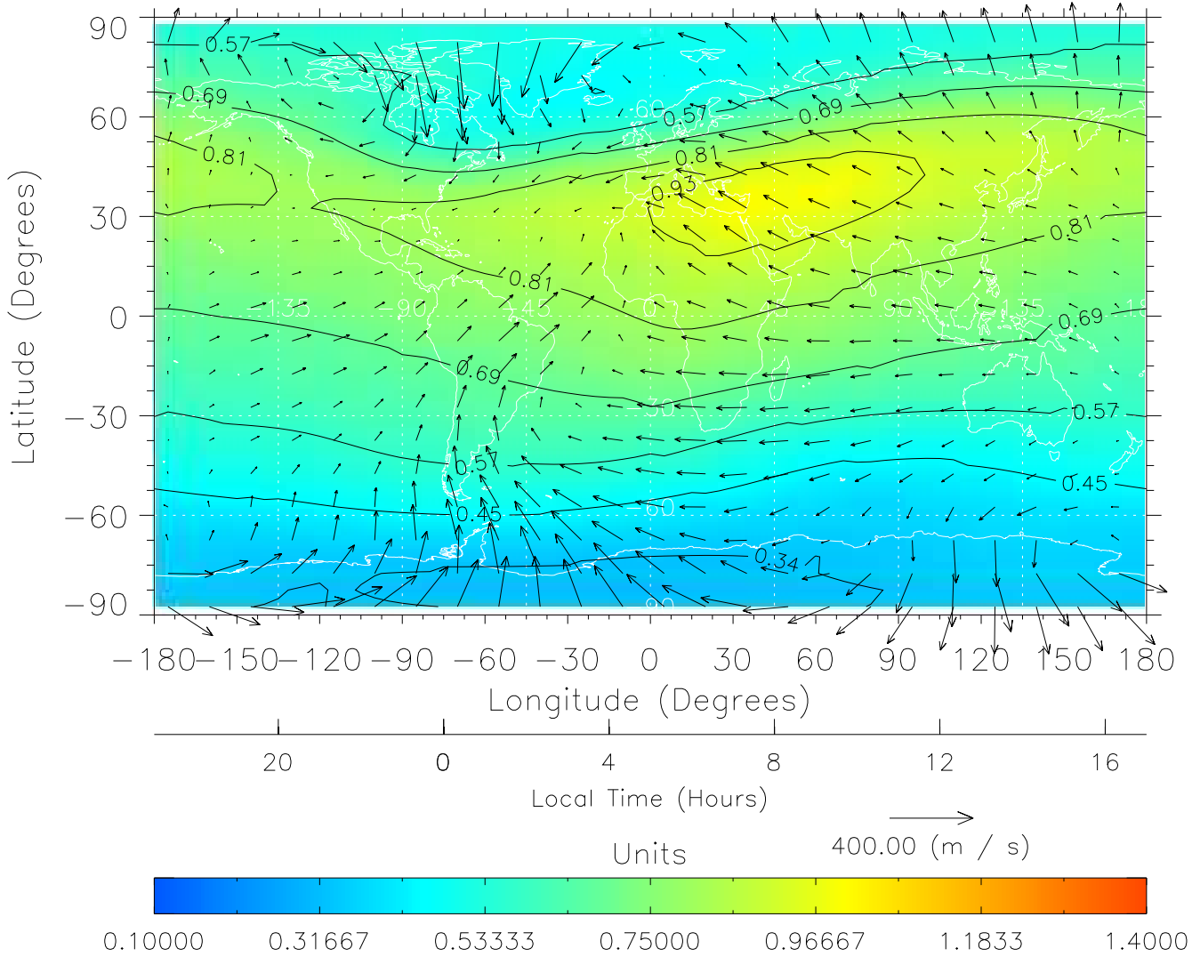
TIME-GCM MAP \Sigma O/N_2 with Neutral Wind vectors ZP = 2.00 UT = 5.00 DOY = 302
