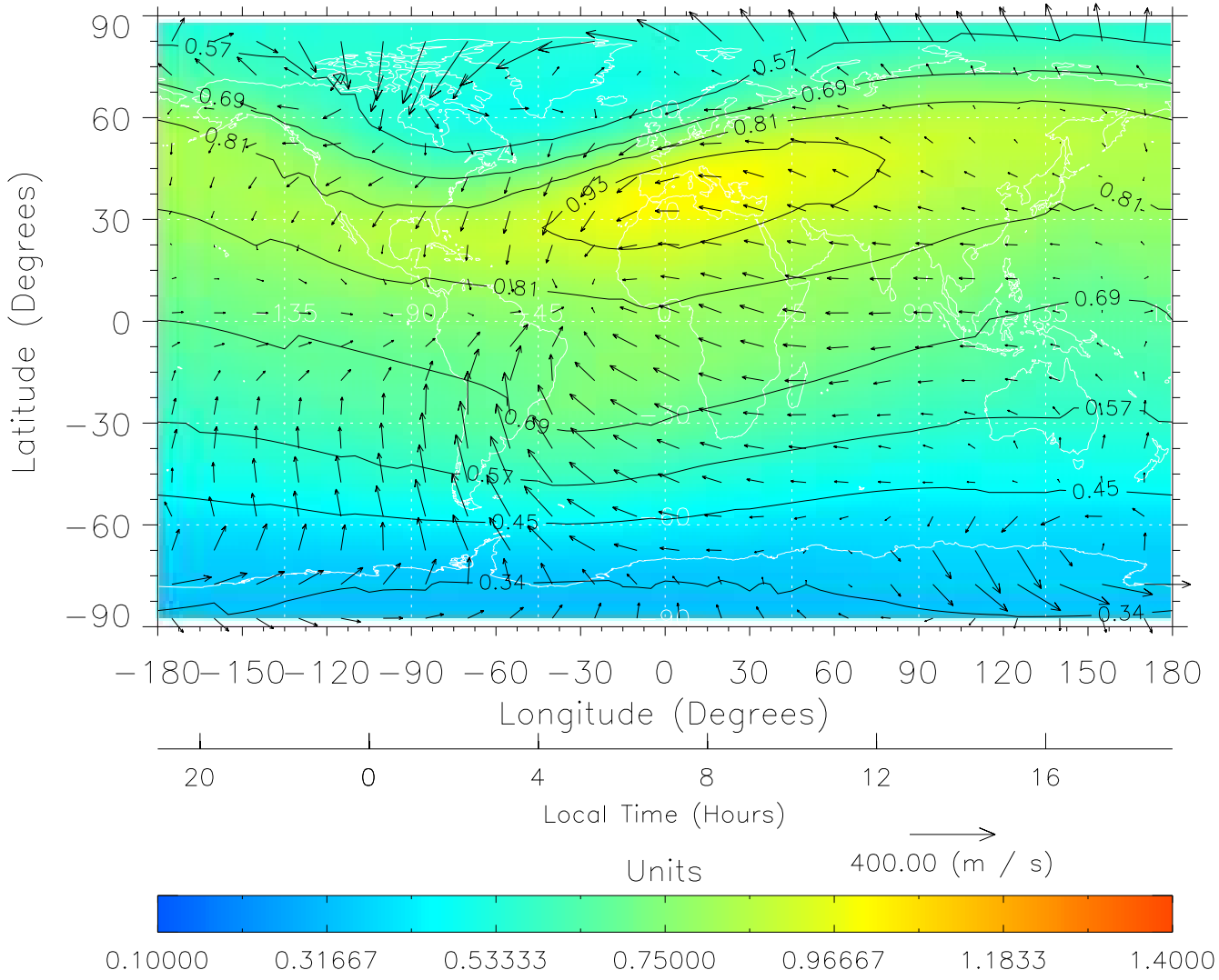
TIME-GCM MAP \Sigma O/N_2 with Neutral Wind vectors ZP = 2.00 UT = 7.00 DOY = 302
