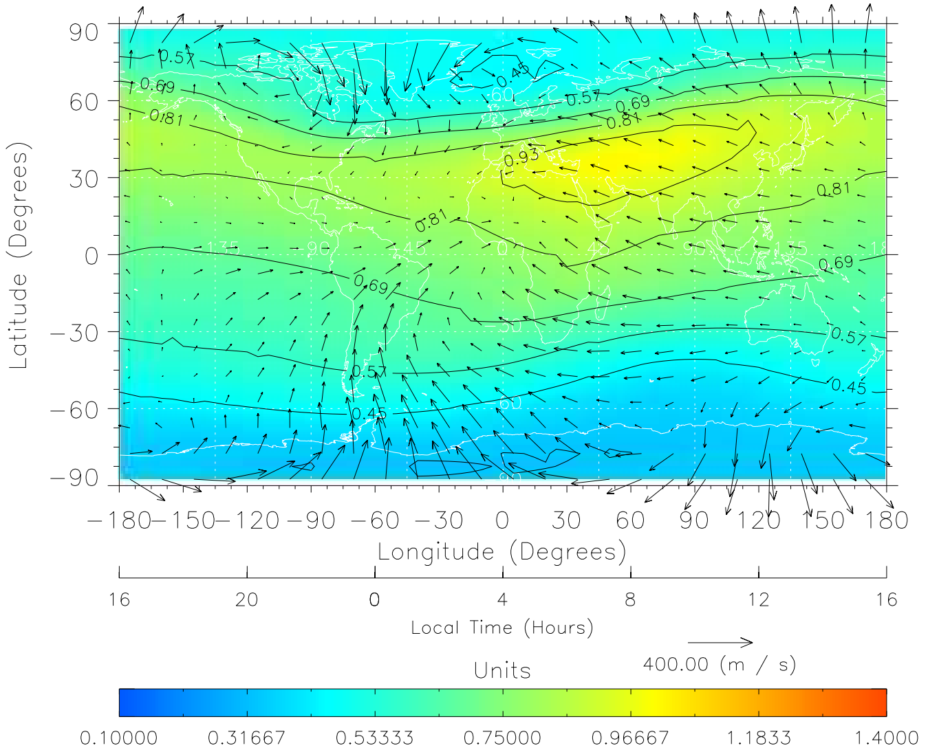
TIME-GCM MAP \Sigma O/N_2 with Neutral Wind vectors ZP = 2.00 UT = 4.00 DOY = 302
