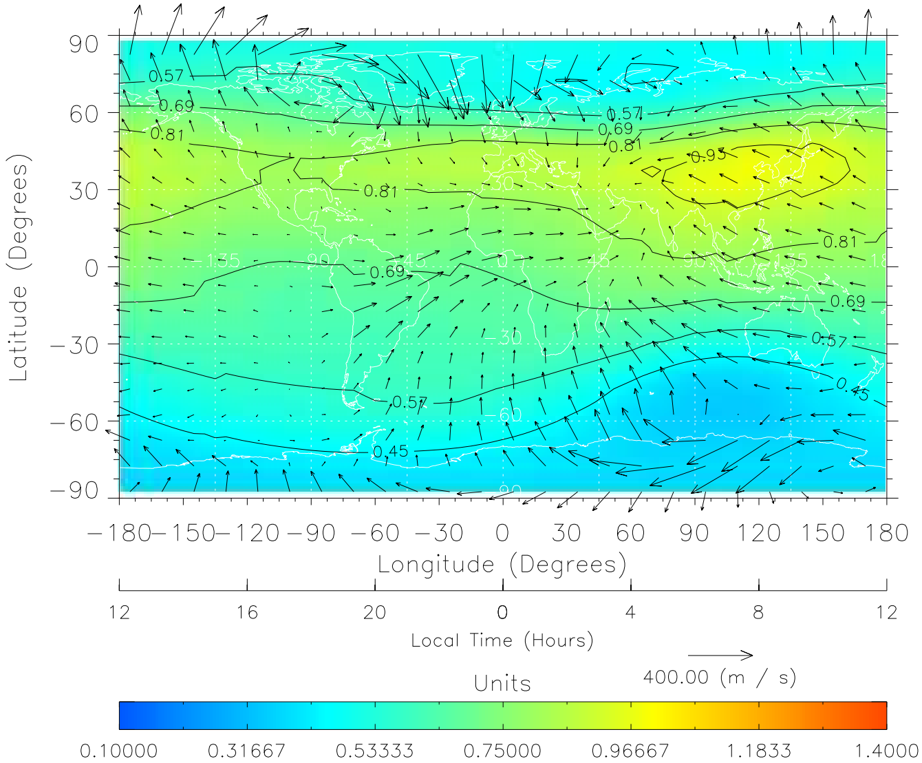
TIME-GCM MAP \Sigma O/N_2 with Neutral Wind vectors ZP = 2.00 UT = 0.00 DOY = 302
