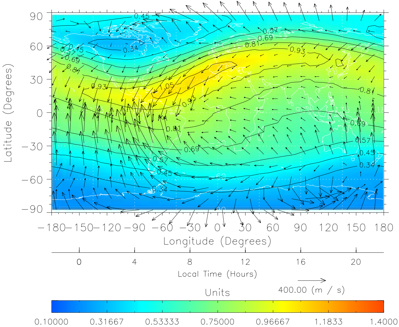
TIME-GCM MAP \Sigma O/N_2 with Neutral Wind vectors ZP = 2.00 UT = 10.00 DOY = 302
