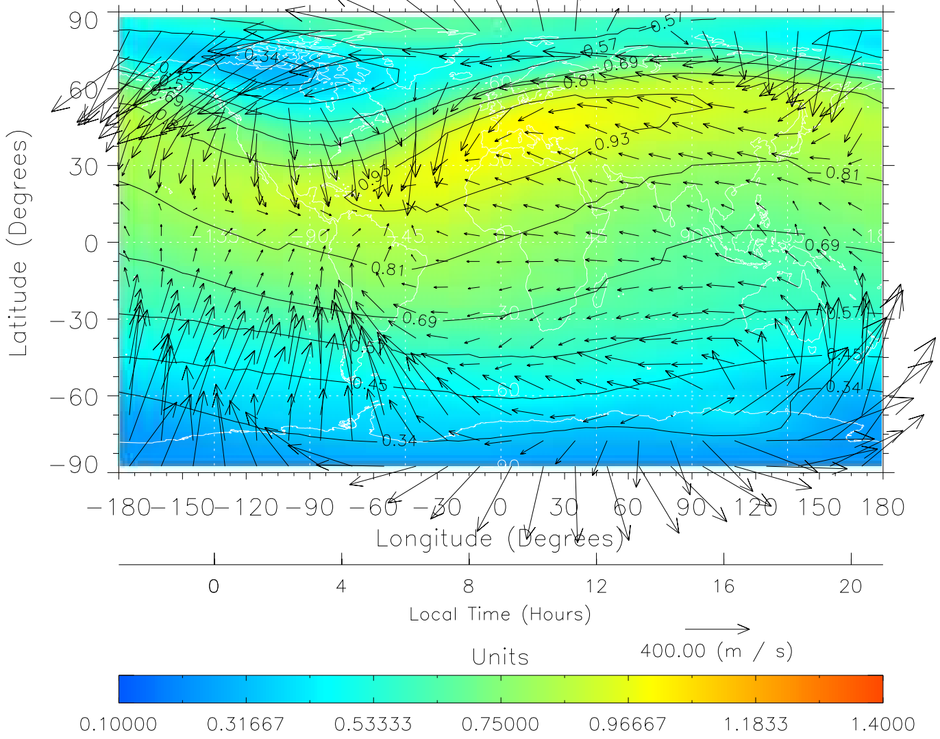
TIME-GCM MAP \Sigma O/N_2 with Neutral Wind vectors ZP = 2.00 UT = 9.00 DOY = 302
