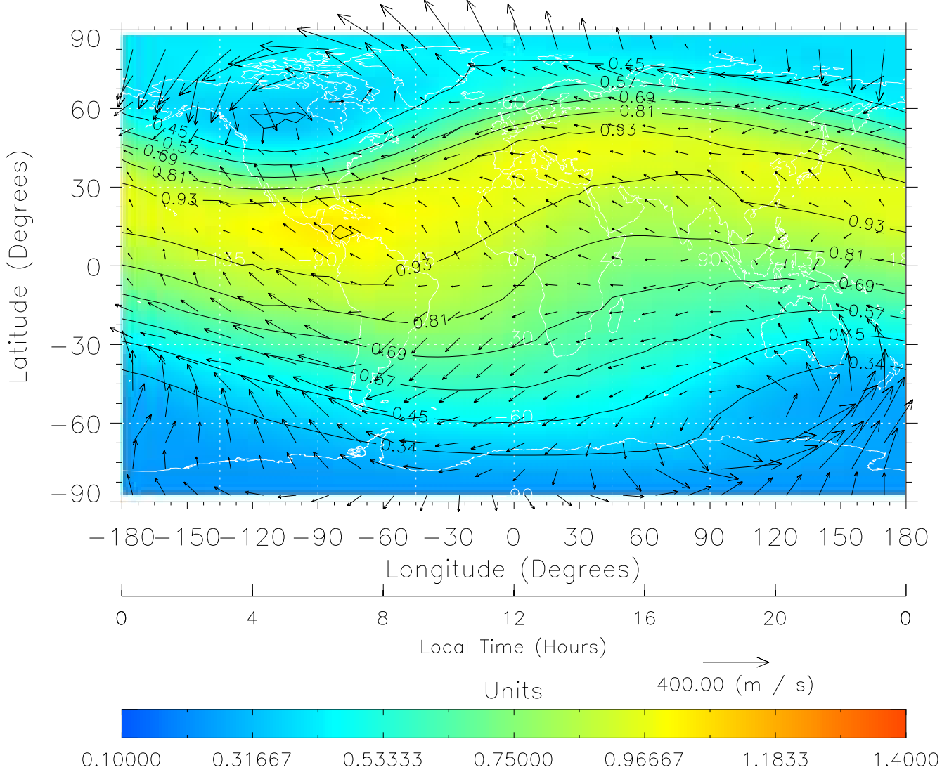
TIME-GCM MAP \Sigma O/N_2 with Neutral Wind vectors ZP = 2.00 UT = 12.00 DOY = 302
