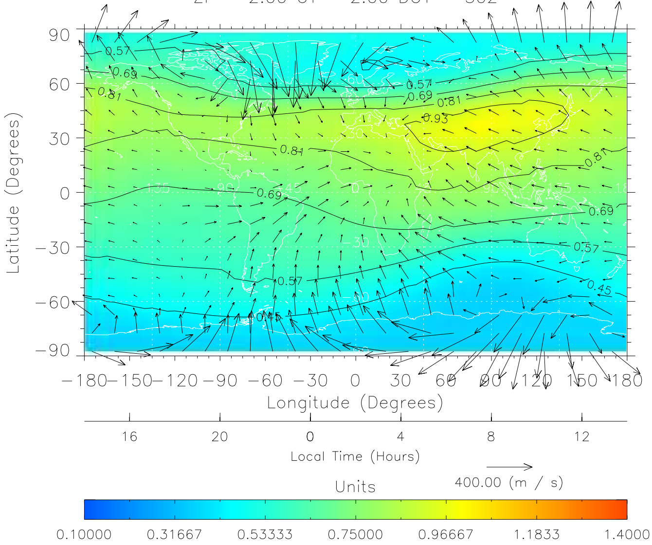
TIME-GCM MAP \Sigma O/N_2 with Neutral Wind vectors ZP = 2.00 UT = 2.00 DOY = 302
