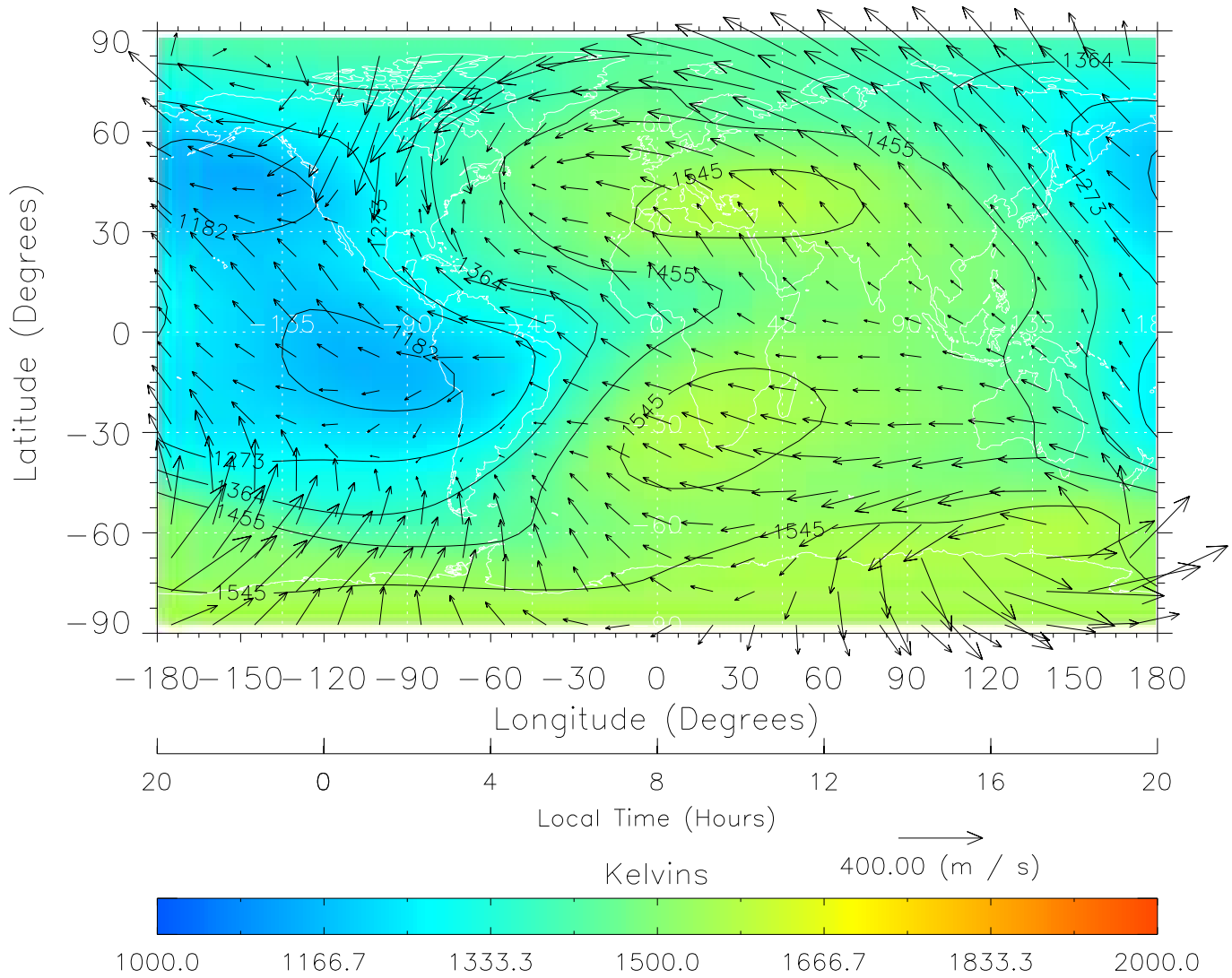
TIME-GCM MAP Temperature with Neutral Wind vectors ZP = 2.00 UT = 8.00 DOY = 325
