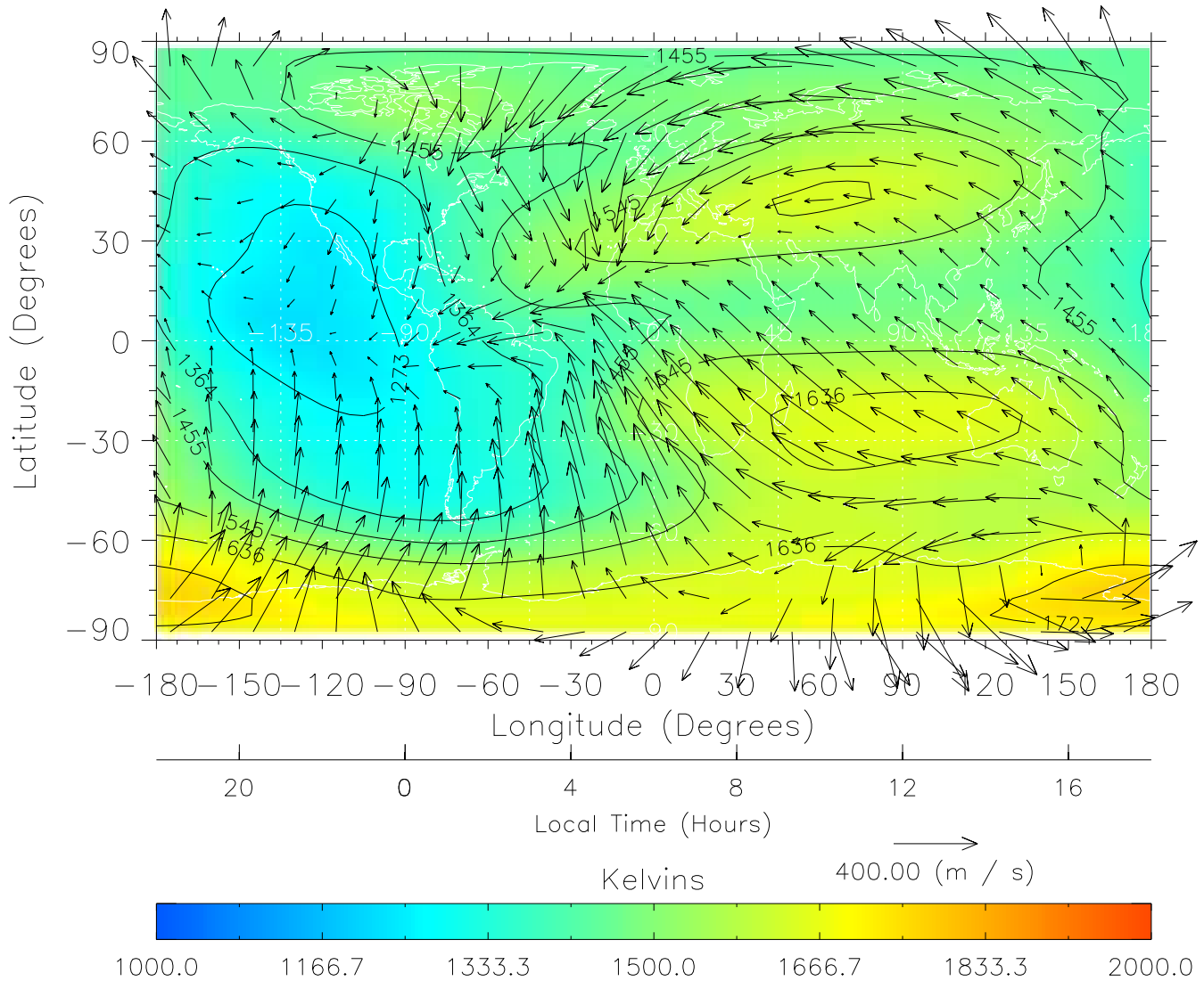
TIME-GCM MAP Temperature with Neutral Wind vectors ZP = 2.00 UT = 6.00 DOY = 325
