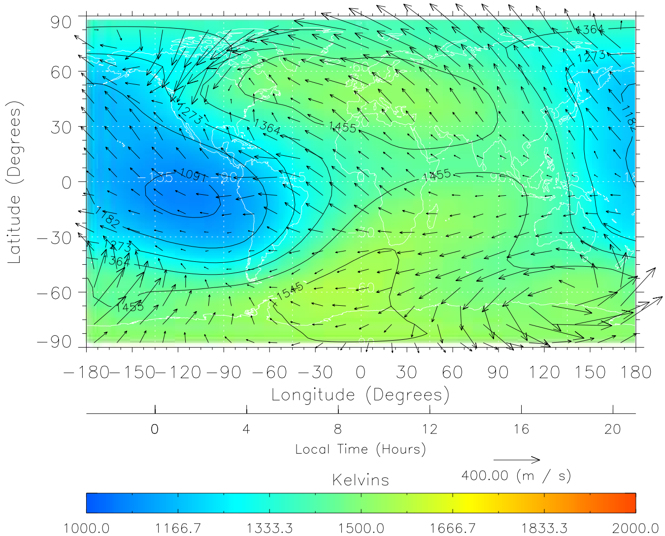
TIME-GCM MAP Temperature with Neutral Wind vectors ZP = 2.00 UT = 9.00 DOY = 325
