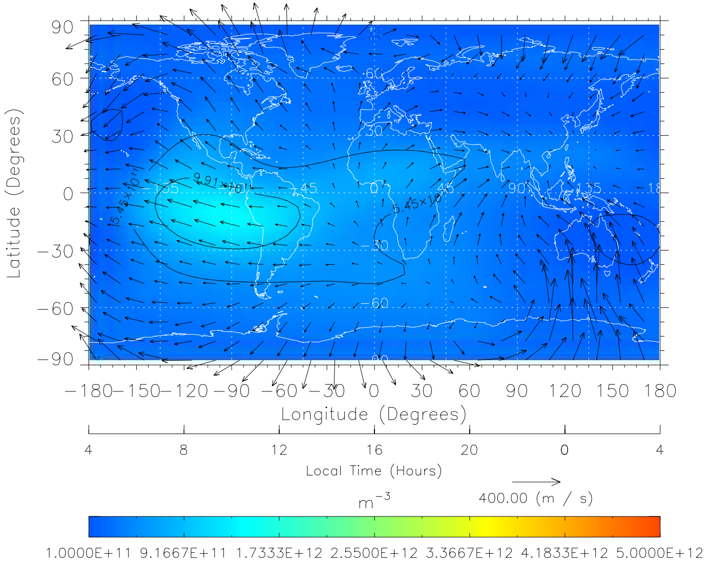
TIME-GCM MAP NmF2 with Neutral Wind vectors ZP = 2.00 UT = 16.00 DOY = 325
