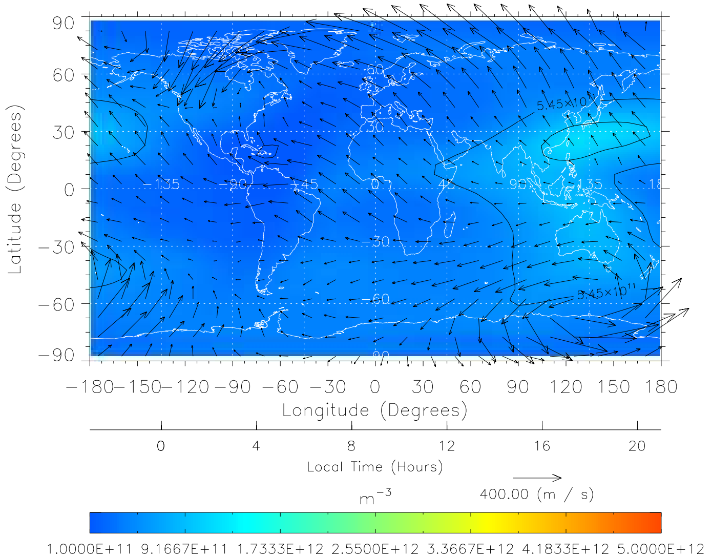
TIME-GCM MAP NmF2 with Neutral Wind vectors ZP = 2.00 UT = 9.00 DOY = 325
