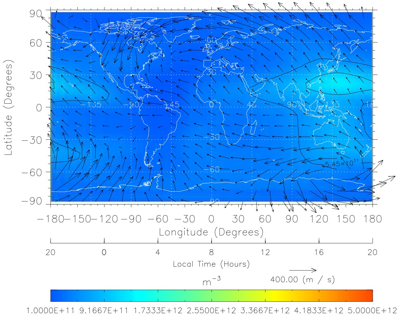
TIME-GCM MAP NmF2 with Neutral Wind vectors ZP = 2.00 UT = 8.00 DOY = 325
