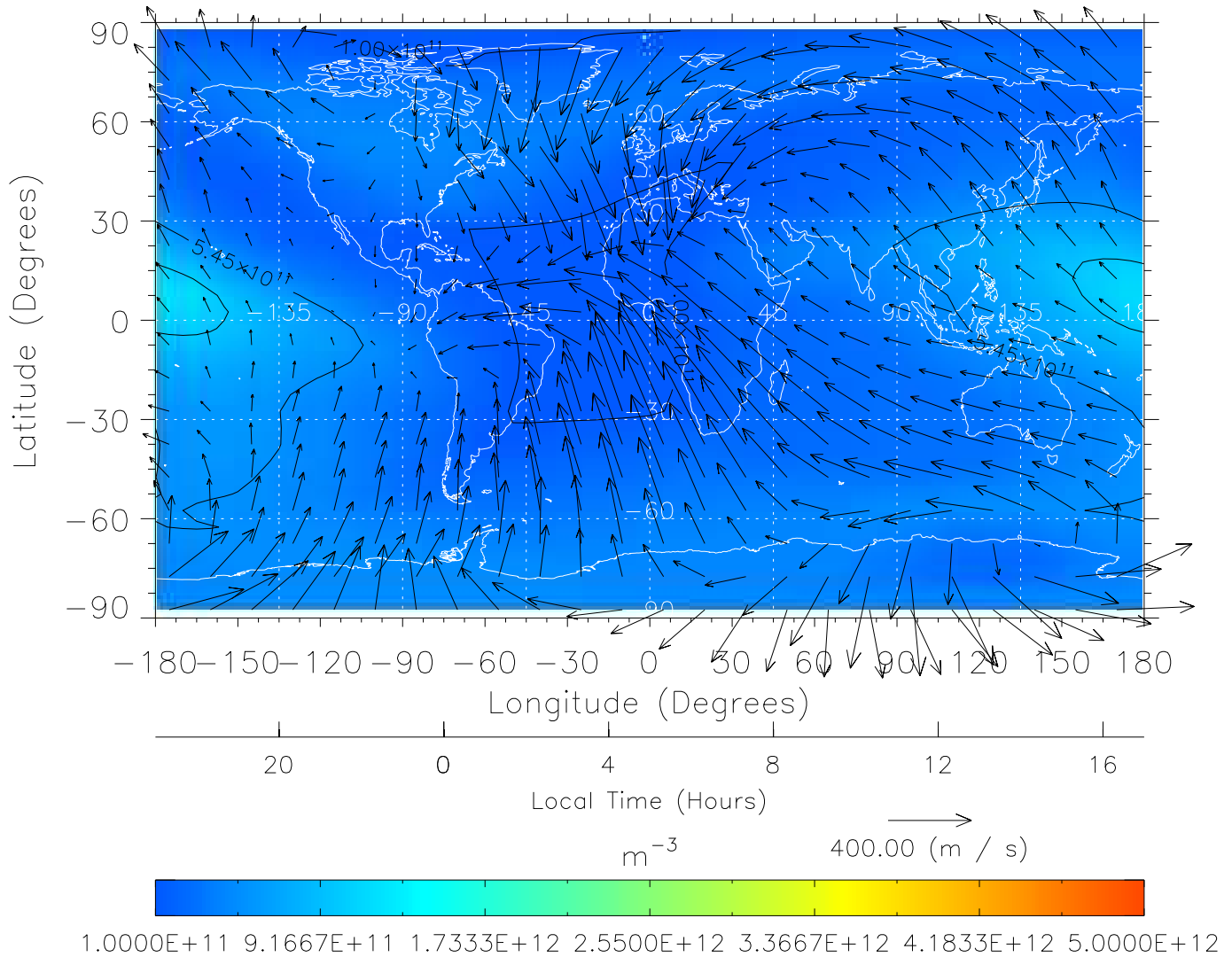
TIME-GCM MAP NmF2 with Neutral Wind vectors ZP = 2.00 UT = 5.00 DOY = 325
