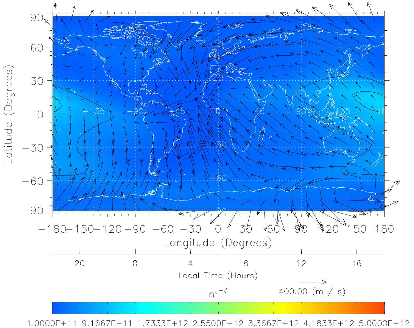
TIME-GCM MAP NmF2 with Neutral Wind vectors ZP = 2.00 UT = 6.00 DOY = 325
