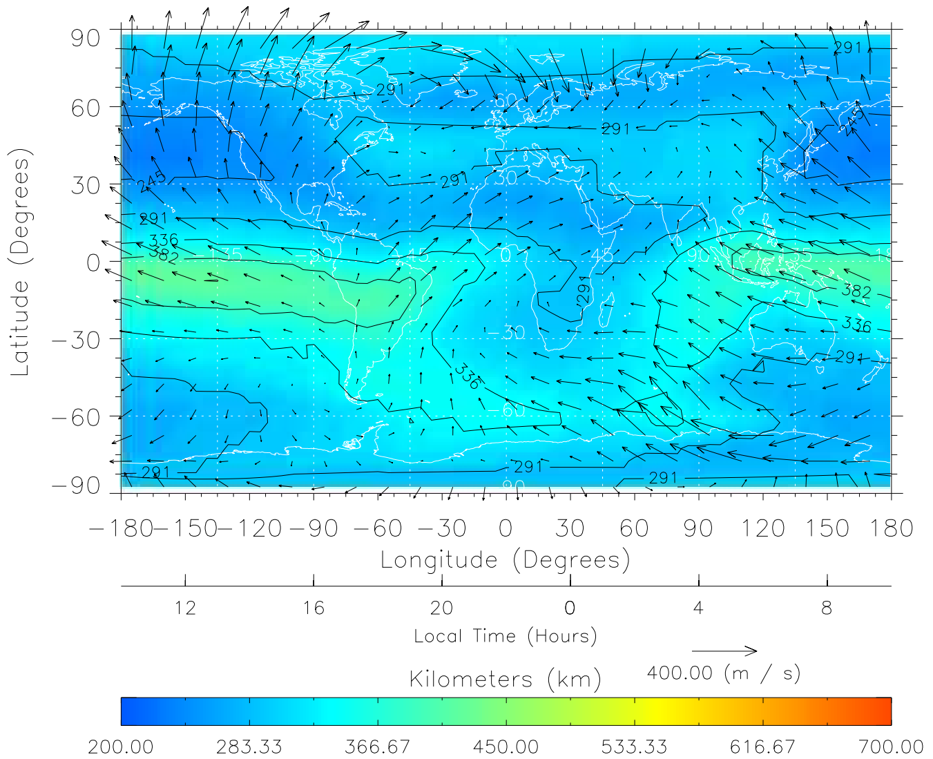
TIME-GCM MAP hmF2 with Neutral Wind vectors ZP = 2.00 UT = 22.00 DOY = 325
