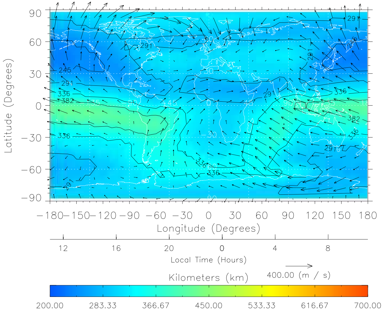
TIME-GCM MAP hmF2 with Neutral Wind vectors ZP = 2.00 UT = 23.00 DOY = 325
