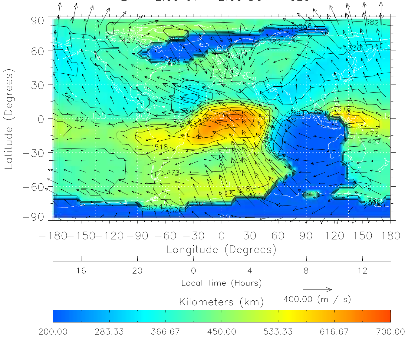
TIME-GCM MAP hmF2 with Neutral Wind vectors ZP = 2.00 UT = 2.00 DOY = 325
