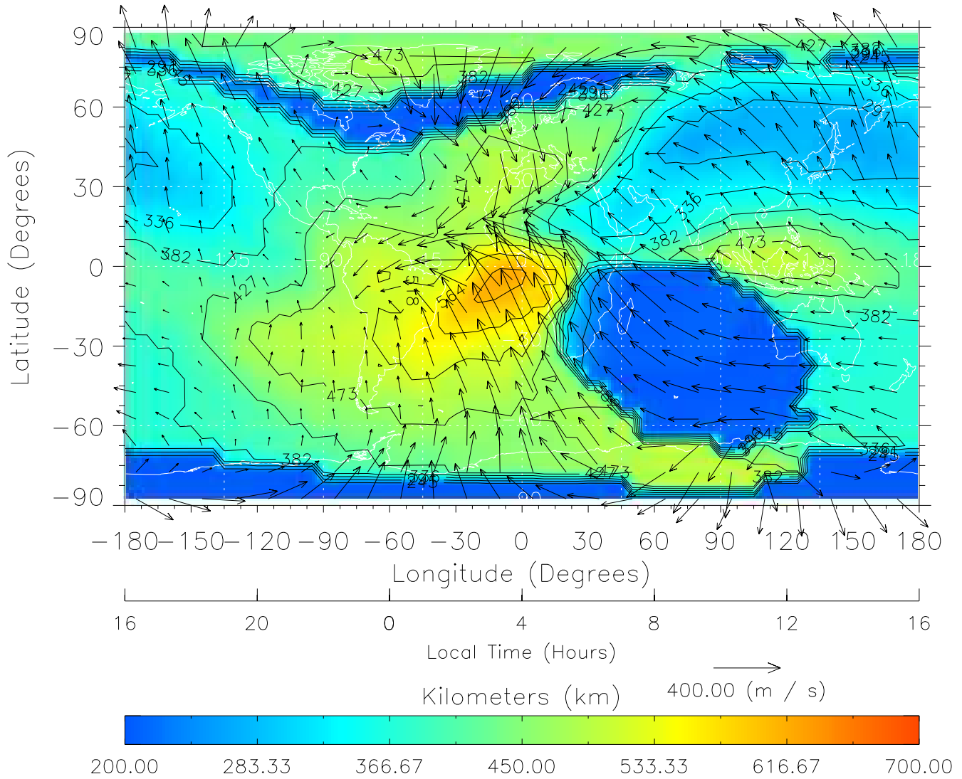
TIME-GCM MAP hmF2 with Neutral Wind vectors ZP = 2.00 UT = 4.00 DOY = 325
