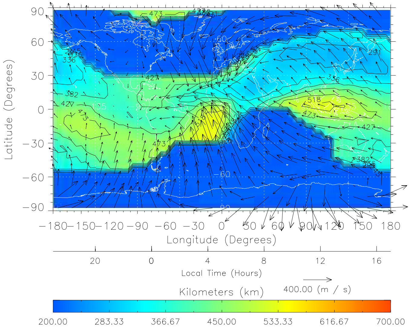
TIME-GCM MAP hmF2 with Neutral Wind vectors ZP = 2.00 UT = 5.00 DOY = 325
