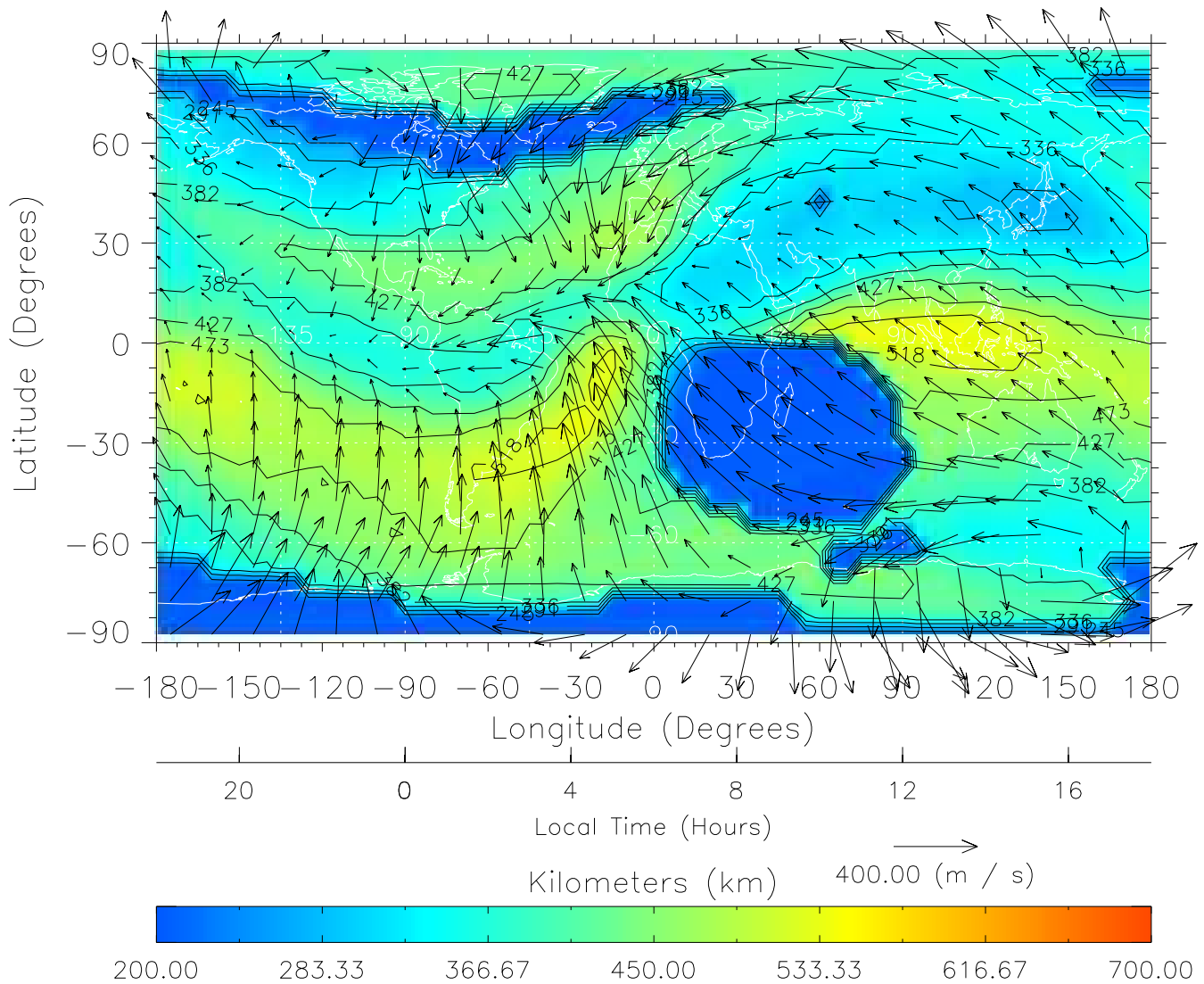
TIME-GCM MAP hmF2 with Neutral Wind vectors ZP = 2.00 UT = 6.00 DOY = 325
