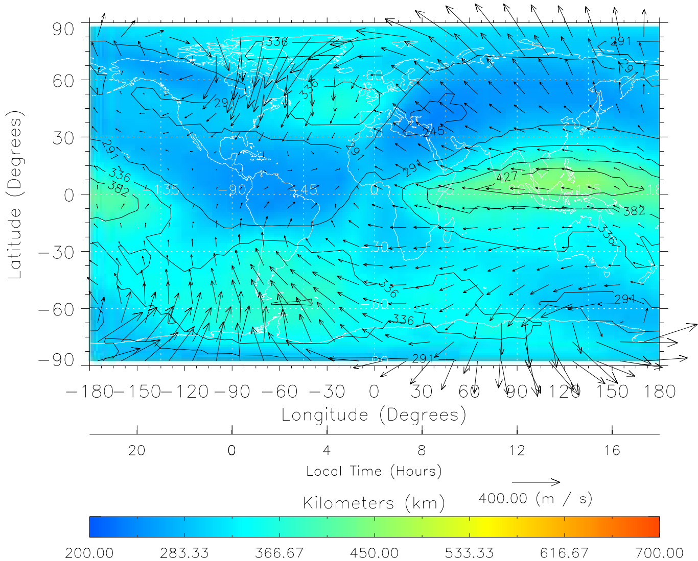
TIME-GCM MAP hmF2 with Neutral Wind vectors ZP = 2.00 UT = 6.00 DOY = 323
