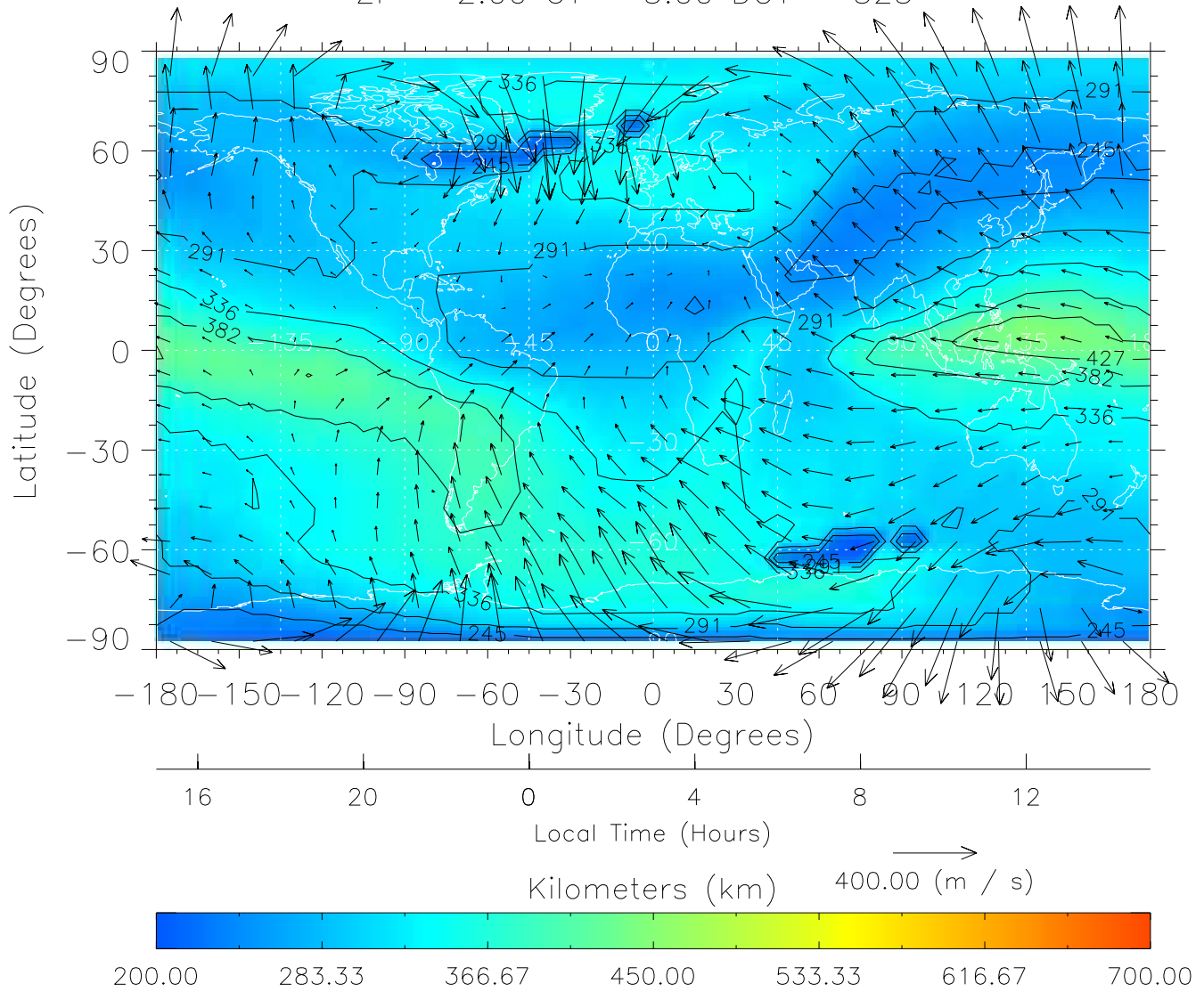
TIME-GCM MAP hmF2 with Neutral Wind vectors ZP = 2.00 UT = 3.00 DOY = 323
