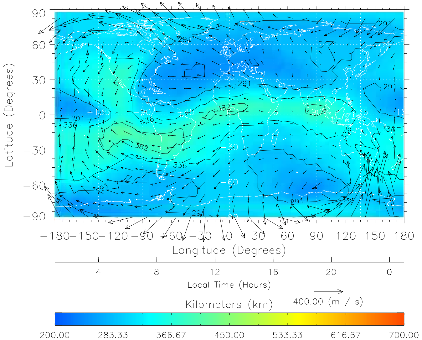
TIME-GCM MAP hmF2 with Neutral Wind vectors ZP = 2.00 UT = 13.00 DOY = 323
