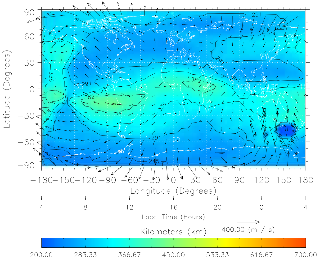
TIME-GCM MAP hmF2 with Neutral Wind vectors ZP = 2.00 UT = 16.00 DOY = 323
