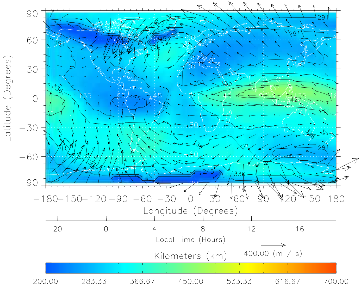
TIME-GCM MAP hmF2 with Neutral Wind vectors ZP = 2.00 UT = 7.00 DOY = 323
