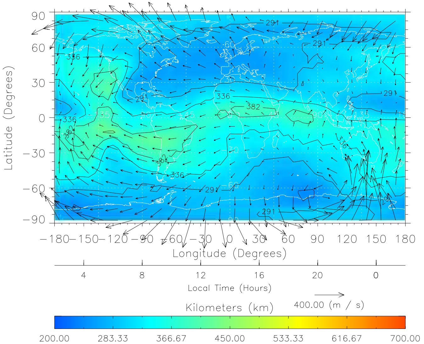
TIME-GCM MAP hmF2 with Neutral Wind vectors ZP = 2.00 UT = 14.00 DOY = 323
