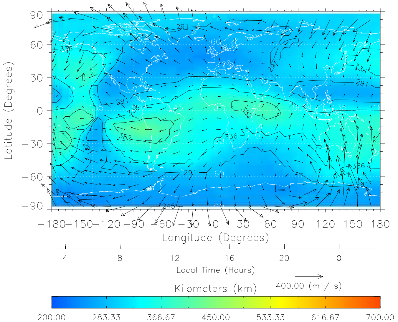
TIME-GCM MAP hmF2 with Neutral Wind vectors ZP = 2.00 UT = 15.00 DOY = 323
