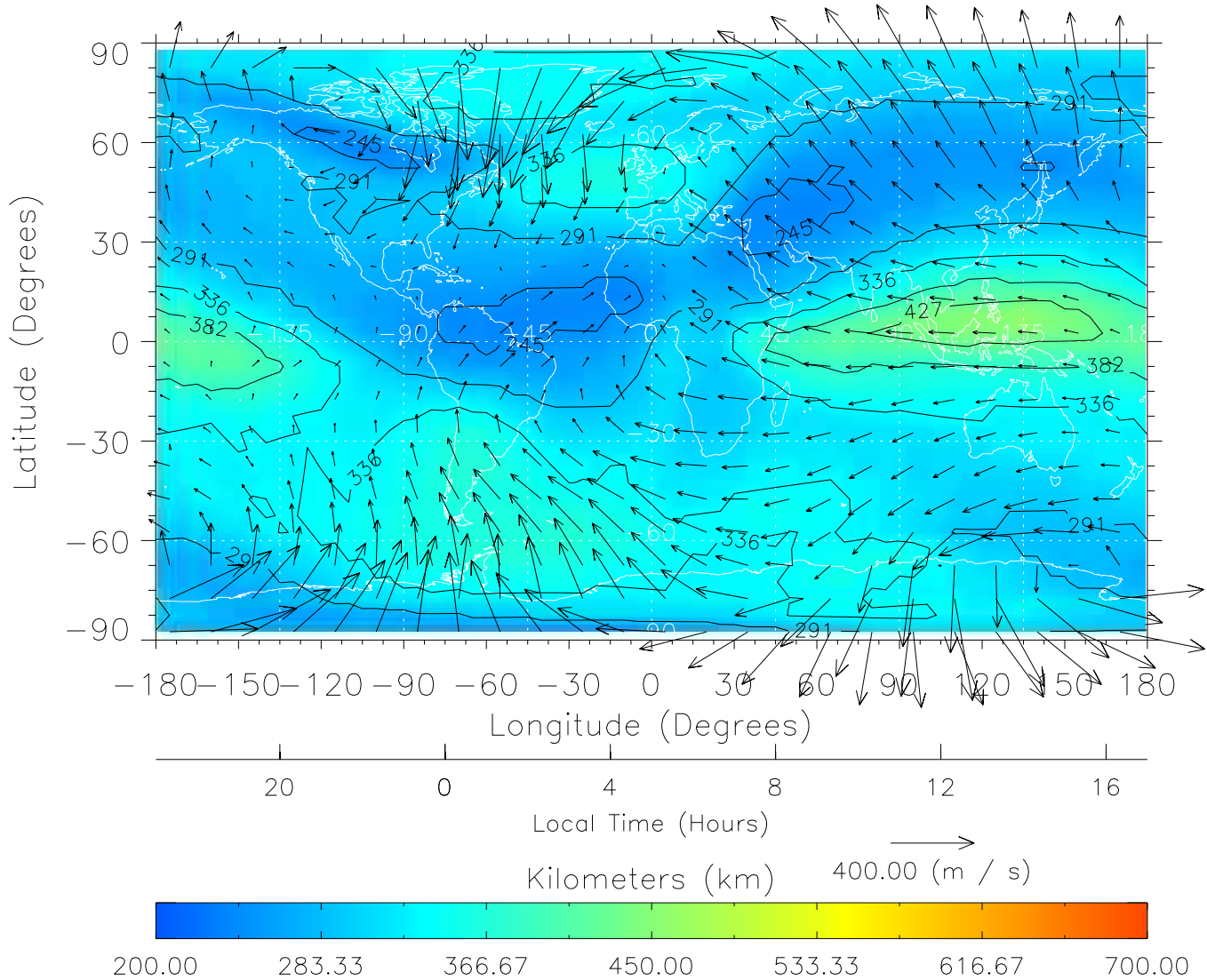
TIME-GCM MAP hmF2 with Neutral Wind vectors ZP = 2.00 UT = 5.00 DOY = 323
