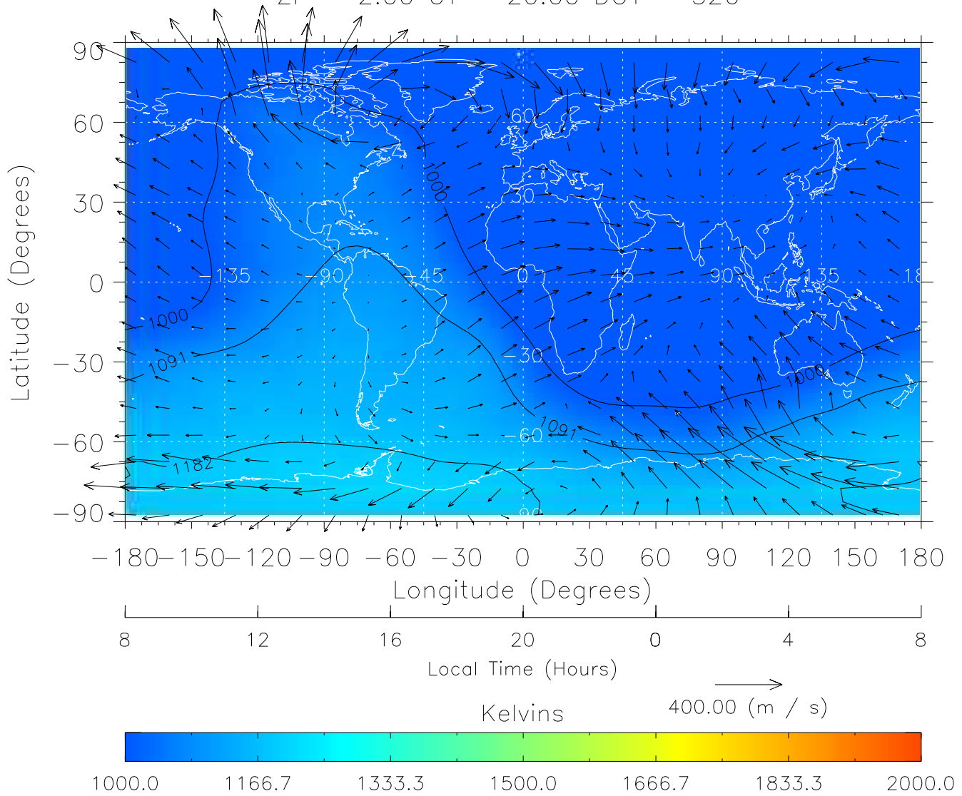
TIME-GCM MAP Temperature with Neutral Wind vectors ZP = 2.00 UT = 20.00 DOY = 326
