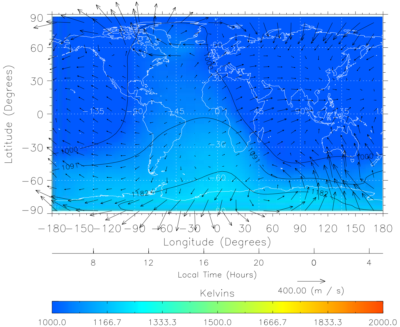
TIME-GCM MAP Temperature with Neutral Wind vectors ZP = 2.00 UT = 17.00 DOY = 326
