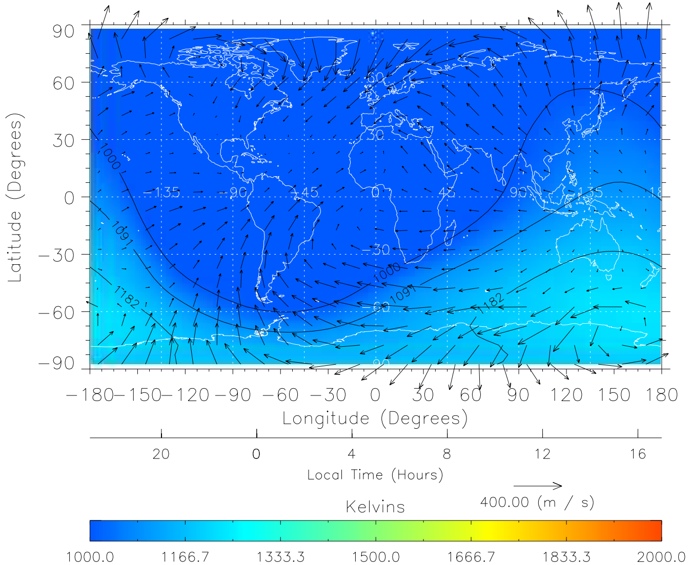
TIME-GCM MAP Temperature with Neutral Wind vectors ZP = 2.00 UT = 5.00 DOY = 326
