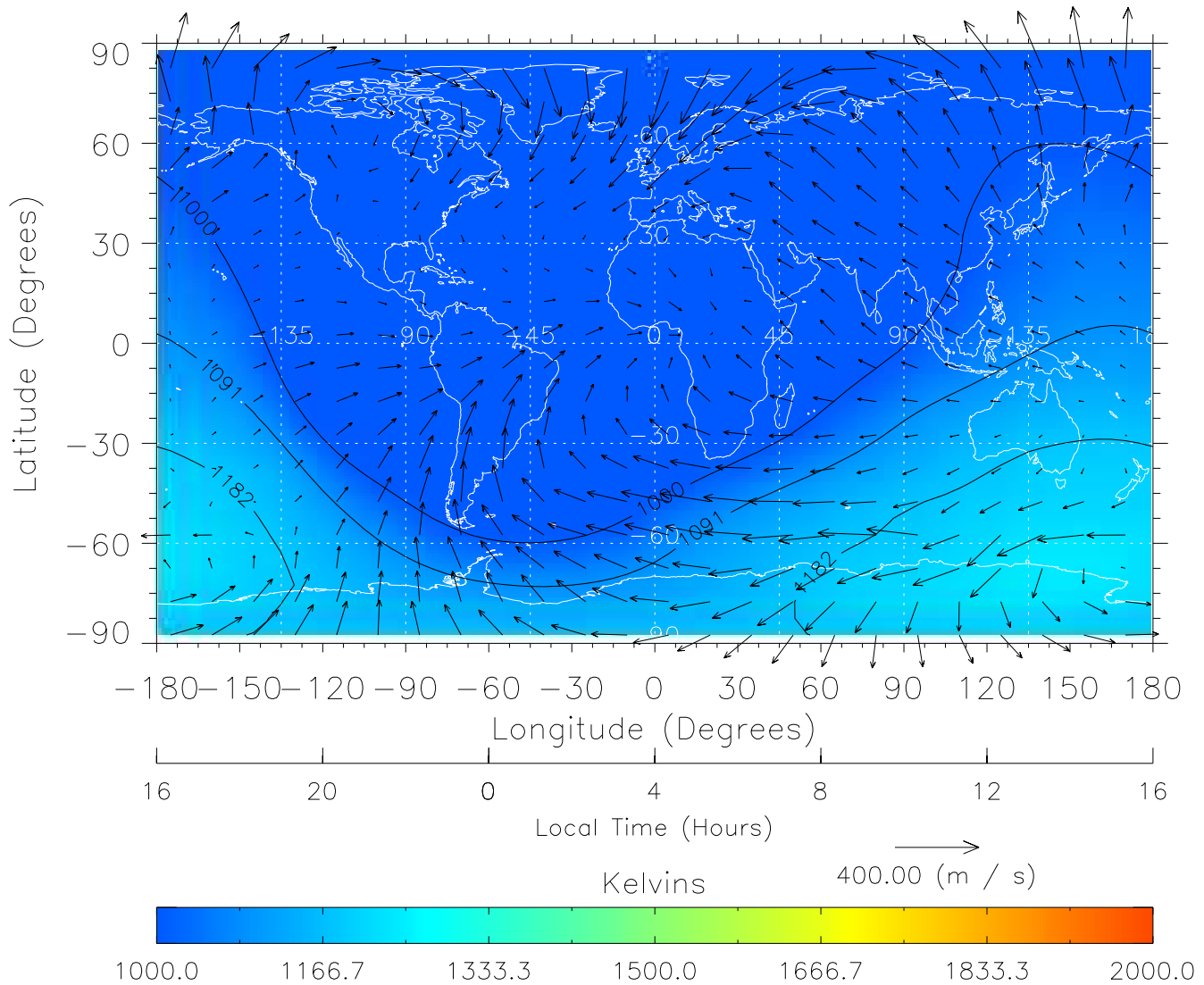
TIME-GCM MAP Temperature with Neutral Wind vectors ZP = 2.00 UT = 4.00 DOY = 326
