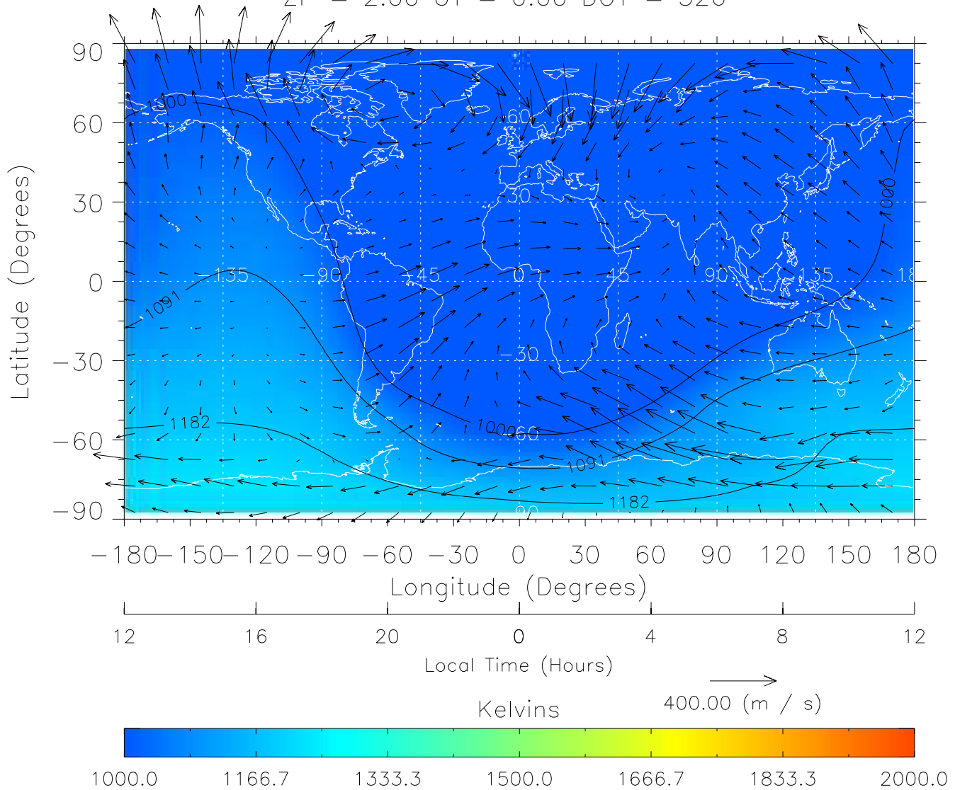
TIME-GCM MAP Temperature with Neutral Wind vectors ZP = 2.00 UT = 0.00 DOY = 326
