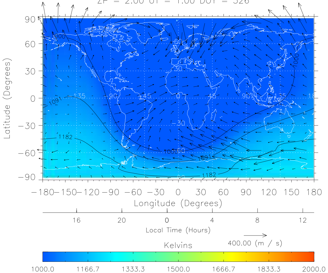
TIME-GCM MAP Temperature with Neutral Wind vectors ZP = 2.00 UT = 1.00 DOY = 326
