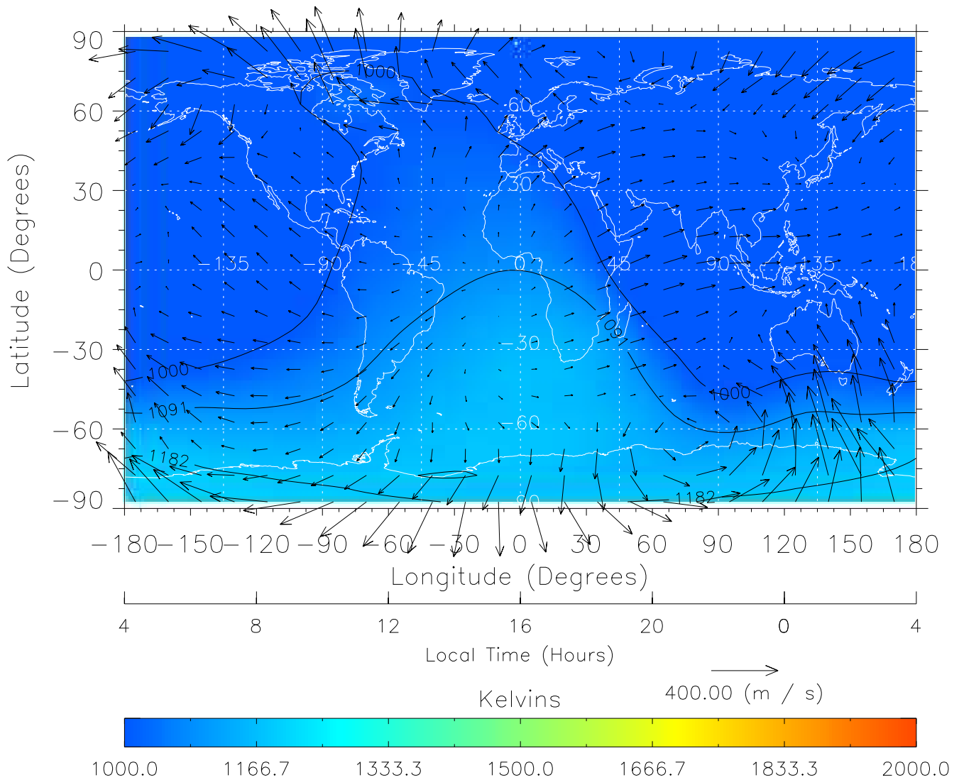
TIME-GCM MAP Temperature with Neutral Wind vectors ZP = 2.00 UT = 16.00 DOY = 326
