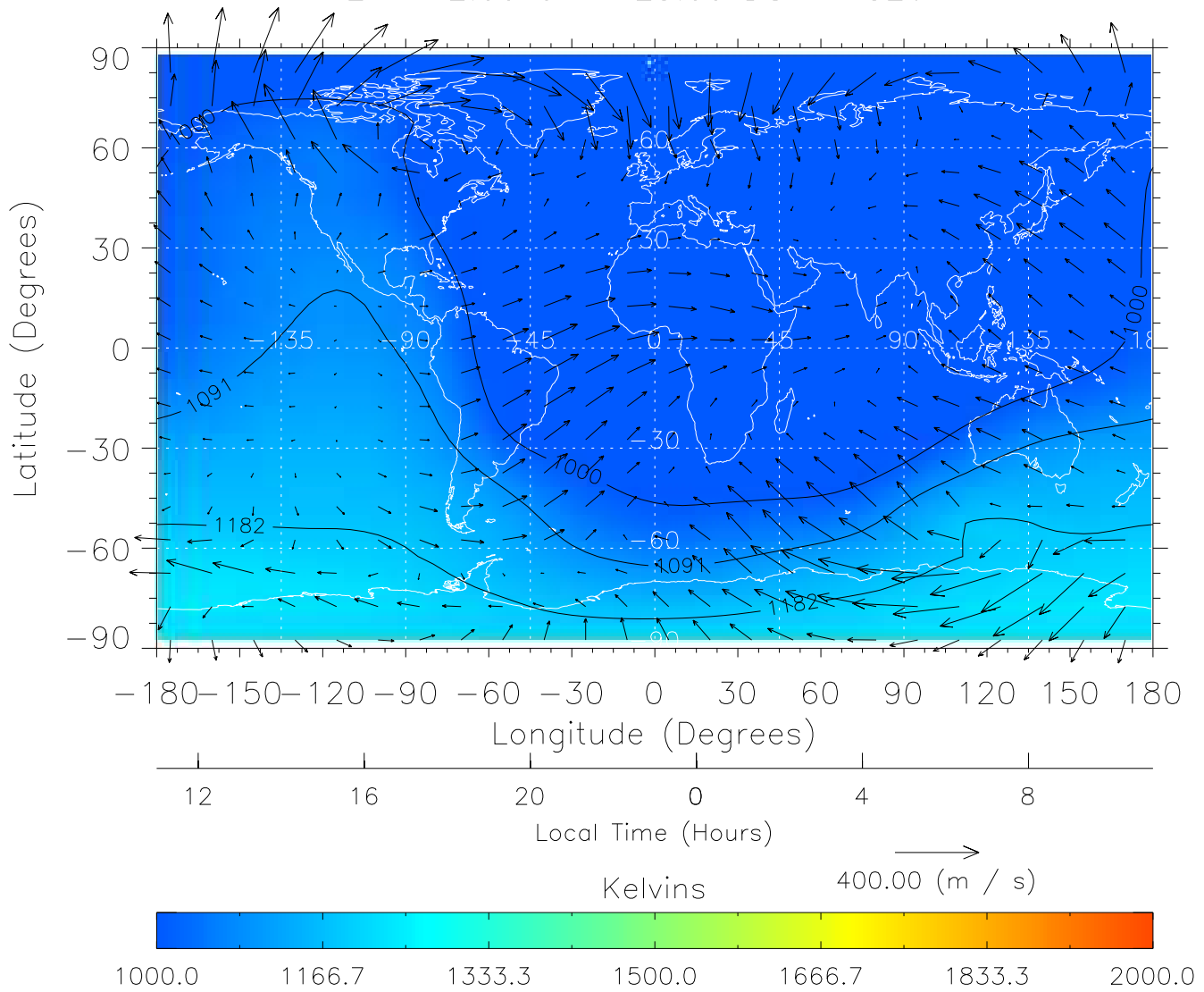
TIME-GCM MAP Temperature with Neutral Wind vectors ZP = 2.00 UT = 23.00 DOY = 326
