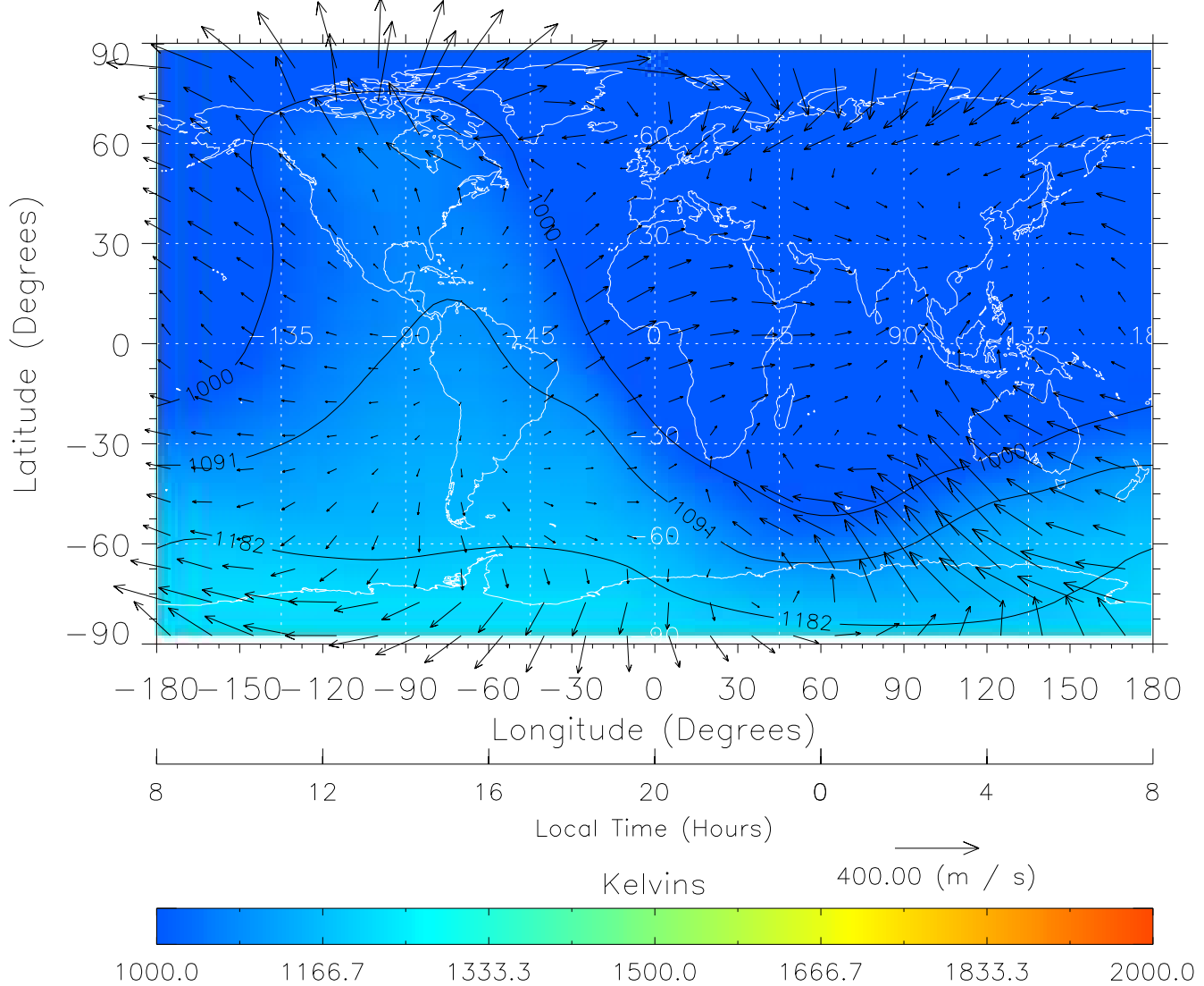
TIME-GCM MAP Temperature with Neutral Wind vectors ZP = 2.00 UT = 20.00 DOY = 325
