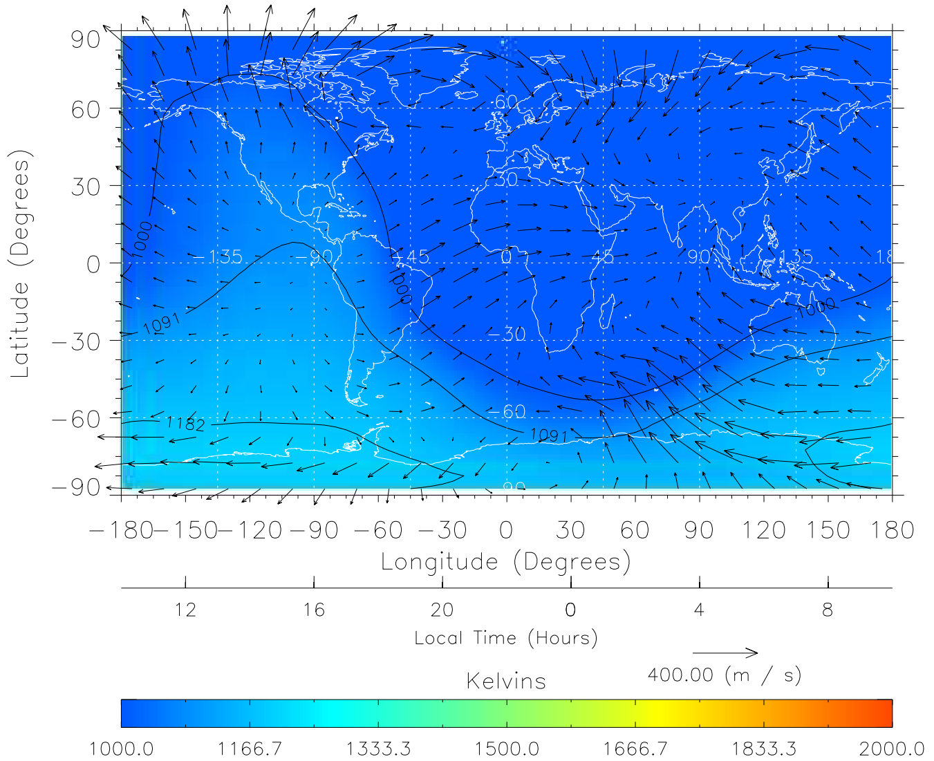
TIME-GCM MAP Temperature with Neutral Wind vectors ZP = 2.00 UT = 22.00 DOY = 325
