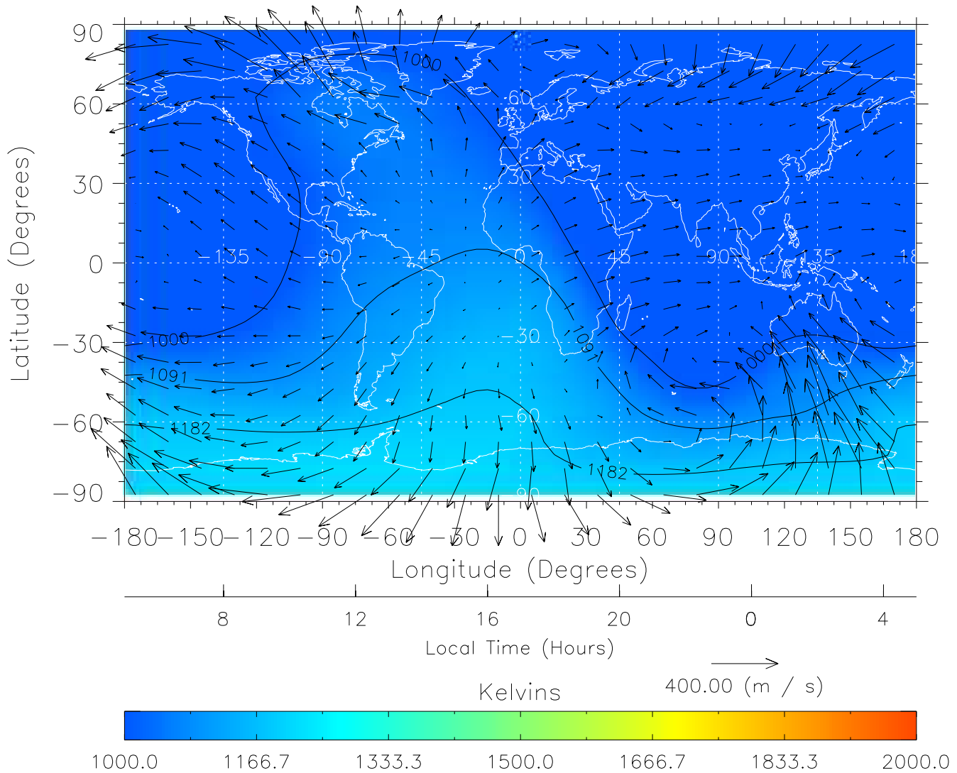
TIME-GCM MAP Temperature with Neutral Wind vectors ZP = 2.00 UT = 17.00 DOY = 325
