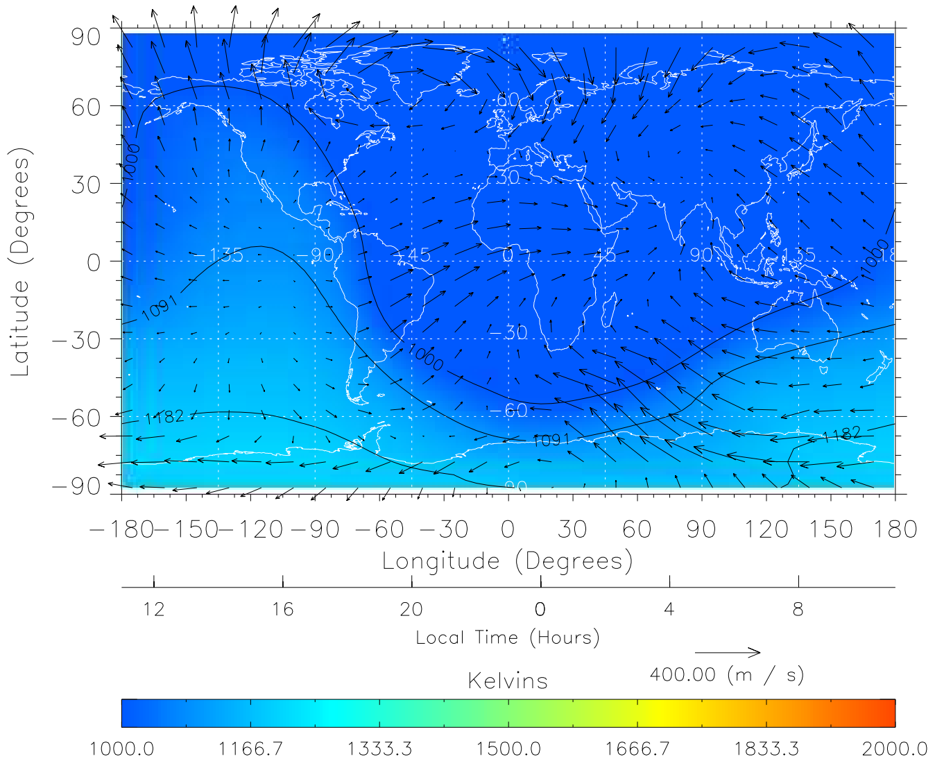
TIME-GCM MAP Temperature with Neutral Wind vectors ZP = 2.00 UT = 23.00 DOY = 325
