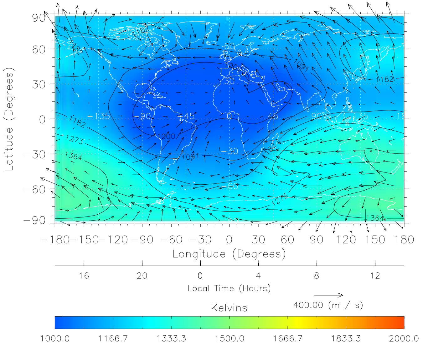
TIME-GCM MAP Temperature with Neutral Wind vectors ZP = 2.00 UT = 2.00 DOY = 325
