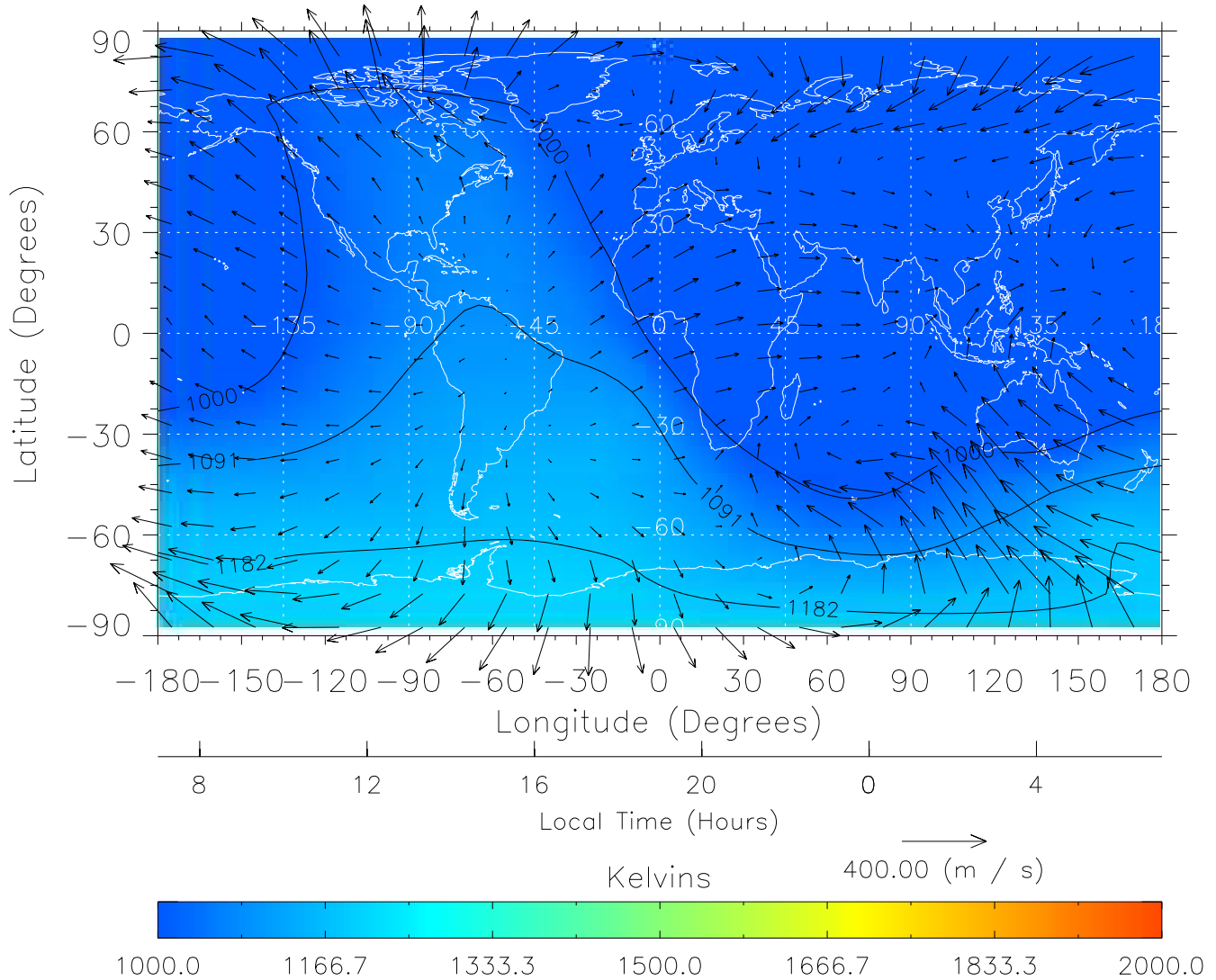
TIME-GCM MAP Temperature with Neutral Wind vectors ZP = 2.00 UT = 19.00 DOY = 325
