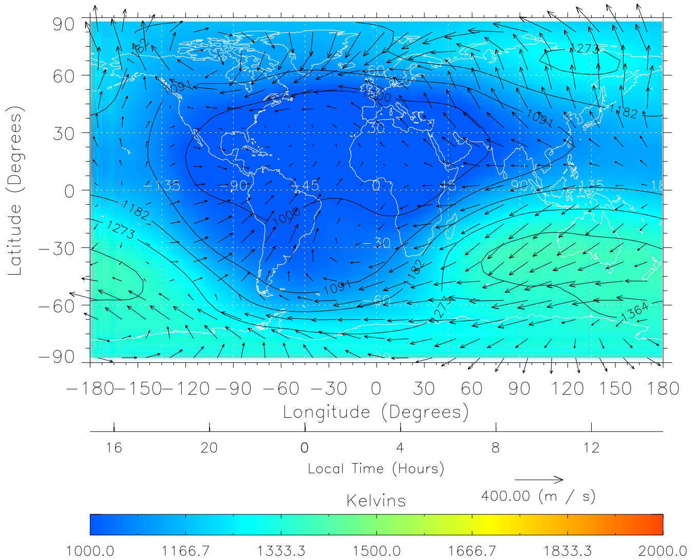
TIME-GCM MAP Temperature with Neutral Wind vectors ZP = 2.00 UT = 3.00 DOY = 325
