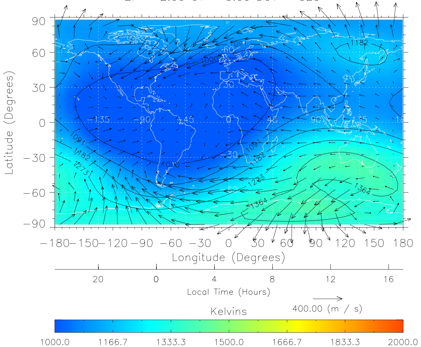
TIME-GCM MAP Temperature with Neutral Wind vectors ZP = 2.00 UT = 5.00 DOY = 325
