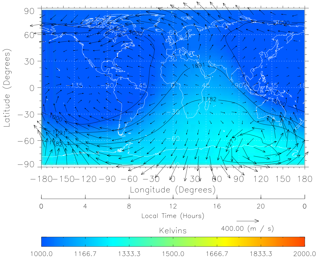
TIME-GCM MAP Temperature with Neutral Wind vectors ZP = 2.00 UT = 12.00 DOY = 325
