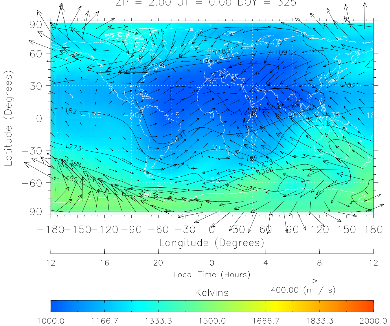
TIME-GCM MAP Temperature with Neutral Wind vectors ZP = 2.00 UT = 0.00 DOY = 325
