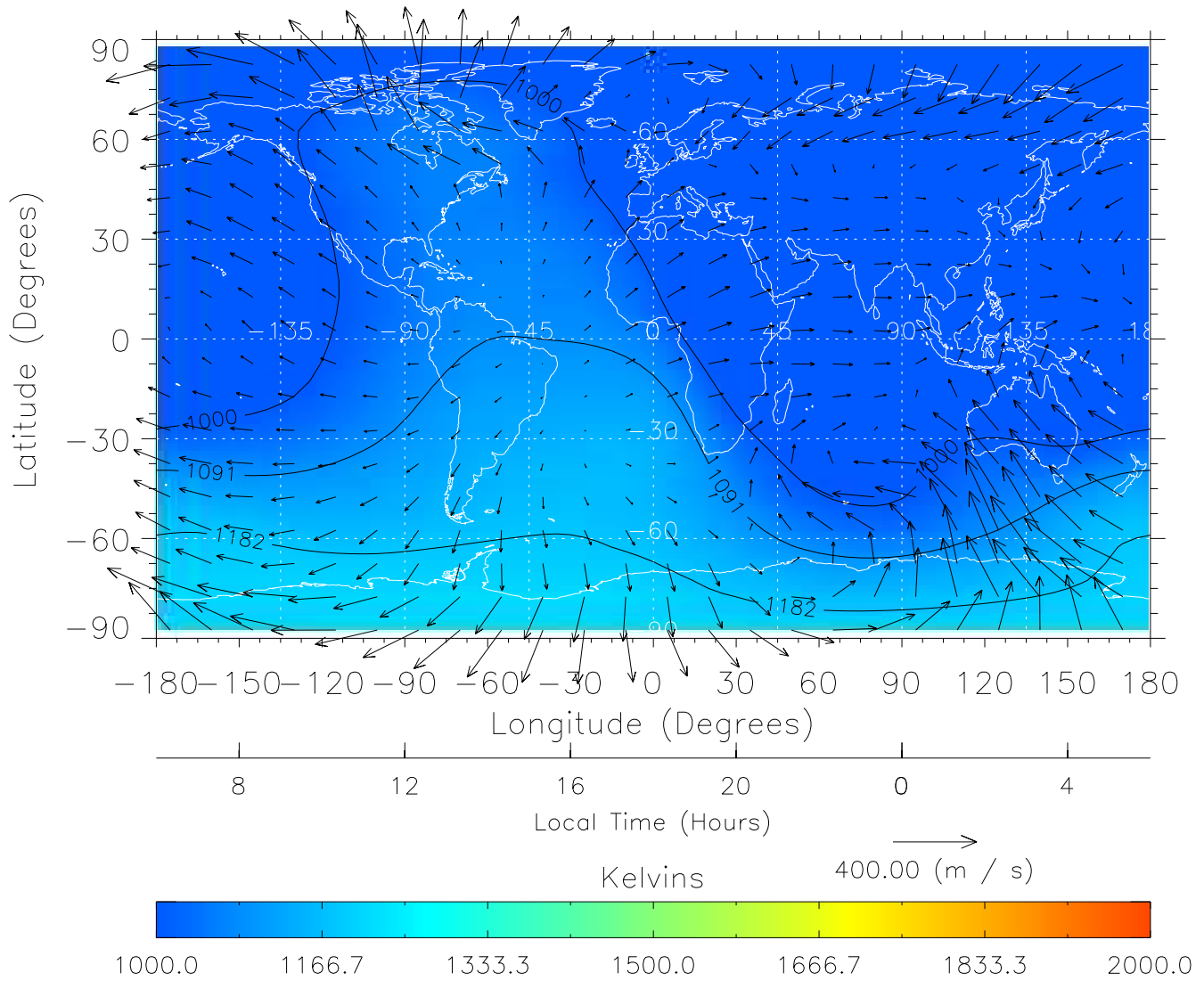
TIME-GCM MAP Temperature with Neutral Wind vectors ZP = 2.00 UT = 18.00 DOY = 325
