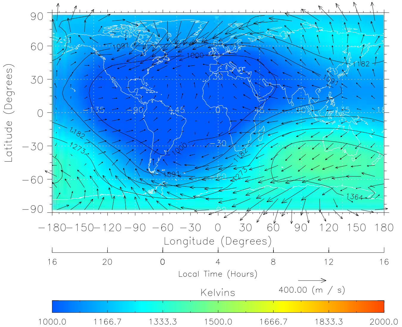
TIME-GCM MAP Temperature with Neutral Wind vectors ZP = 2.00 UT = 4.00 DOY = 325
