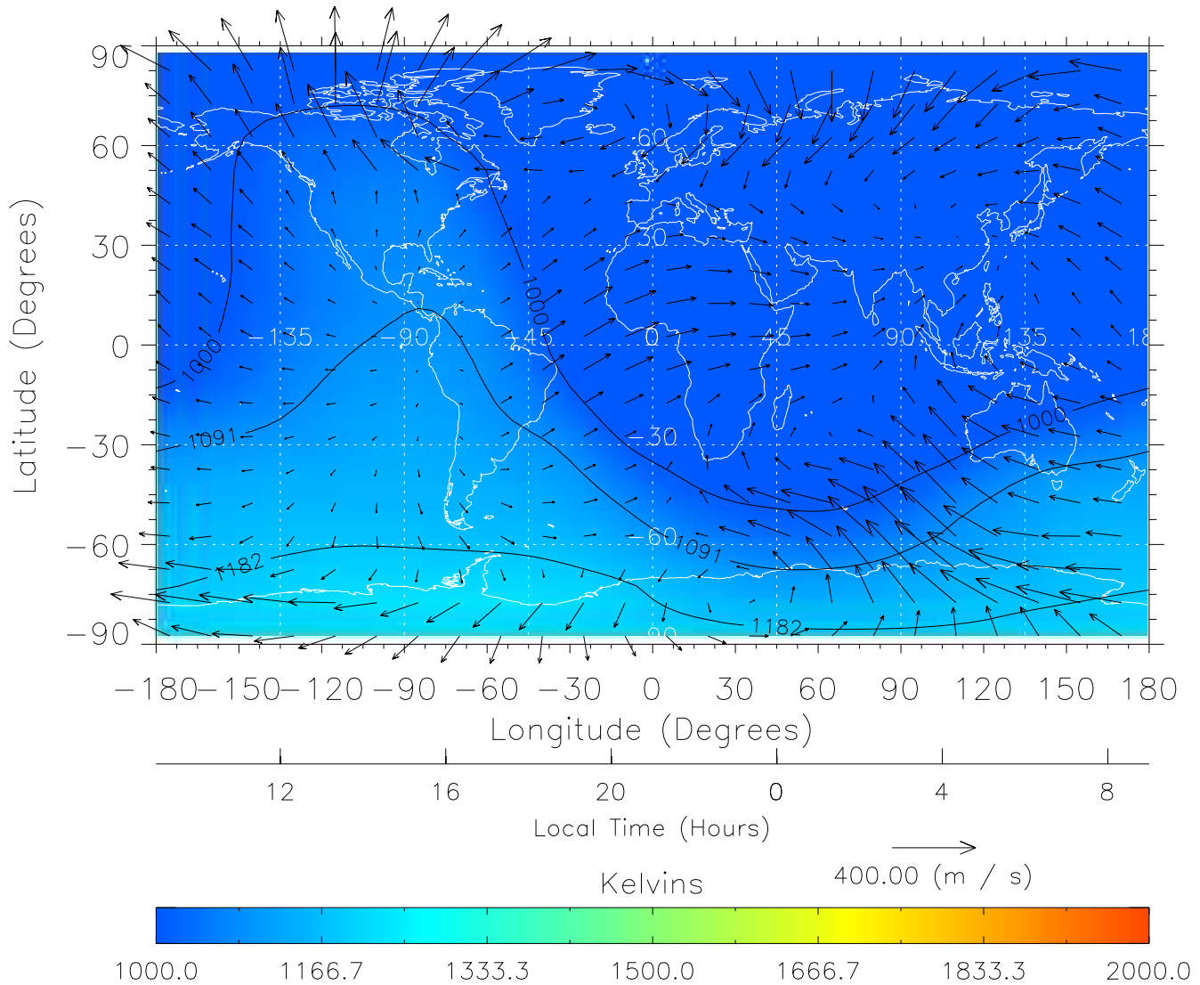
TIME-GCM MAP Temperature with Neutral Wind vectors ZP = 2.00 UT = 21.00 DOY = 325
