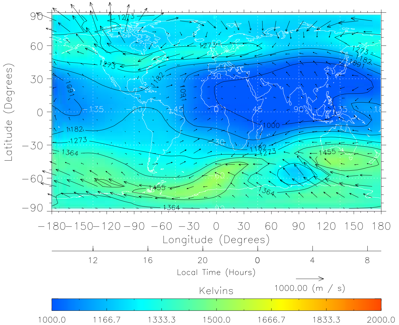
TIME-GCM MAP Temperature with Neutral Wind vectors ZP = 2.00 UT = 21.00 DOY = 324
