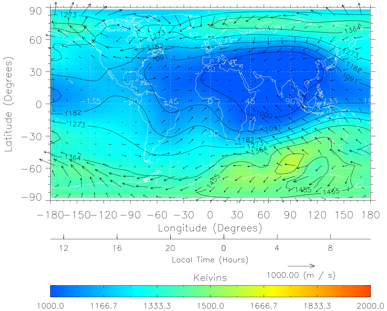
TIME-GCM MAP Temperature with Neutral Wind vectors ZP = 2.00 UT = 23.00 DOY = 324
