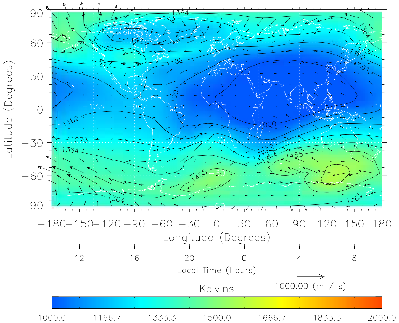
TIME-GCM MAP Temperature with Neutral Wind vectors ZP = 2.00 UT = 22.00 DOY = 324
