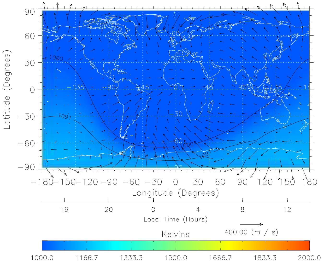
TIME-GCM MAP Temperature with Neutral Wind vectors ZP = 2.00 UT = 2.00 DOY = 323
