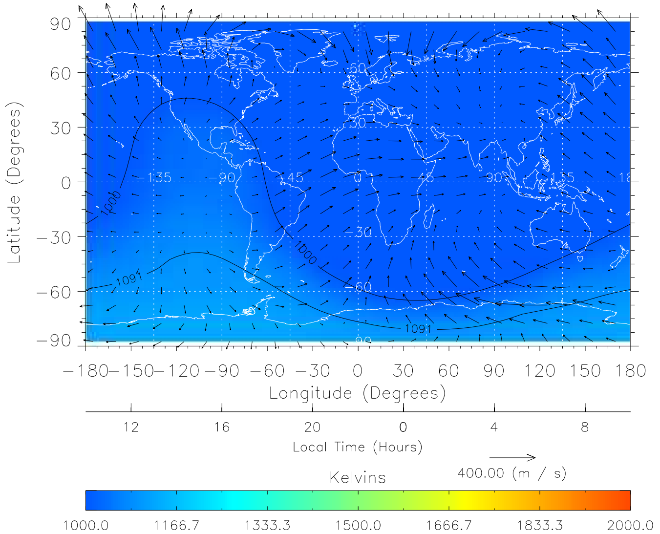
TIME-GCM MAP Temperature with Neutral Wind vectors ZP = 2.00 UT = 22.00 DOY = 323
