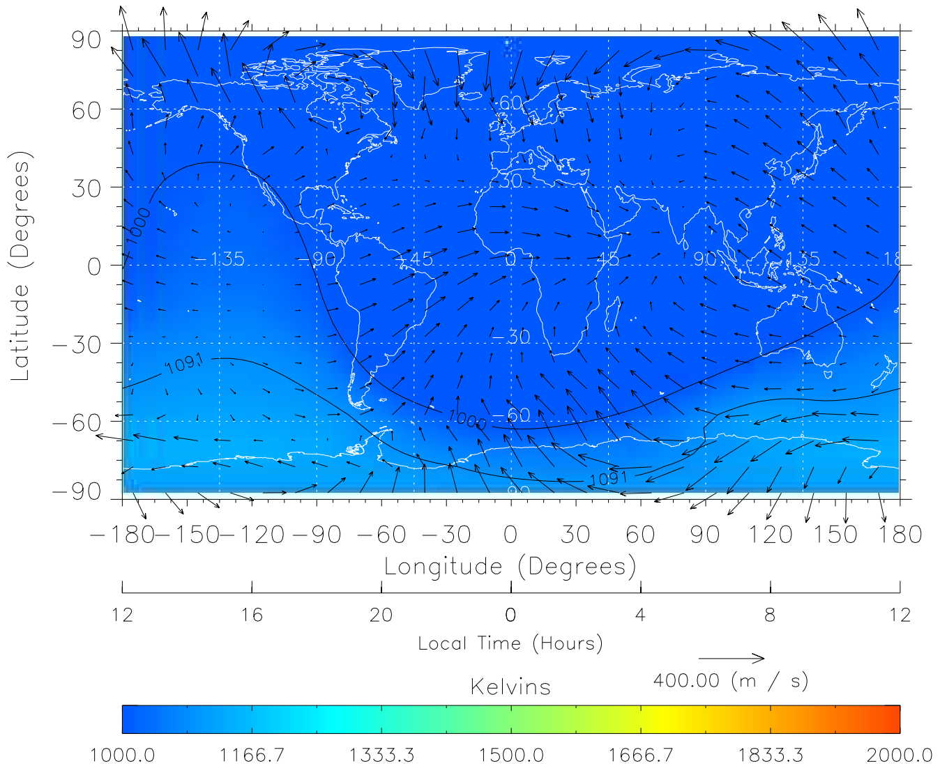
TIME-GCM MAP Temperature with Neutral Wind vectors ZP = 2.00 UT = 0.00 DOY = 323
