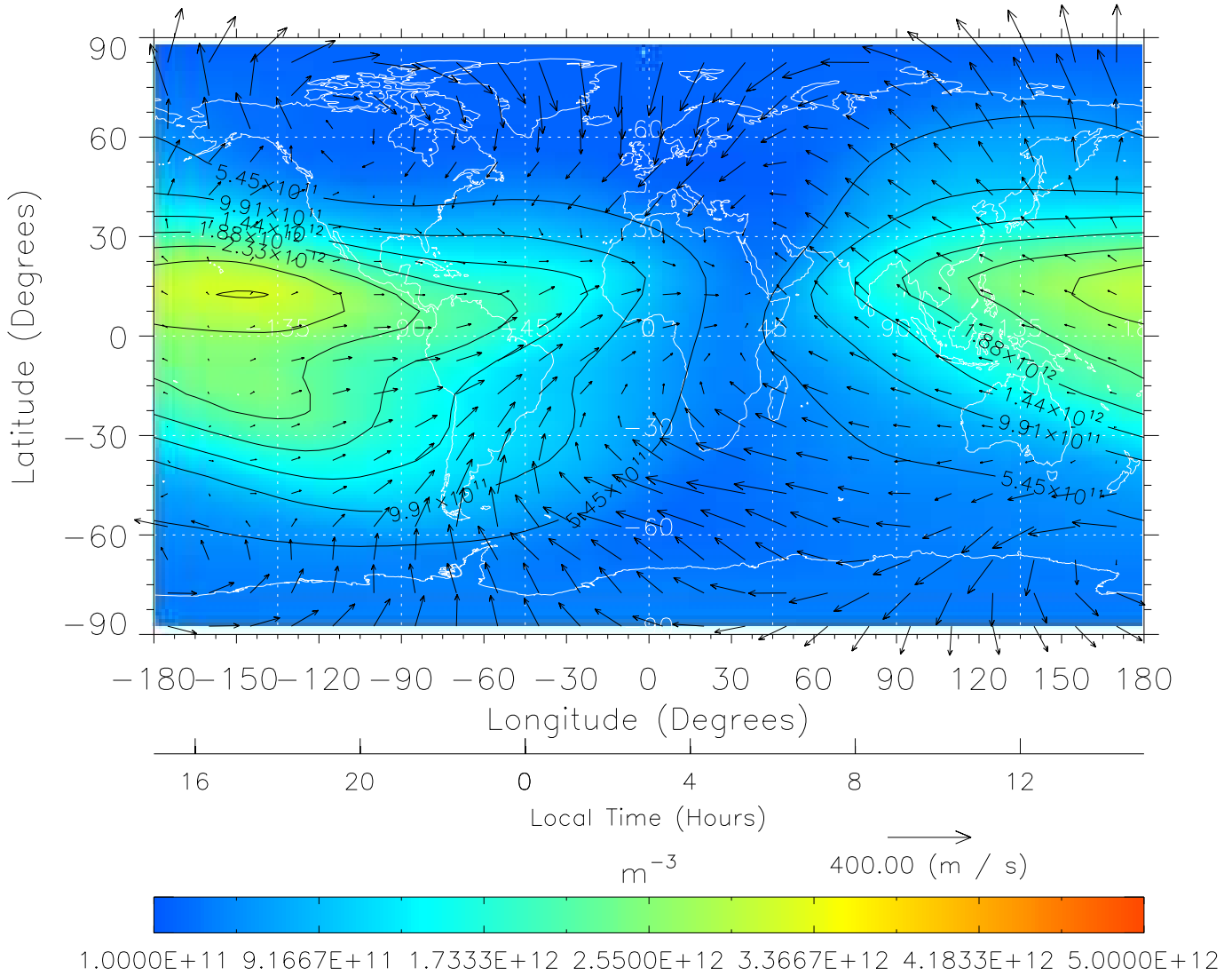
TIME-GCM MAP NmF2 with Neutral Wind vectors ZP = 2.00 UT = 3.00 DOY = 326
