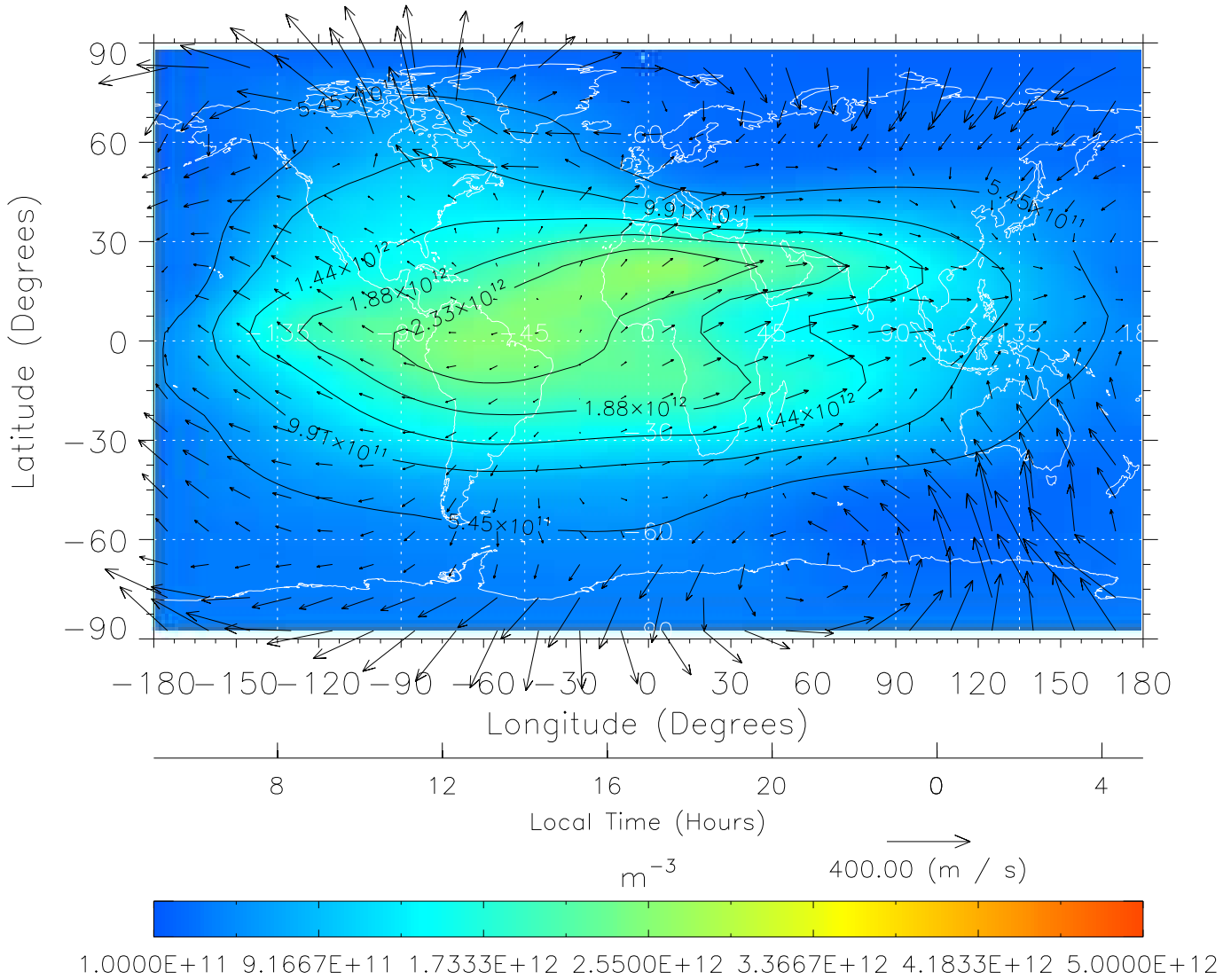
TIME-GCM MAP NmF2 with Neutral Wind vectors ZP = 2.00 UT = 17.00 DOY = 326
