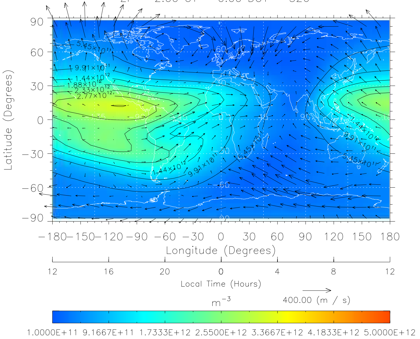
TIME-GCM MAP NmF2 with Neutral Wind vectors ZP = 2.00 UT = 0.00 DOY = 326
