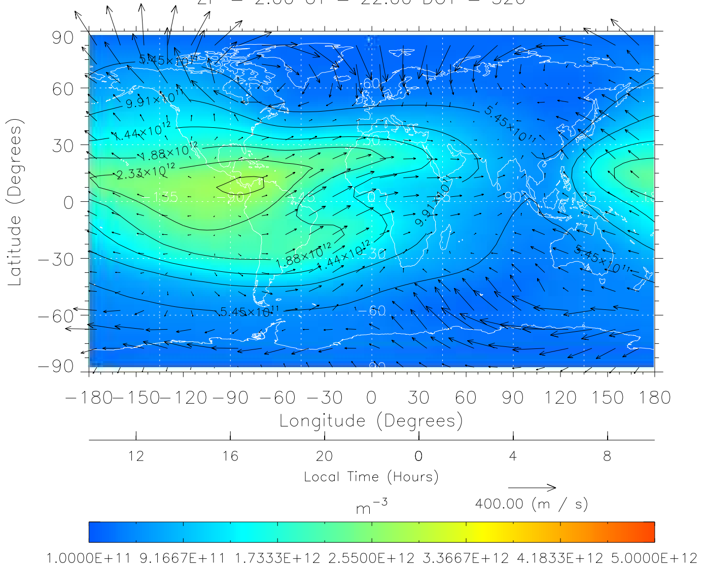
TIME-GCM MAP NmF2 with Neutral Wind vectors ZP = 2.00 UT = 22.00 DOY = 326
