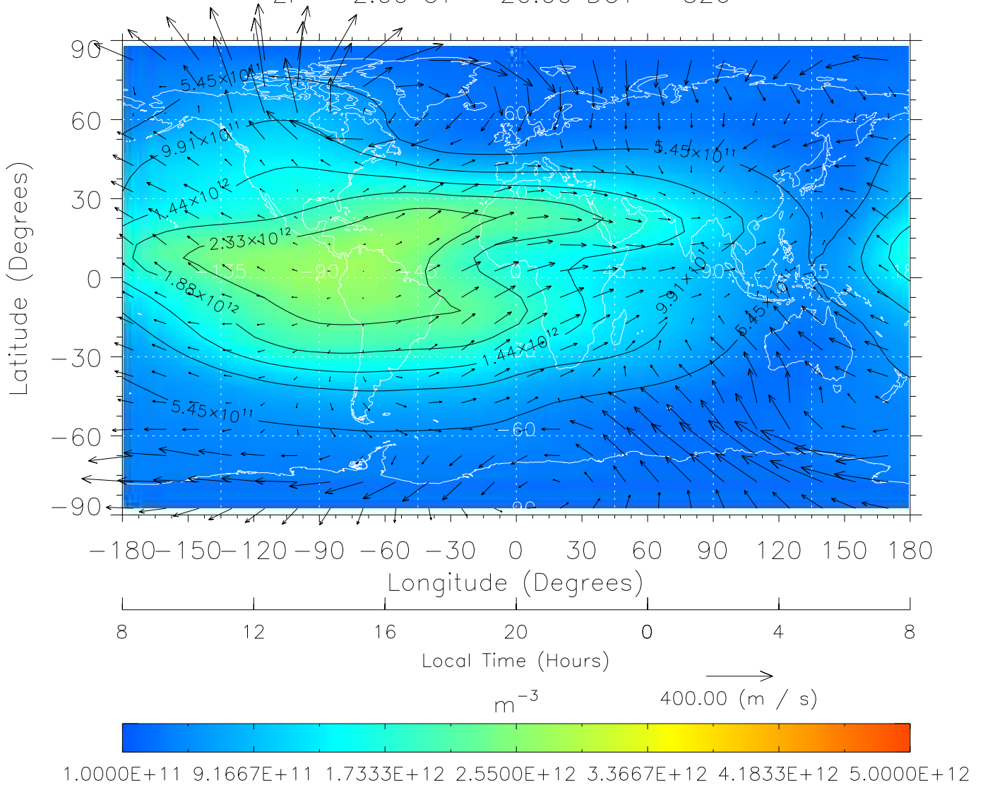
TIME-GCM MAP NmF2 with Neutral Wind vectors ZP = 2.00 UT = 20.00 DOY = 326
