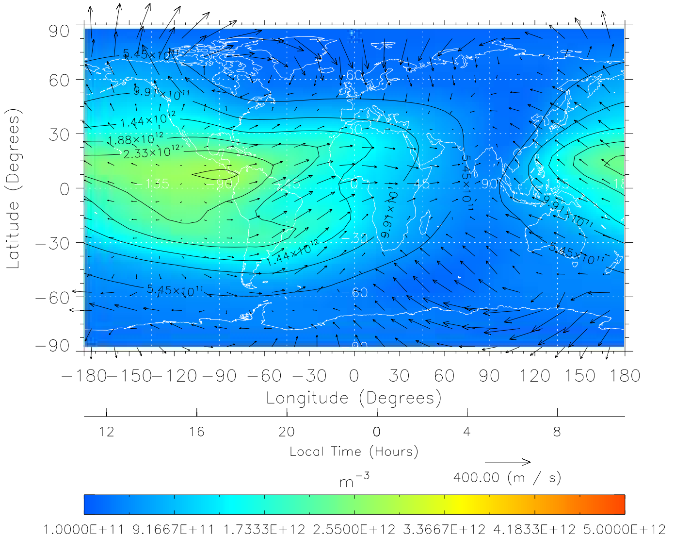
TIME-GCM MAP NmF2 with Neutral Wind vectors ZP = 2.00 UT = 23.00 DOY = 326
