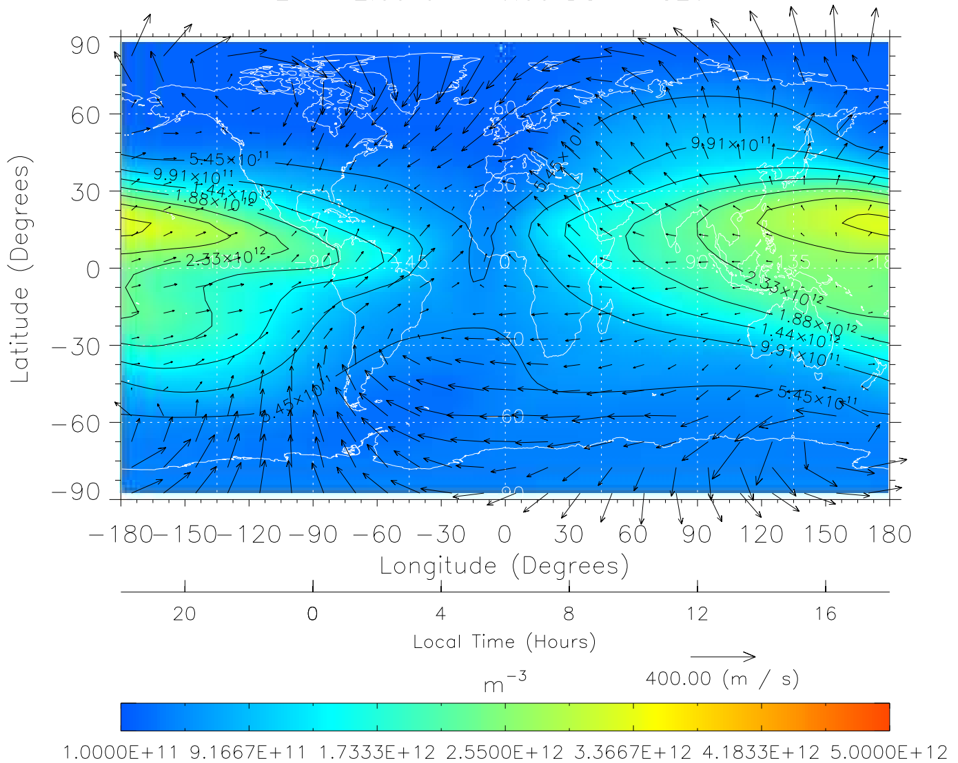
TIME-GCM MAP NmF2 with Neutral Wind vectors ZP = 2.00 UT = 6.00 DOY = 326
