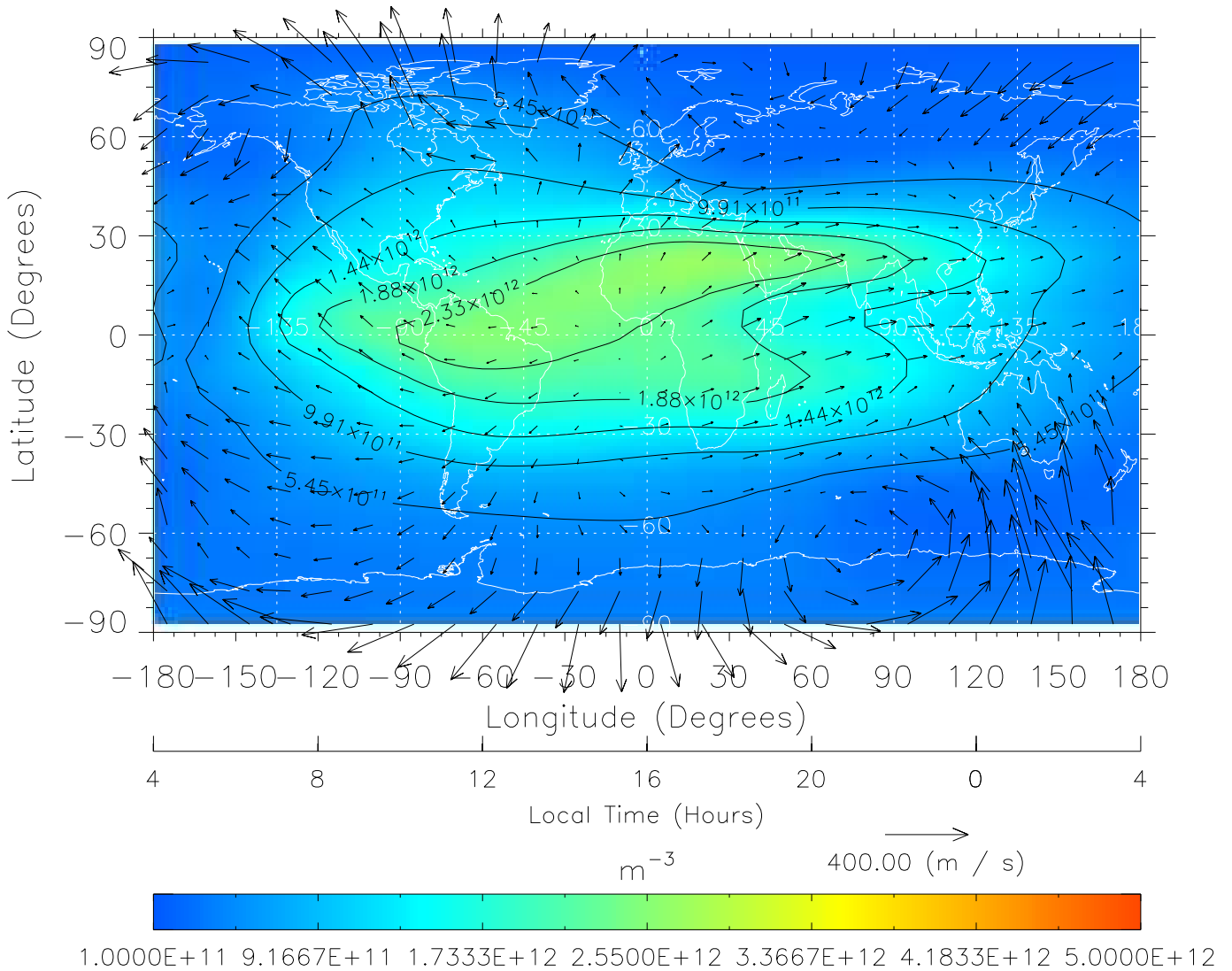
TIME-GCM MAP NmF2 with Neutral Wind vectors ZP = 2.00 UT = 16.00 DOY = 326
