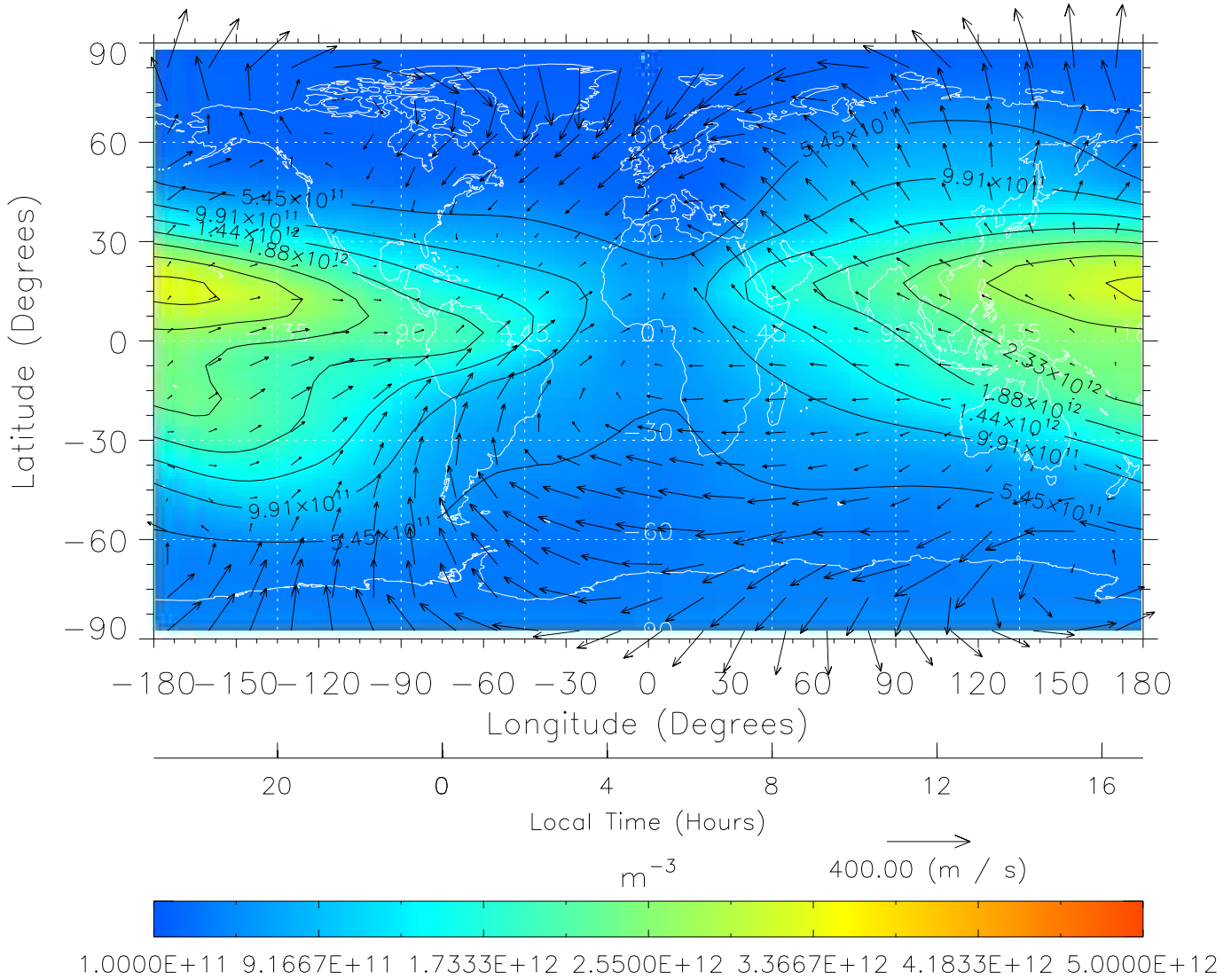
TIME-GCM MAP NmF2 with Neutral Wind vectors ZP = 2.00 UT = 5.00 DOY = 326
