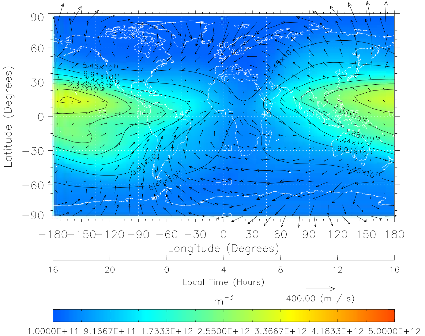
TIME-GCM MAP NmF2 with Neutral Wind vectors ZP = 2.00 UT = 4.00 DOY = 326
