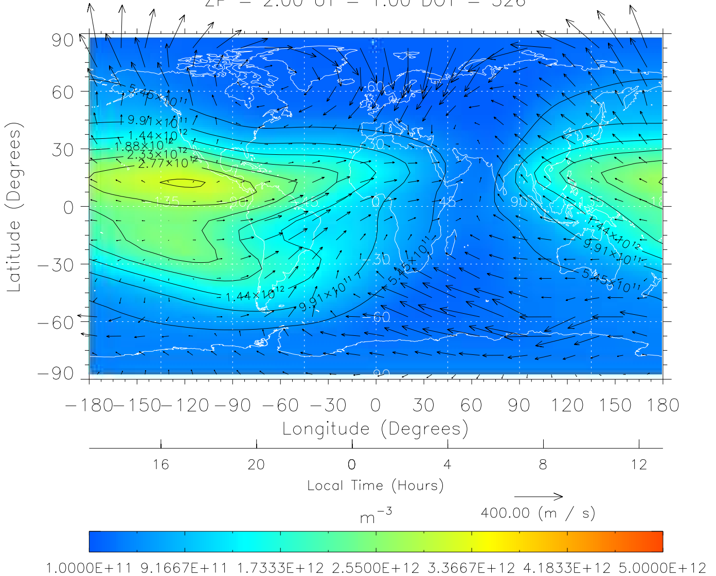
TIME-GCM MAP NmF2 with Neutral Wind vectors ZP = 2.00 UT = 1.00 DOY = 326
