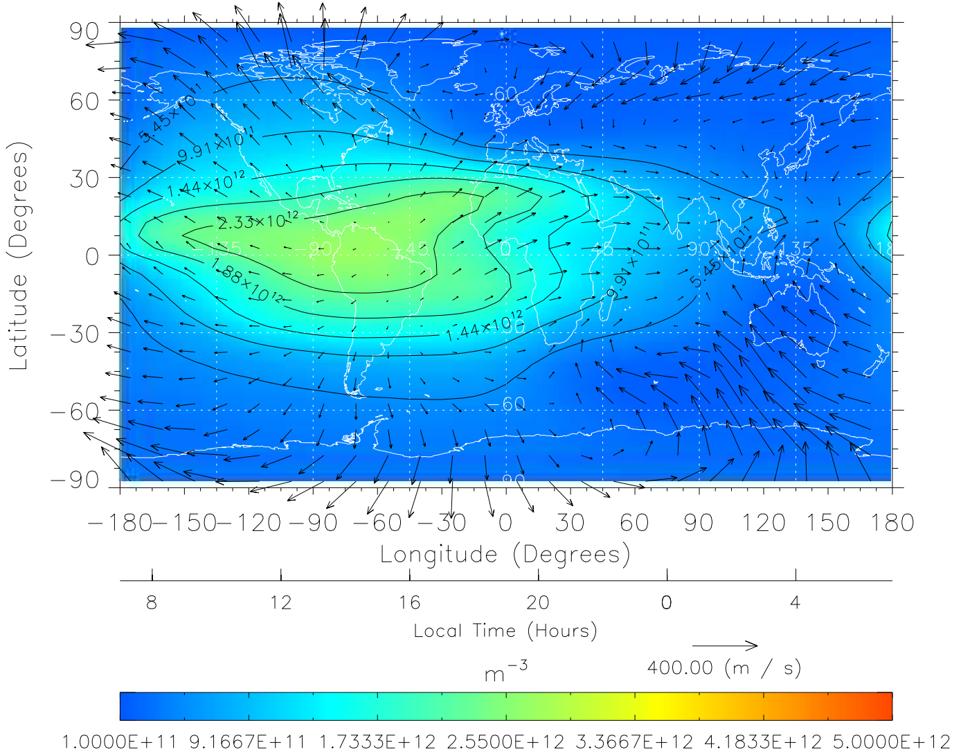
TIME-GCM MAP NmF2 with Neutral Wind vectors ZP = 2.00 UT = 19.00 DOY = 325
