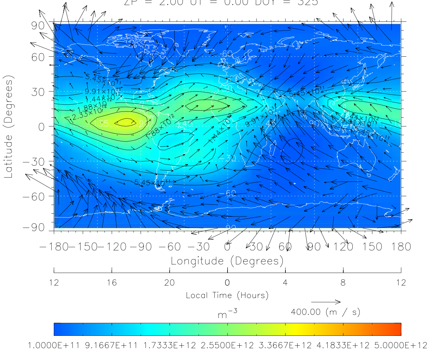
TIME-GCM MAP NmF2 with Neutral Wind vectors ZP = 2.00 UT = 0.00 DOY = 325
