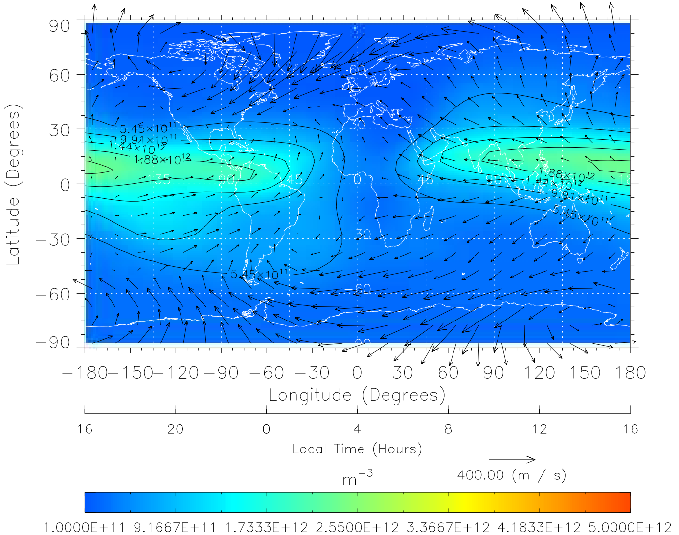
TIME-GCM MAP NmF2 with Neutral Wind vectors ZP = 2.00 UT = 4.00 DOY = 325
