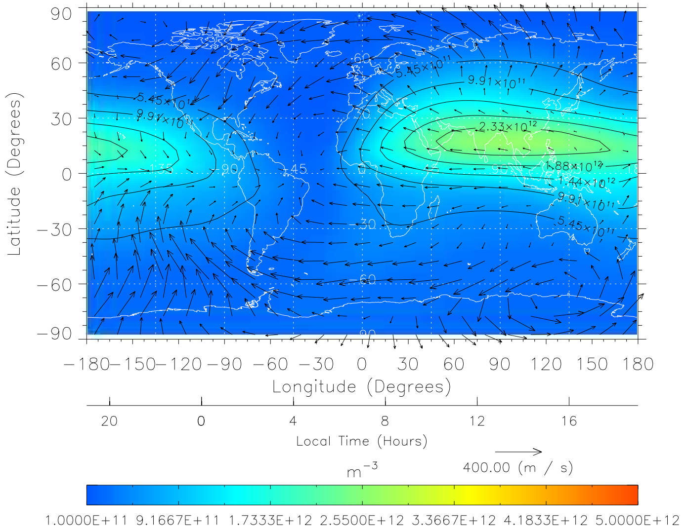
TIME-GCM MAP NmF2 with Neutral Wind vectors ZP = 2.00 UT = 7.00 DOY = 325
