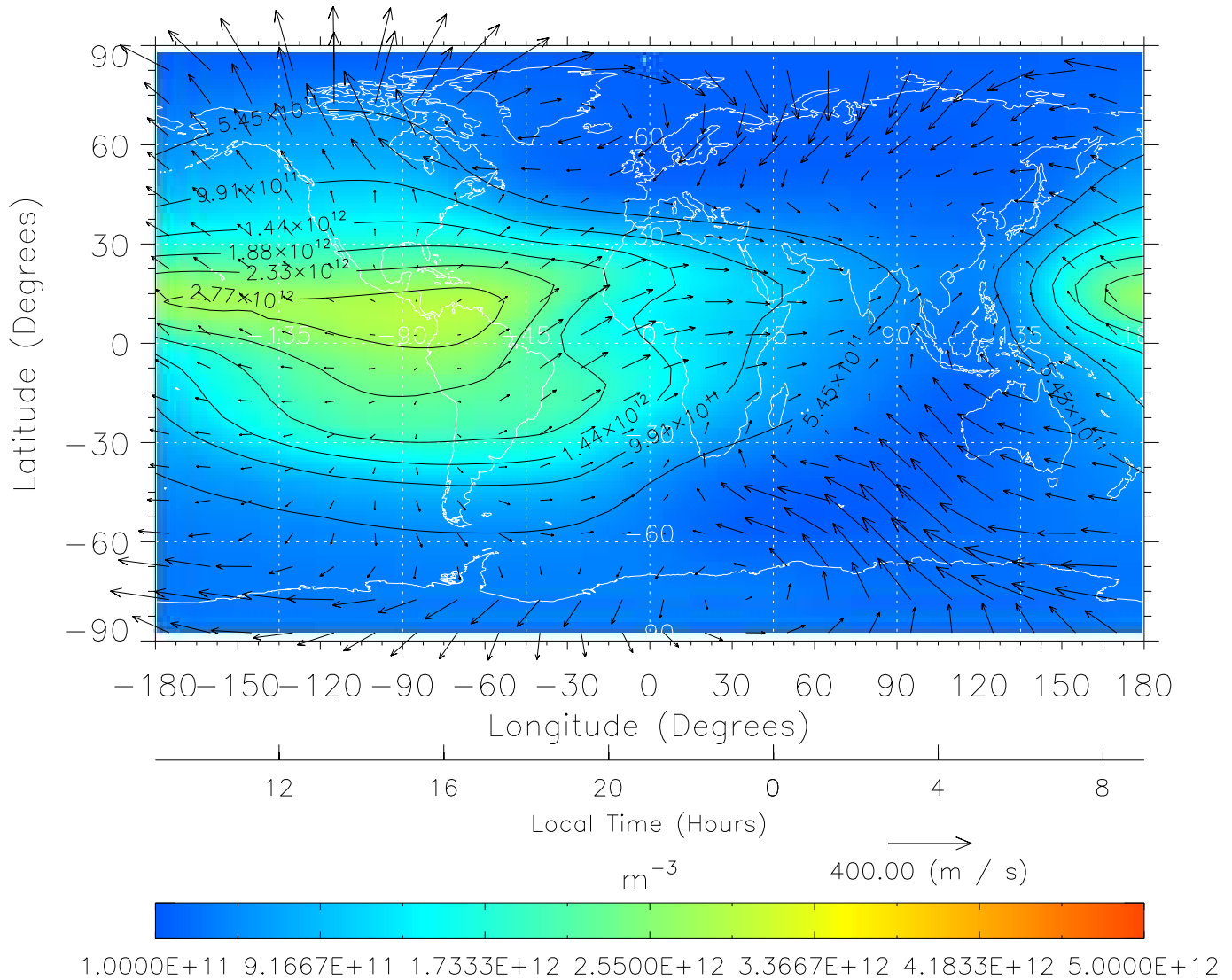
TIME-GCM MAP NmF2 with Neutral Wind vectors ZP = 2.00 UT = 21.00 DOY = 325
