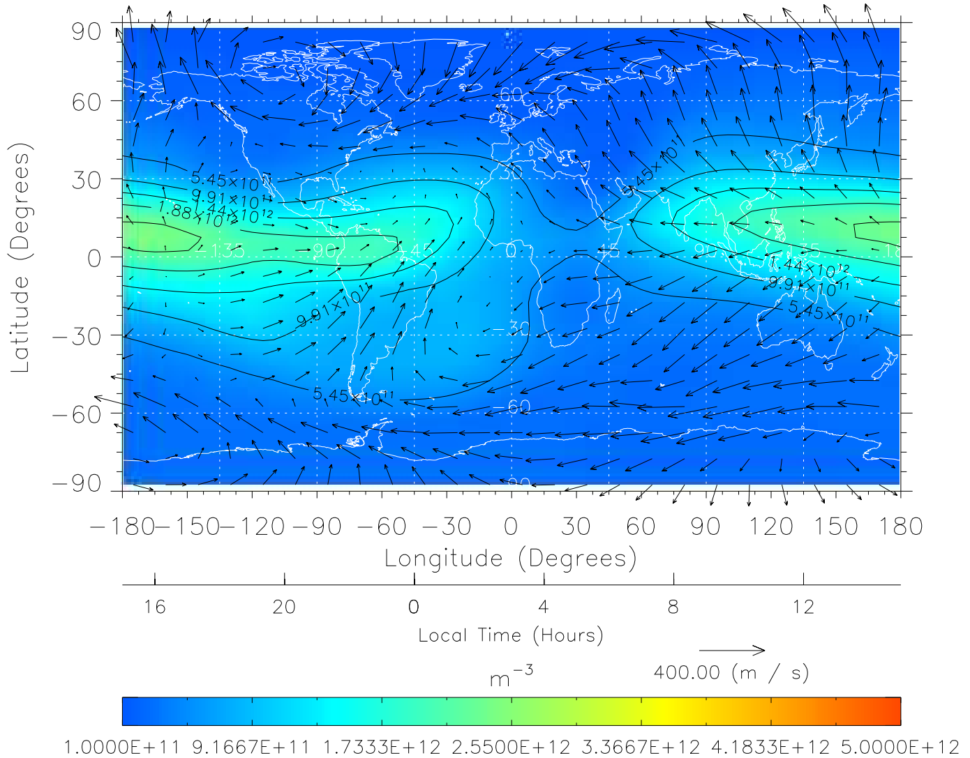
TIME-GCM MAP NmF2 with Neutral Wind vectors ZP = 2.00 UT = 3.00 DOY = 325
