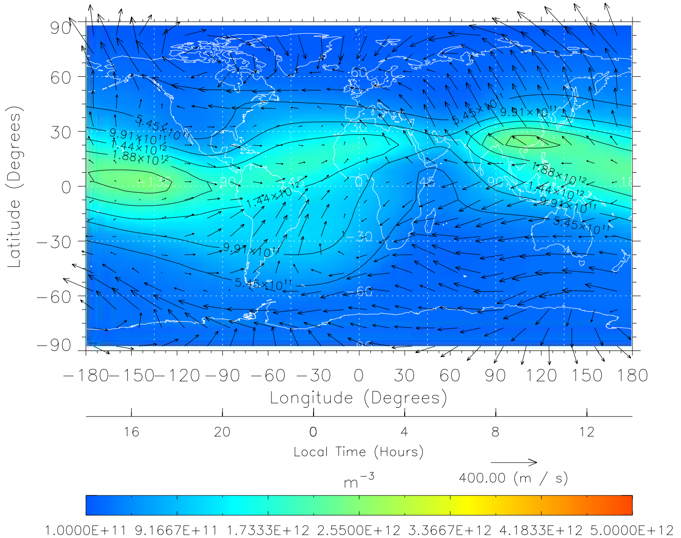
TIME-GCM MAP NmF2 with Neutral Wind vectors ZP = 2.00 UT = 2.00 DOY = 325
