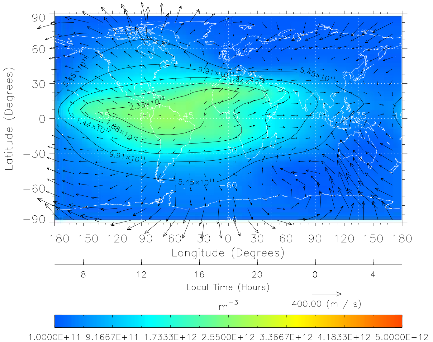
TIME-GCM MAP NmF2 with Neutral Wind vectors ZP = 2.00 UT = 18.00 DOY = 325
