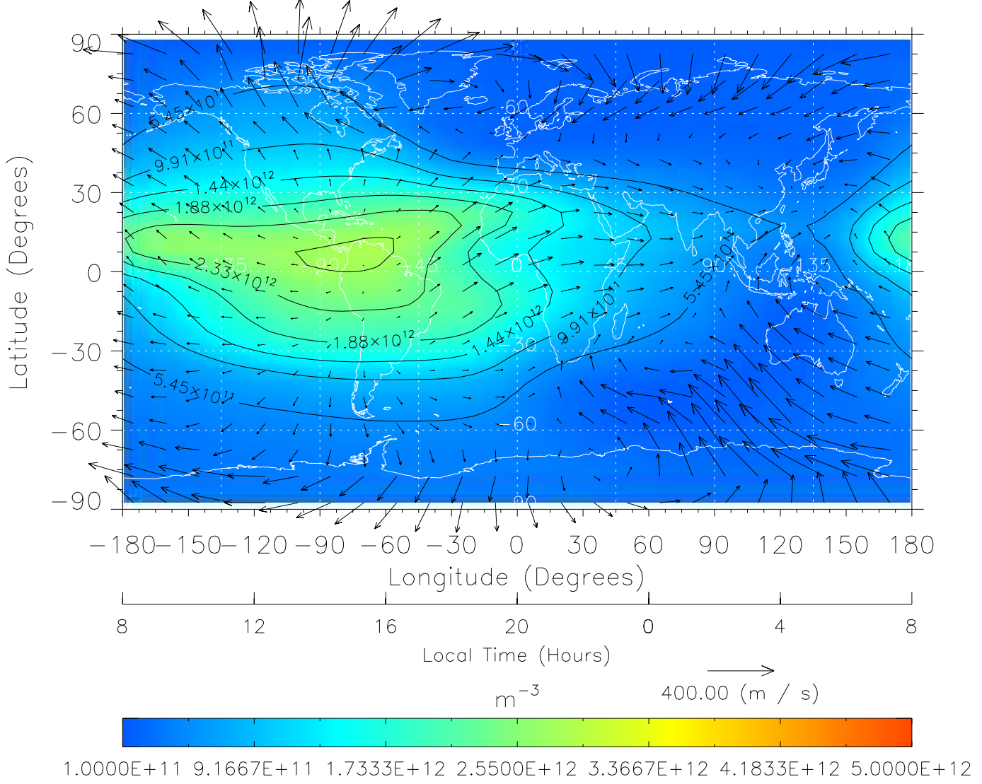
TIME-GCM MAP NmF2 with Neutral Wind vectors ZP = 2.00 UT = 20.00 DOY = 325
