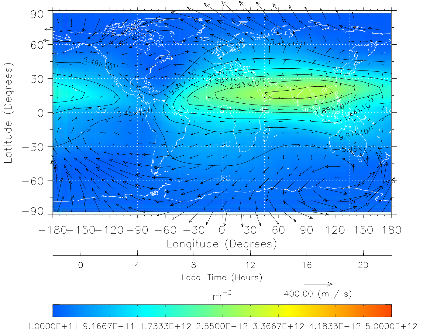
TIME-GCM MAP NmF2 with Neutral Wind vectors ZP = 2.00 UT = 10.00 DOY = 325
