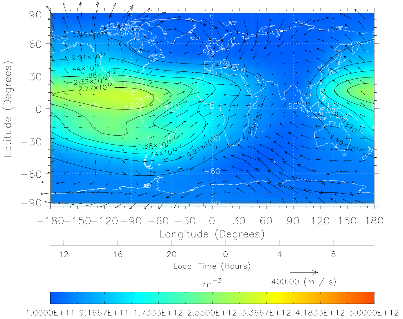
TIME-GCM MAP NmF2 with Neutral Wind vectors ZP = 2.00 UT = 23.00 DOY = 325
