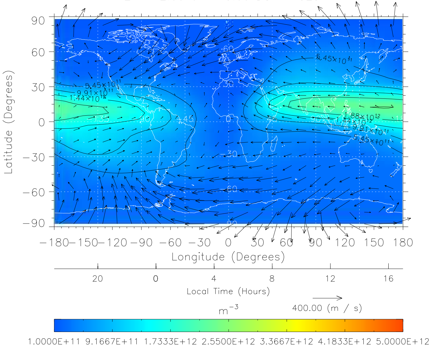
TIME-GCM MAP NmF2 with Neutral Wind vectors ZP = 2.00 UT = 5.00 DOY = 325
