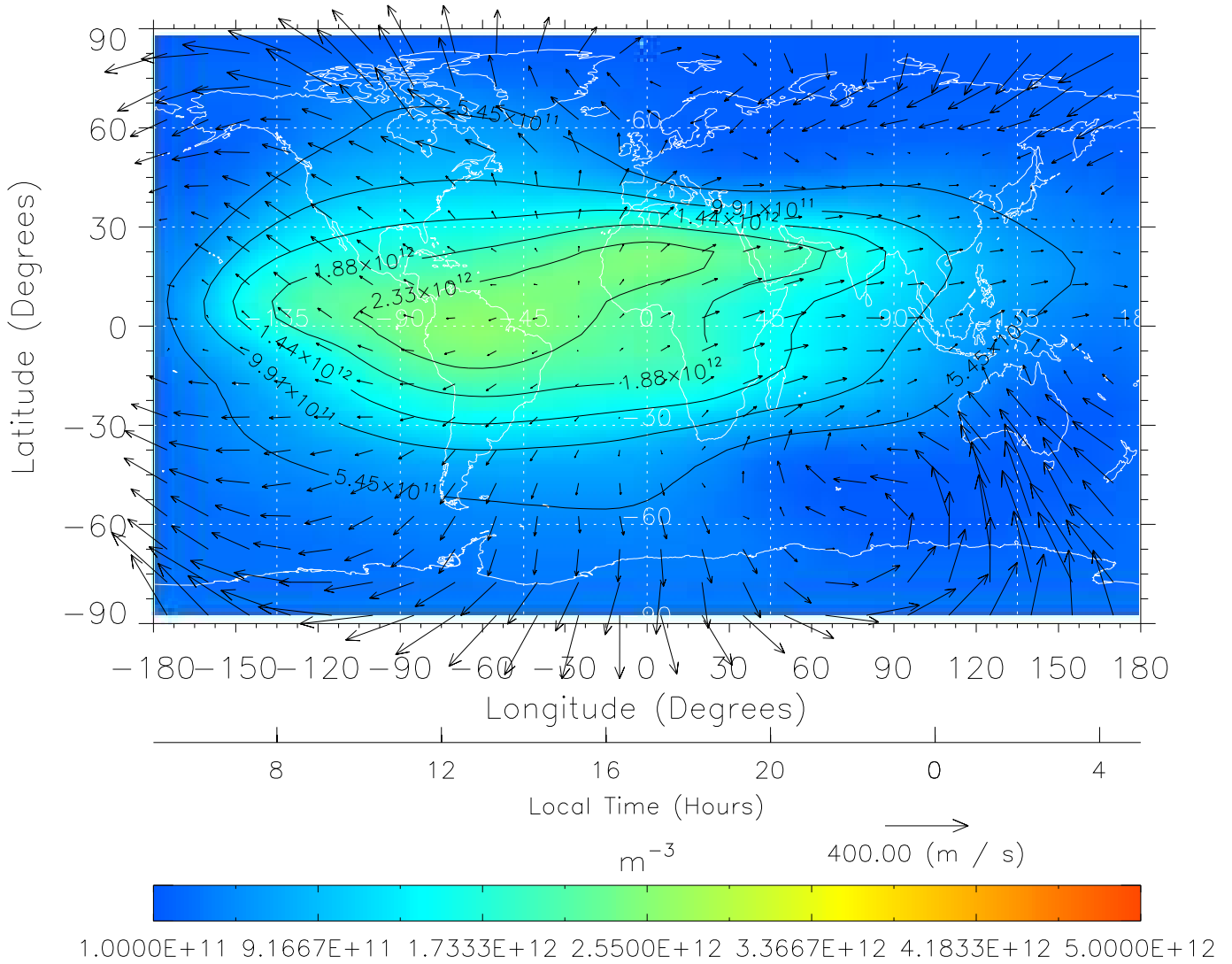
TIME-GCM MAP NmF2 with Neutral Wind vectors ZP = 2.00 UT = 17.00 DOY = 325
