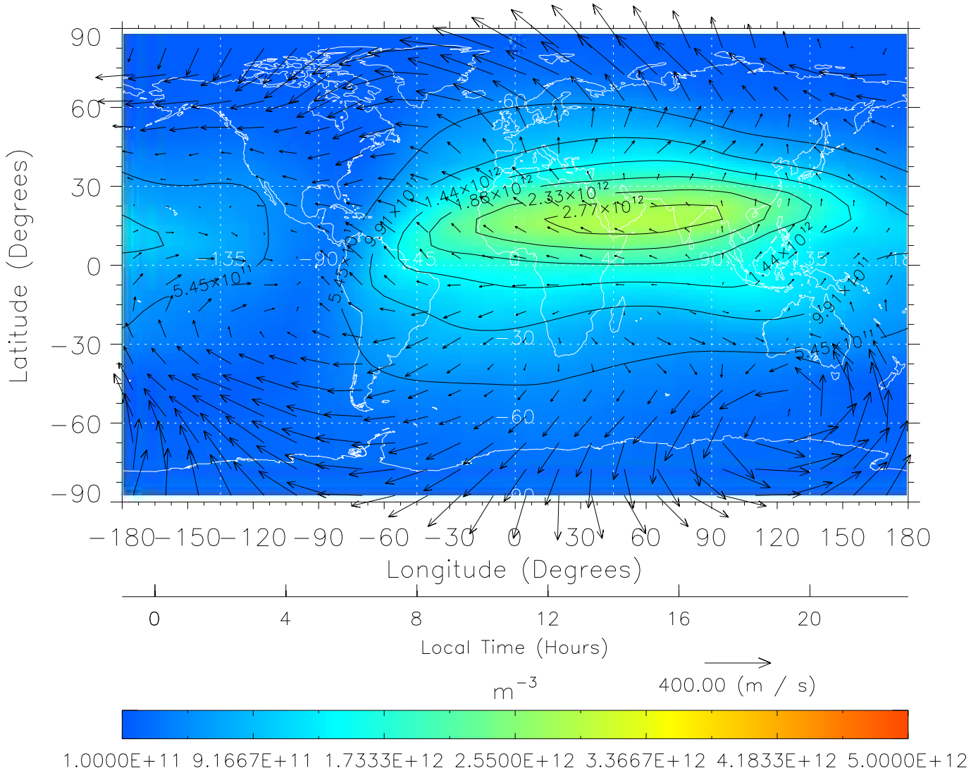
TIME-GCM MAP NmF2 with Neutral Wind vectors ZP = 2.00 UT = 11.00 DOY = 325
