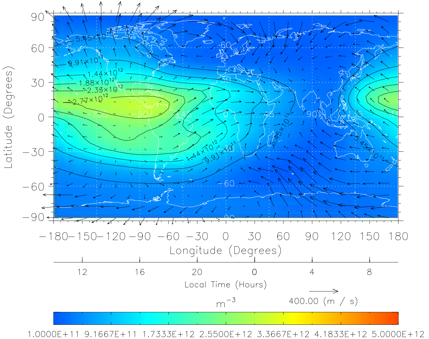
TIME-GCM MAP NmF2 with Neutral Wind vectors ZP = 2.00 UT = 22.00 DOY = 325
