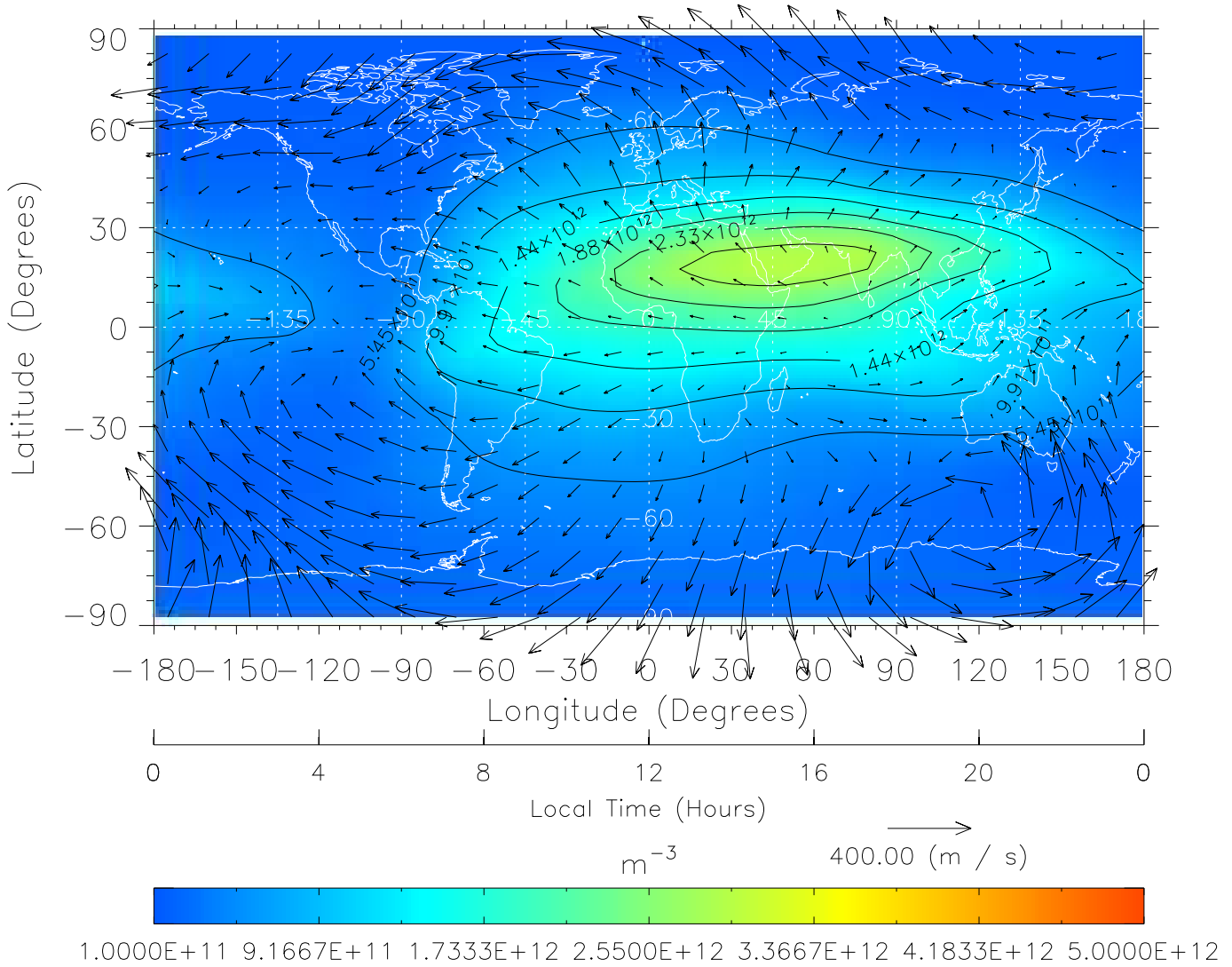
TIME-GCM MAP NmF2 with Neutral Wind vectors ZP = 2.00 UT = 12.00 DOY = 325
