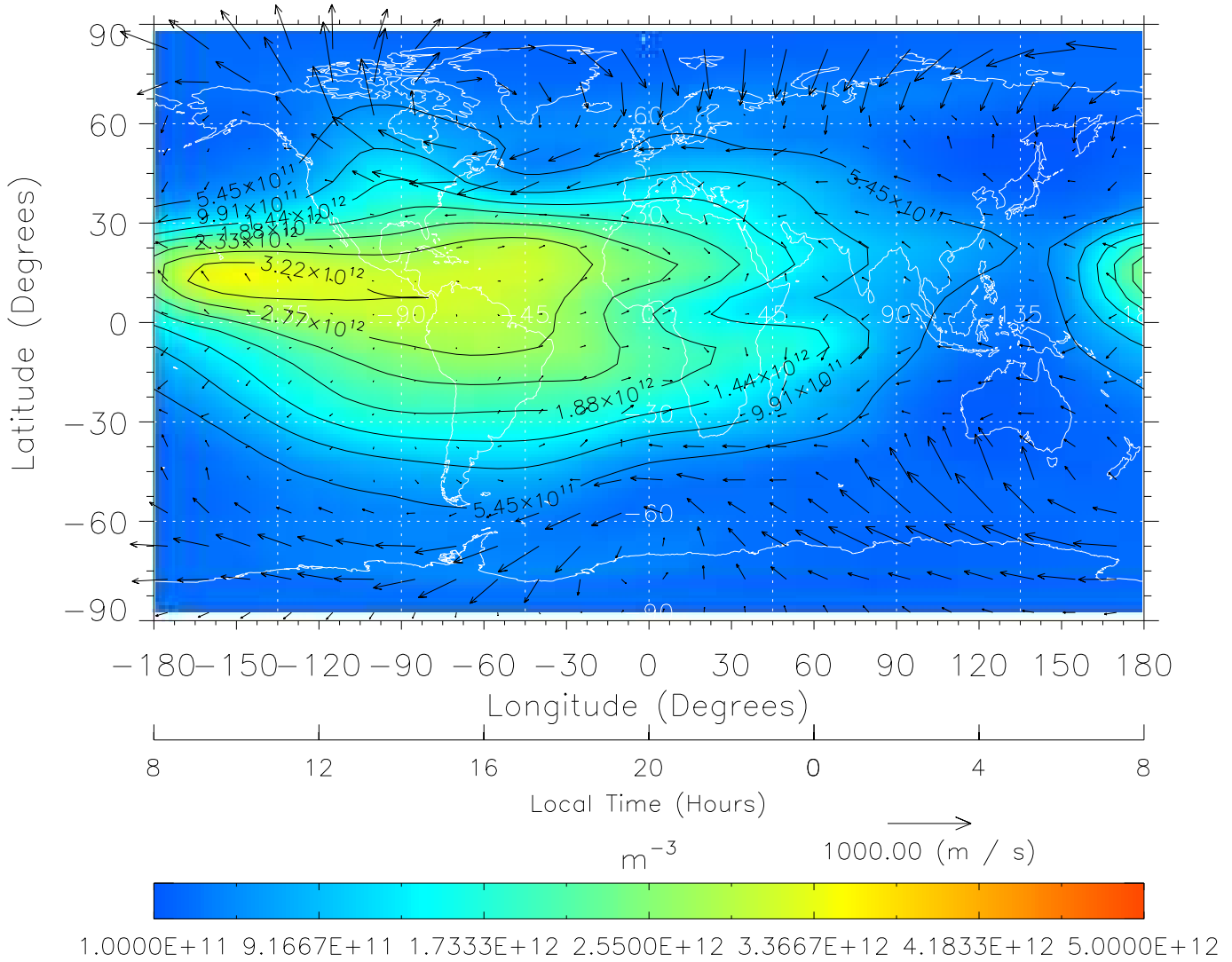
TIME-GCM MAP NmF2 with Neutral Wind vectors ZP = 2.00 UT = 20.00 DOY = 324
