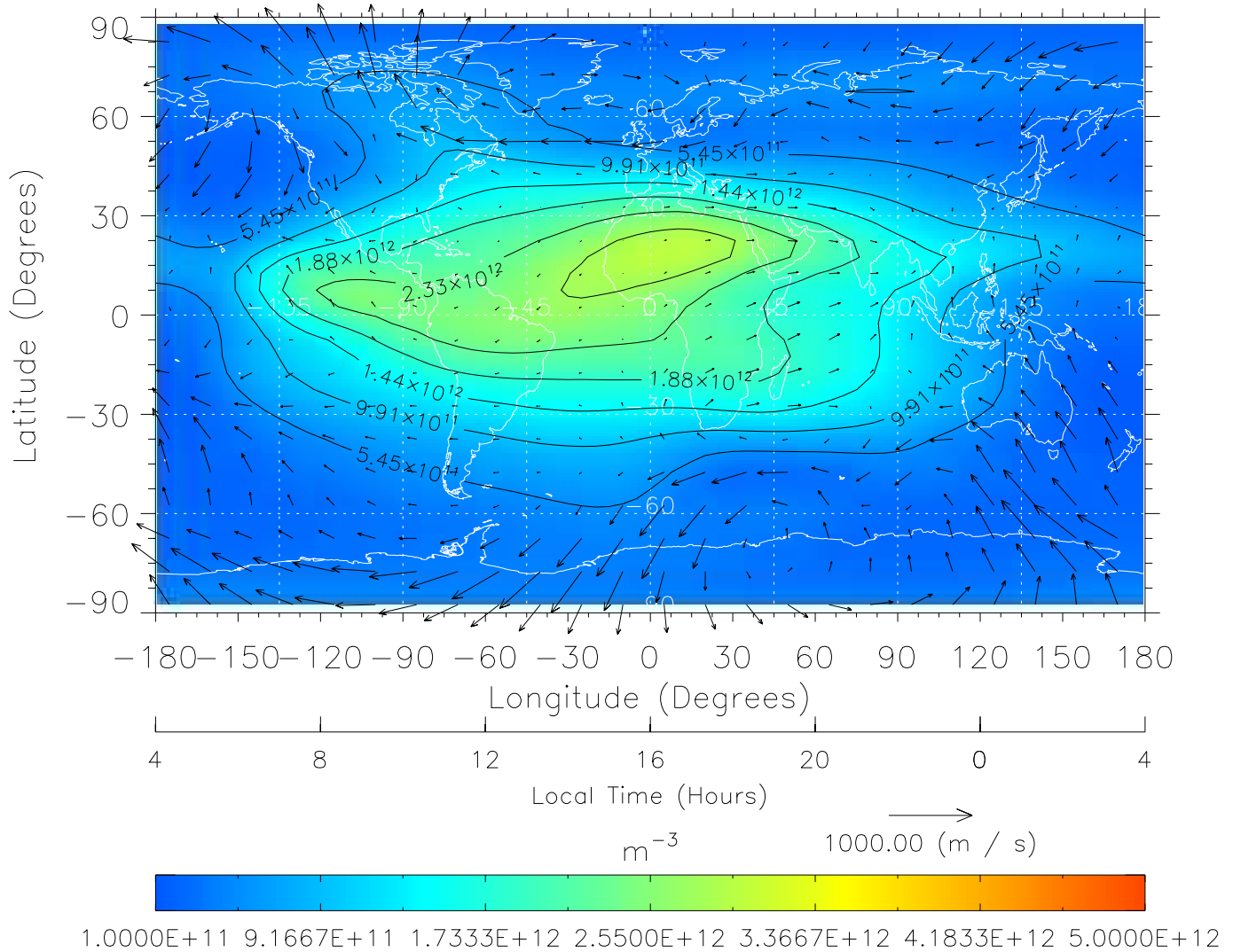
TIME-GCM MAP NmF2 with Neutral Wind vectors ZP = 2.00 UT = 16.00 DOY = 324
