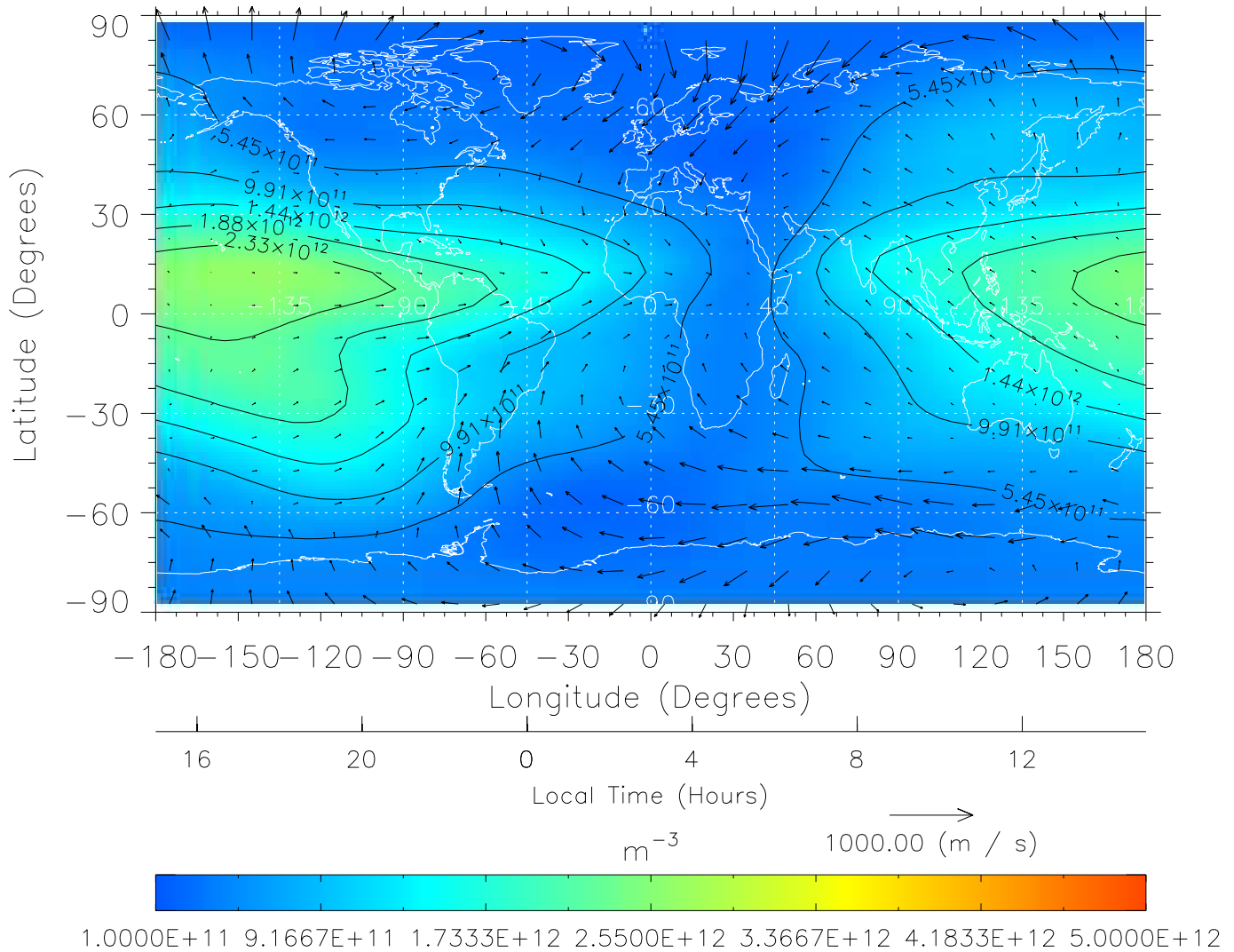
TIME-GCM MAP NmF2 with Neutral Wind vectors ZP = 2.00 UT = 3.00 DOY = 324
