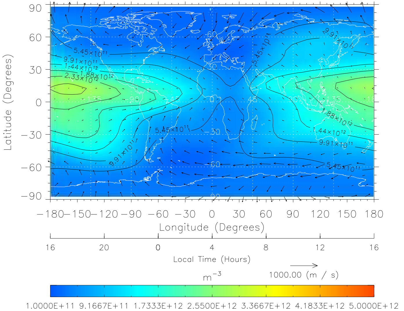
TIME-GCM MAP NmF2 with Neutral Wind vectors ZP = 2.00 UT = 4.00 DOY = 324
