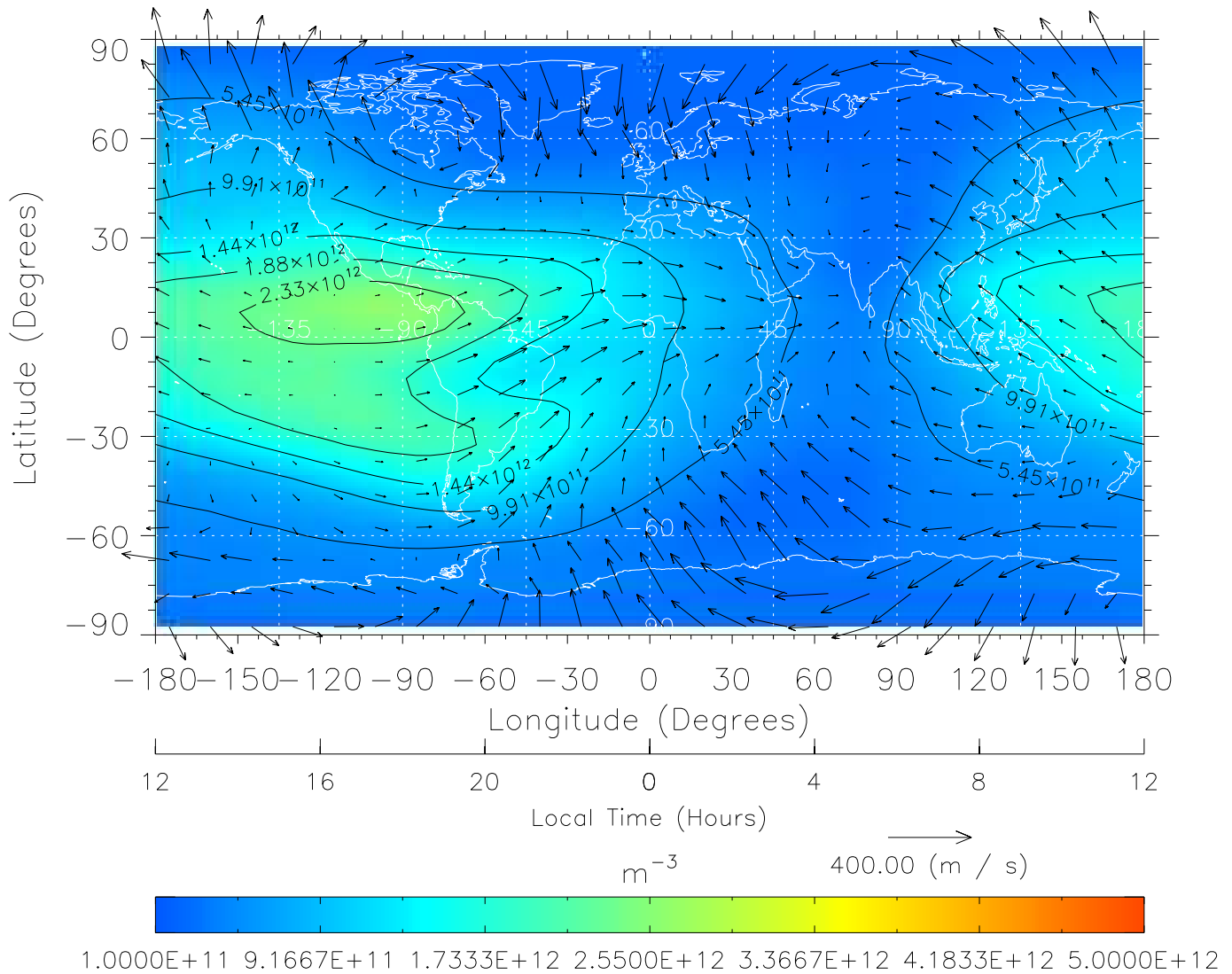
TIME-GCM MAP NmF2 with Neutral Wind vectors ZP = 2.00 UT = 0.00 DOY = 323
