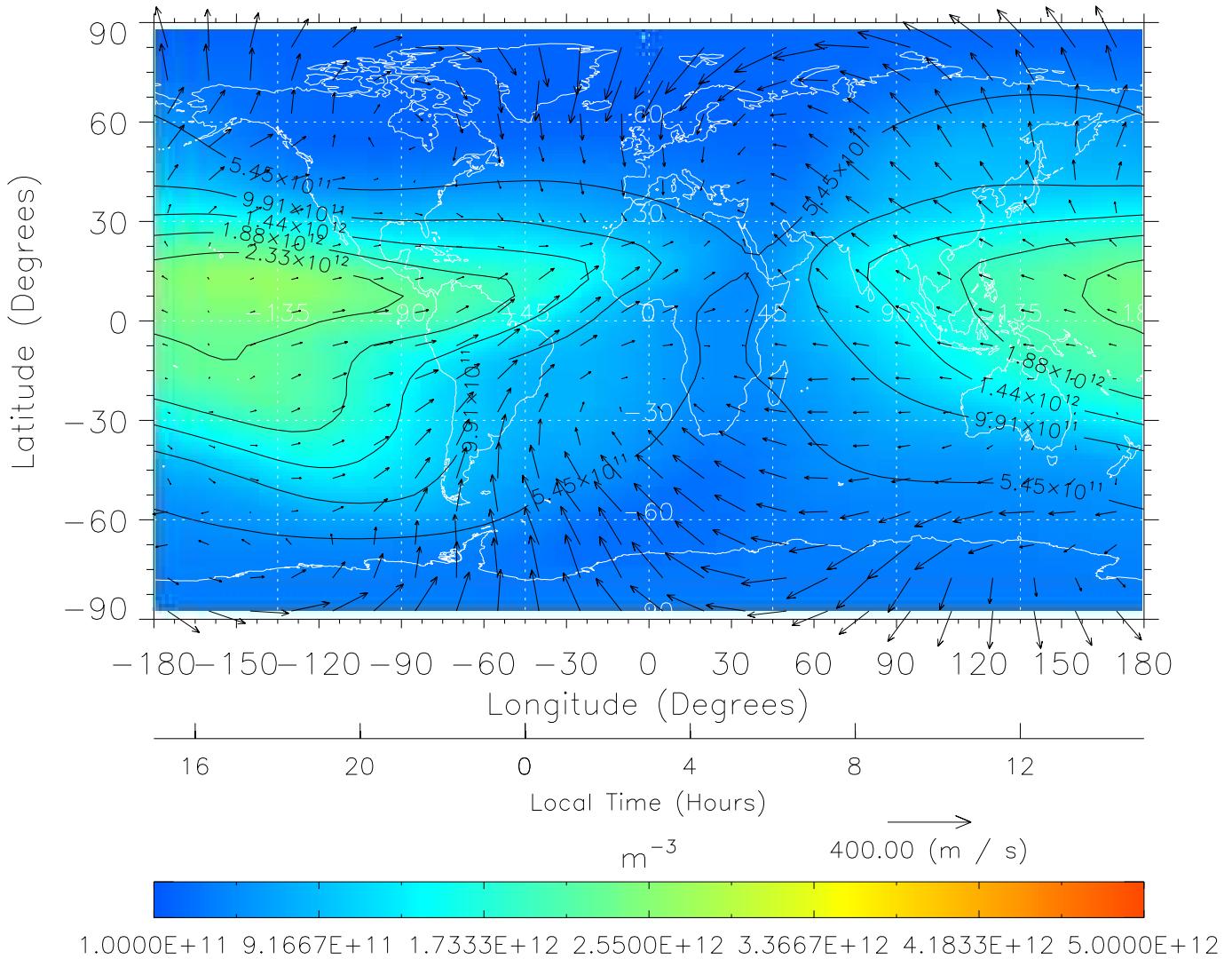
TIME-GCM MAP NmF2 with Neutral Wind vectors ZP = 2.00 UT = 3.00 DOY = 323
