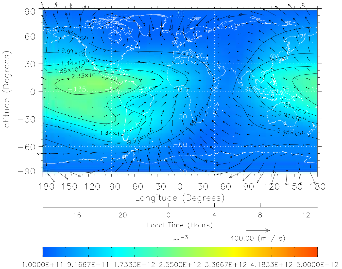
TIME-GCM MAP NmF2 with Neutral Wind vectors ZP = 2.00 UT = 1.00 DOY = 323
