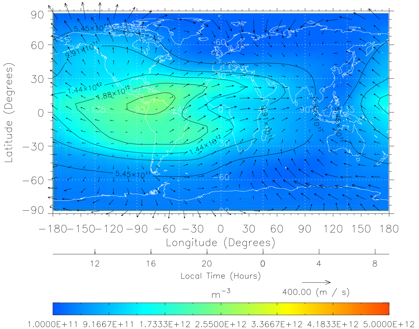
TIME-GCM MAP NmF2 with Neutral Wind vectors ZP = 2.00 UT = 21.00 DOY = 323
