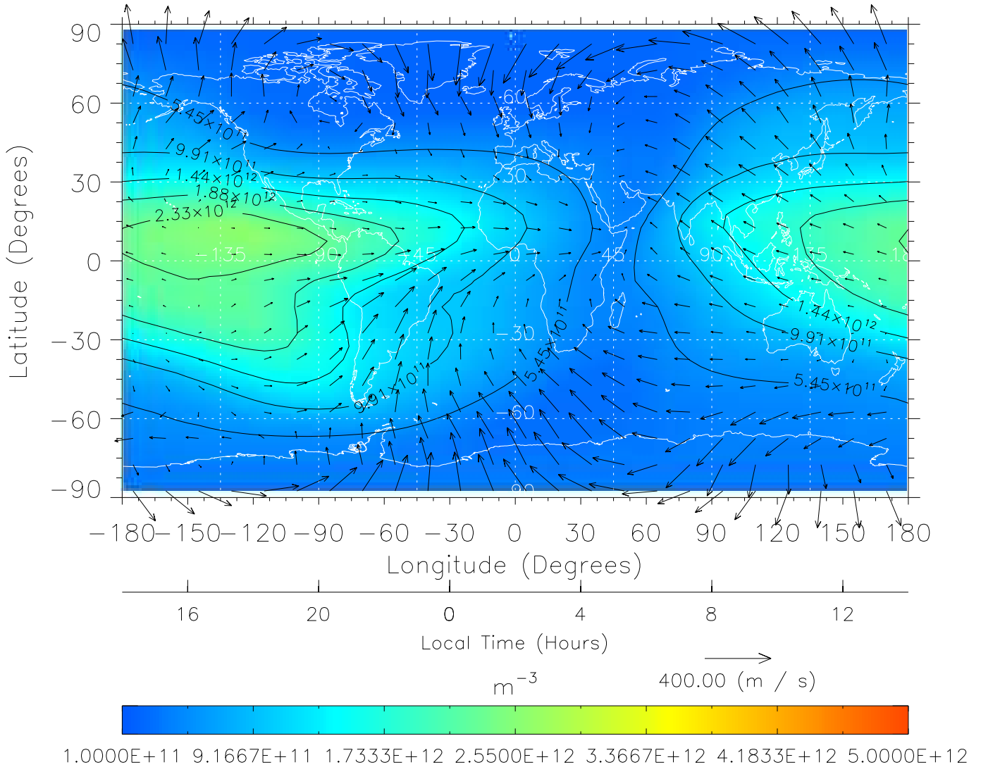
TIME-GCM MAP NmF2 with Neutral Wind vectors ZP = 2.00 UT = 2.00 DOY = 323
