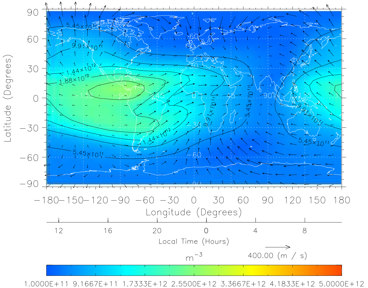
TIME-GCM MAP NmF2 with Neutral Wind vectors ZP = 2.00 UT = 23.00 DOY = 323
