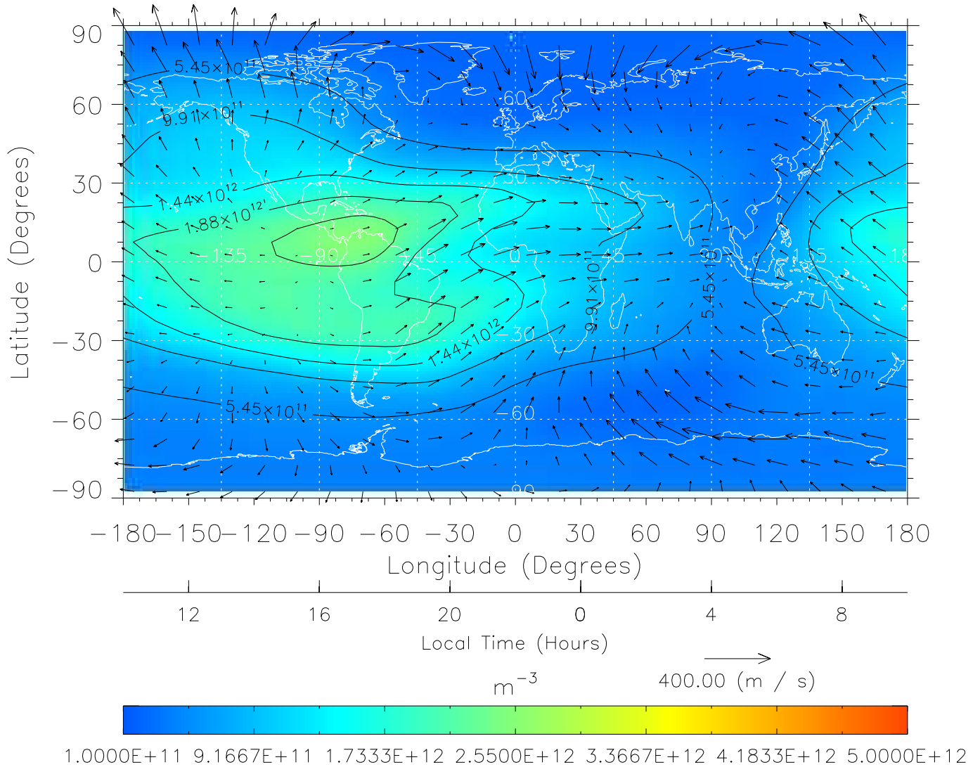
TIME-GCM MAP NmF2 with Neutral Wind vectors ZP = 2.00 UT = 22.00 DOY = 323
