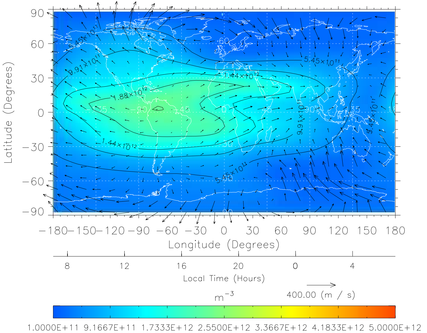
TIME-GCM MAP NmF2 with Neutral Wind vectors ZP = 2.00 UT = 19.00 DOY = 322
