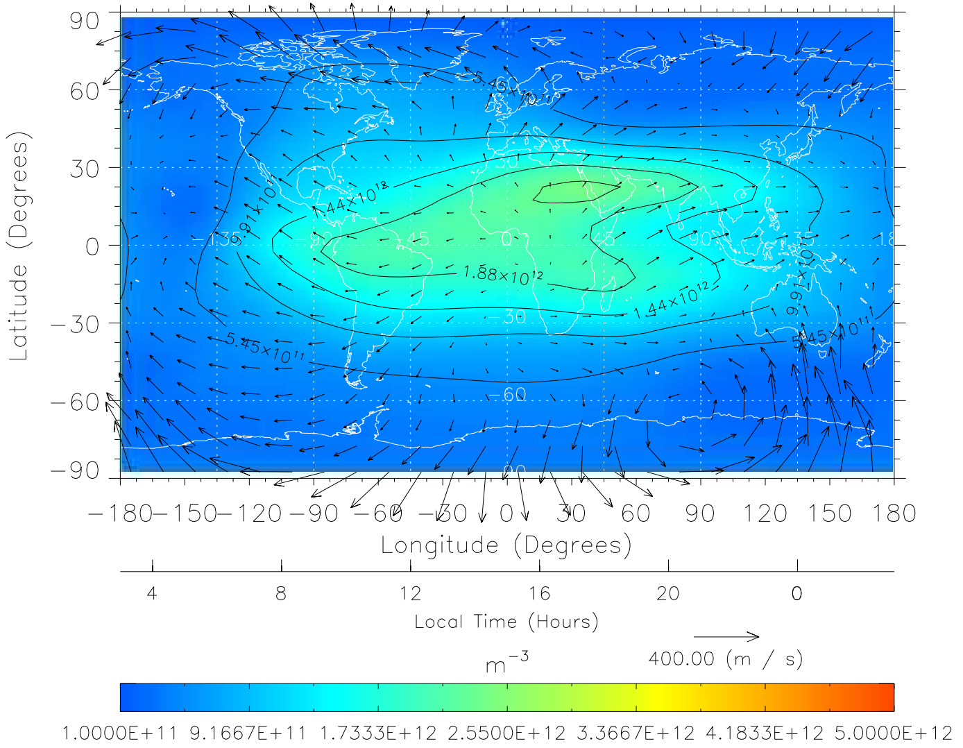
TIME-GCM MAP NmF2 with Neutral Wind vectors ZP = 2.00 UT = 15.00 DOY = 322
