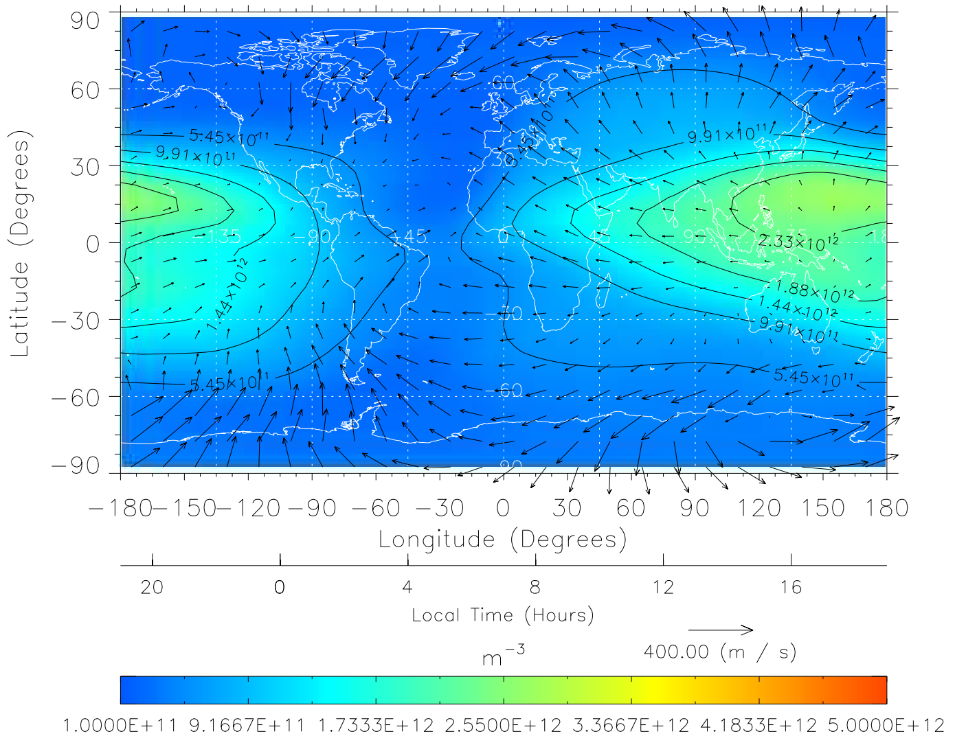
TIME-GCM MAP NmF2 with Neutral Wind vectors ZP = 2.00 UT = 7.00 DOY = 322
