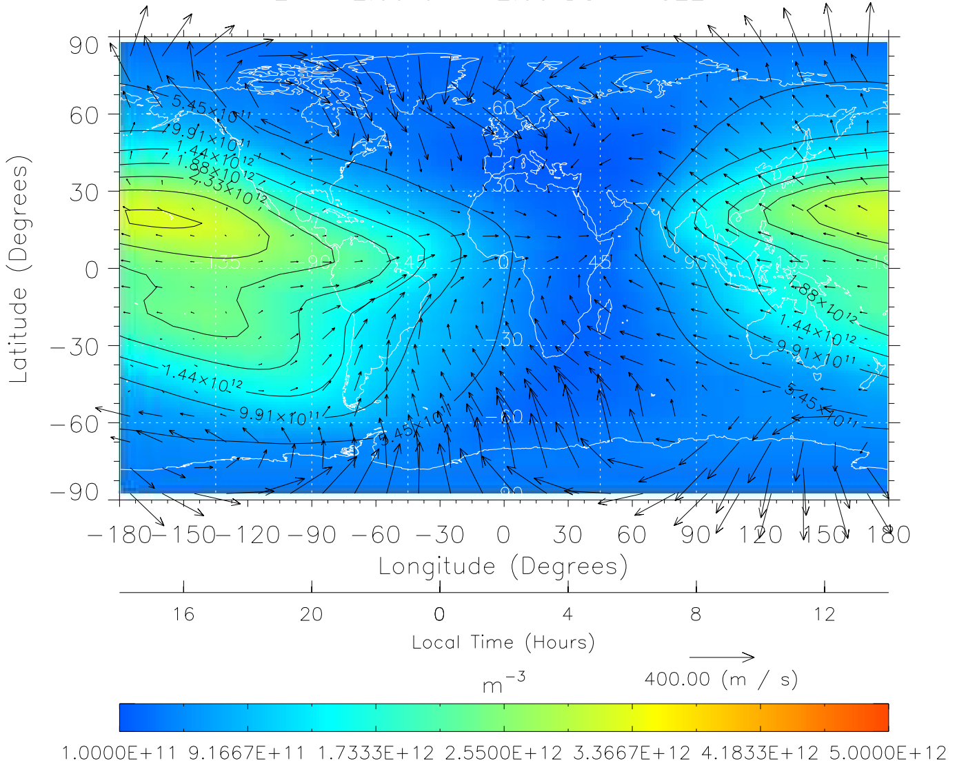
TIME-GCM MAP NmF2 with Neutral Wind vectors ZP = 2.00 UT = 2.00 DOY = 322
