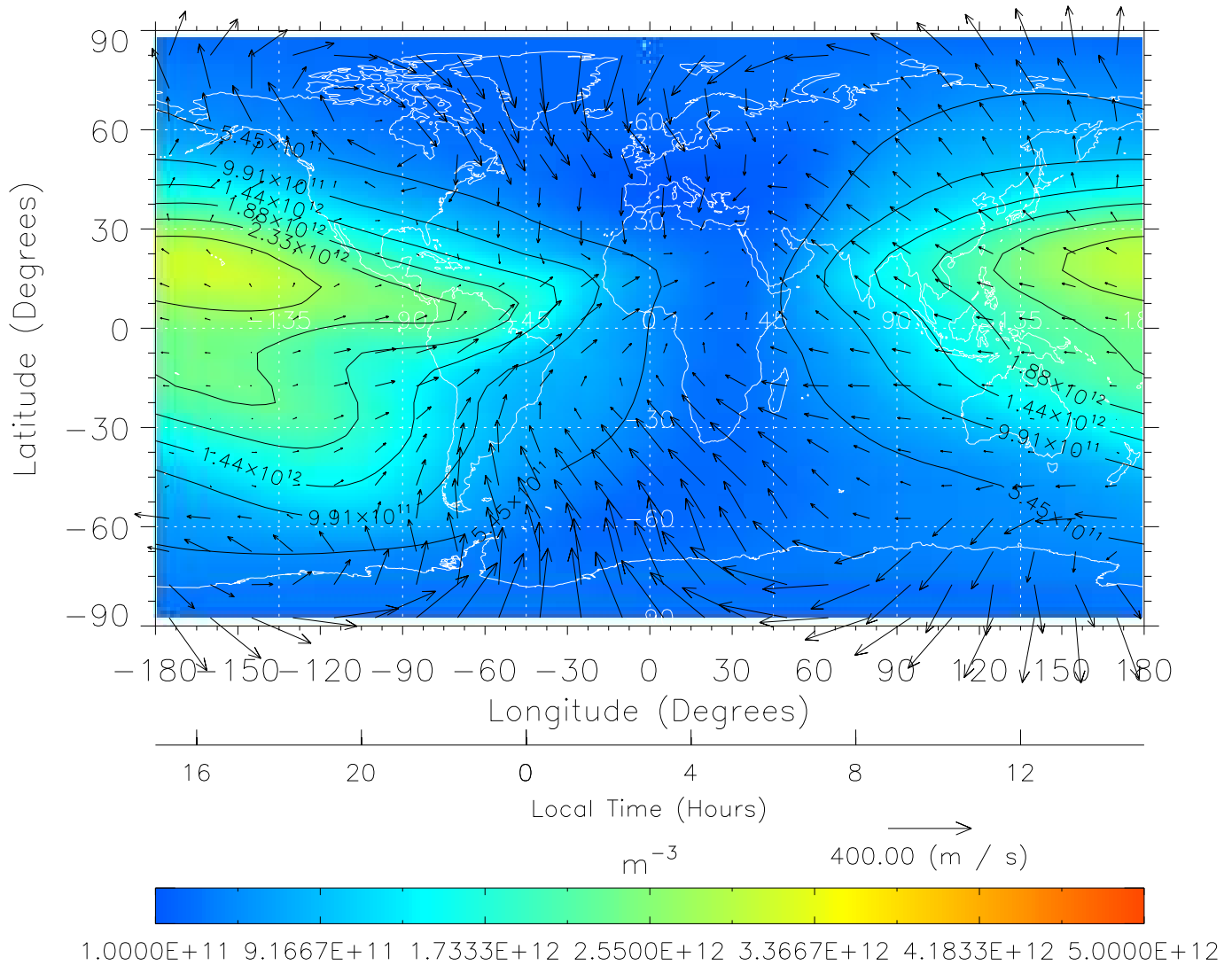
TIME-GCM MAP NmF2 with Neutral Wind vectors ZP = 2.00 UT = 3.00 DOY = 322
