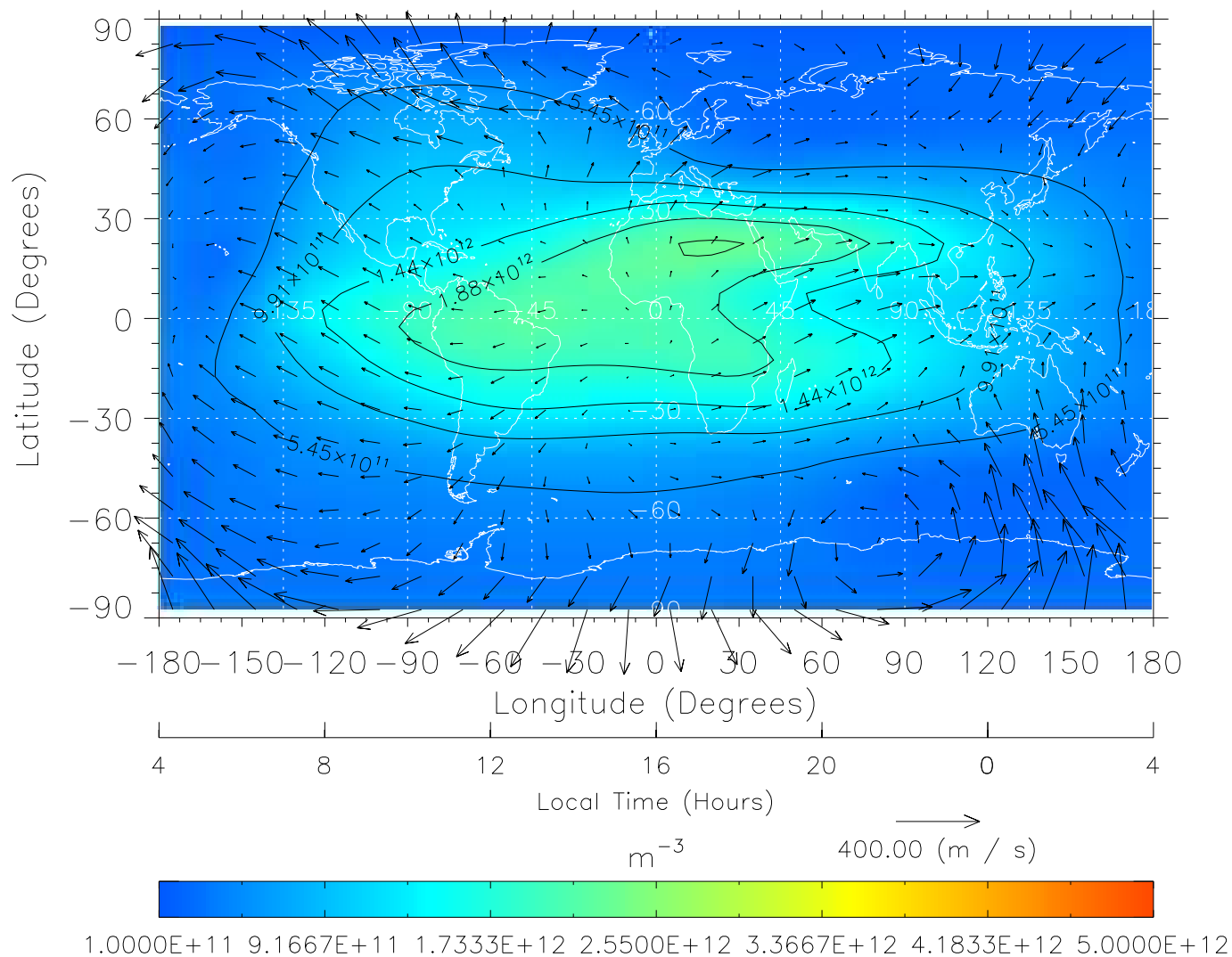
TIME-GCM MAP NmF2 with Neutral Wind vectors ZP = 2.00 UT = 16.00 DOY = 322
