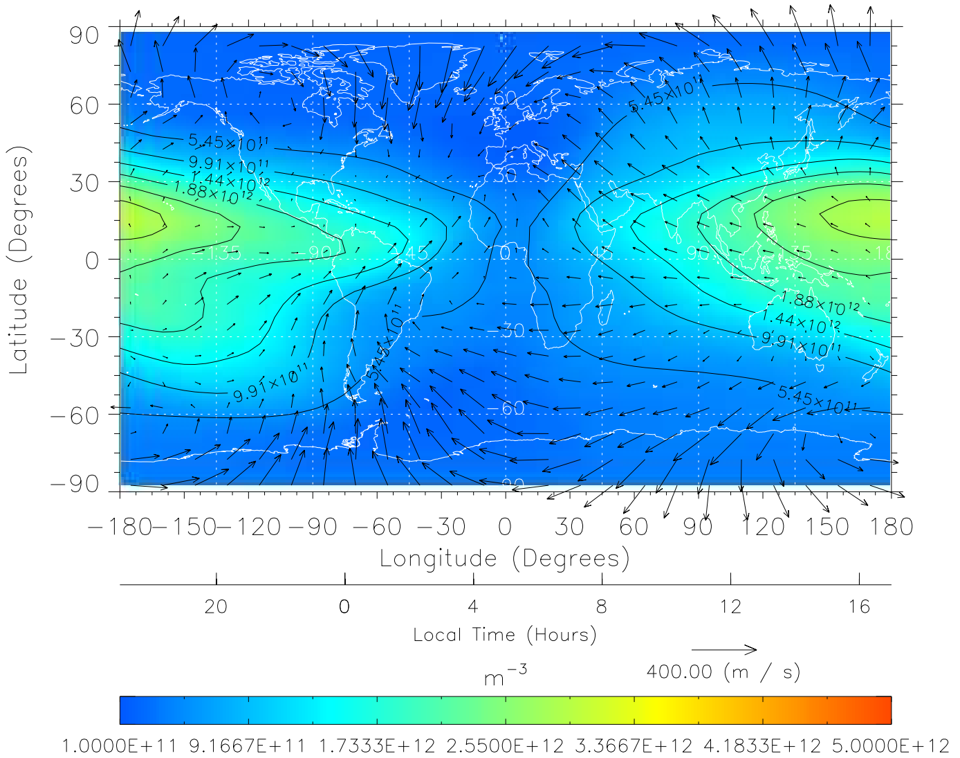
TIME-GCM MAP NmF2 with Neutral Wind vectors ZP = 2.00 UT = 5.00 DOY = 322
