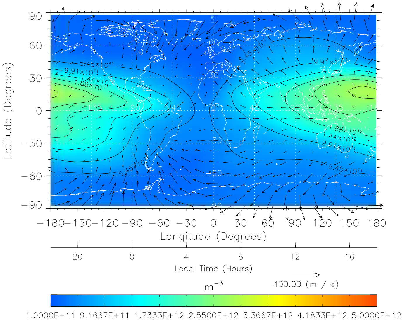
TIME-GCM MAP NmF2 with Neutral Wind vectors ZP = 2.00 UT = 6.00 DOY = 322
