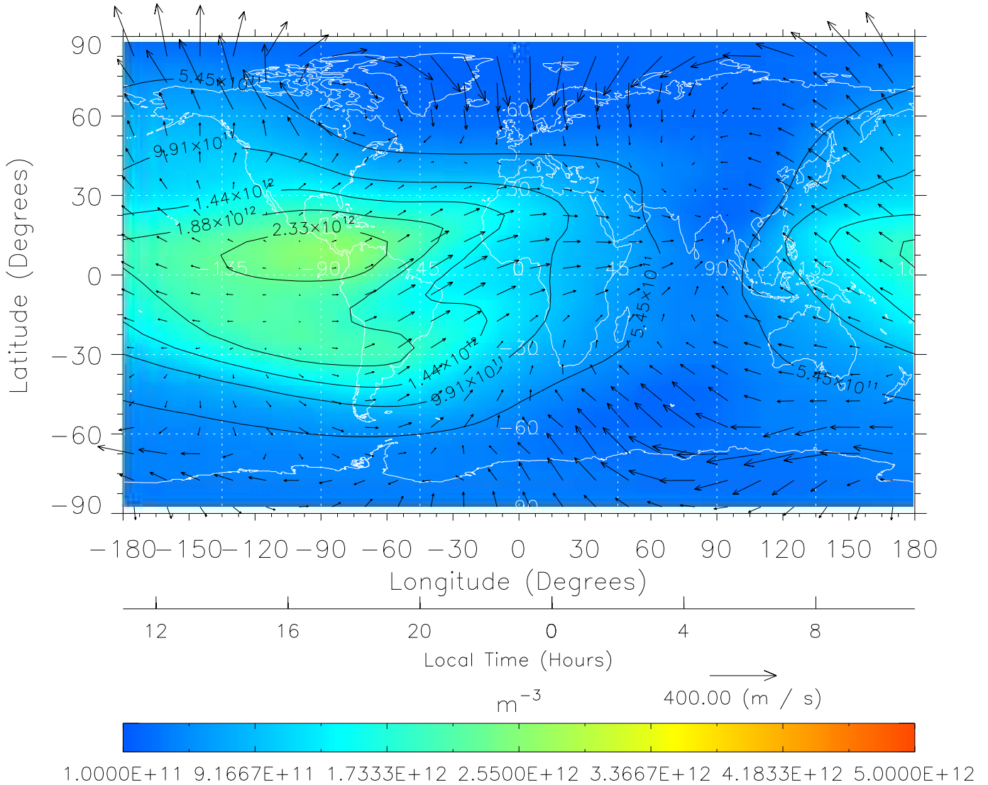
TIME-GCM MAP NmF2 with Neutral Wind vectors ZP = 2.00 UT = 23.00 DOY = 322
