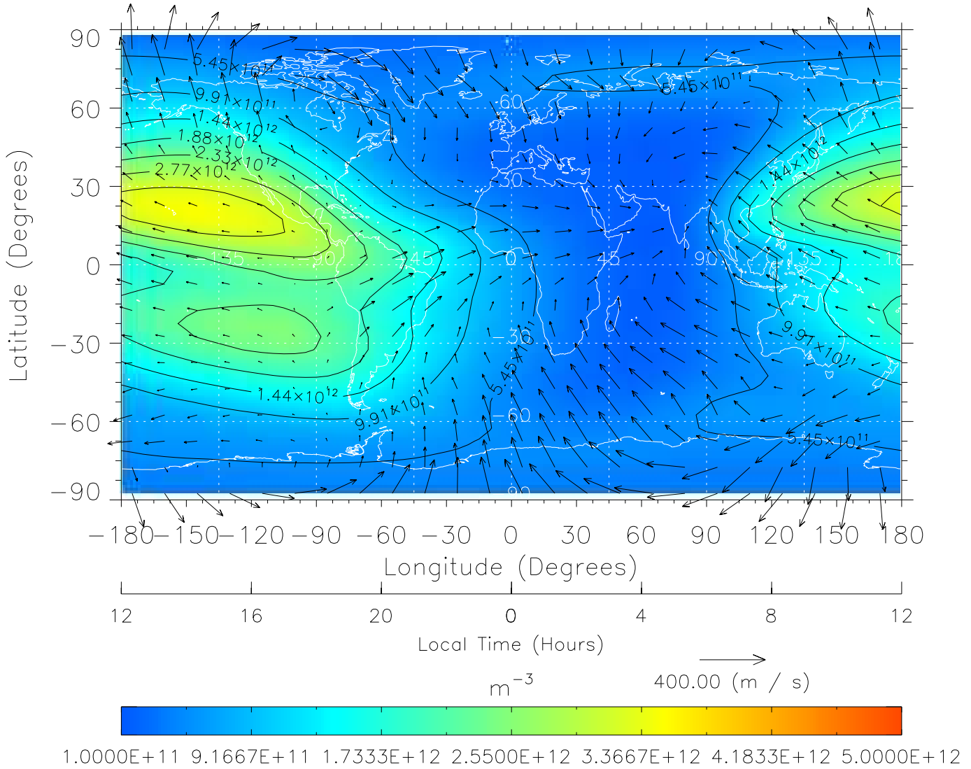
TIME-GCM MAP NmF2 with Neutral Wind vectors ZP = 2.00 UT = 0.00 DOY = 322
