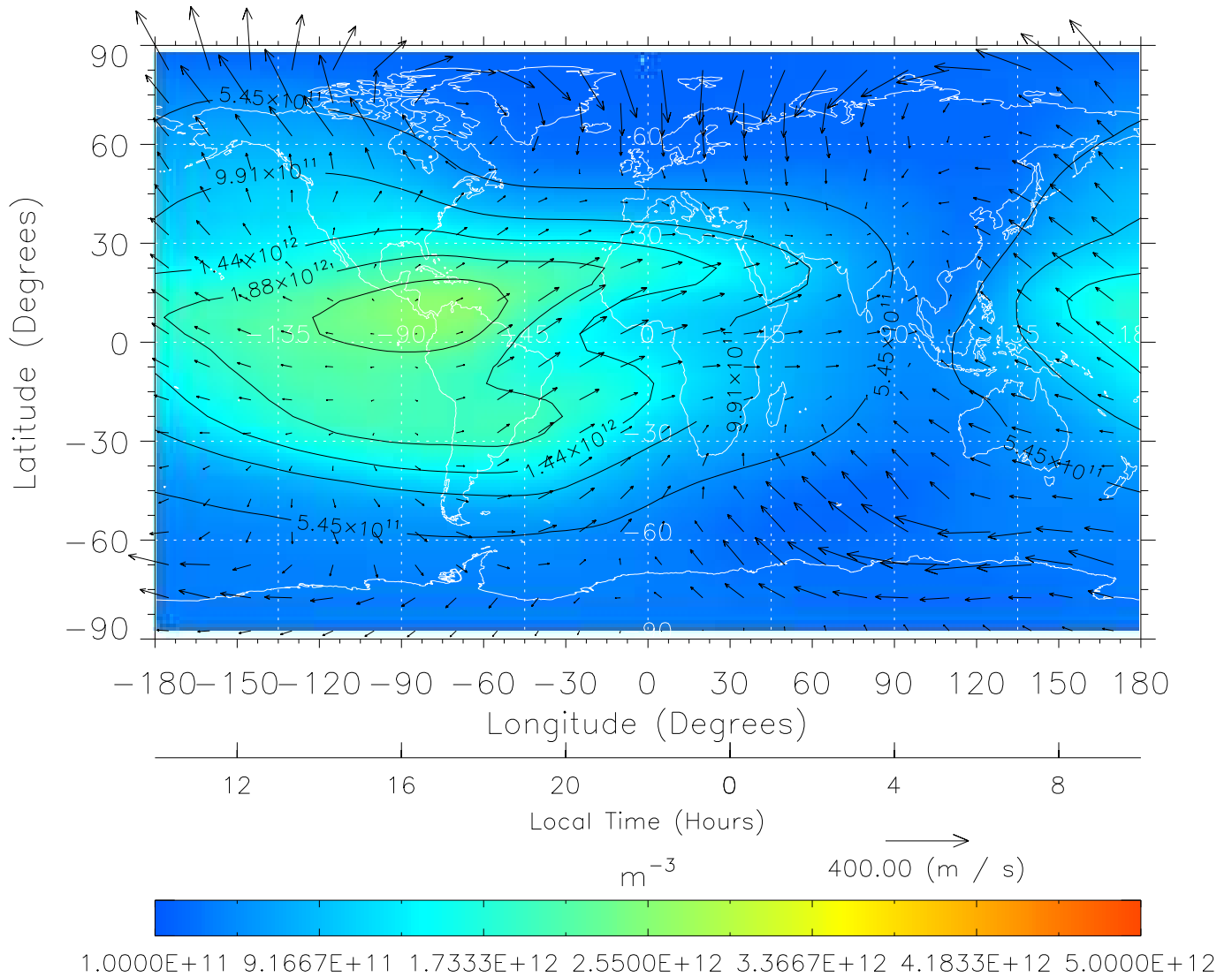
TIME-GCM MAP NmF2 with Neutral Wind vectors ZP = 2.00 UT = 22.00 DOY = 322
