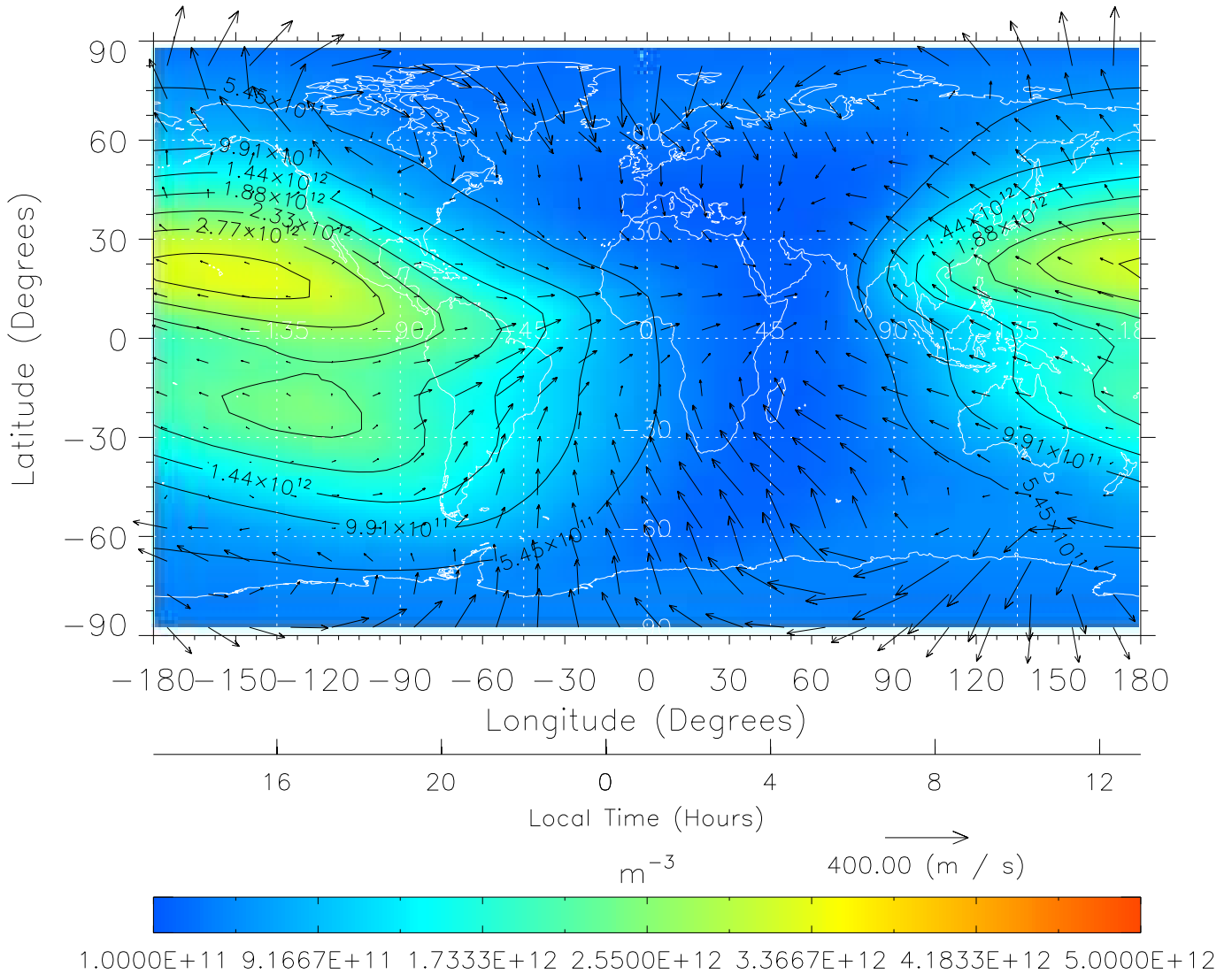
TIME-GCM MAP NmF2 with Neutral Wind vectors ZP = 2.00 UT = 1.00 DOY = 322
