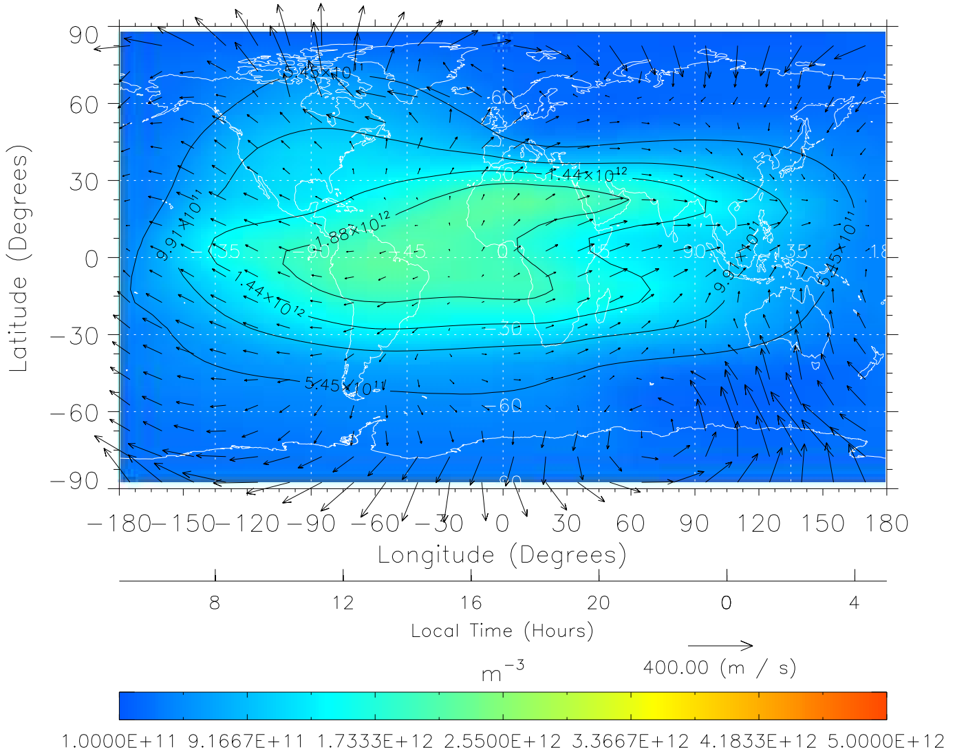
TIME-GCM MAP NmF2 with Neutral Wind vectors ZP = 2.00 UT = 17.00 DOY = 322
