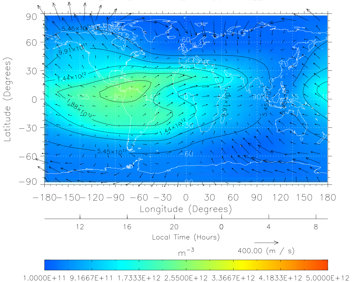
TIME-GCM MAP NmF2 with Neutral Wind vectors ZP = 2.00 UT = 21.00 DOY = 322
