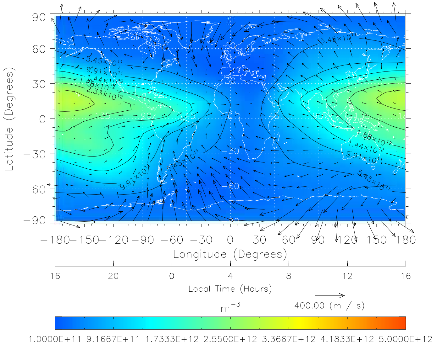
TIME-GCM MAP NmF2 with Neutral Wind vectors ZP = 2.00 UT = 4.00 DOY = 322
