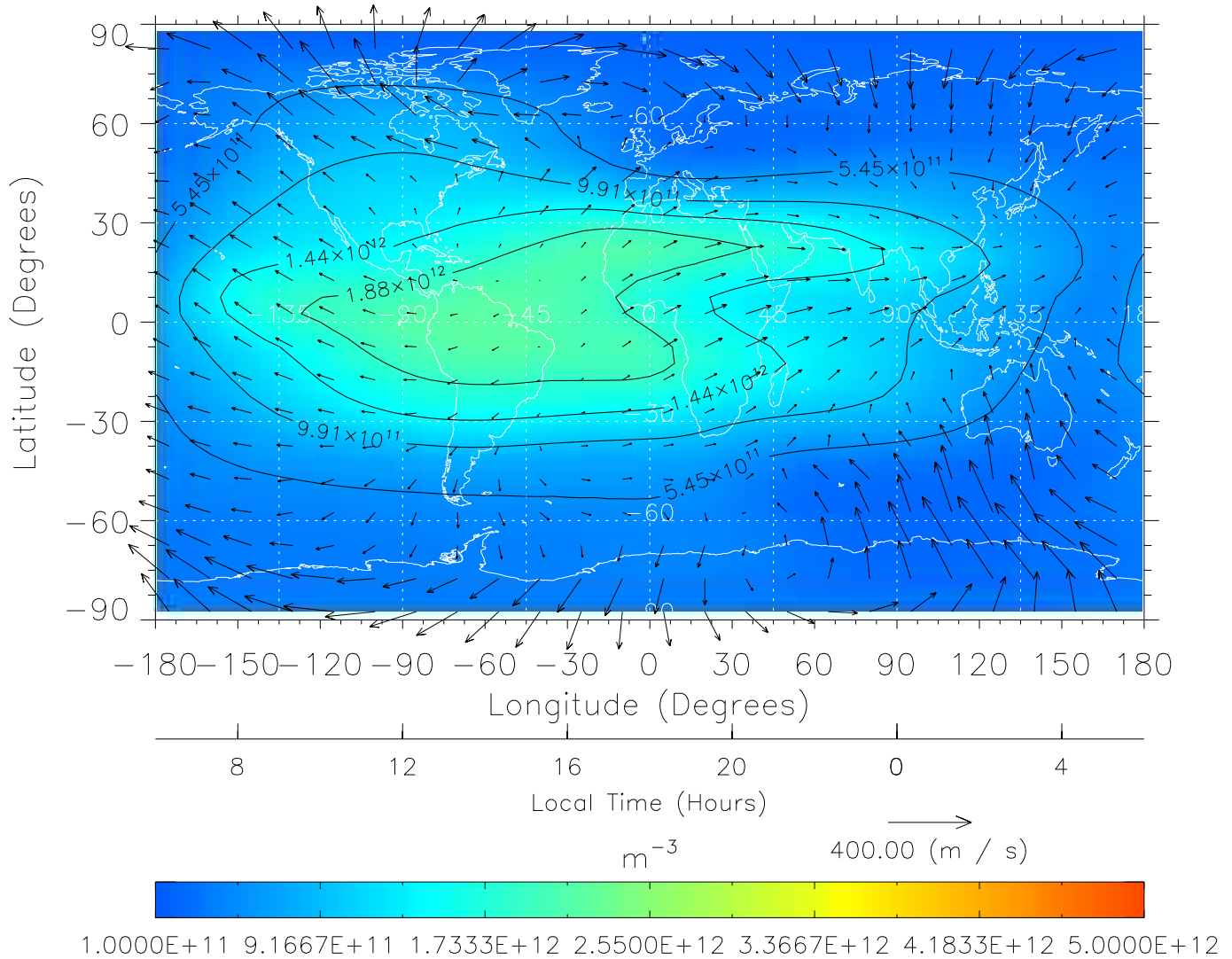
TIME-GCM MAP NmF2 with Neutral Wind vectors ZP = 2.00 UT = 18.00 DOY = 322
