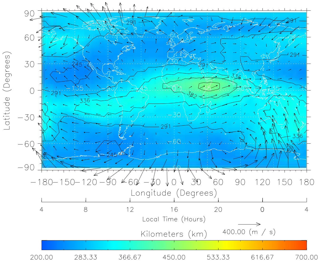
TIME-GCM MAP hmF2 with Neutral Wind vectors ZP = 2.00 UT = 16.00 DOY = 326
