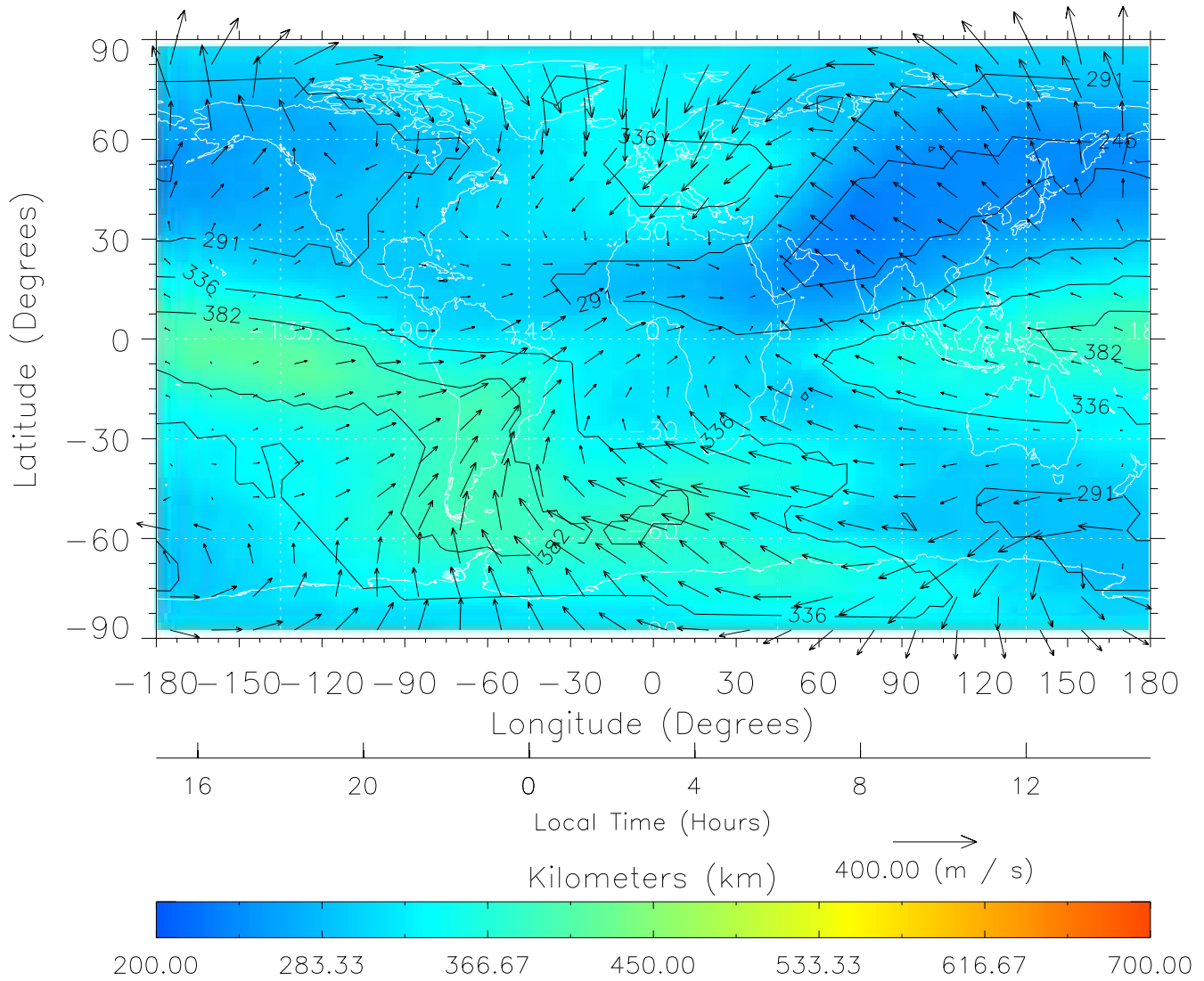
TIME-GCM MAP hmF2 with Neutral Wind vectors ZP = 2.00 UT = 3.00 DOY = 326
