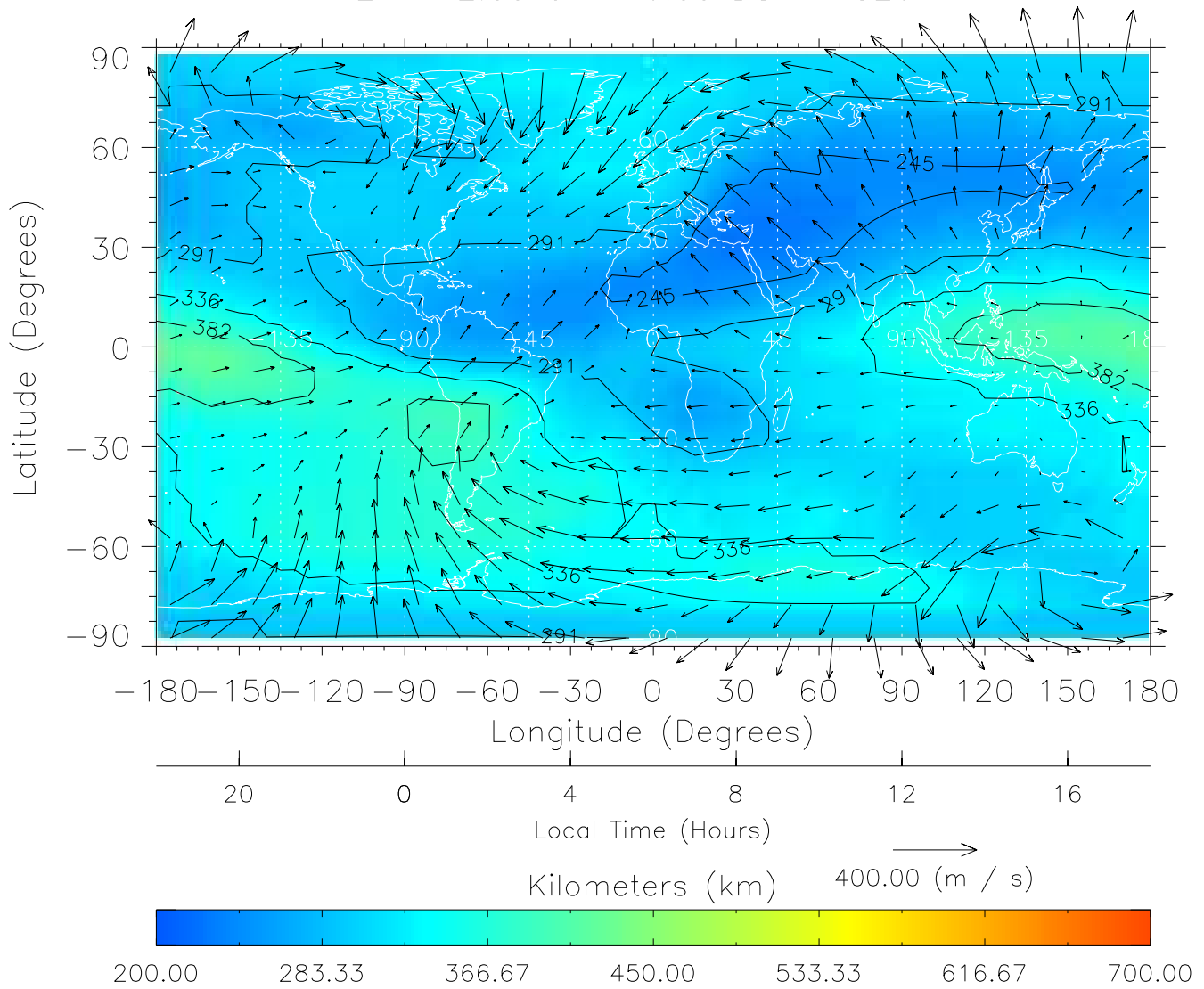
TIME-GCM MAP hmF2 with Neutral Wind vectors ZP = 2.00 UT = 6.00 DOY = 326
