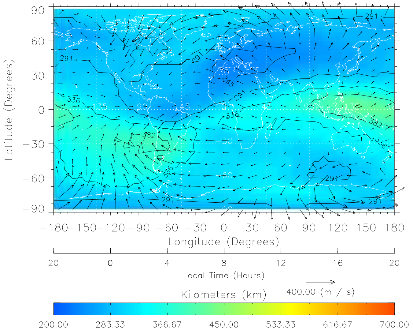
TIME-GCM MAP hmF2 with Neutral Wind vectors ZP = 2.00 UT = 8.00 DOY = 326
