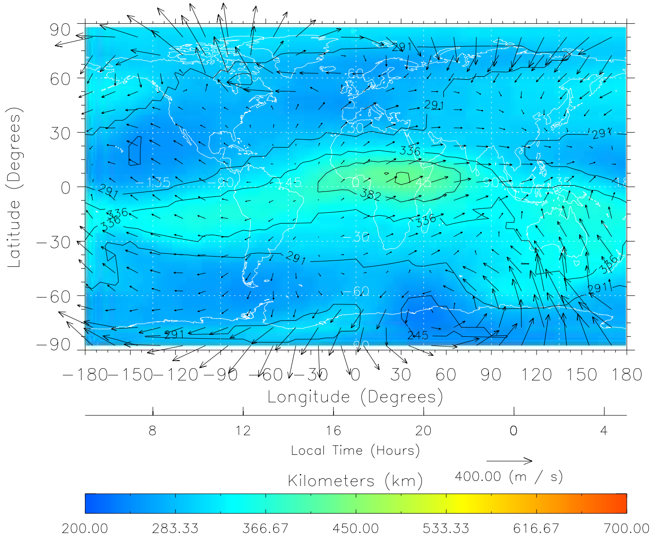
TIME-GCM MAP hmF2 with Neutral Wind vectors ZP = 2.00 UT = 17.00 DOY = 326
