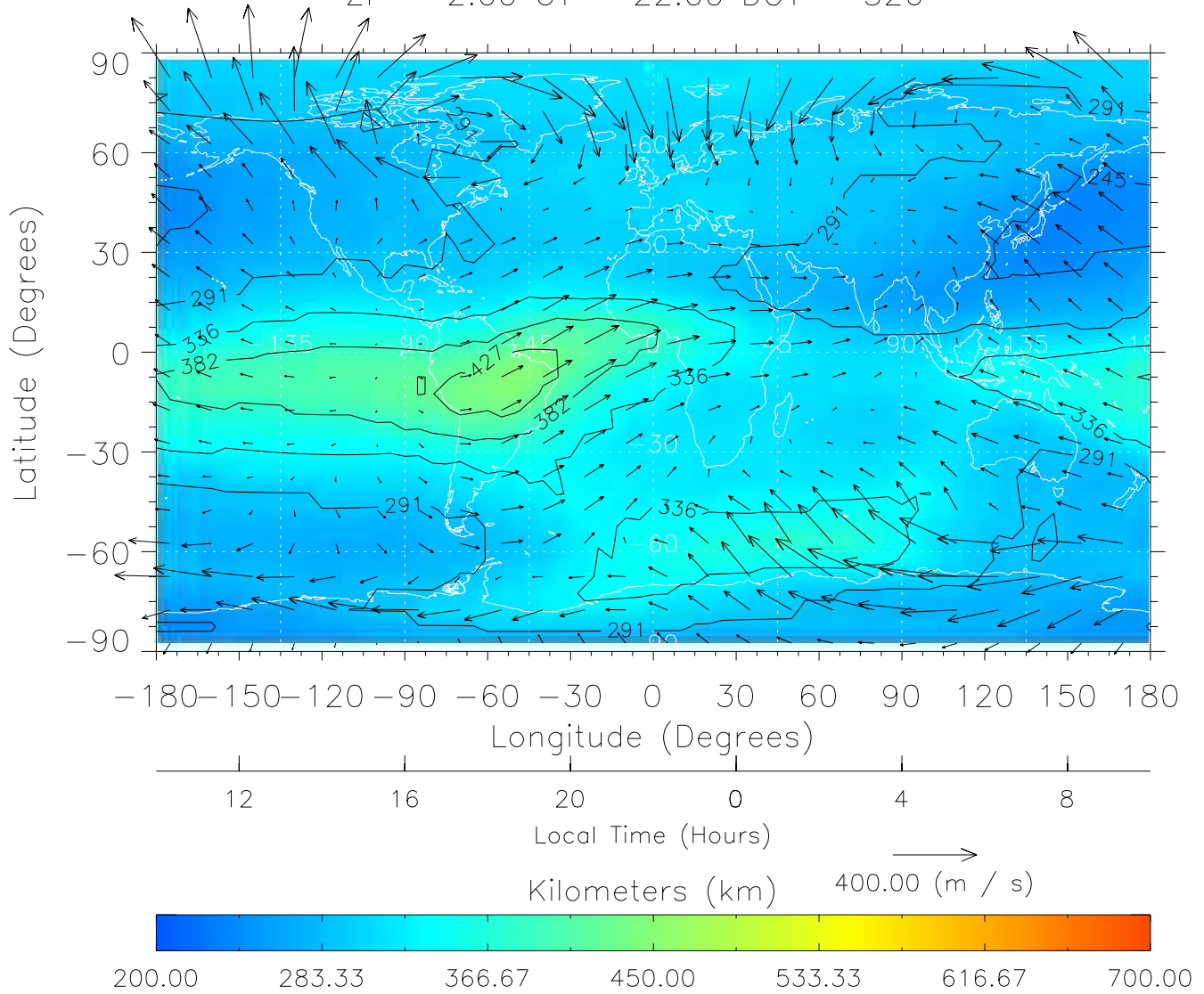
TIME-GCM MAP hmF2 with Neutral Wind vectors ZP = 2.00 UT = 22.00 DOY = 326
