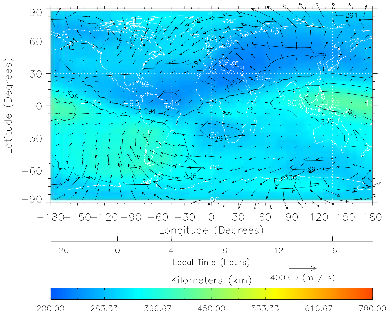
TIME-GCM MAP hmF2 with Neutral Wind vectors ZP = 2.00 UT = 7.00 DOY = 326
