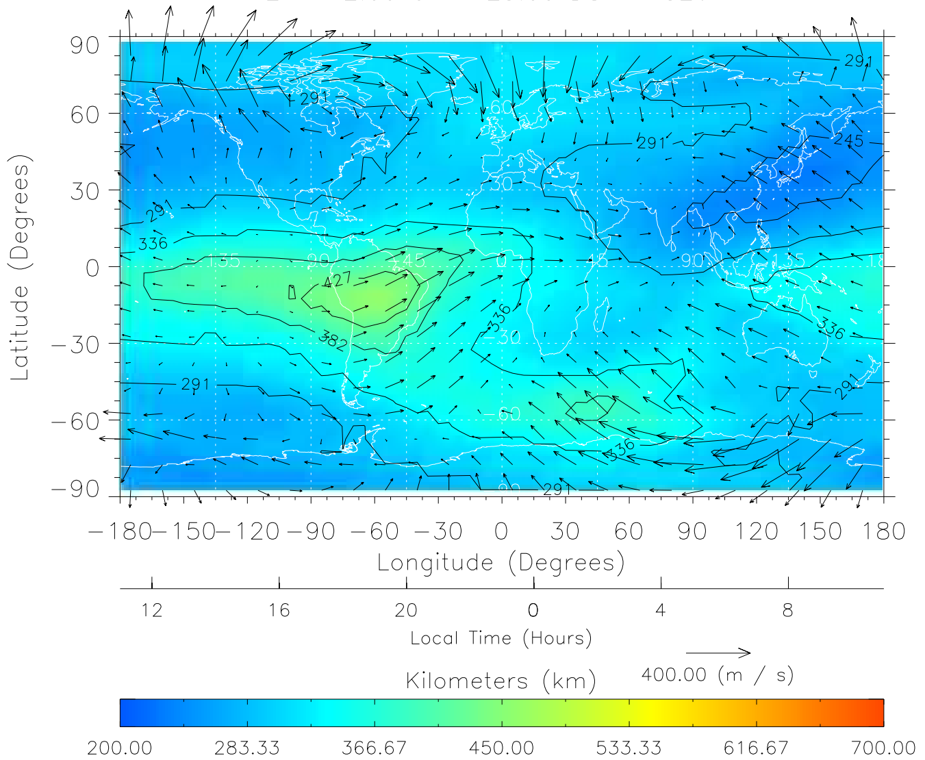
TIME-GCM MAP hmF2 with Neutral Wind vectors ZP = 2.00 UT = 23.00 DOY = 326
