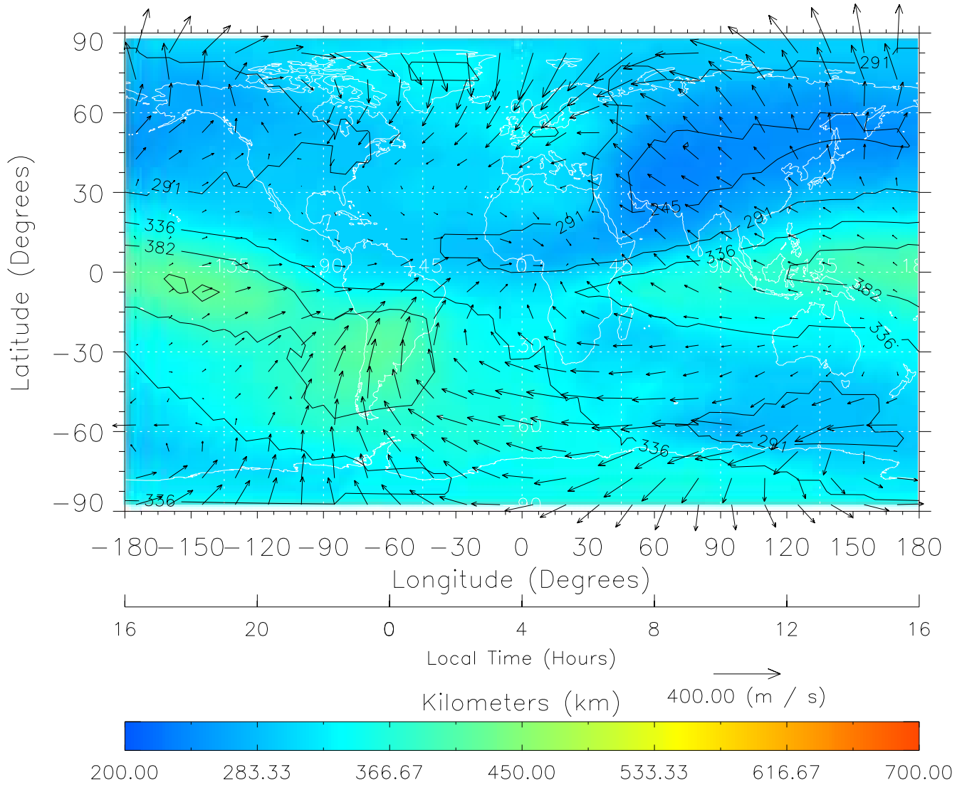
TIME-GCM MAP hmF2 with Neutral Wind vectors ZP = 2.00 UT = 4.00 DOY = 326
