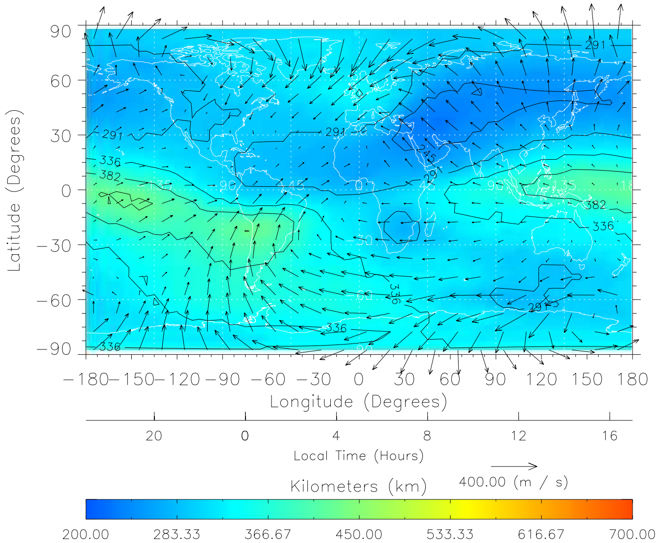
TIME-GCM MAP hmF2 with Neutral Wind vectors ZP = 2.00 UT = 5.00 DOY = 326
