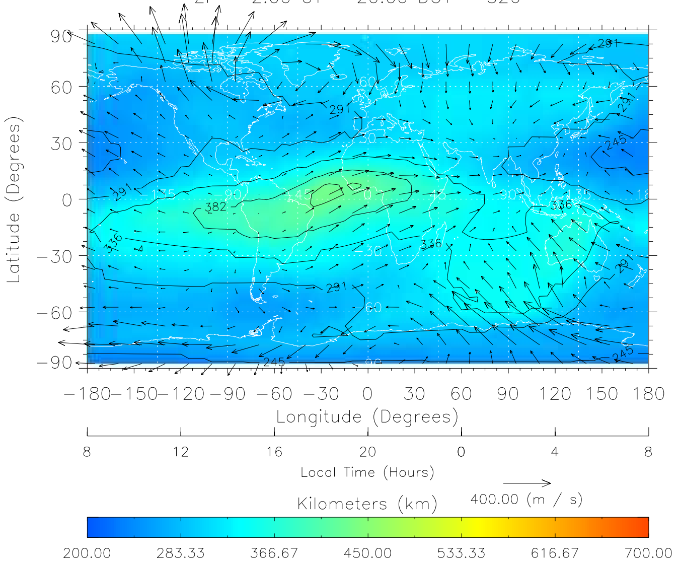
TIME-GCM MAP hmF2 with Neutral Wind vectors ZP = 2.00 UT = 20.00 DOY = 326
