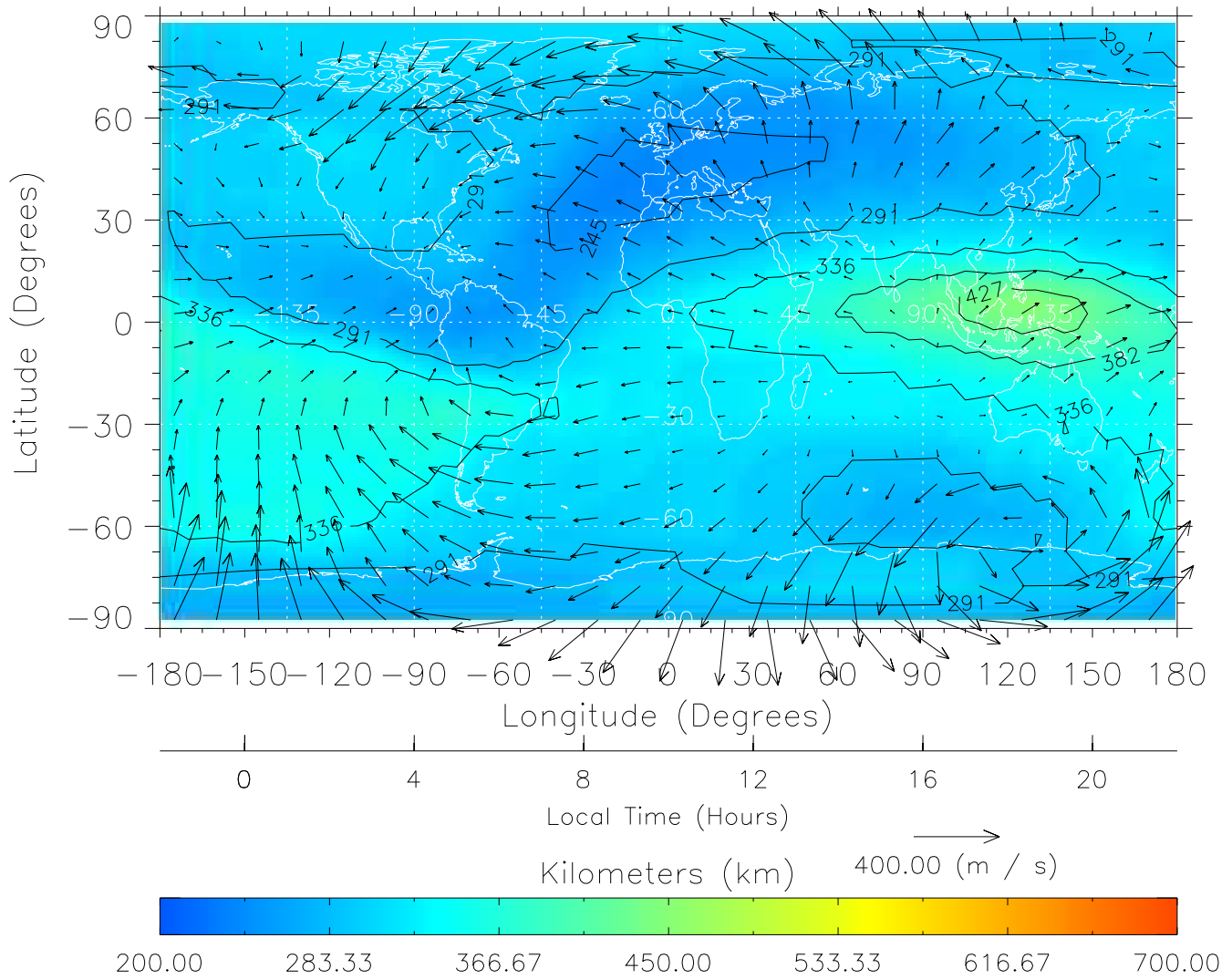
TIME-GCM MAP hmF2 with Neutral Wind vectors ZP = 2.00 UT = 10.00 DOY = 326
