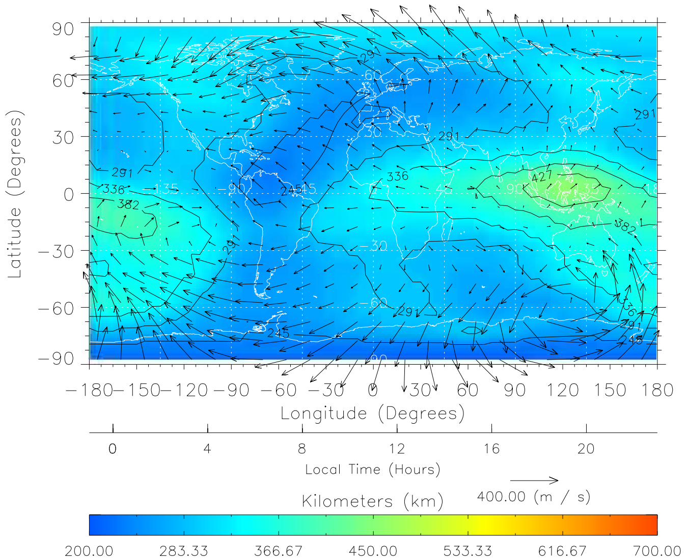
TIME-GCM MAP hmF2 with Neutral Wind vectors ZP = 2.00 UT = 11.00 DOY = 325
