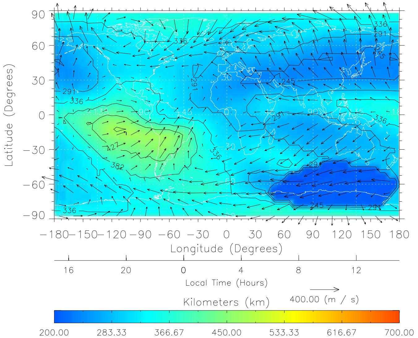
TIME-GCM MAP hmF2 with Neutral Wind vectors ZP = 2.00 UT = 3.00 DOY = 325
