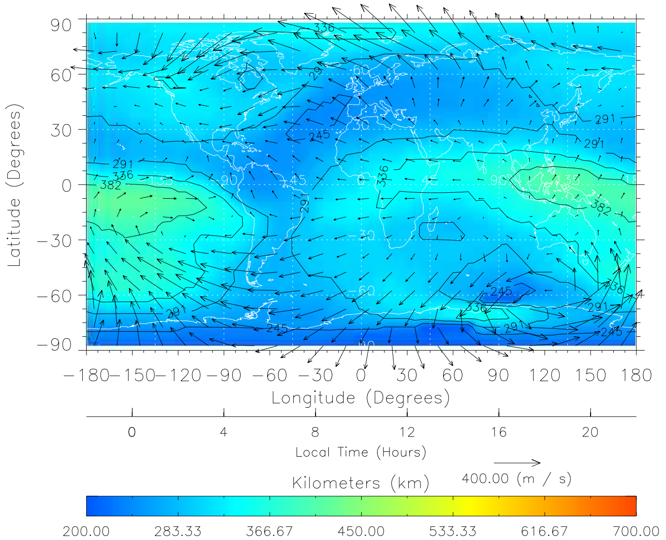
TIME-GCM MAP hmF2 with Neutral Wind vectors ZP = 2.00 UT = 10.00 DOY = 325
