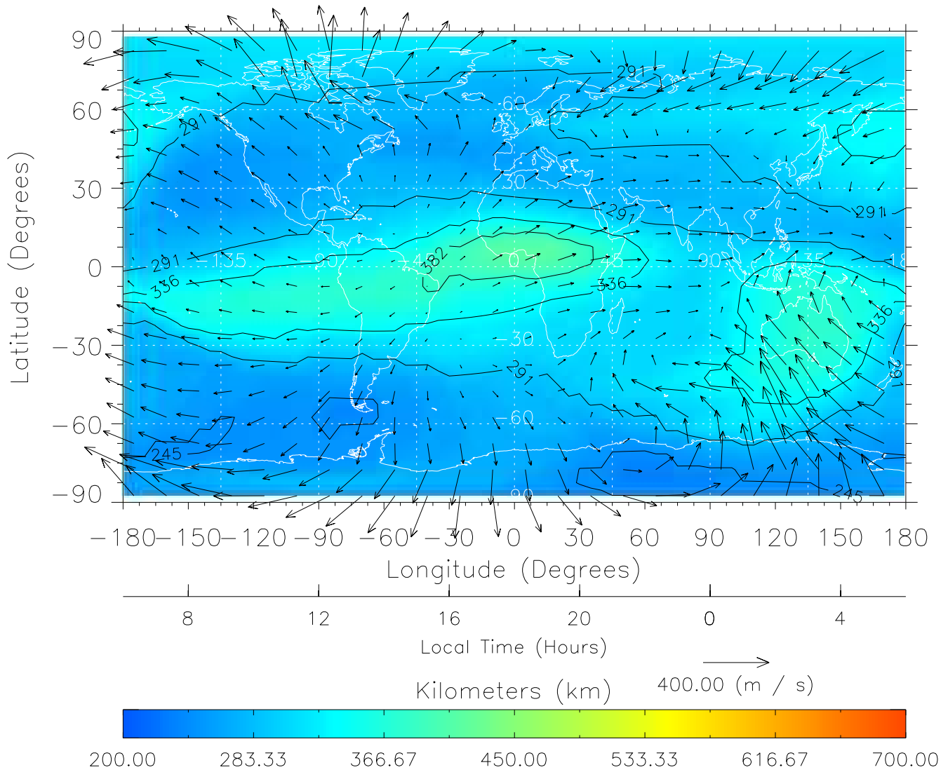
TIME-GCM MAP hmF2 with Neutral Wind vectors ZP = 2.00 UT = 18.00 DOY = 325
