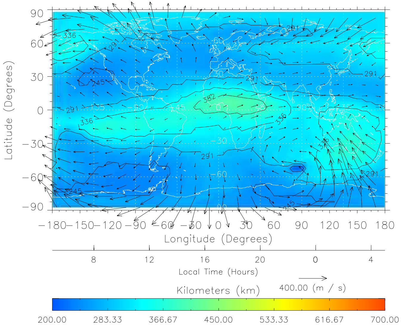
TIME-GCM MAP hmF2 with Neutral Wind vectors ZP = 2.00 UT = 17.00 DOY = 325
