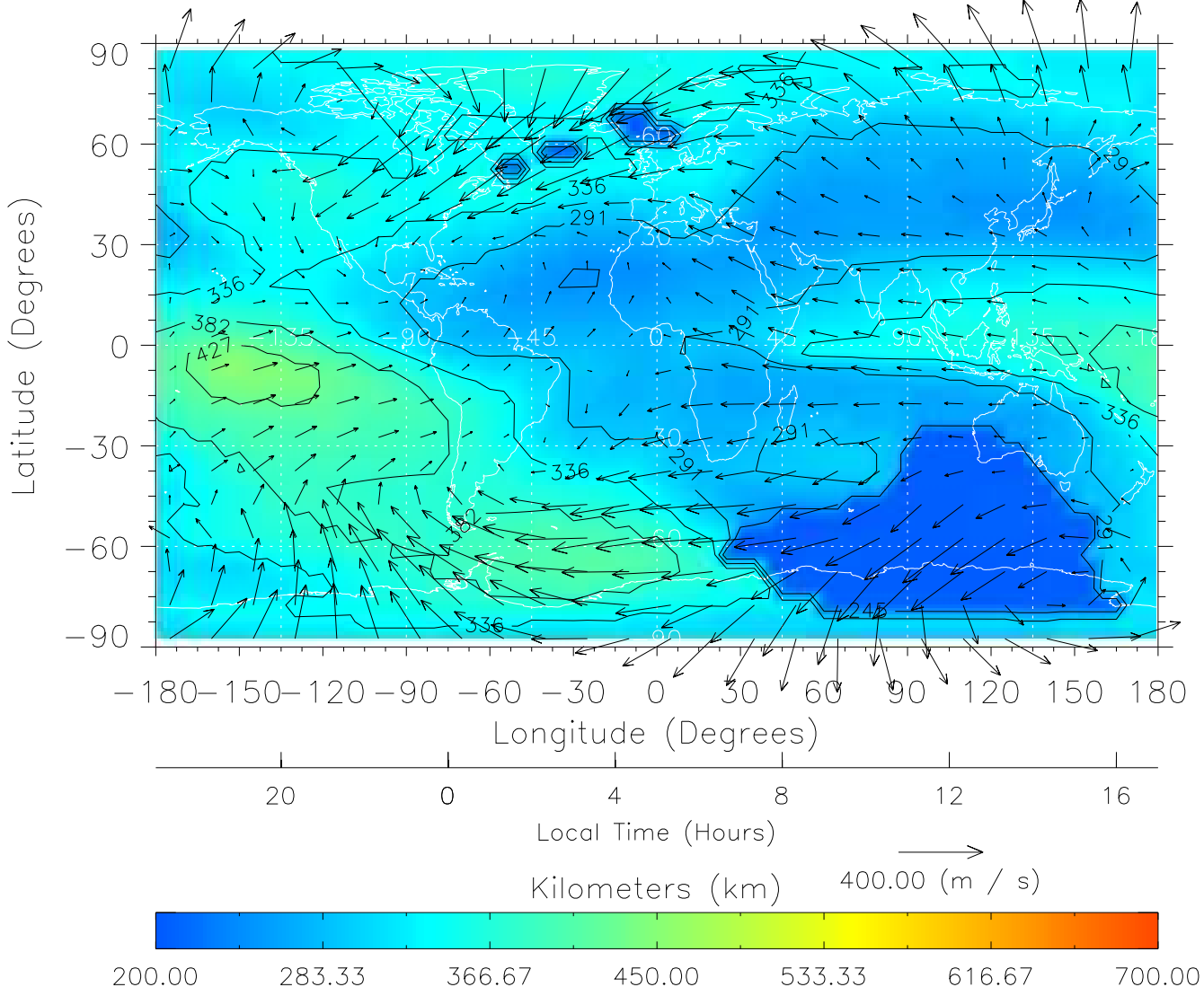
TIME-GCM MAP hmF2 with Neutral Wind vectors ZP = 2.00 UT = 5.00 DOY = 325
