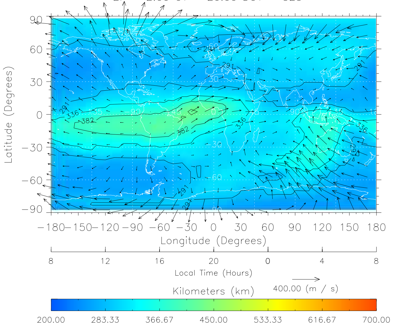
TIME-GCM MAP hmF2 with Neutral Wind vectors ZP = 2.00 UT = 20.00 DOY = 325
