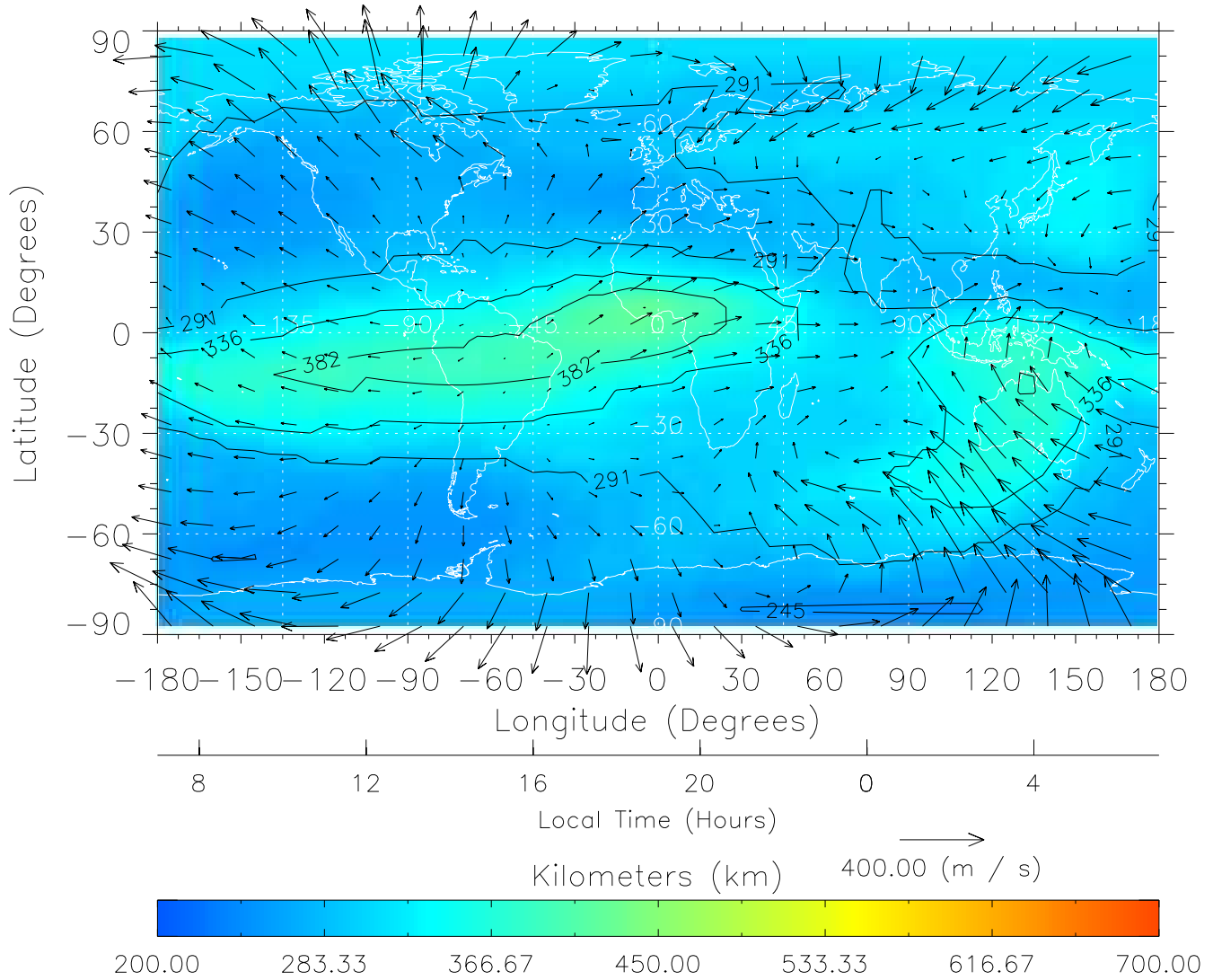
TIME-GCM MAP hmF2 with Neutral Wind vectors ZP = 2.00 UT = 19.00 DOY = 325
