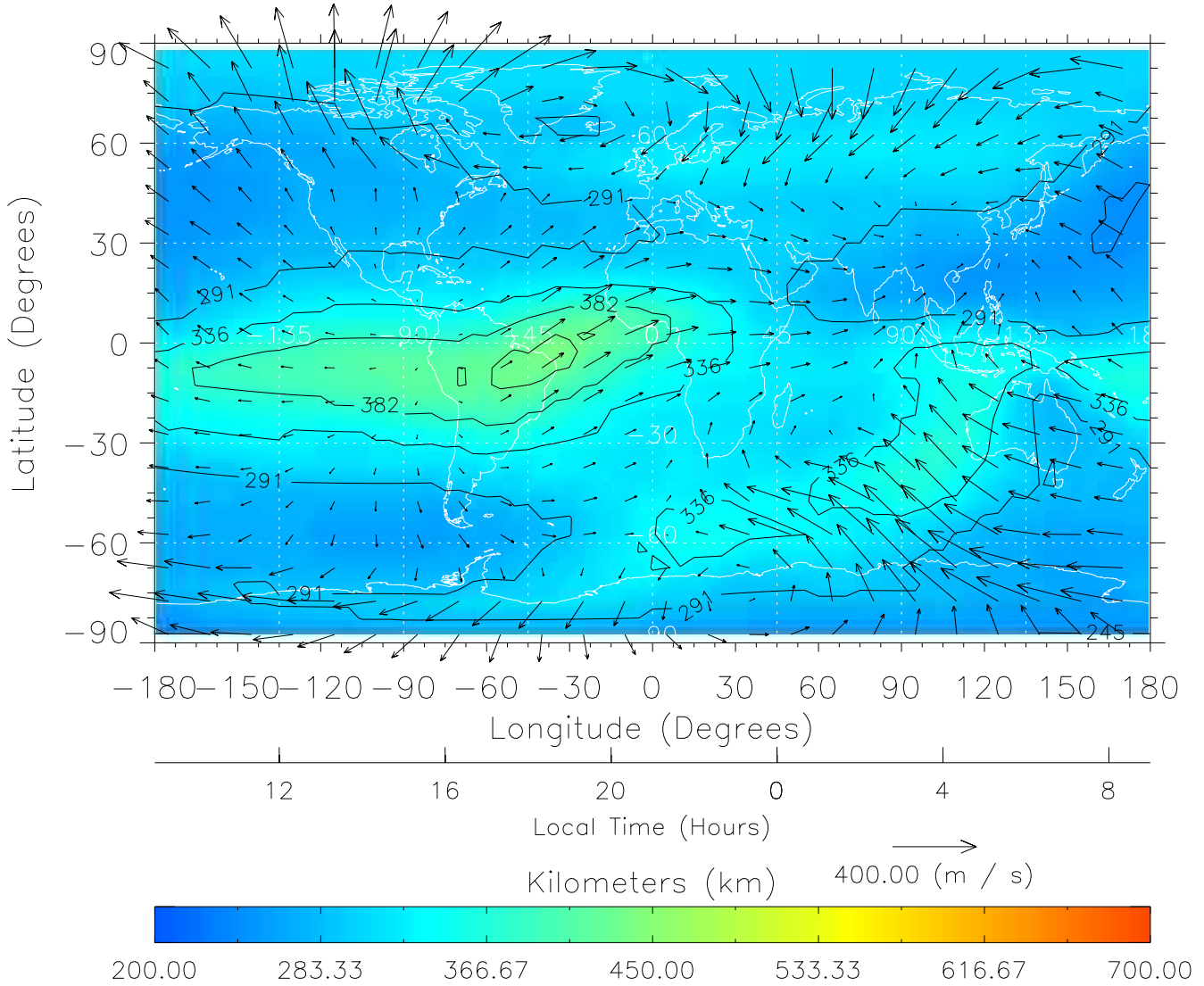
TIME-GCM MAP hmF2 with Neutral Wind vectors ZP = 2.00 UT = 21.00 DOY = 325
