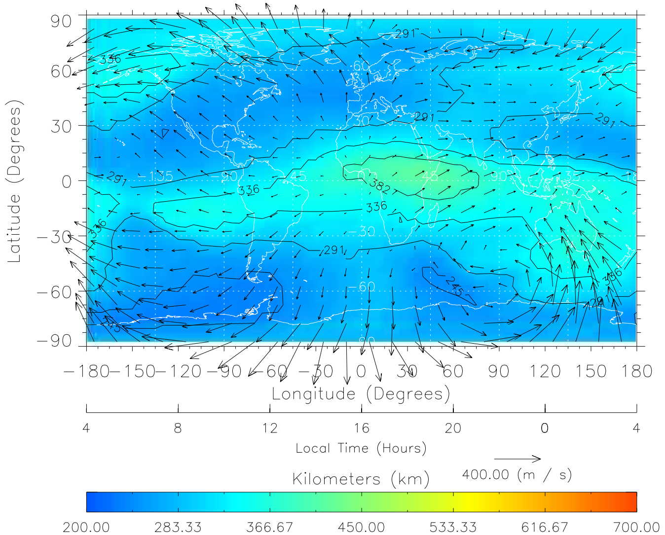
TIME-GCM MAP hmF2 with Neutral Wind vectors ZP = 2.00 UT = 16.00 DOY = 325
