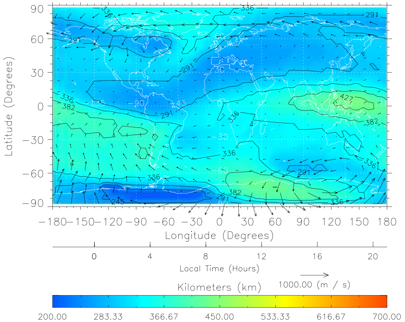
TIME-GCM MAP hmF2 with Neutral Wind vectors ZP = 2.00 UT = 9.00 DOY = 324
