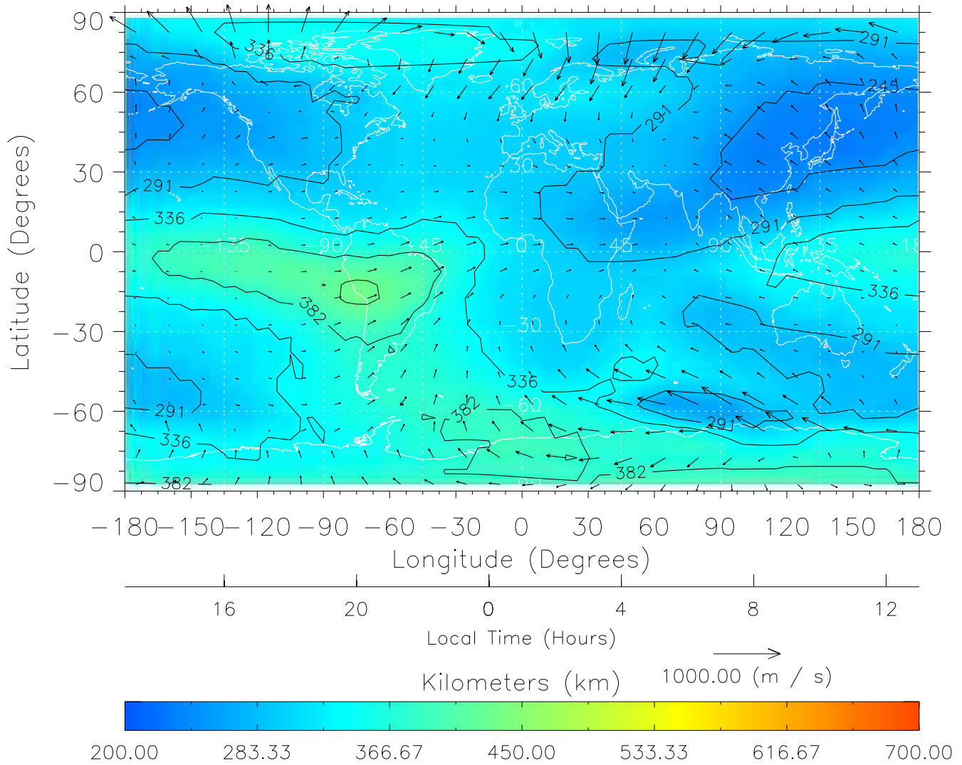
TIME-GCM MAP hmF2 with Neutral Wind vectors ZP = 2.00 UT = 1.00 DOY = 324
