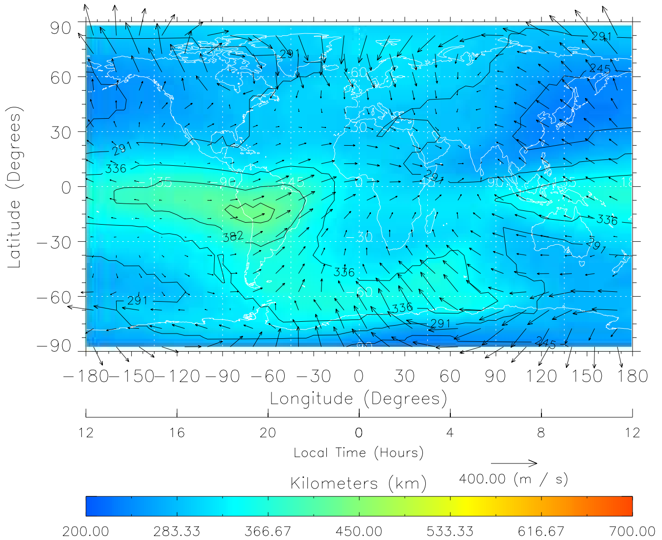
TIME-GCM MAP hmF2 with Neutral Wind vectors ZP = 2.00 UT = 0.00 DOY = 323
