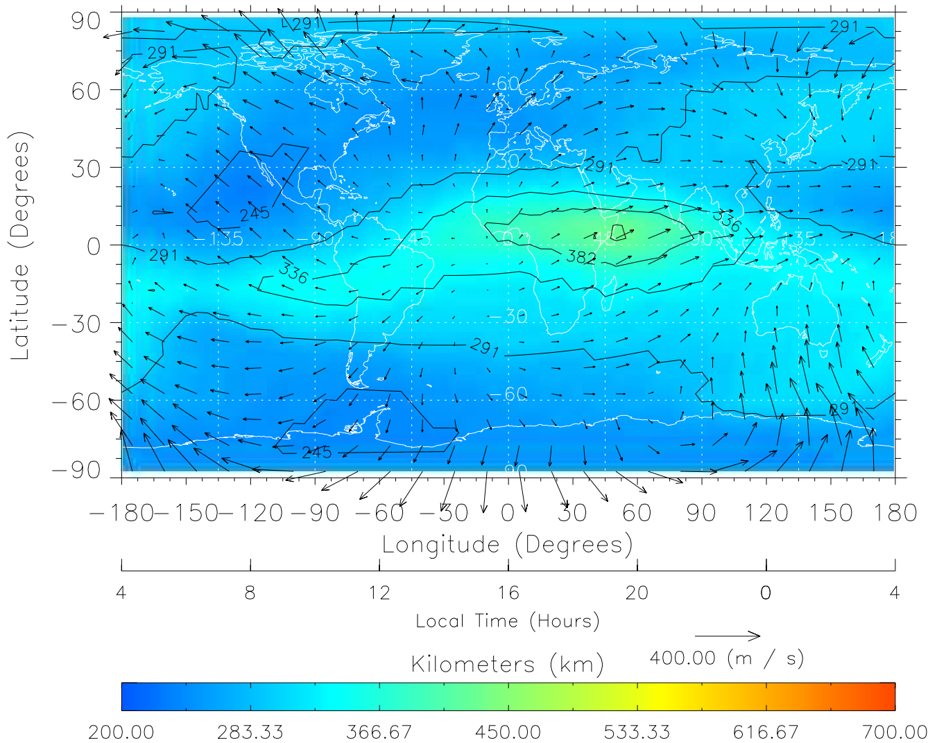
TIME-GCM MAP hmF2 with Neutral Wind vectors ZP = 2.00 UT = 16.00 DOY = 323
