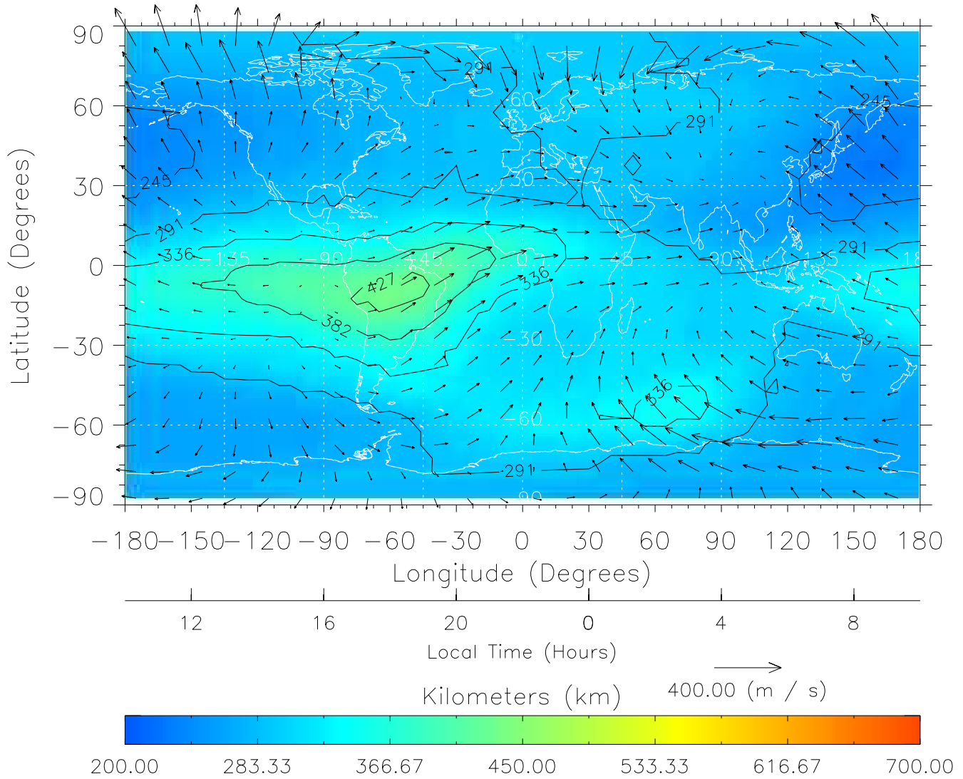
TIME-GCM MAP hmF2 with Neutral Wind vectors ZP = 2.00 UT = 22.00 DOY = 323
