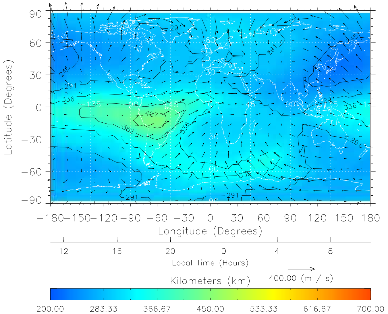
TIME-GCM MAP hmF2 with Neutral Wind vectors ZP = 2.00 UT = 23.00 DOY = 323
