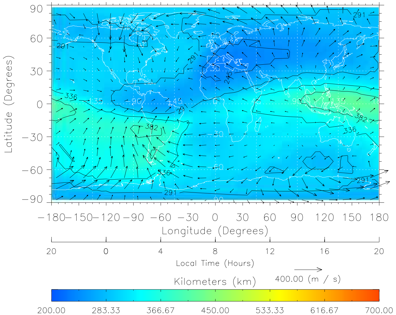
TIME-GCM MAP hmF2 with Neutral Wind vectors ZP = 2.00 UT = 8.00 DOY = 323
