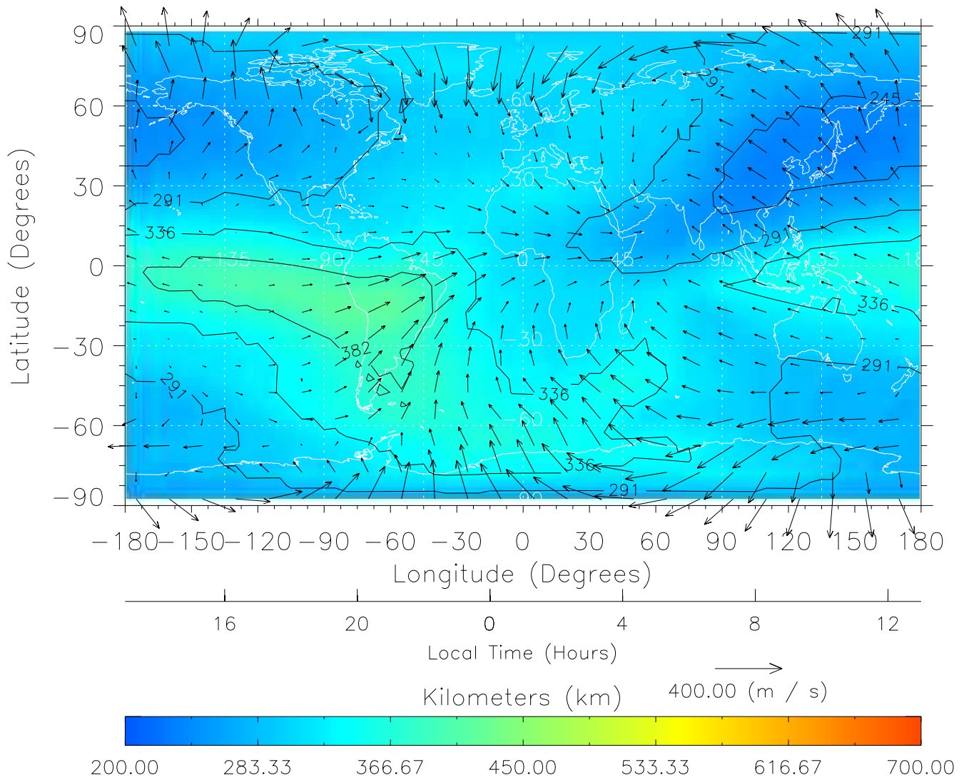
TIME-GCM MAP hmF2 with Neutral Wind vectors ZP = 2.00 UT = 1.00 DOY = 323
