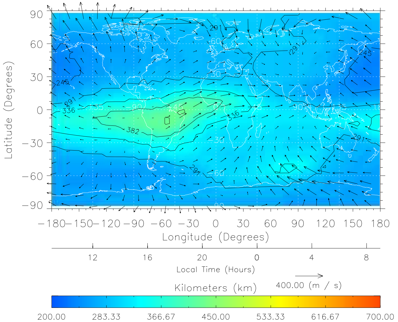
TIME-GCM MAP hmF2 with Neutral Wind vectors ZP = 2.00 UT = 21.00 DOY = 323
