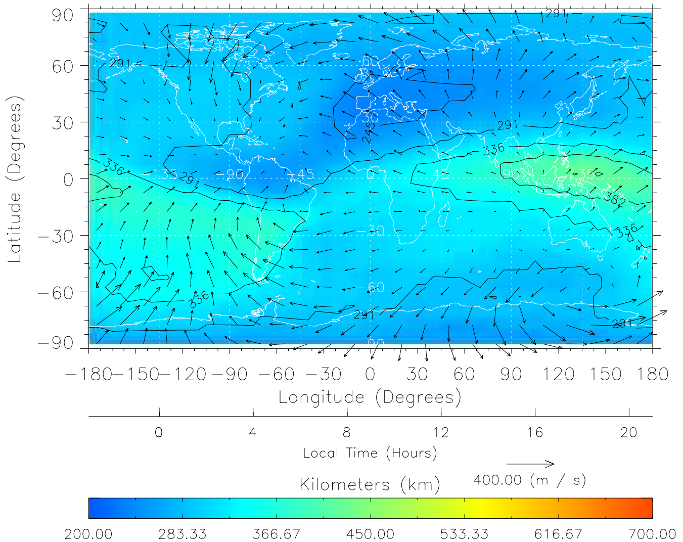
TIME-GCM MAP hmF2 with Neutral Wind vectors ZP = 2.00 UT = 9.00 DOY = 323
