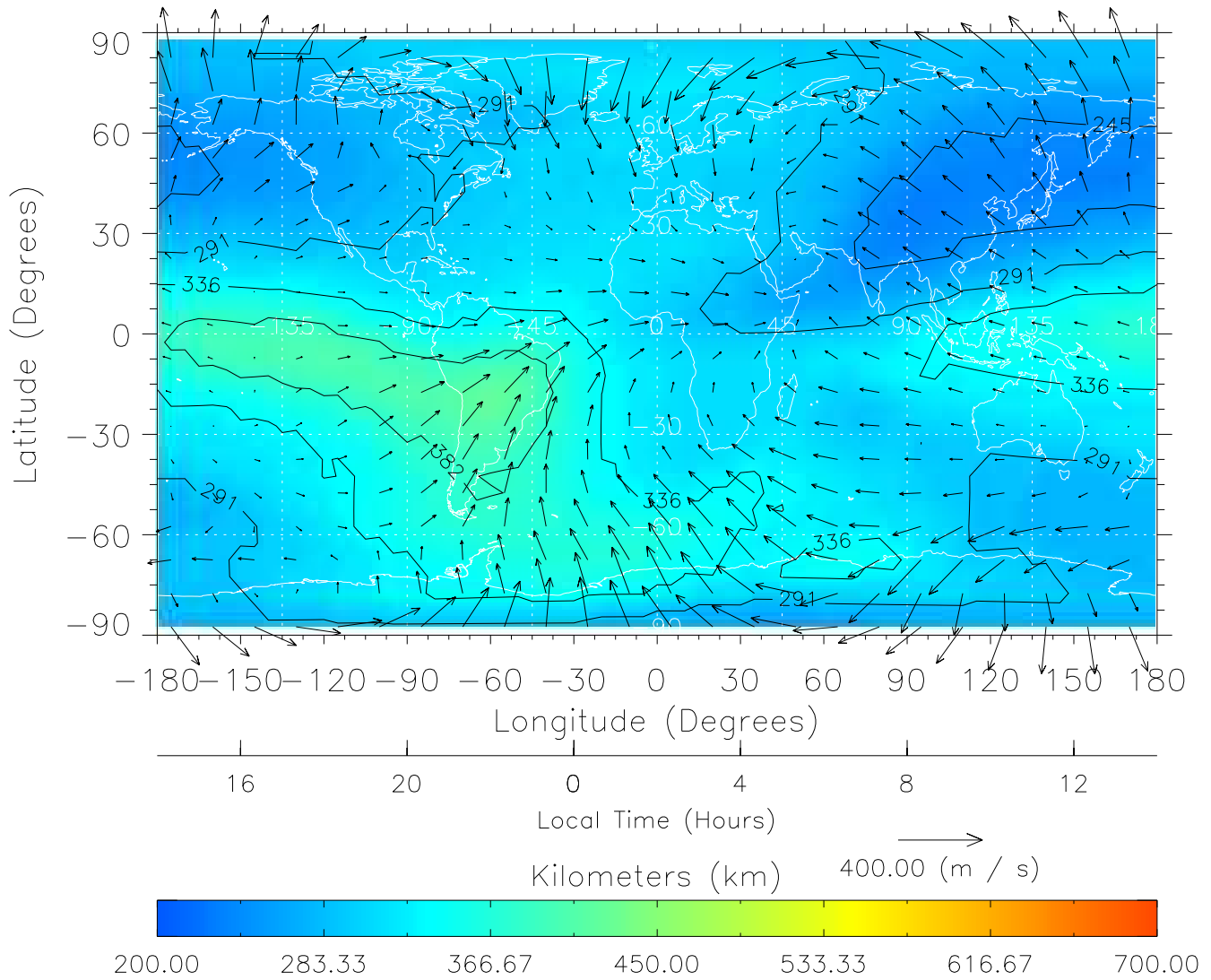
TIME-GCM MAP hmF2 with Neutral Wind vectors ZP = 2.00 UT = 2.00 DOY = 323
