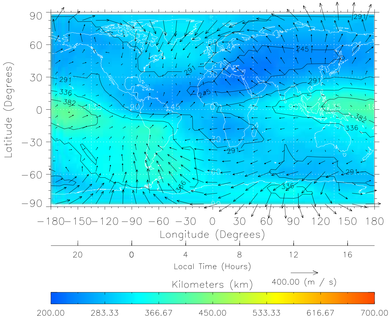
TIME-GCM MAP hmF2 with Neutral Wind vectors ZP = 2.00 UT = 6.00 DOY = 322
