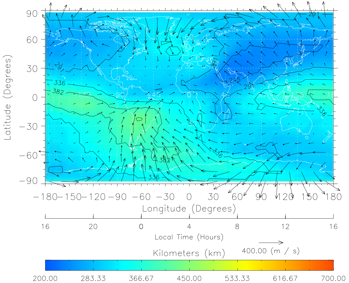
TIME-GCM MAP hmF2 with Neutral Wind vectors ZP = 2.00 UT = 4.00 DOY = 322
