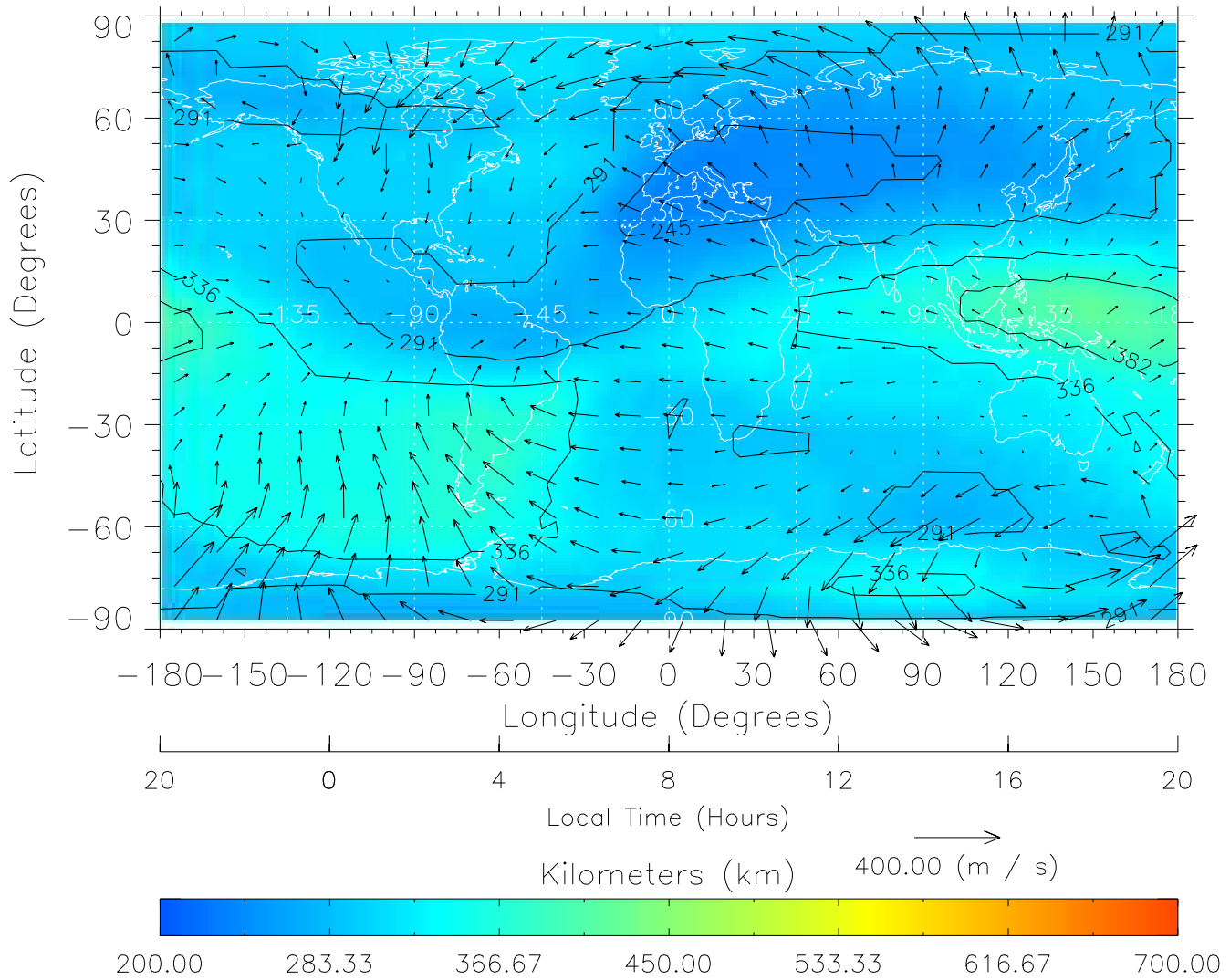
TIME-GCM MAP hmF2 with Neutral Wind vectors ZP = 2.00 UT = 8.00 DOY = 322
