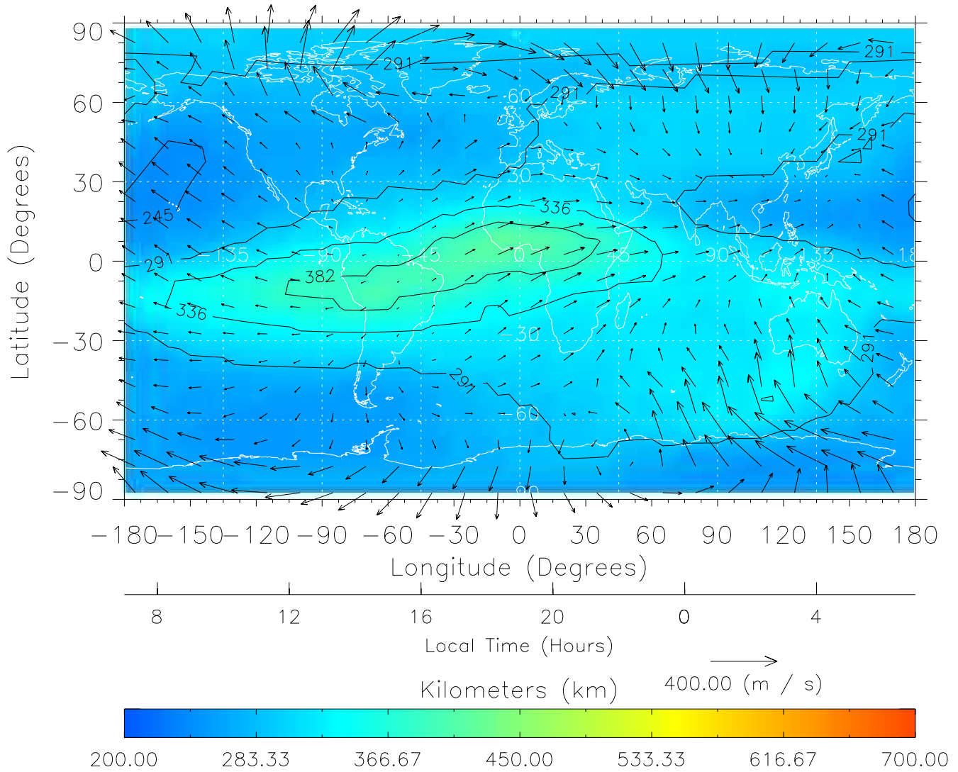
TIME-GCM MAP hmF2 with Neutral Wind vectors ZP = 2.00 UT = 19.00 DOY = 322
