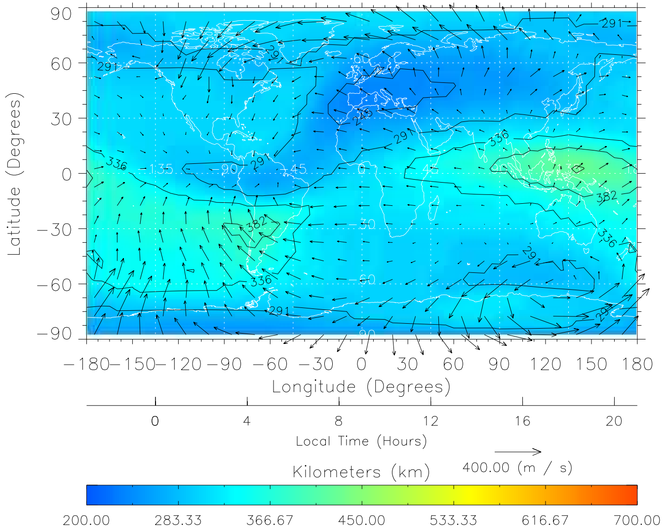
TIME-GCM MAP hmF2 with Neutral Wind vectors ZP = 2.00 UT = 9.00 DOY = 322
