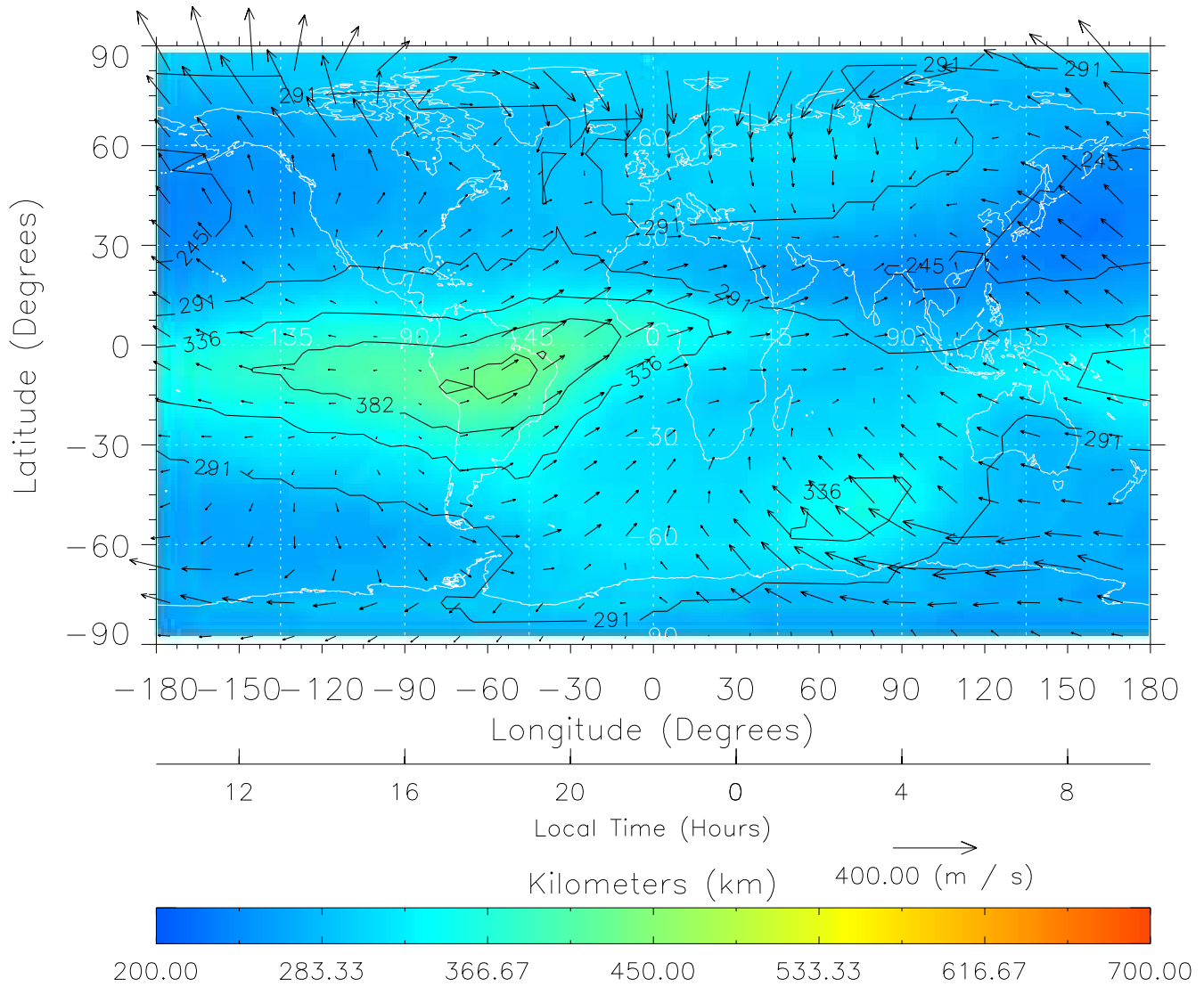
TIME-GCM MAP hmF2 with Neutral Wind vectors ZP = 2.00 UT = 22.00 DOY = 322
