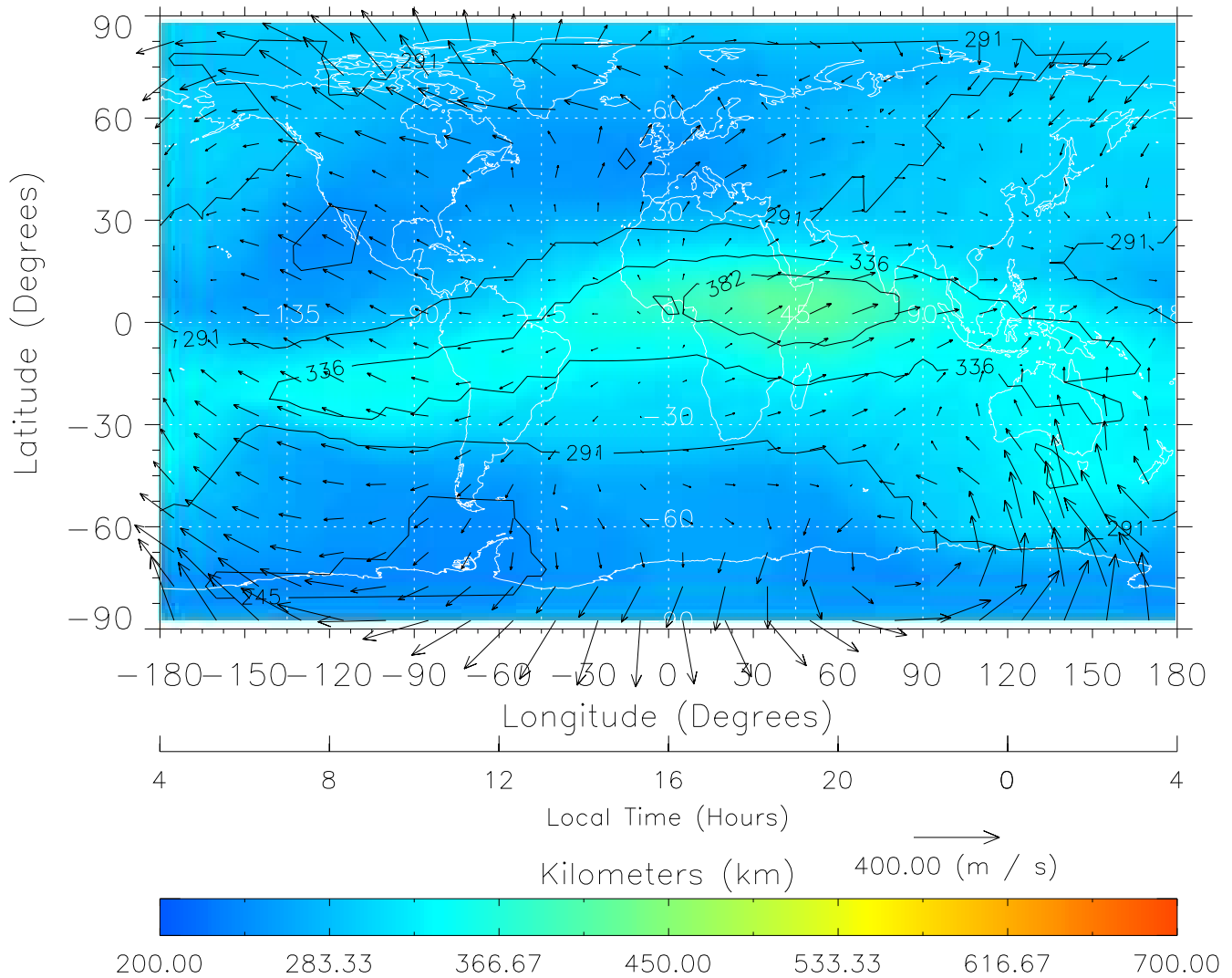
TIME-GCM MAP hmF2 with Neutral Wind vectors ZP = 2.00 UT = 16.00 DOY = 322
