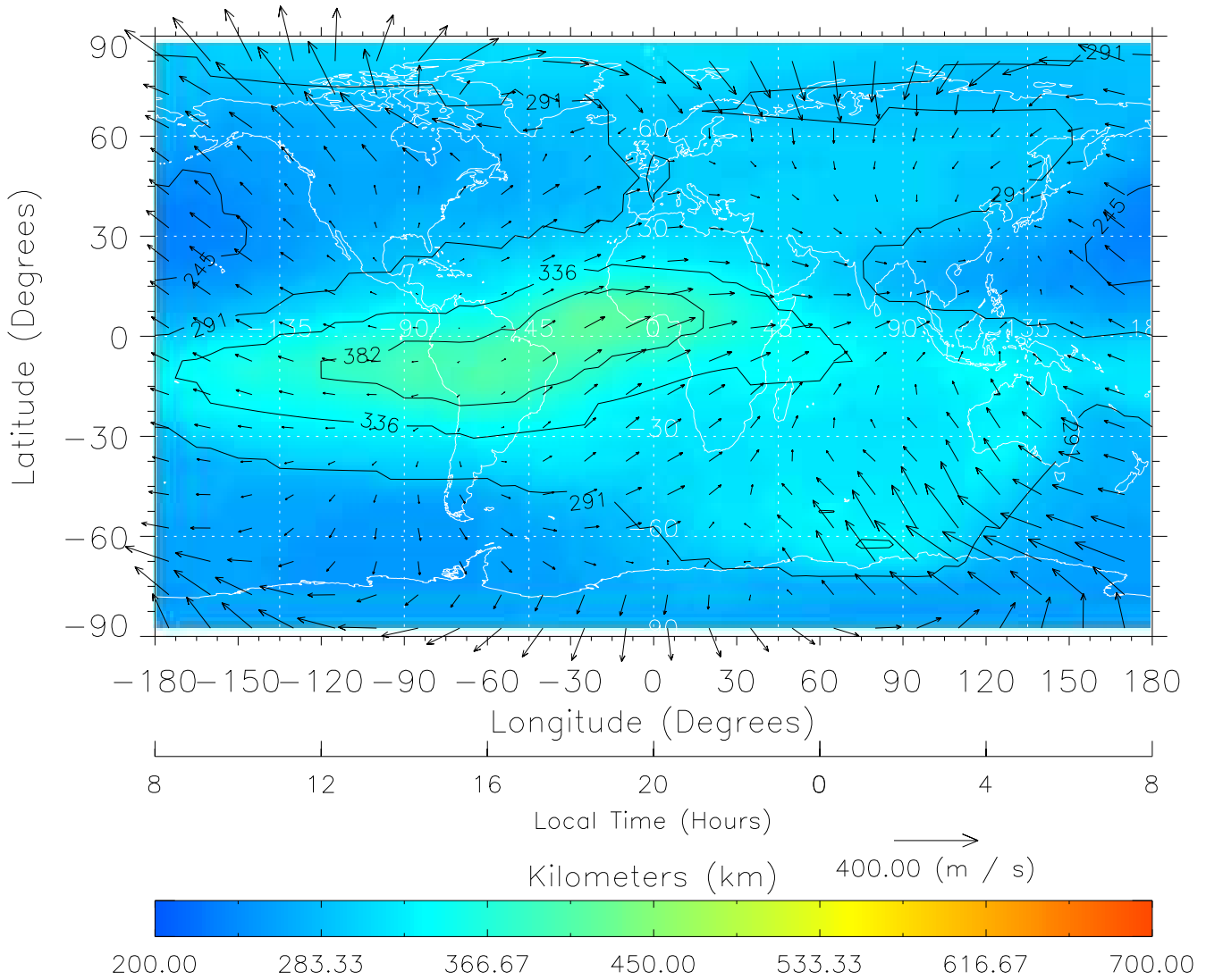
TIME-GCM MAP hmF2 with Neutral Wind vectors ZP = 2.00 UT = 20.00 DOY = 322
