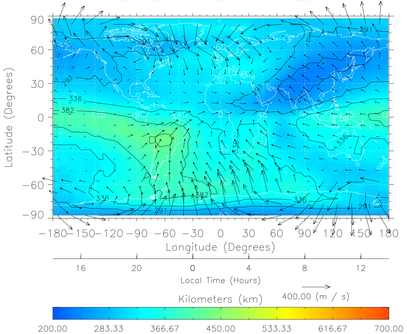
TIME-GCM MAP hmF2 with Neutral Wind vectors ZP = 2.00 UT = 2.00 DOY = 322
