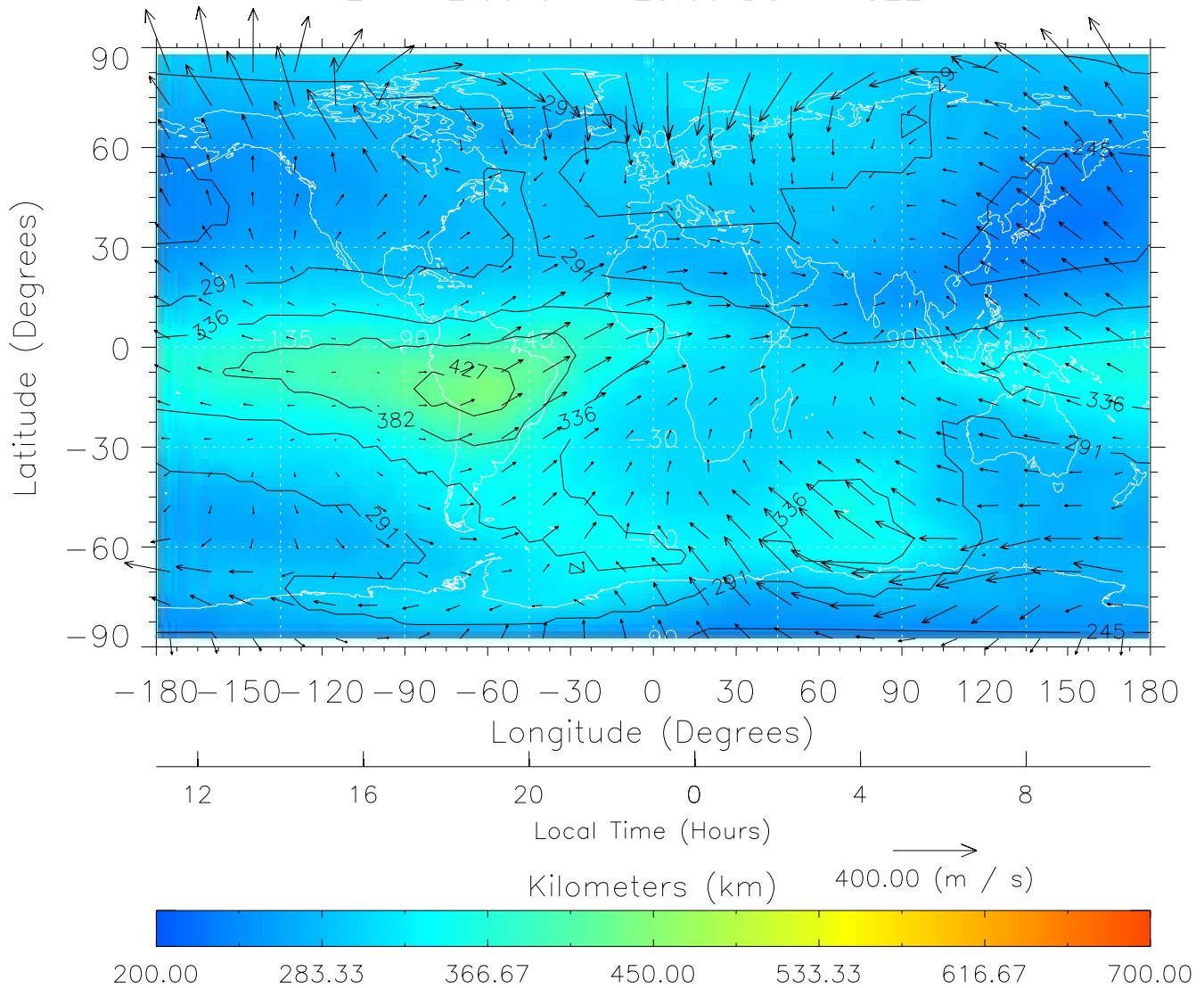
TIME-GCM MAP hmF2 with Neutral Wind vectors ZP = 2.00 UT = 23.00 DOY = 322
