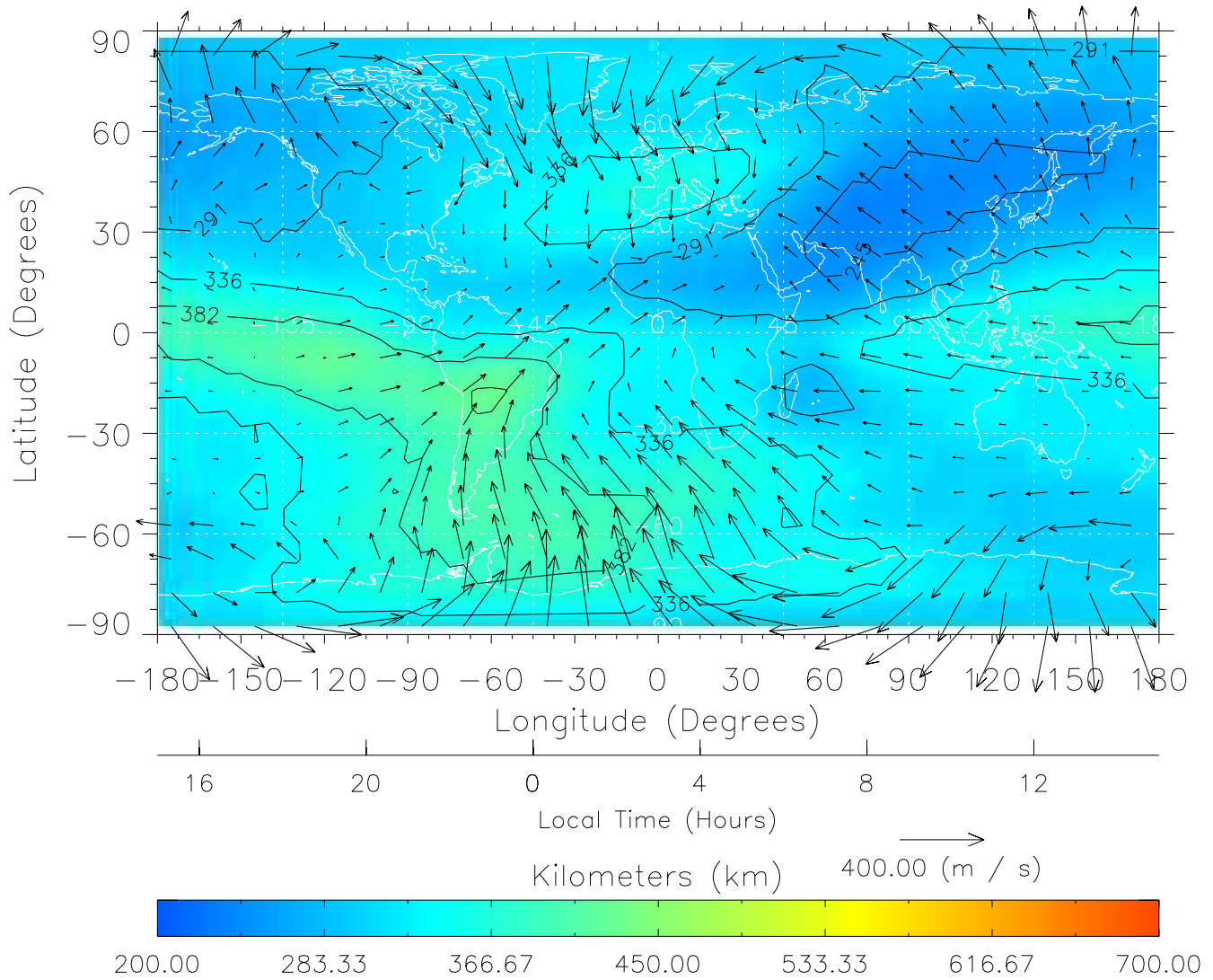
TIME-GCM MAP hmF2 with Neutral Wind vectors ZP = 2.00 UT = 3.00 DOY = 322
