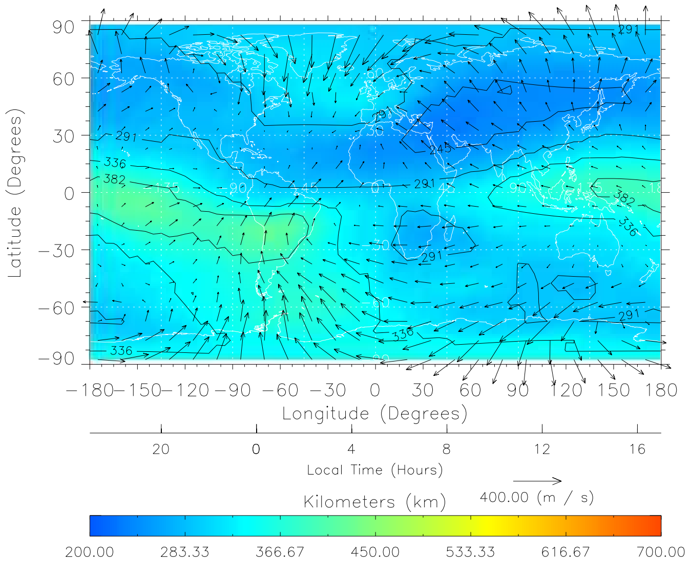
TIME-GCM MAP hmF2 with Neutral Wind vectors ZP = 2.00 UT = 5.00 DOY = 322
