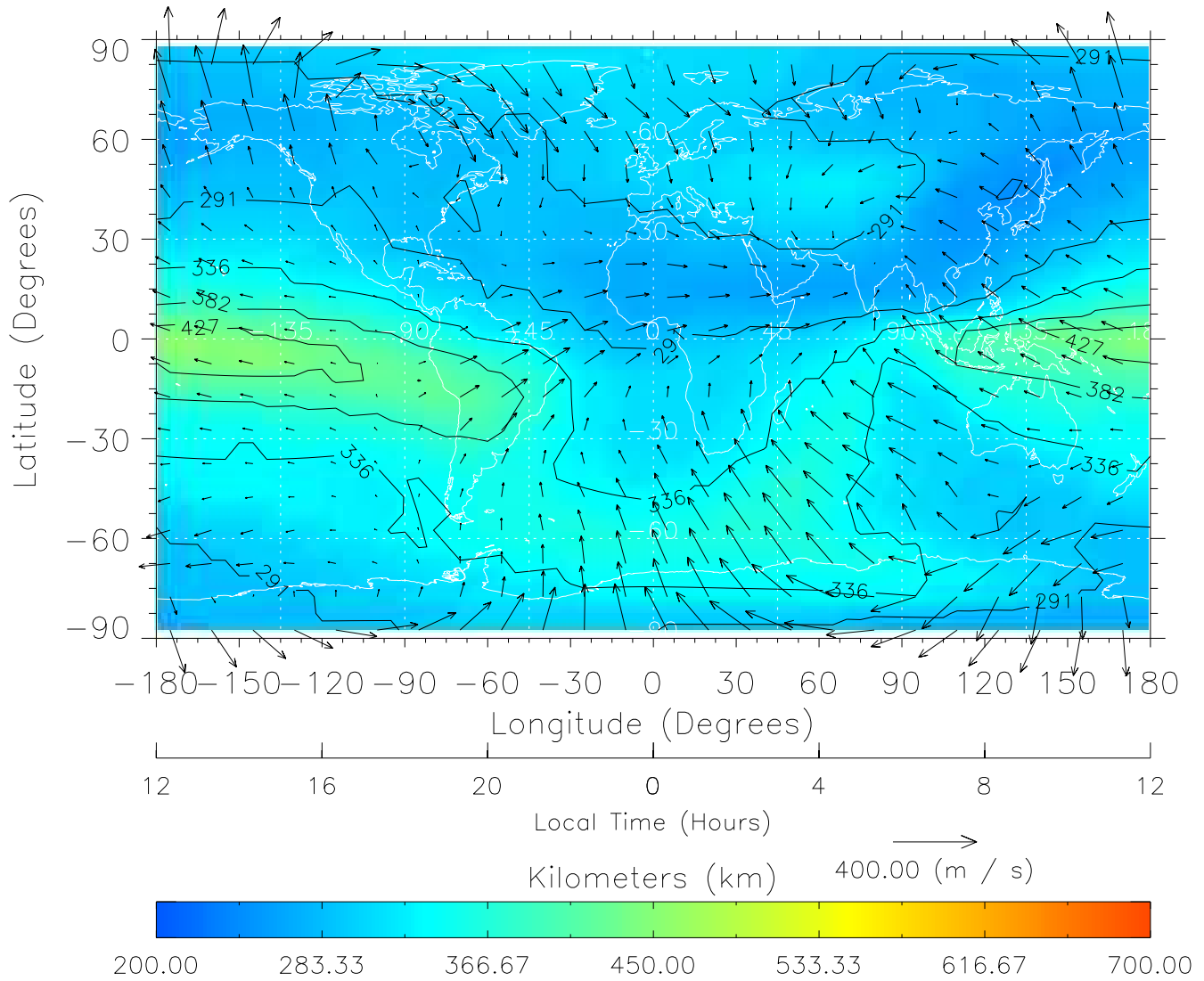
TIME-GCM MAP hmF2 with Neutral Wind vectors ZP = 2.00 UT = 0.00 DOY = 322
