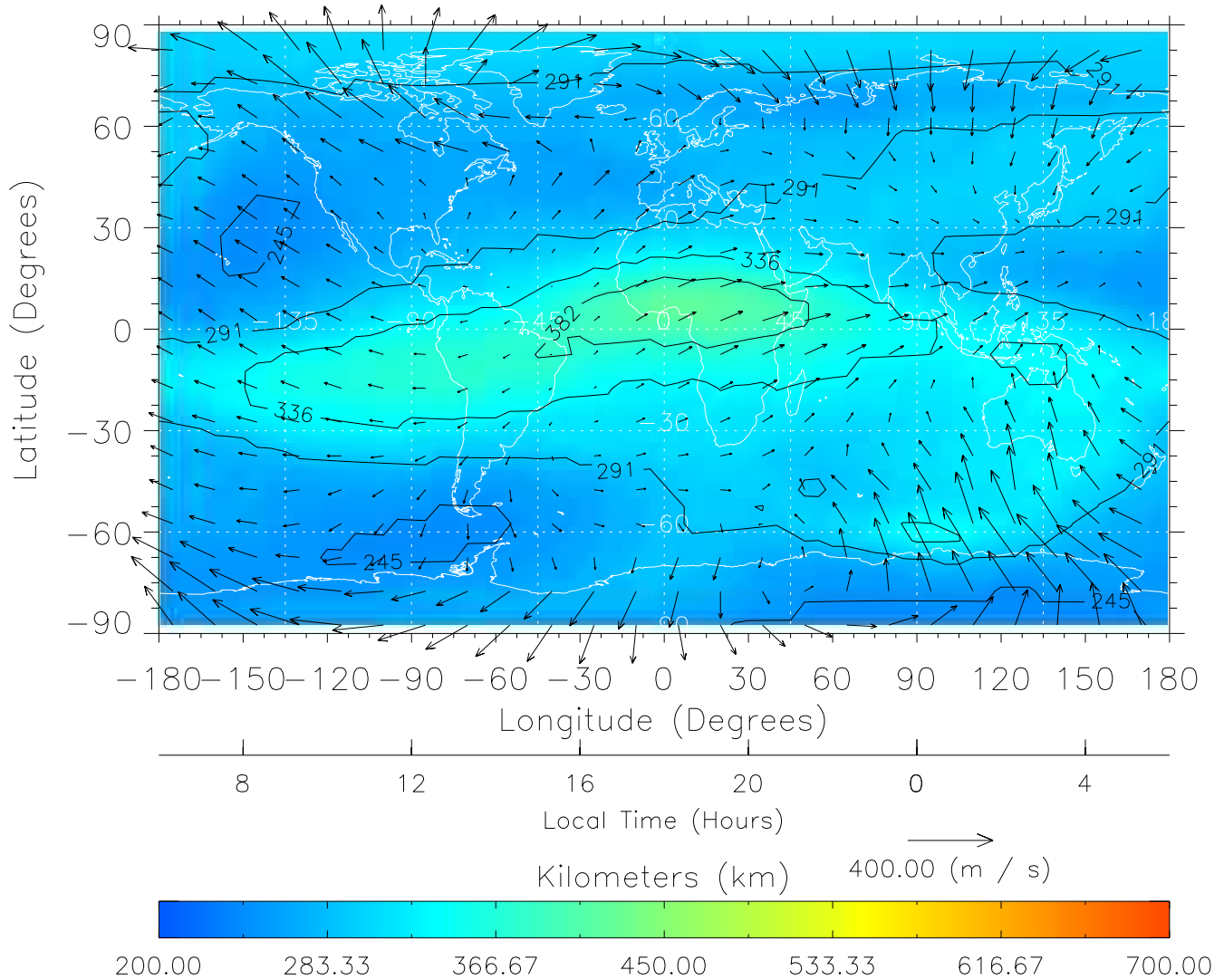
TIME-GCM MAP hmF2 with Neutral Wind vectors ZP = 2.00 UT = 18.00 DOY = 322
