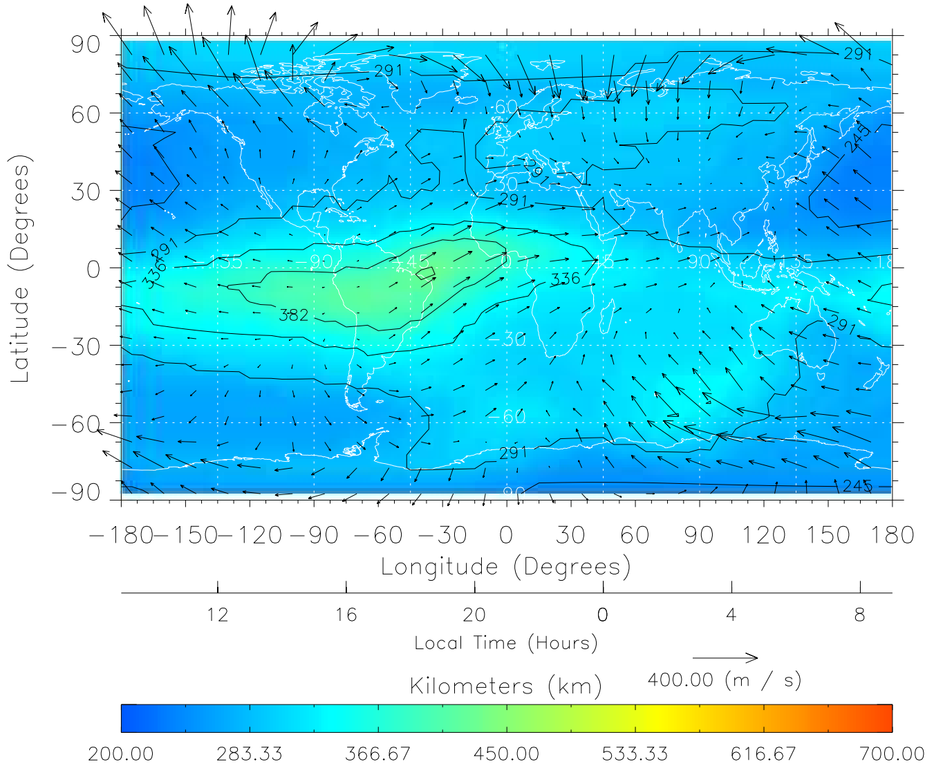
TIME-GCM MAP hmF2 with Neutral Wind vectors ZP = 2.00 UT = 21.00 DOY = 322
