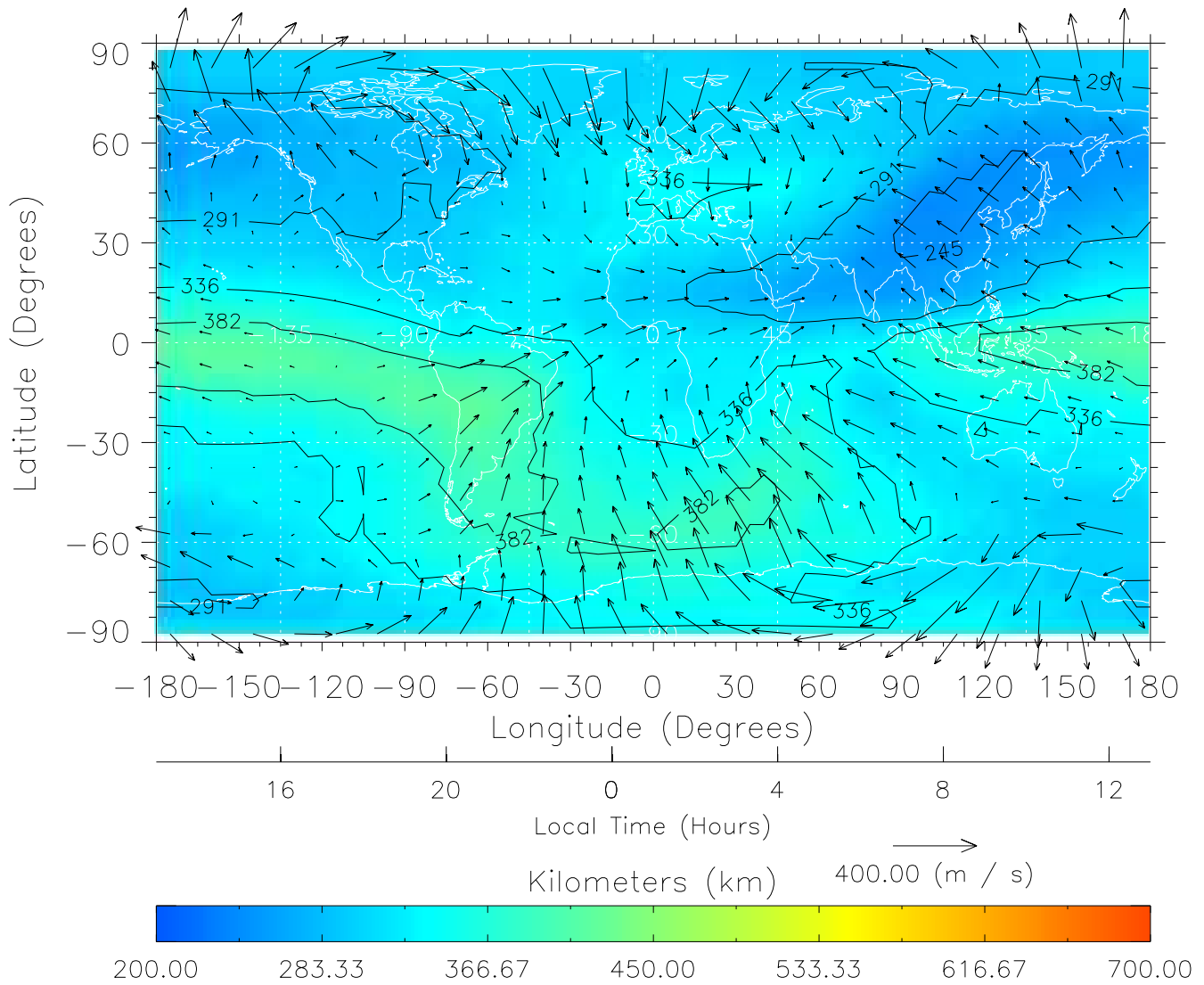
TIME-GCM MAP hmF2 with Neutral Wind vectors ZP = 2.00 UT = 1.00 DOY = 322
