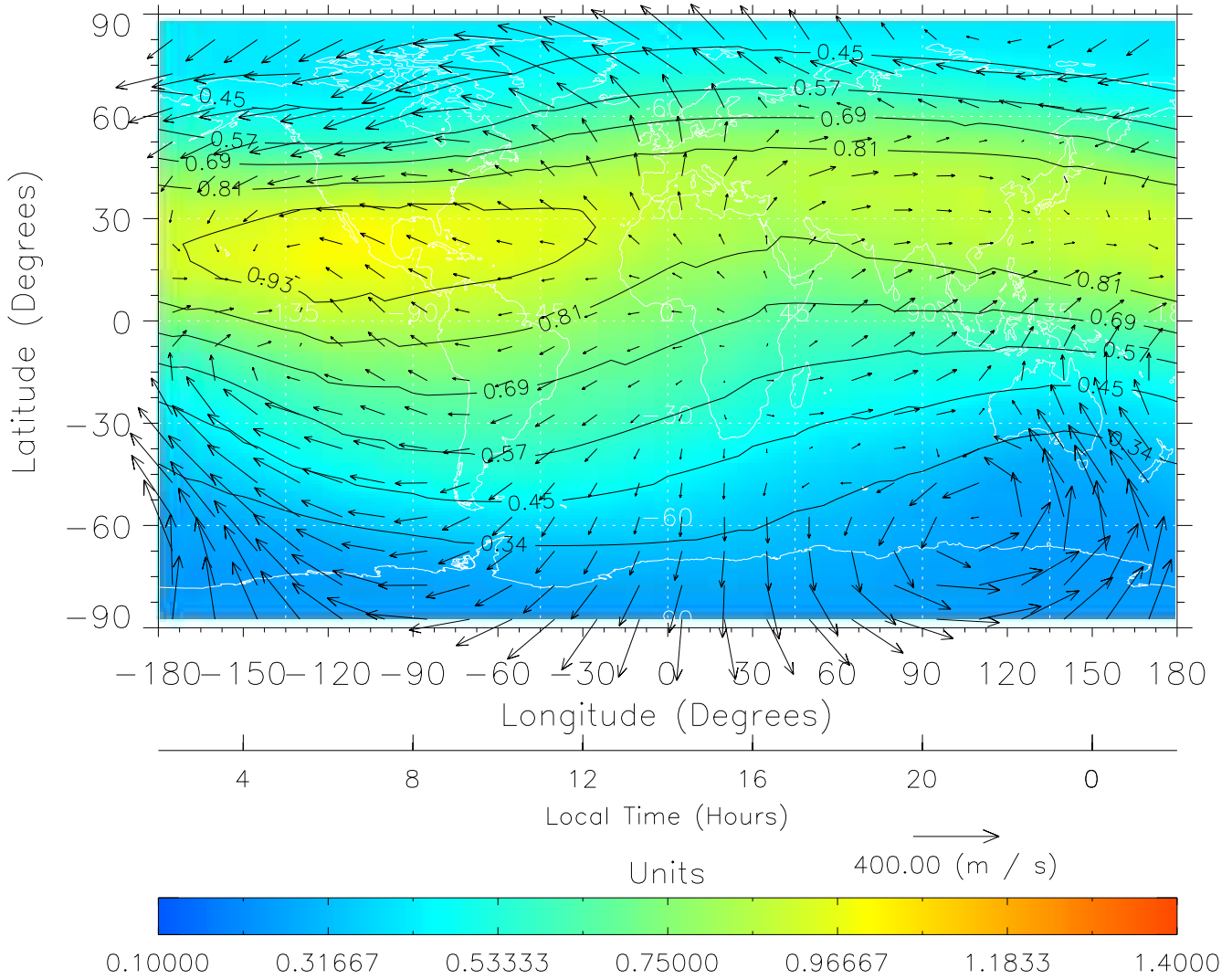
TIME-GCM MAP \Sigma O/N_2 with Neutral Wind vectors ZP = 2.00 UT = 14.00 DOY = 325
