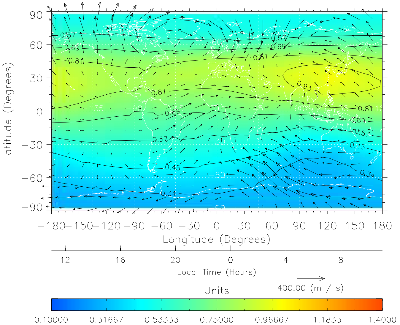
TIME-GCM MAP \Sigma O/N_2 with Neutral Wind vectors ZP = 2.00 UT = 23.00 DOY = 325
