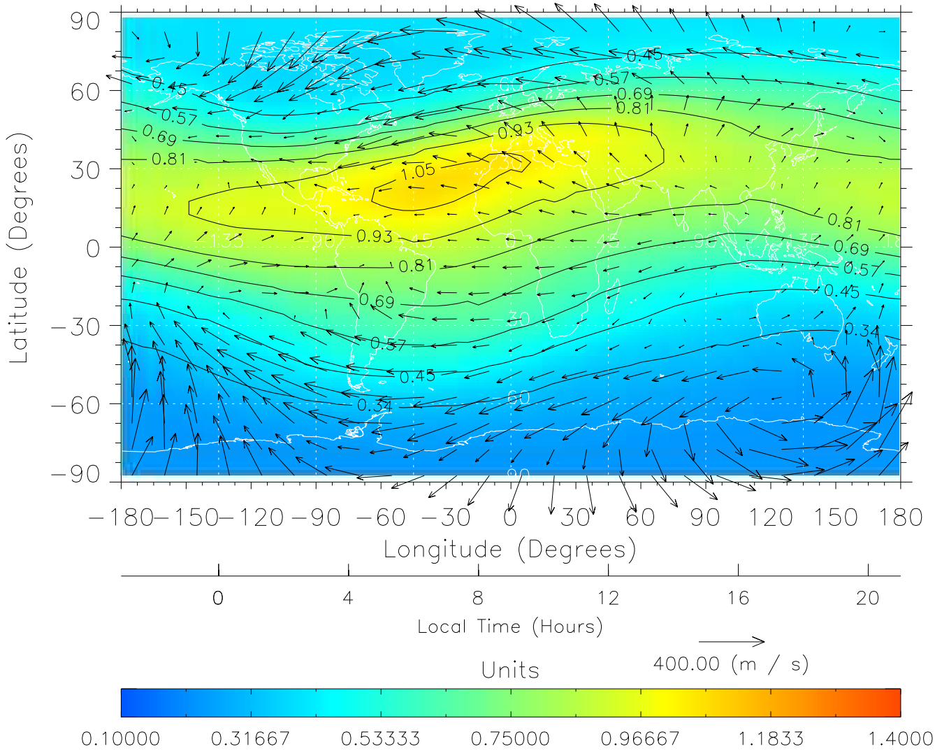
TIME-GCM MAP \Sigma O/N_2 with Neutral Wind vectors ZP = 2.00 UT = 9.00 DOY = 325
