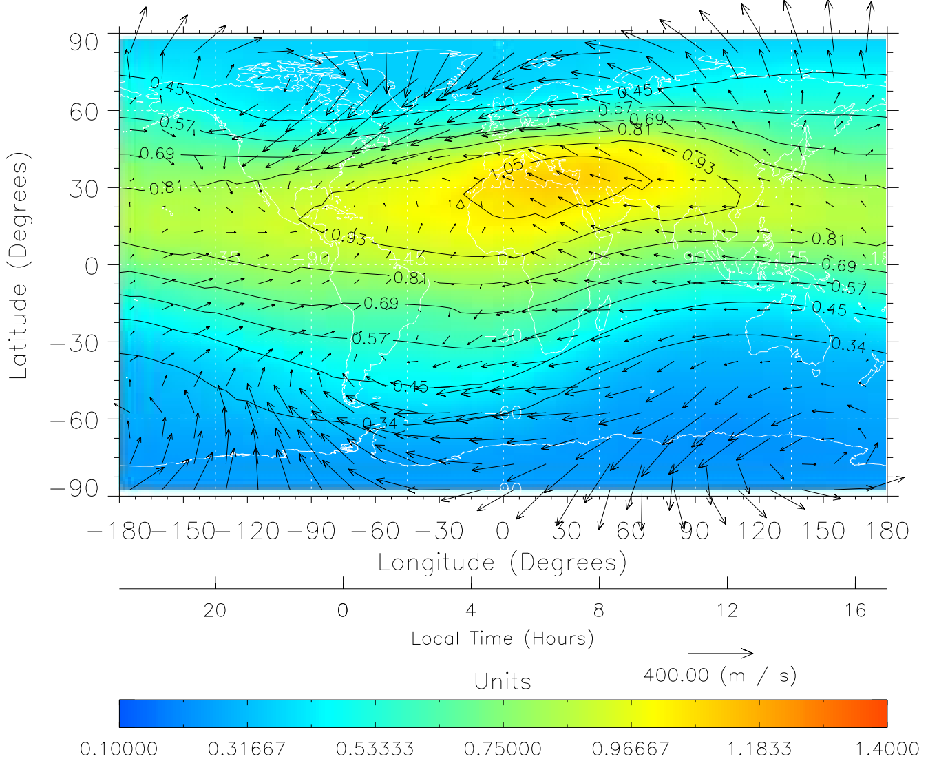
TIME-GCM MAP \Sigma O/N_2 with Neutral Wind vectors ZP = 2.00 UT = 5.00 DOY = 325
