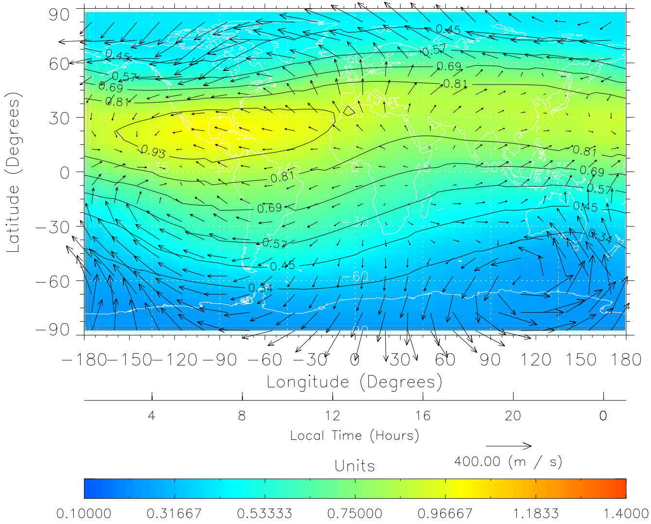
TIME-GCM MAP \Sigma O/N_2 with Neutral Wind vectors ZP = 2.00 UT = 13.00 DOY = 325
