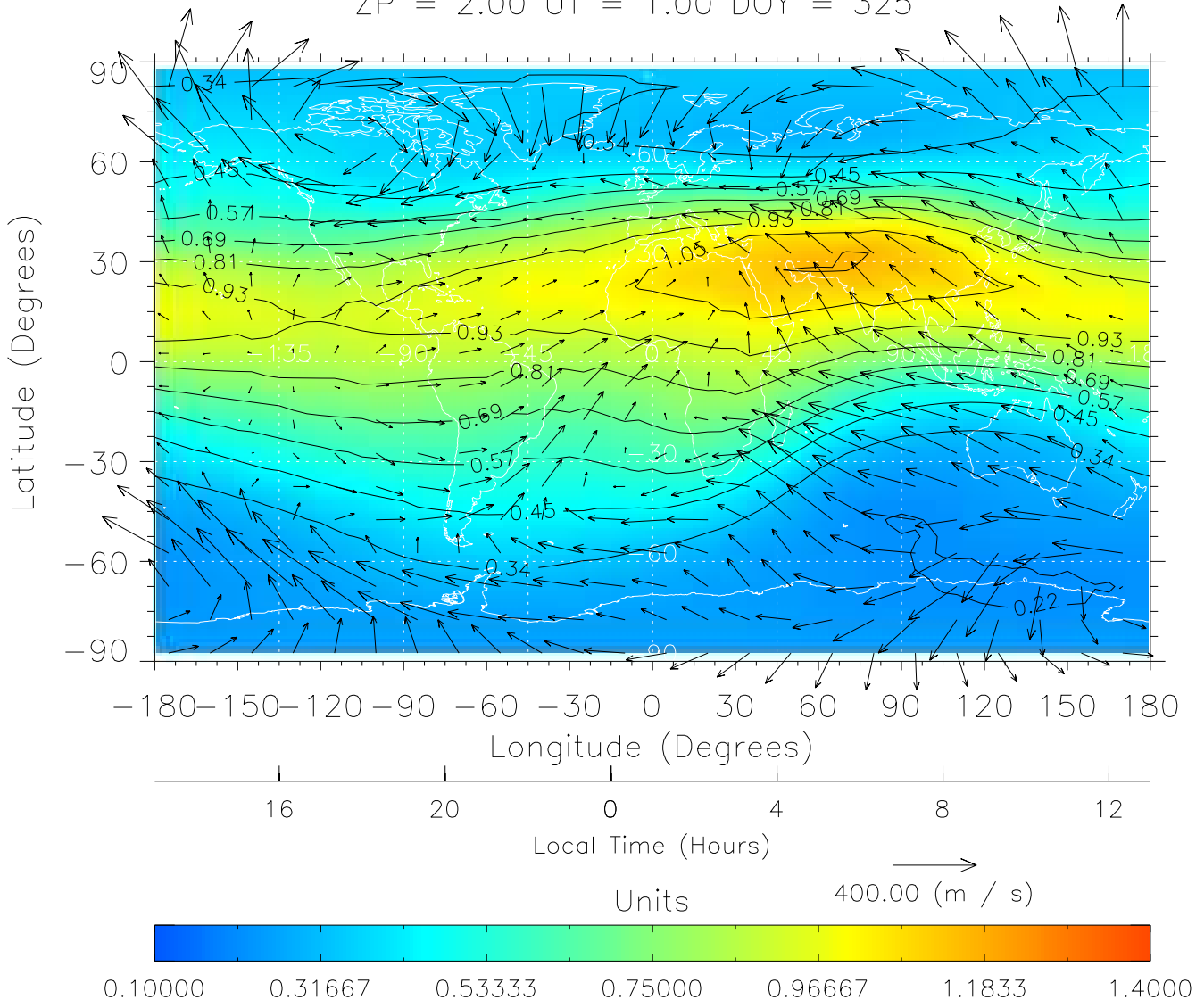
TIME-GCM MAP \Sigma O/N_2 with Neutral Wind vectors ZP = 2.00 UT = 1.00 DOY = 325
