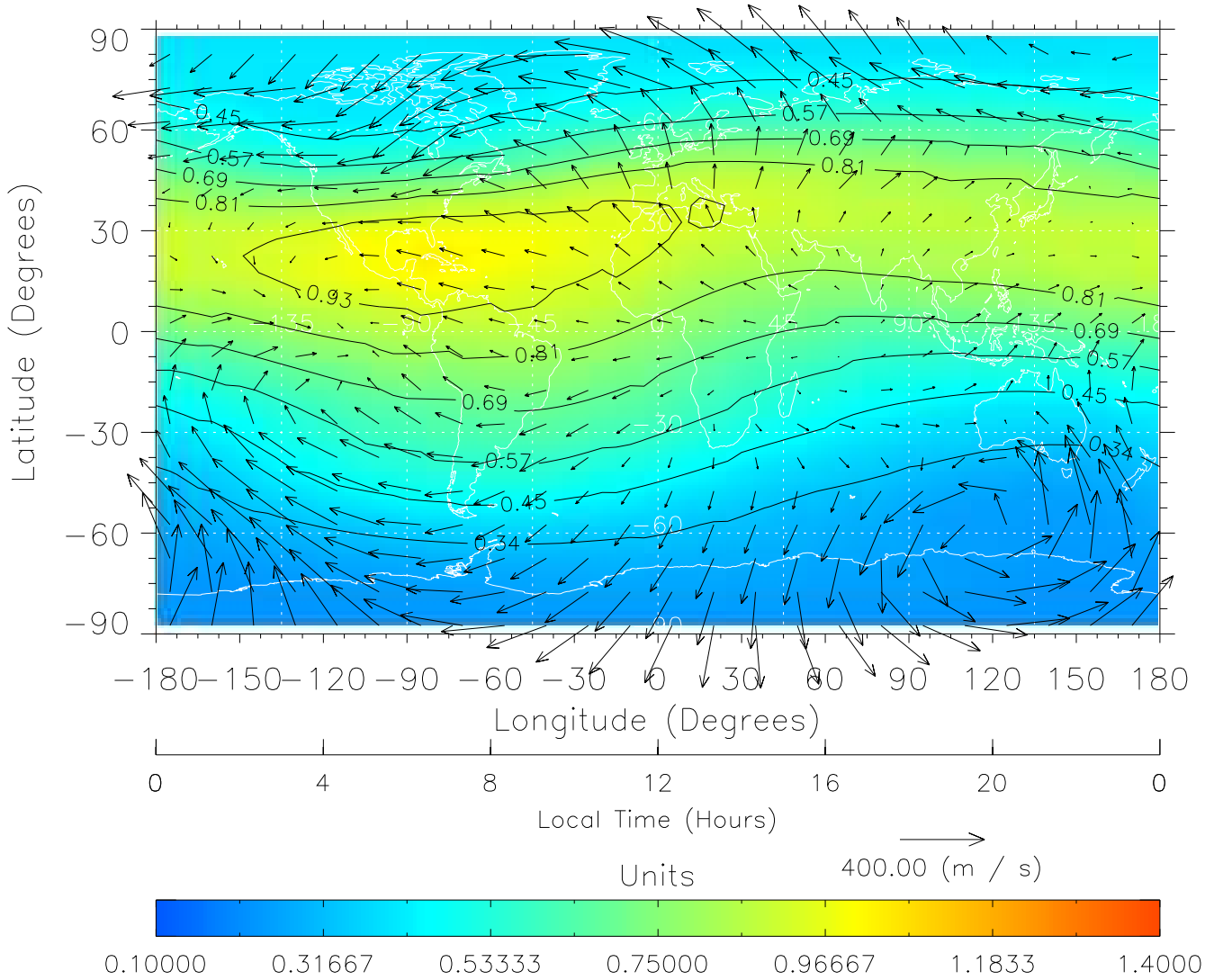
TIME-GCM MAP \Sigma O/N_2 with Neutral Wind vectors ZP = 2.00 UT = 12.00 DOY = 325
