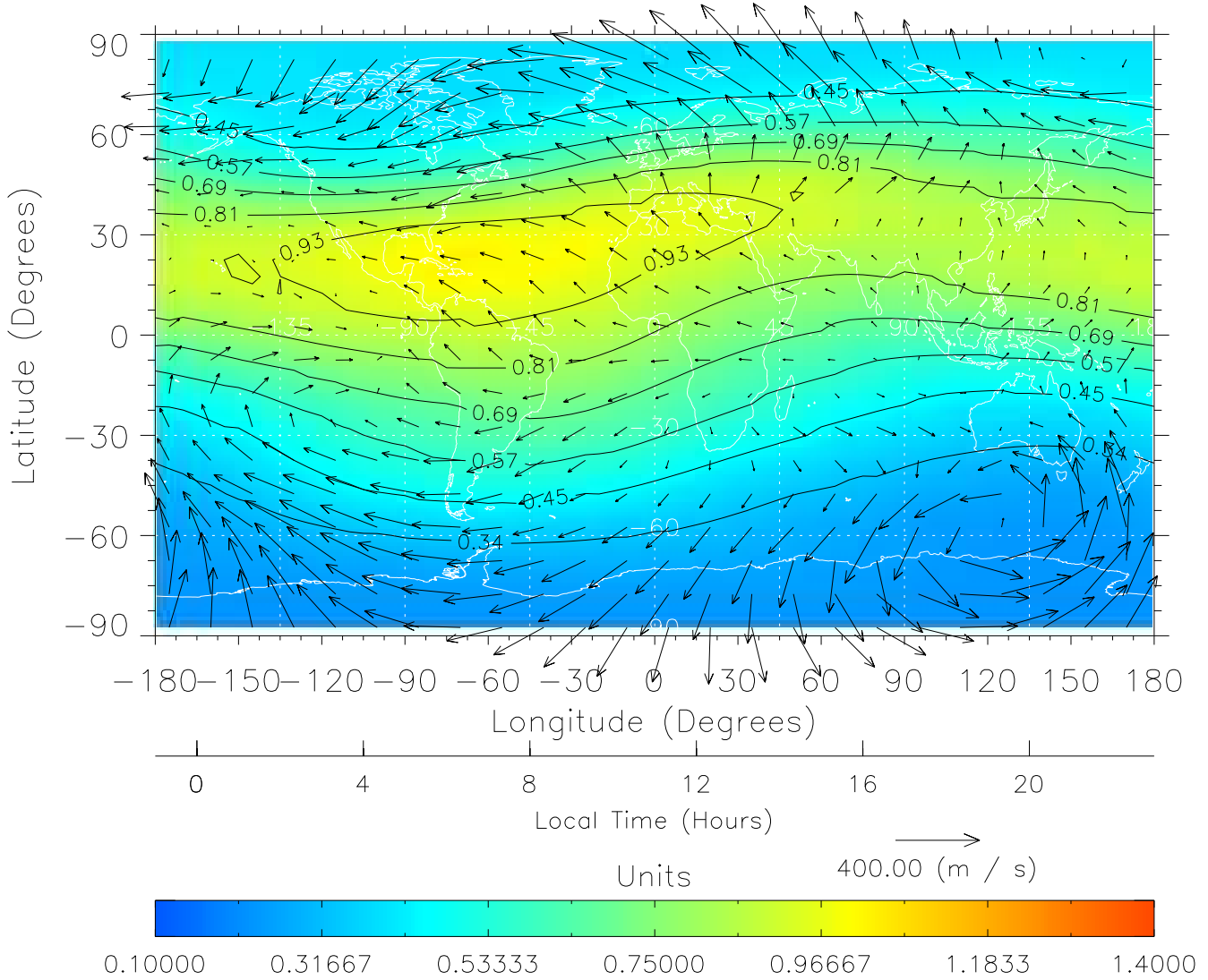
TIME-GCM MAP \Sigma O/N_2 with Neutral Wind vectors ZP = 2.00 UT = 11.00 DOY = 325
