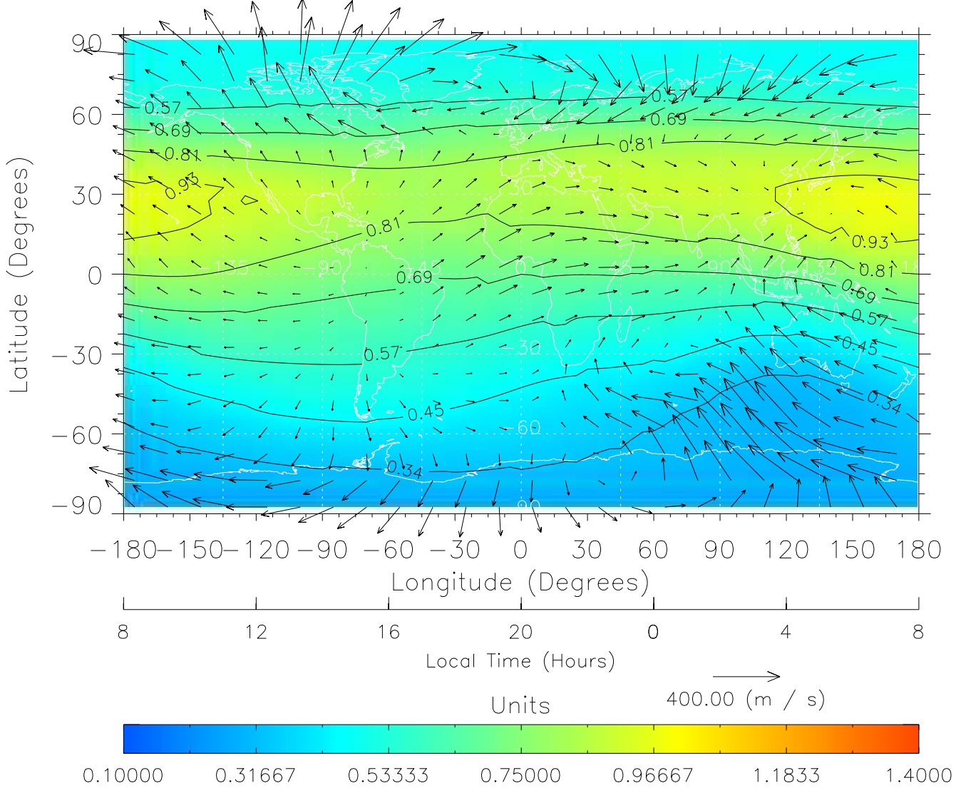
TIME-GCM MAP \Sigma O/N_2 with Neutral Wind vectors ZP = 2.00 UT = 20.00 DOY = 325
