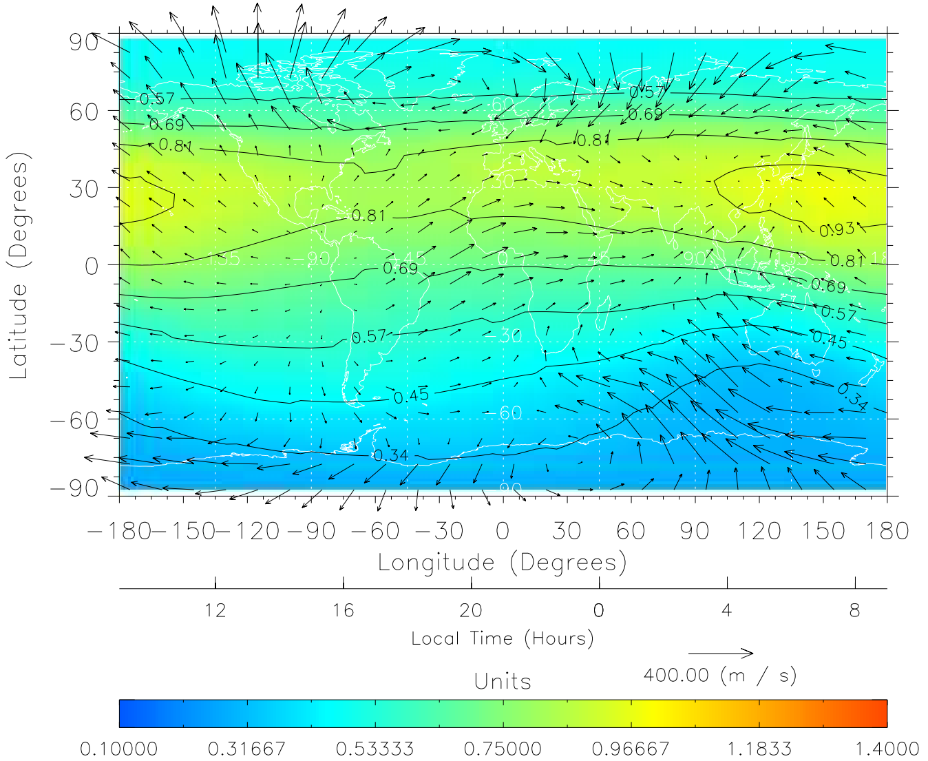
TIME-GCM MAP \Sigma O/N_2 with Neutral Wind vectors ZP = 2.00 UT = 21.00 DOY = 325
