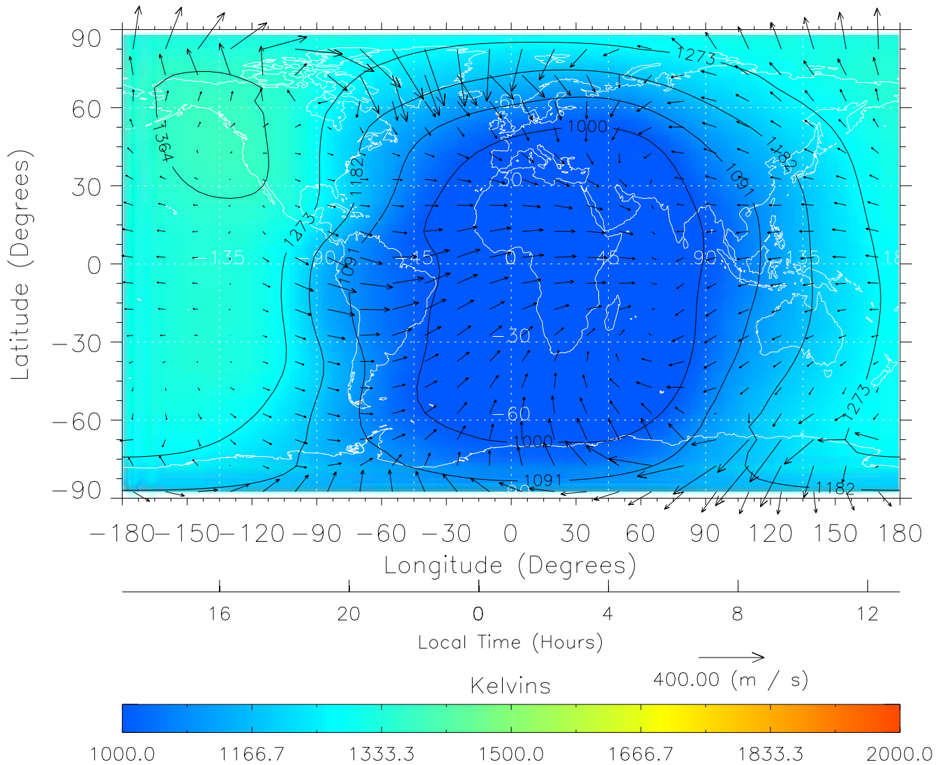
TIME-GCM MAP Temperature with Neutral Wind vectors ZP = 2.00 UT = 1.00 DOY = 089
