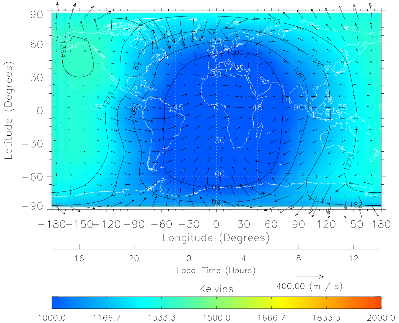
TIME-GCM MAP Temperature with Neutral Wind vectors ZP = 2.00 UT = 2.00 DOY = 089
