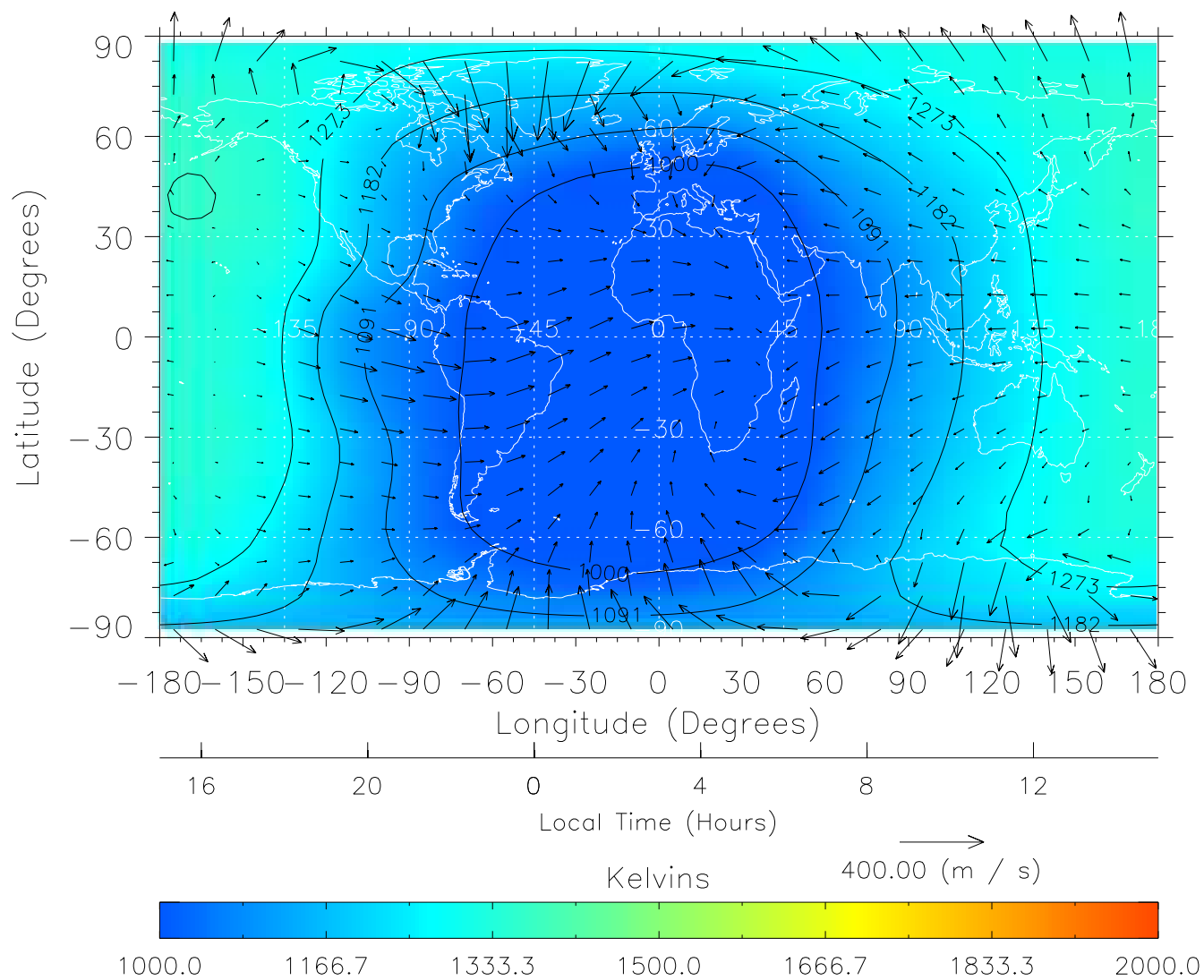
TIME-GCM MAP Temperature with Neutral Wind vectors ZP = 2.00 UT = 3.00 DOY = 089
