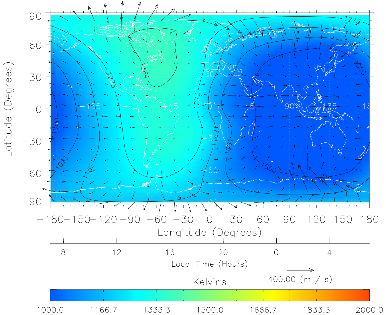
TIME-GCM MAP Temperature with Neutral Wind vectors ZP = 2.00 UT = 19.00 DOY = 089
