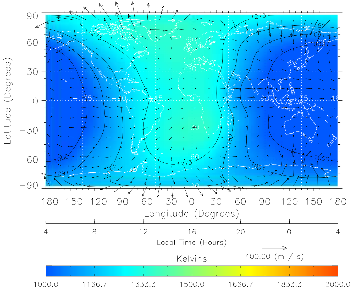
TIME-GCM MAP Temperature with Neutral Wind vectors ZP = 2.00 UT = 16.00 DOY = 089
