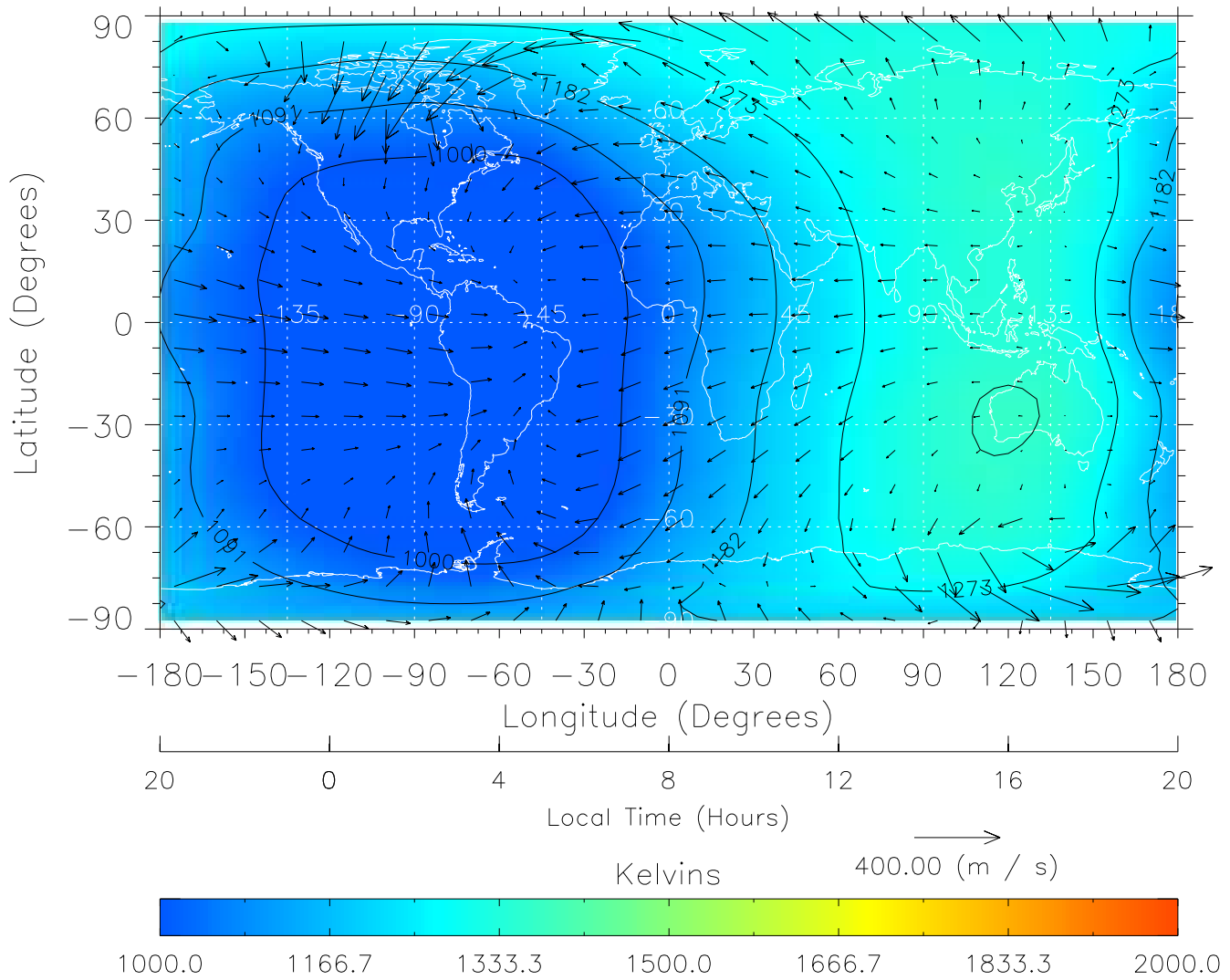
TIME-GCM MAP Temperature with Neutral Wind vectors ZP = 2.00 UT = 8.00 DOY = 089
