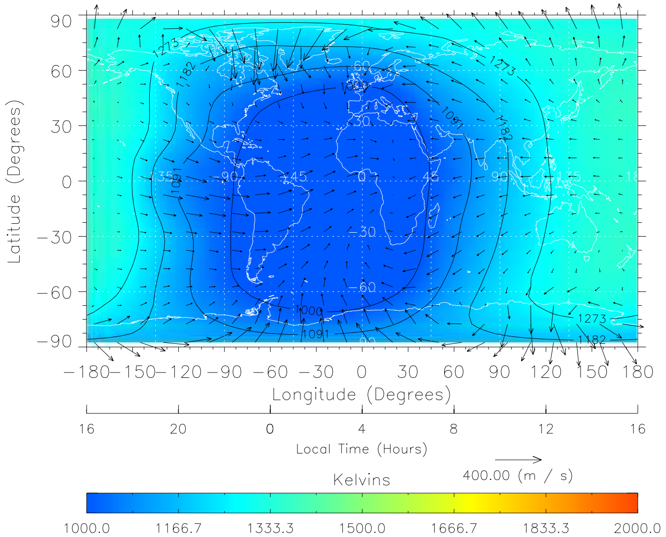
TIME-GCM MAP Temperature with Neutral Wind vectors ZP = 2.00 UT = 4.00 DOY = 089
