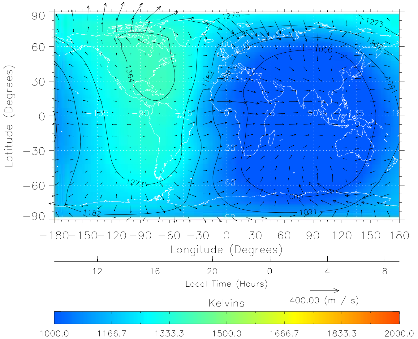
TIME-GCM MAP Temperature with Neutral Wind vectors ZP = 2.00 UT = 21.00 DOY = 089
