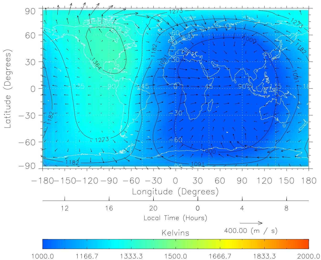
TIME-GCM MAP Temperature with Neutral Wind vectors ZP = 2.00 UT = 22.00 DOY = 089
