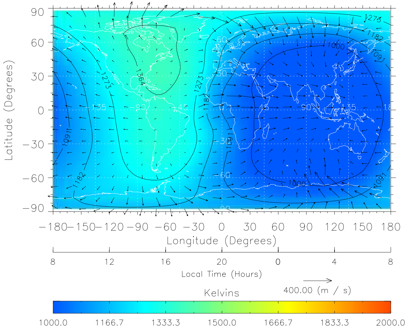
TIME-GCM MAP Temperature with Neutral Wind vectors ZP = 2.00 UT = 20.00 DOY = 089
