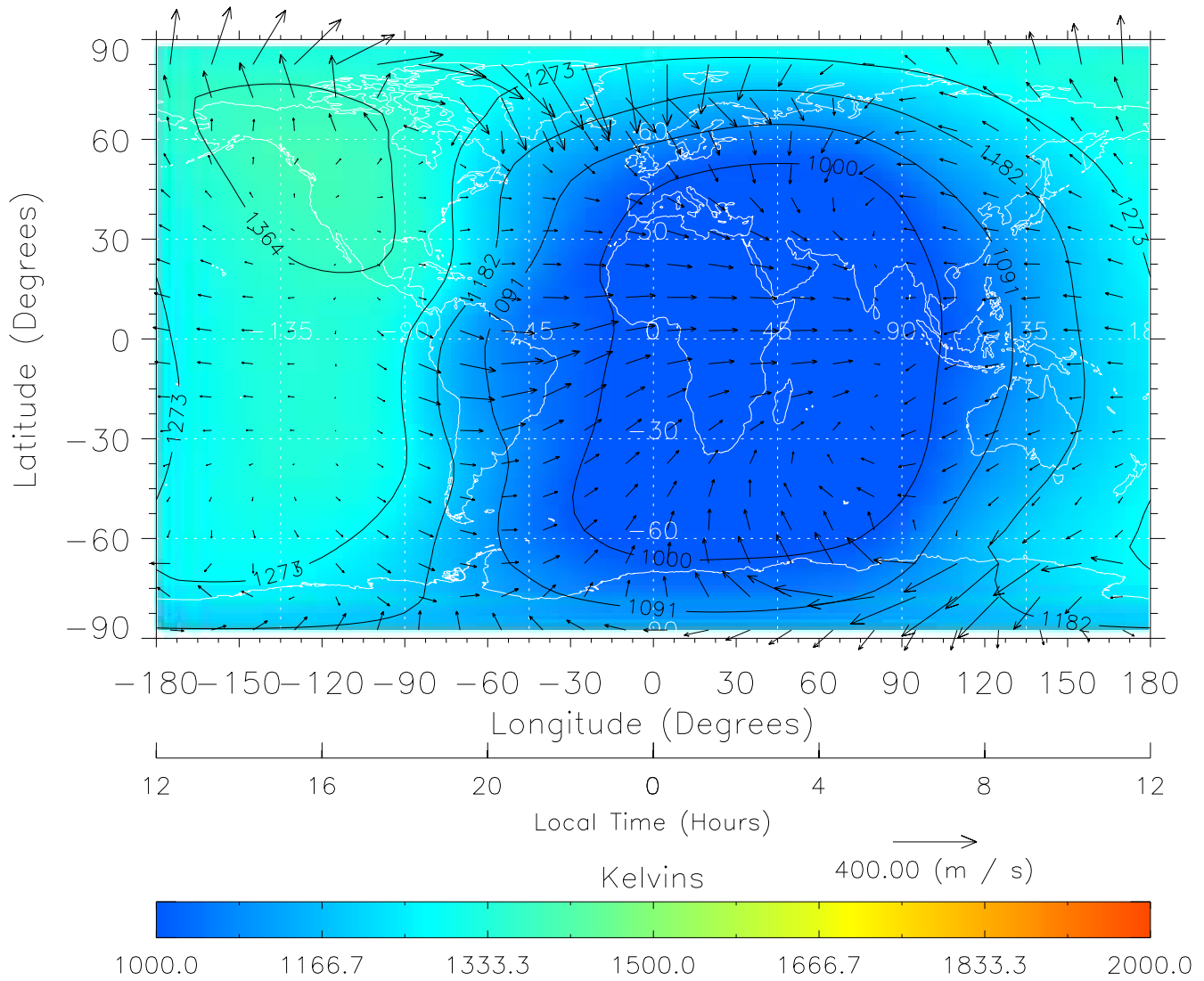
TIME-GCM MAP Temperature with Neutral Wind vectors ZP = 2.00 UT = 0.00 DOY = 089
