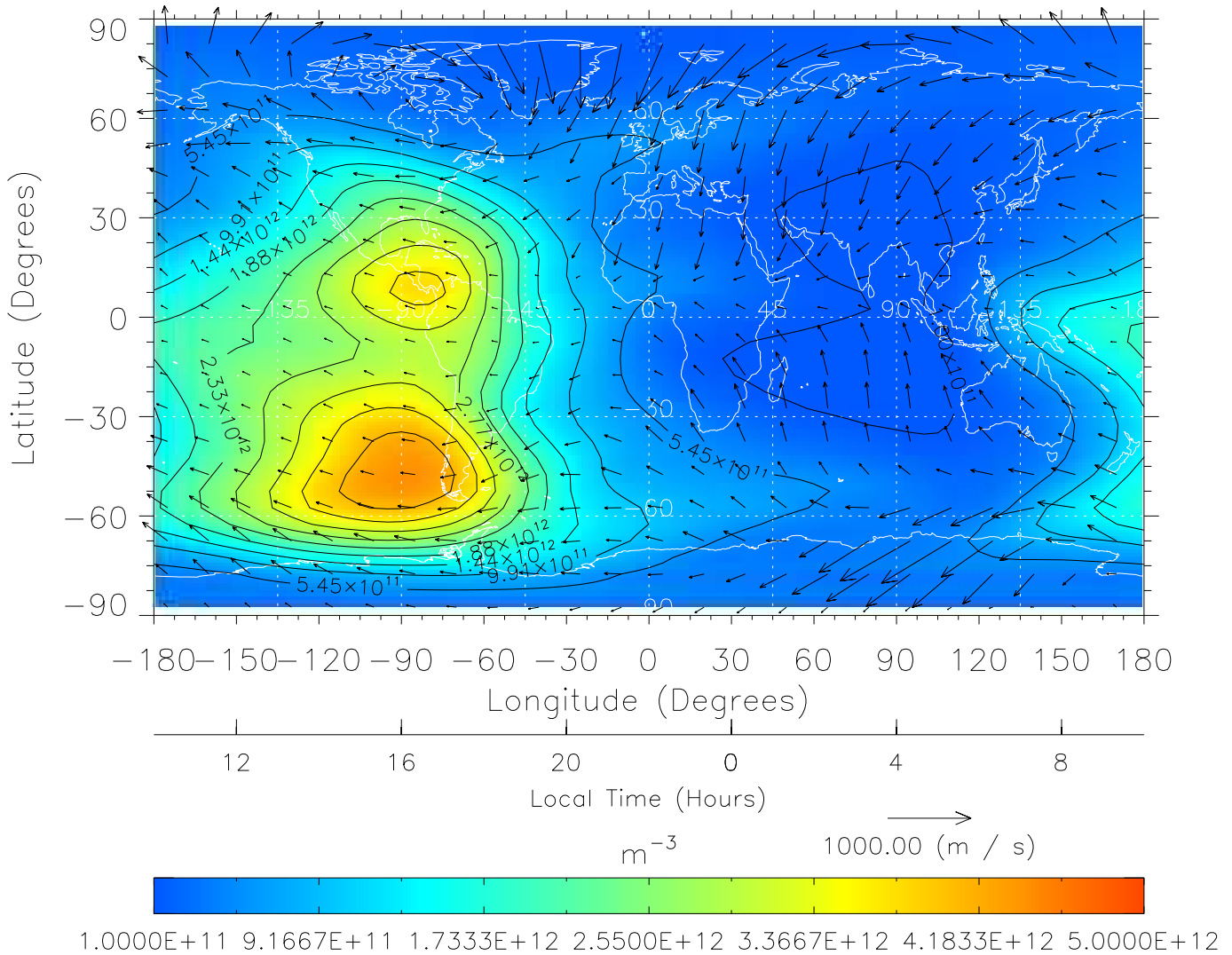
TIME-GCM MAP NmF2 with Neutral Wind vectors ZP = 2.00 UT = 22.00 DOY = 090
