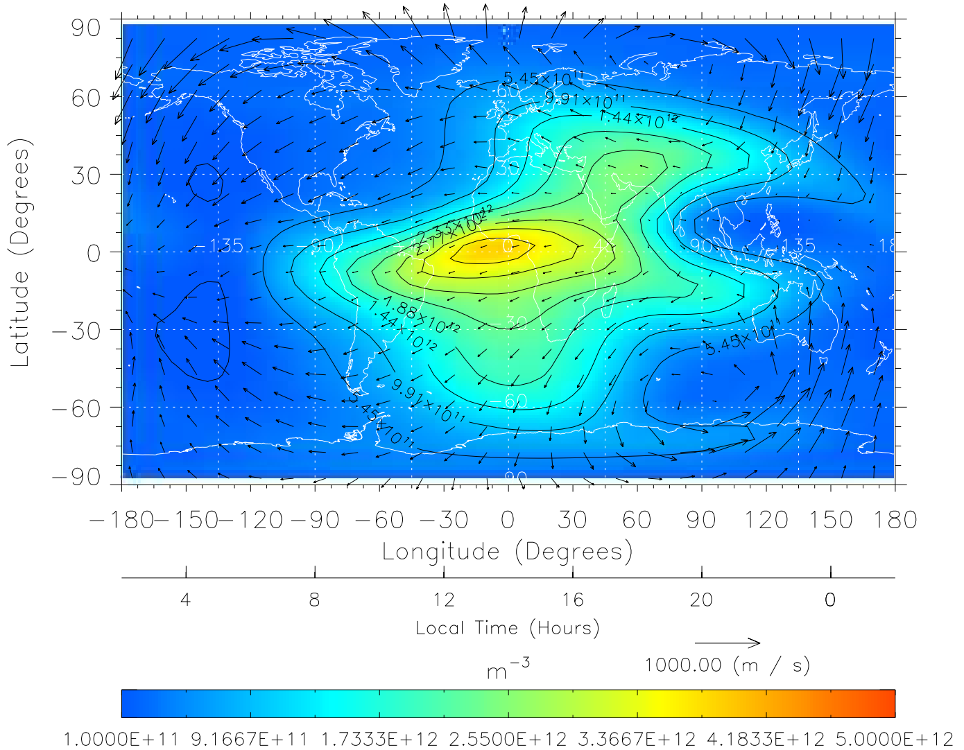
TIME-GCM MAP NmF2 with Neutral Wind vectors ZP = 2.00 UT = 14.00 DOY = 090
