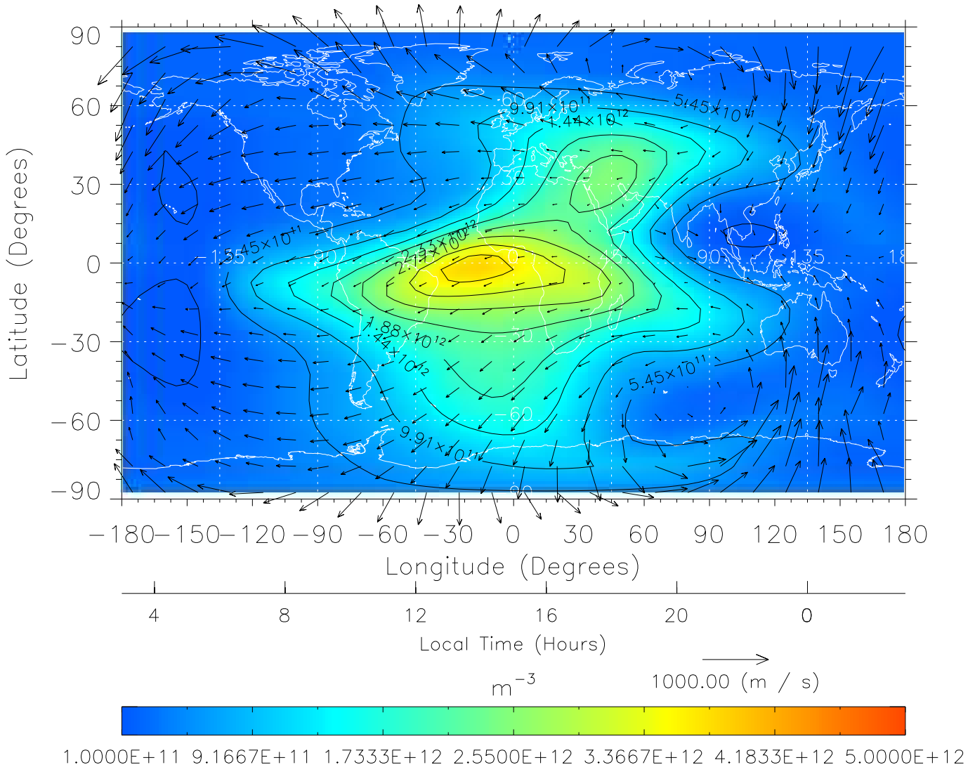
TIME-GCM MAP NmF2 with Neutral Wind vectors ZP = 2.00 UT = 15.00 DOY = 090
