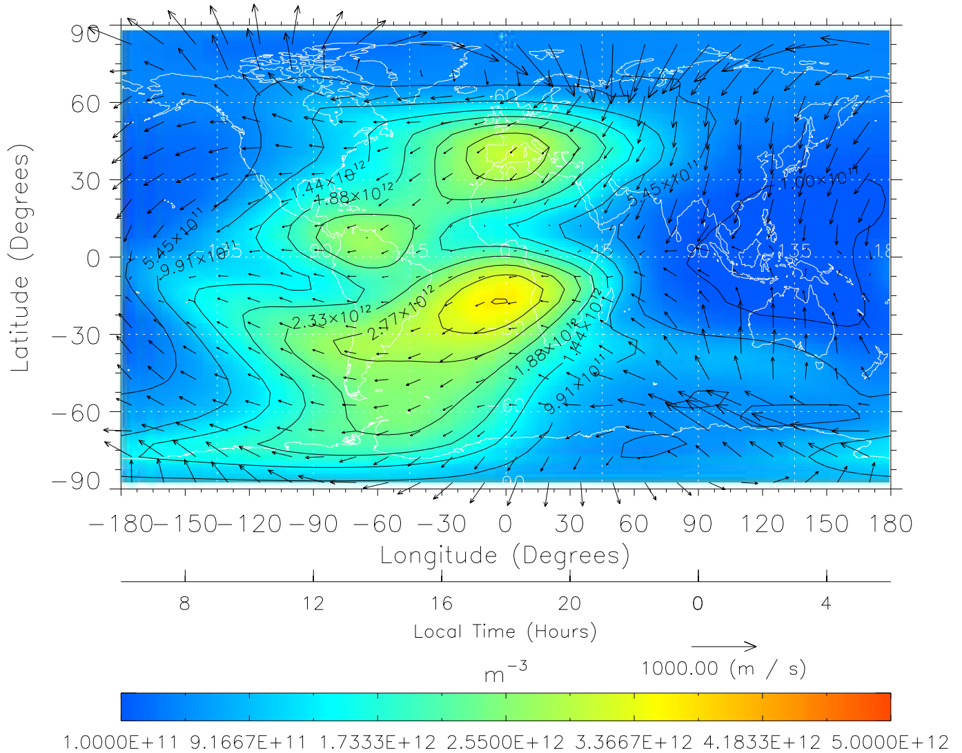
TIME-GCM MAP NmF2 with Neutral Wind vectors ZP = 2.00 UT = 18.00 DOY = 090
