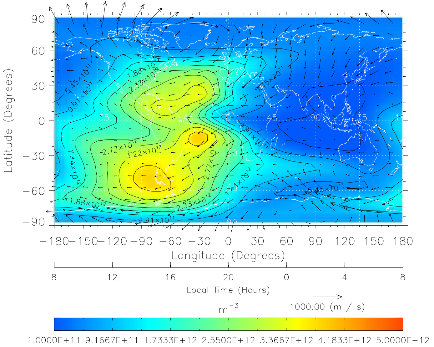
TIME-GCM MAP NmF2 with Neutral Wind vectors ZP = 2.00 UT = 20.00 DOY = 090
