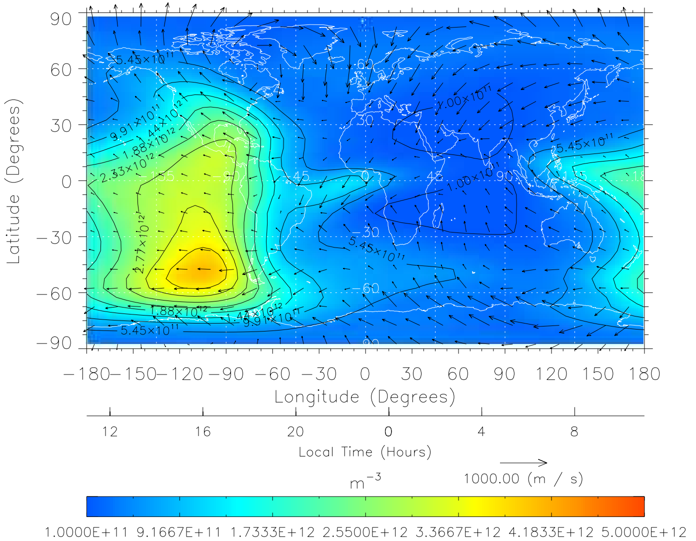
TIME-GCM MAP NmF2 with Neutral Wind vectors ZP = 2.00 UT = 23.00 DOY = 090
