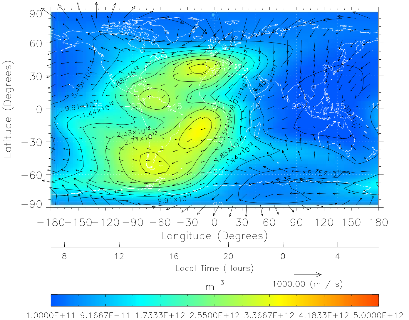
TIME-GCM MAP NmF2 with Neutral Wind vectors ZP = 2.00 UT = 19.00 DOY = 090
