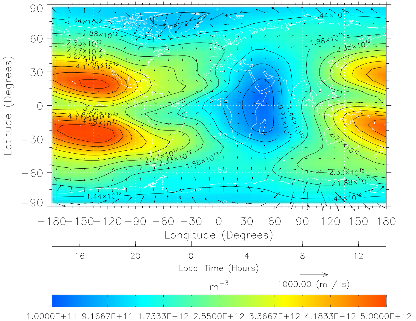
TIME-GCM MAP NmF2 with Neutral Wind vectors ZP = 2.00 UT = 2.00 DOY = 090
