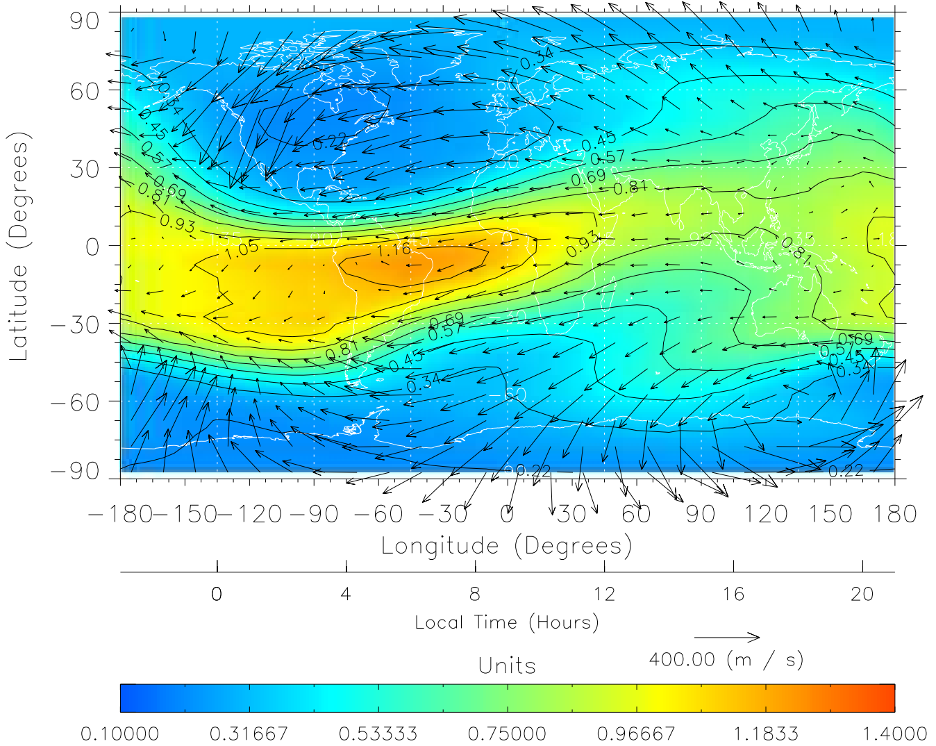
TIME-GCM MAP \Sigma O/N_2 with Neutral Wind vectors ZP = 2.00 UT = 9.00 DOY = 091
