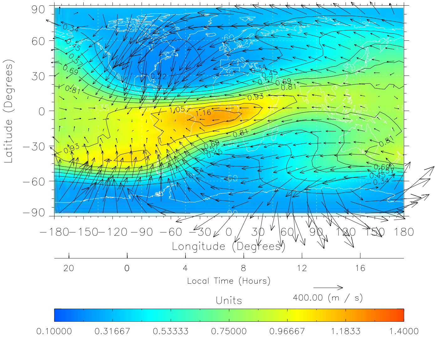
TIME-GCM MAP \Sigma O/N_2 with Neutral Wind vectors ZP = 2.00 UT = 7.00 DOY = 091
