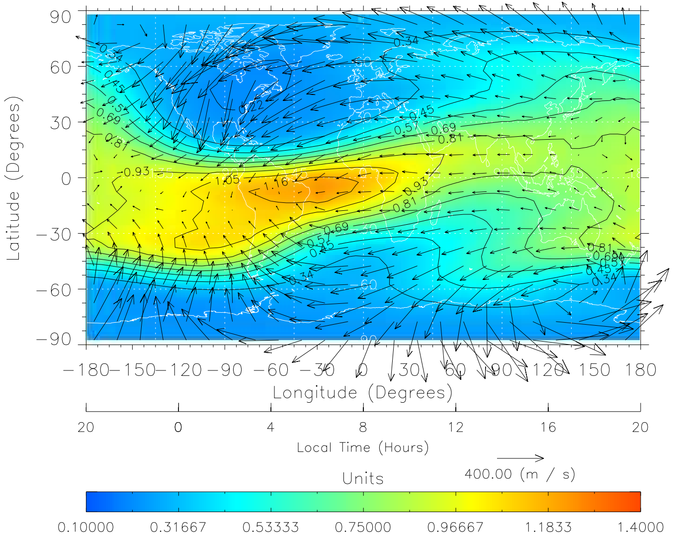
TIME-GCM MAP \Sigma O/N_2 with Neutral Wind vectors ZP = 2.00 UT = 8.00 DOY = 091
