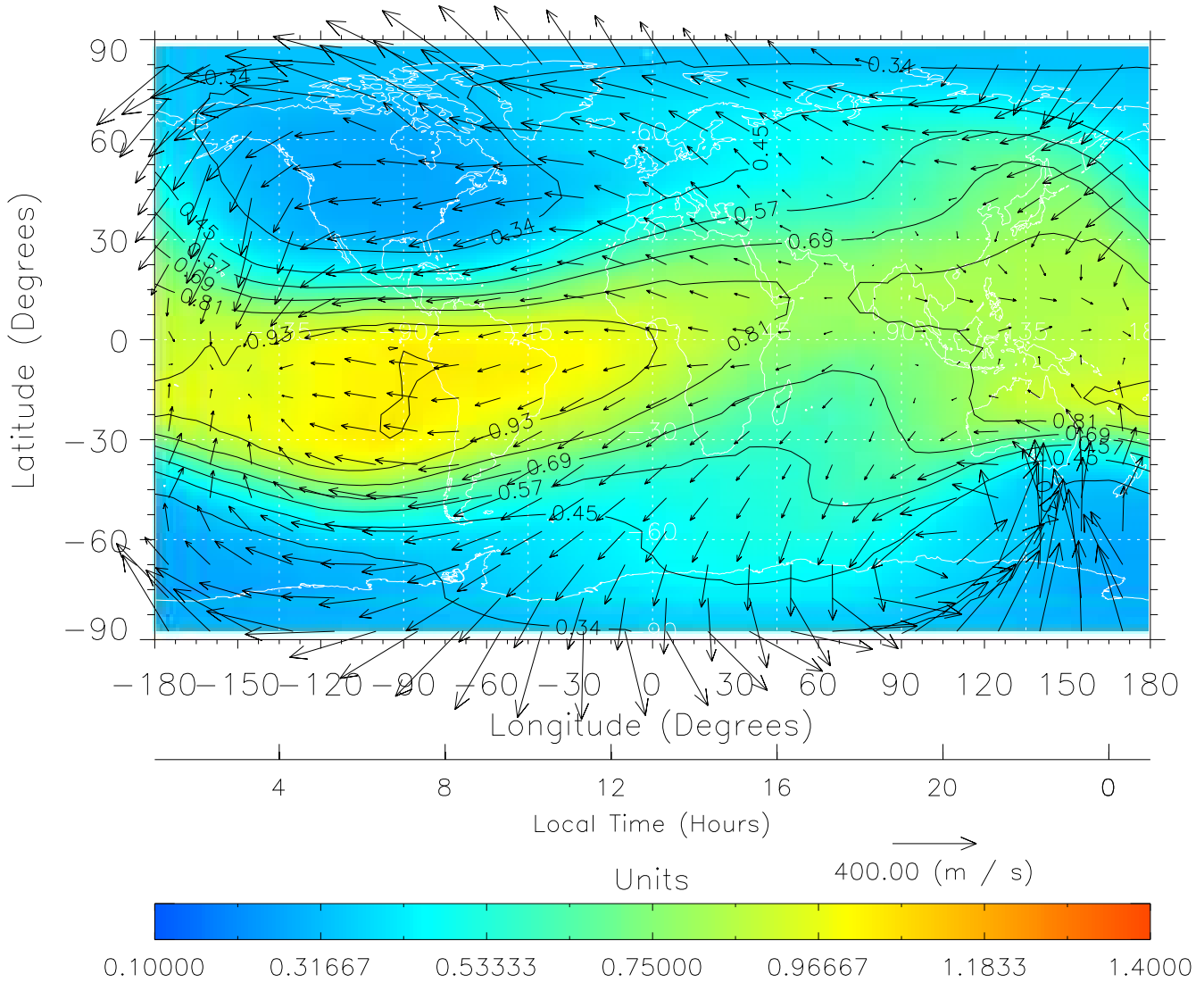
TIME-GCM MAP \Sigma O/N_2 with Neutral Wind vectors ZP = 2.00 UT = 13.00 DOY = 091
