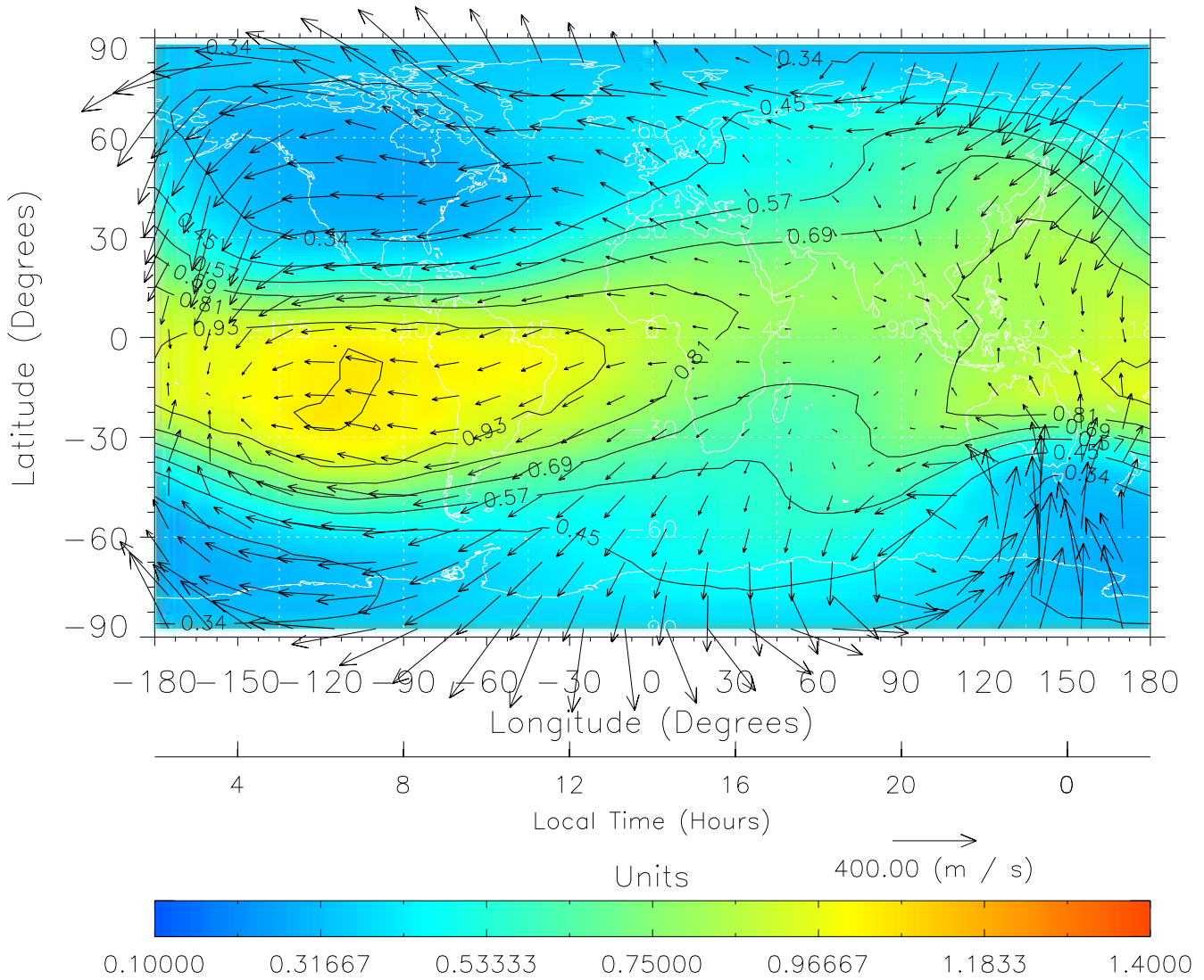
TIME-GCM MAP \Sigma O/N_2 with Neutral Wind vectors ZP = 2.00 UT = 14.00 DOY = 091
