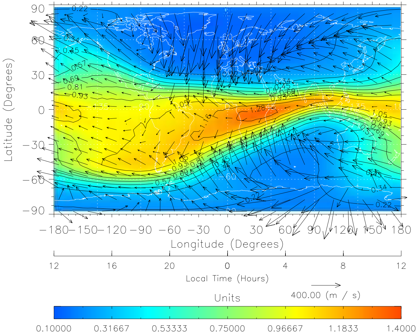
TIME-GCM MAP \Sigma O/N_2 with Neutral Wind vectors ZP = 2.00 UT = 0.00 DOY = 091
