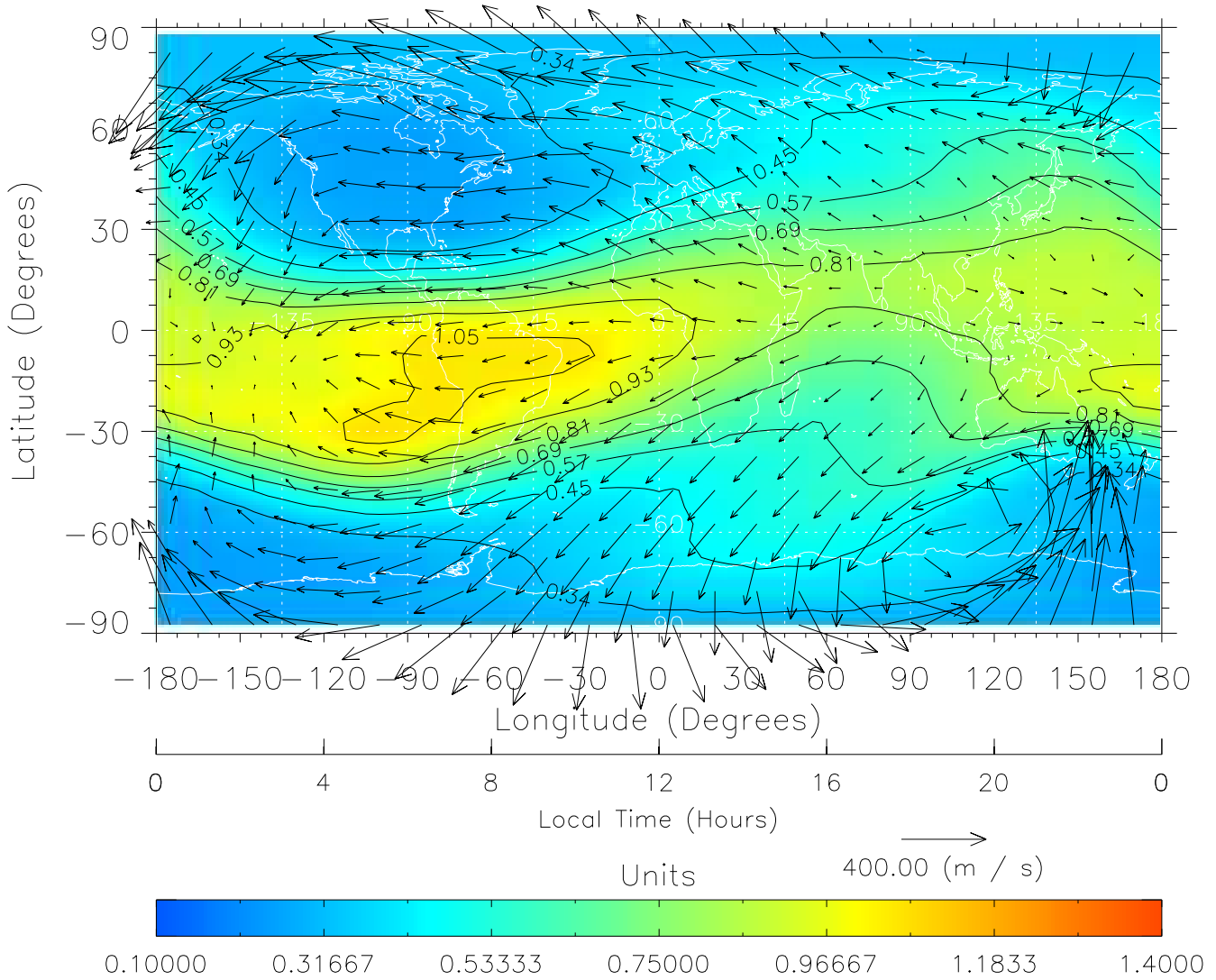
TIME-GCM MAP \Sigma O/N_2 with Neutral Wind vectors ZP = 2.00 UT = 12.00 DOY = 091
