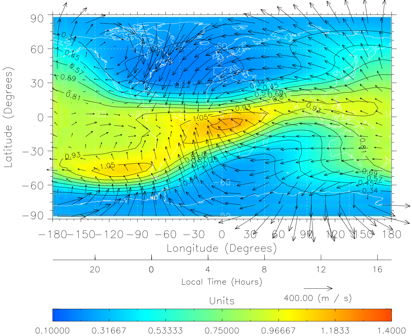
TIME-GCM MAP \Sigma O/N_2 with Neutral Wind vectors ZP = 2.00 UT = 5.00 DOY = 091
