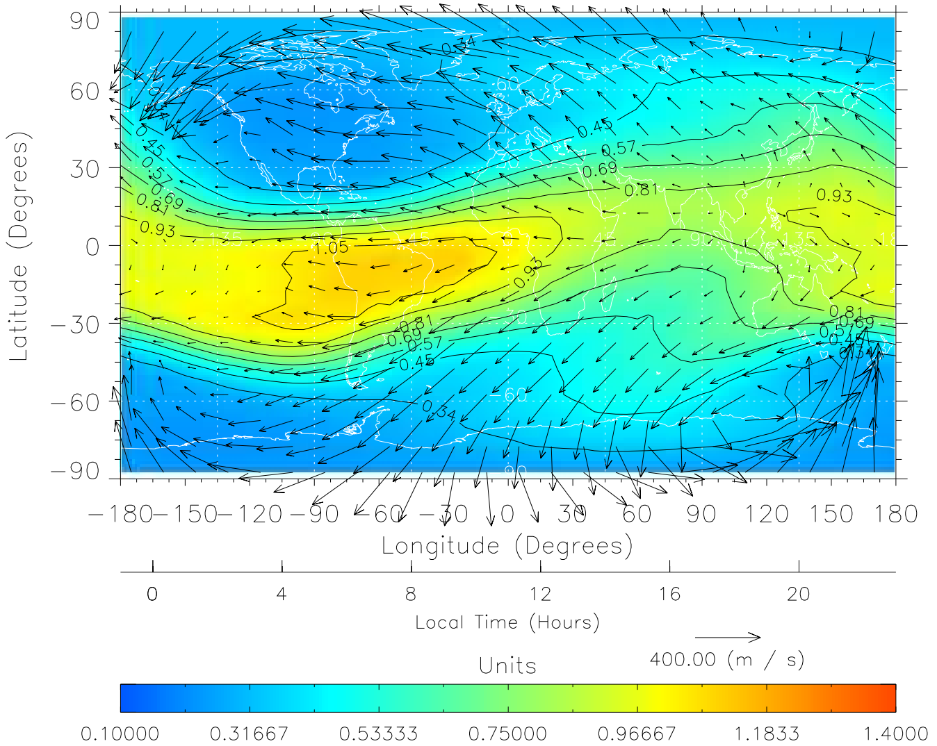
TIME-GCM MAP \Sigma O/N_2 with Neutral Wind vectors ZP = 2.00 UT = 11.00 DOY = 091
