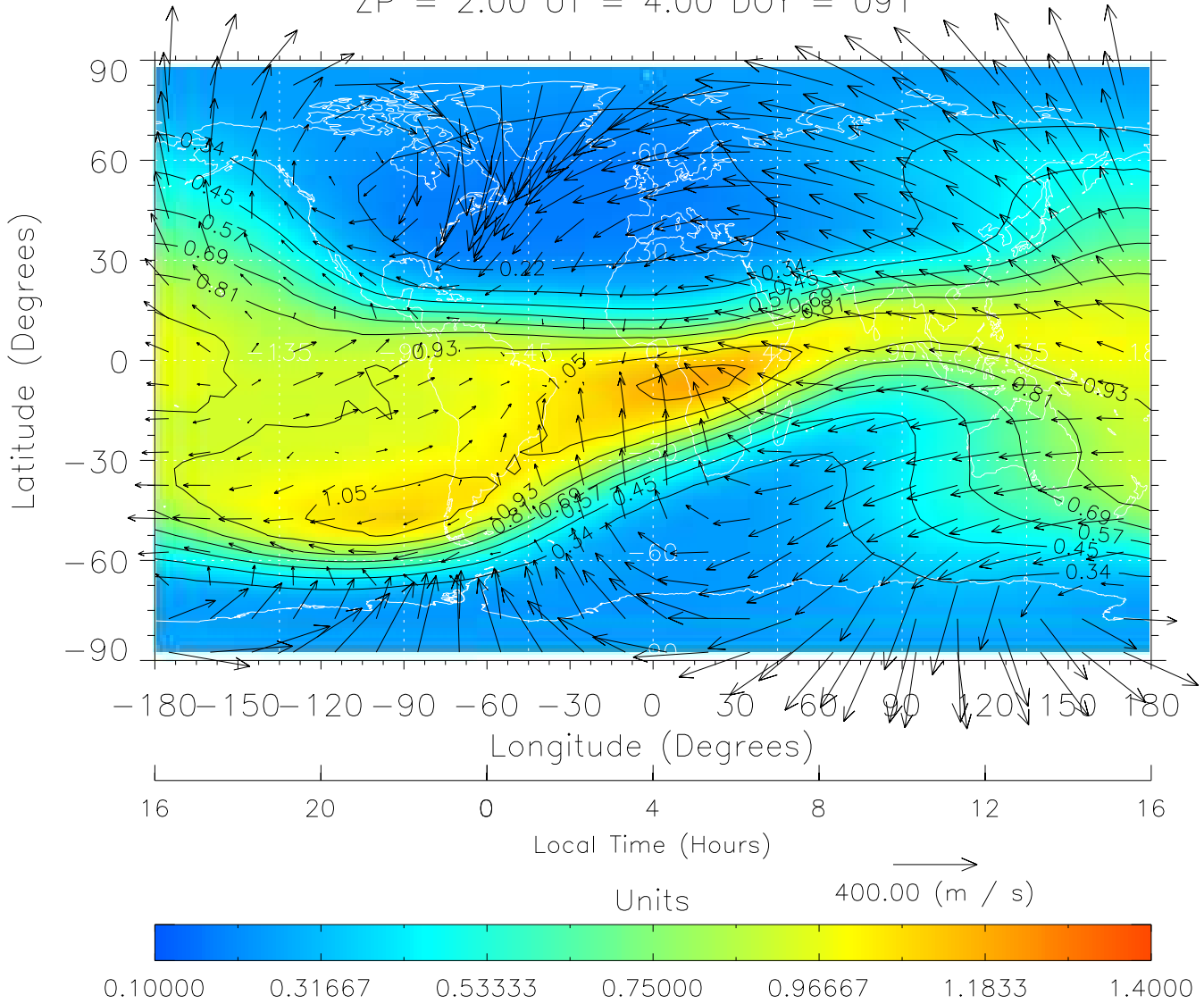
TIME-GCM MAP \Sigma O/N_2 with Neutral Wind vectors ZP = 2.00 UT = 4.00 DOY = 091
