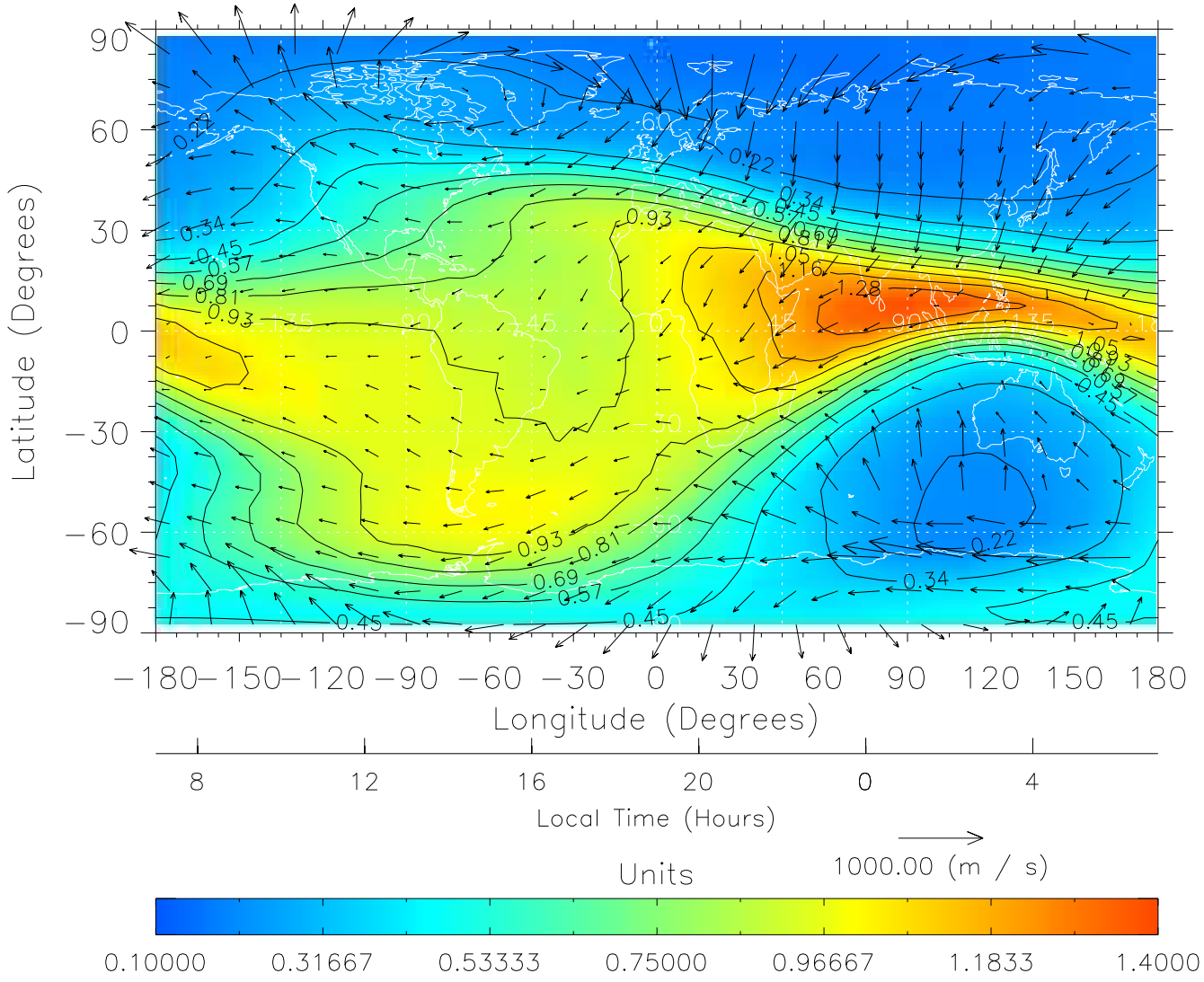
TIME-GCM MAP \Sigma O/N_2 with Neutral Wind vectors ZP = 2.00 UT = 19.00 DOY = 090
