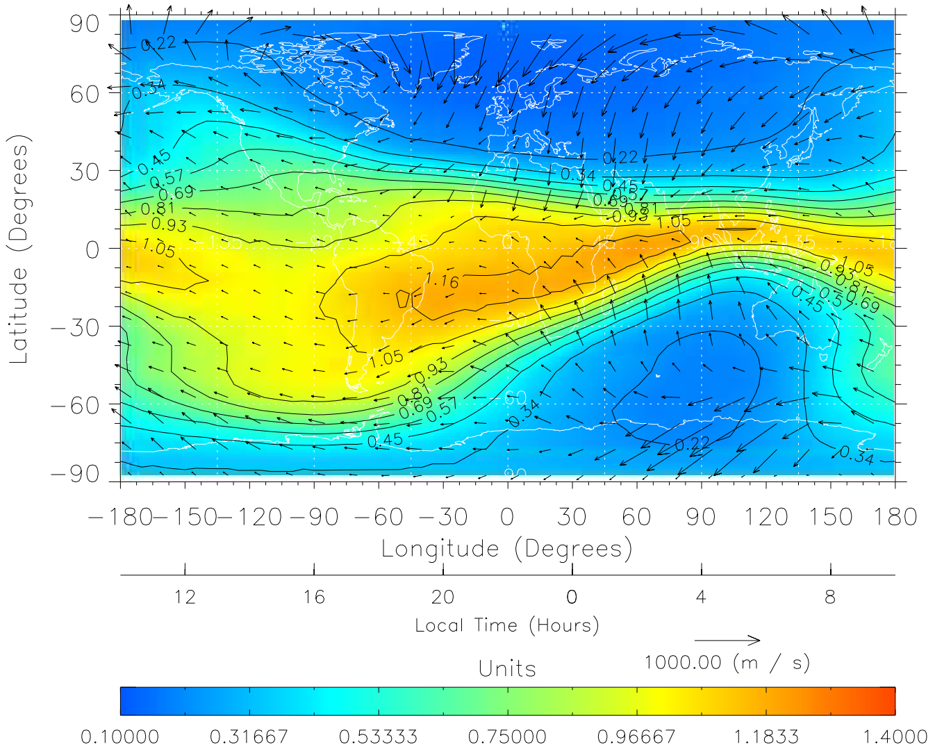
TIME-GCM MAP \Sigma O/N_2 with Neutral Wind vectors ZP = 2.00 UT = 22.00 DOY = 090
