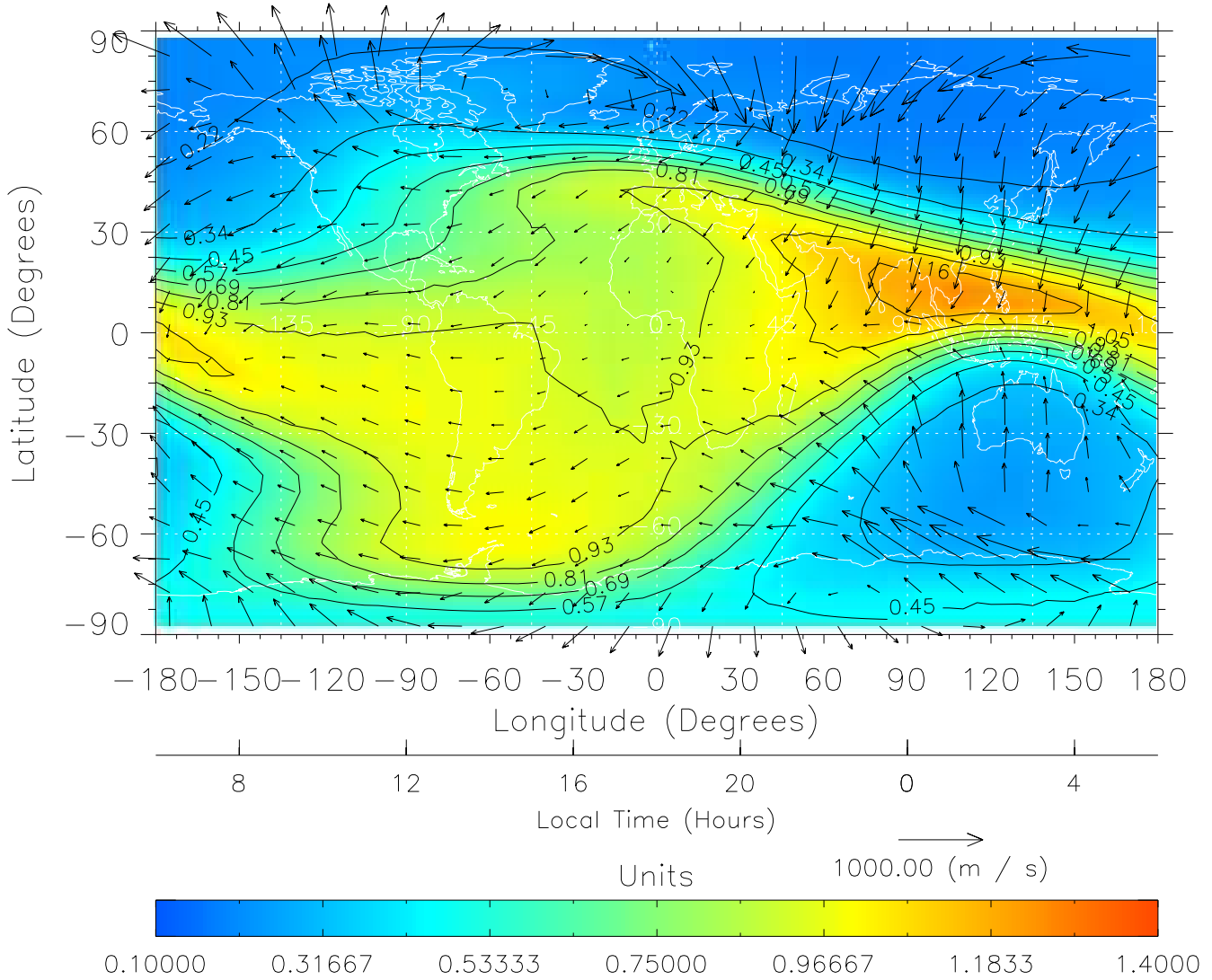
TIME-GCM MAP \Sigma O/N_2 with Neutral Wind vectors ZP = 2.00 UT = 18.00 DOY = 090
