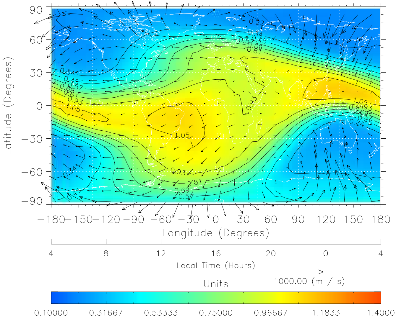
TIME-GCM MAP \Sigma O/N_2 with Neutral Wind vectors ZP = 2.00 UT = 16.00 DOY = 090
