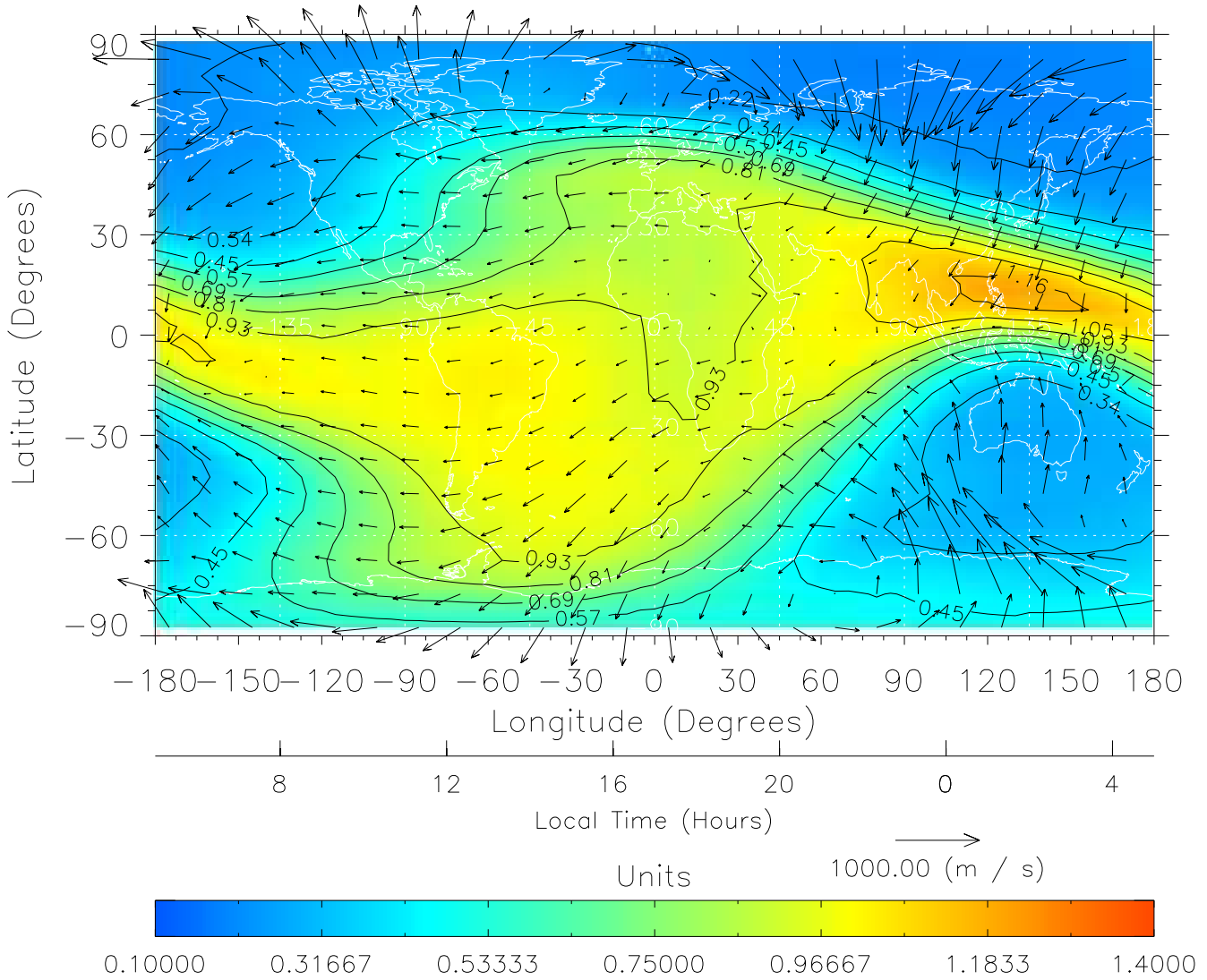
TIME-GCM MAP \Sigma O/N_2 with Neutral Wind vectors ZP = 2.00 UT = 17.00 DOY = 090
