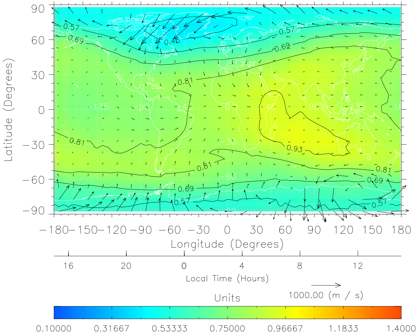
TIME-GCM MAP \Sigma O/N_2 with Neutral Wind vectors ZP = 2.00 UT = 3.00 DOY = 090
