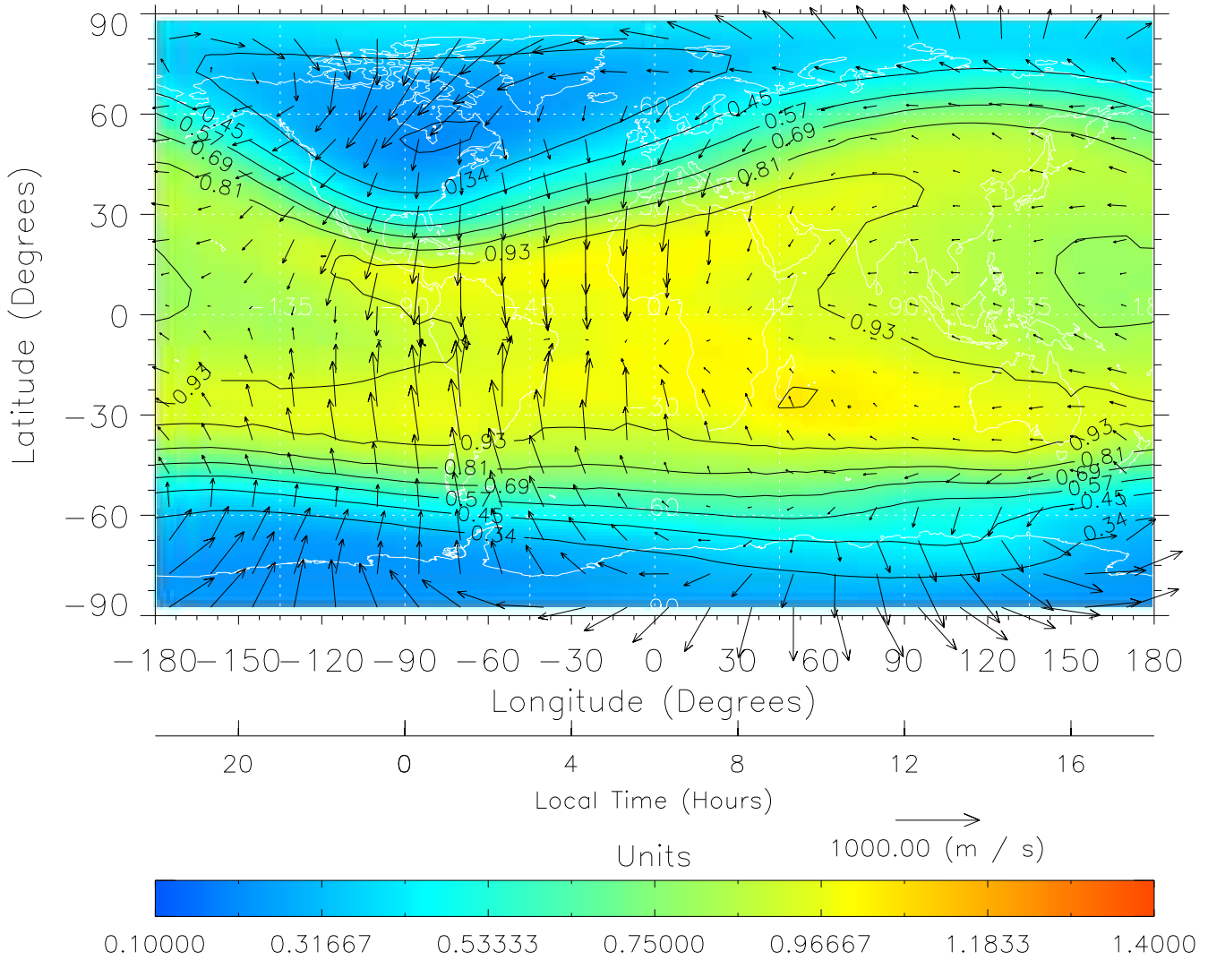
TIME-GCM MAP \Sigma O/N_2 with Neutral Wind vectors ZP = 2.00 UT = 6.00 DOY = 090
