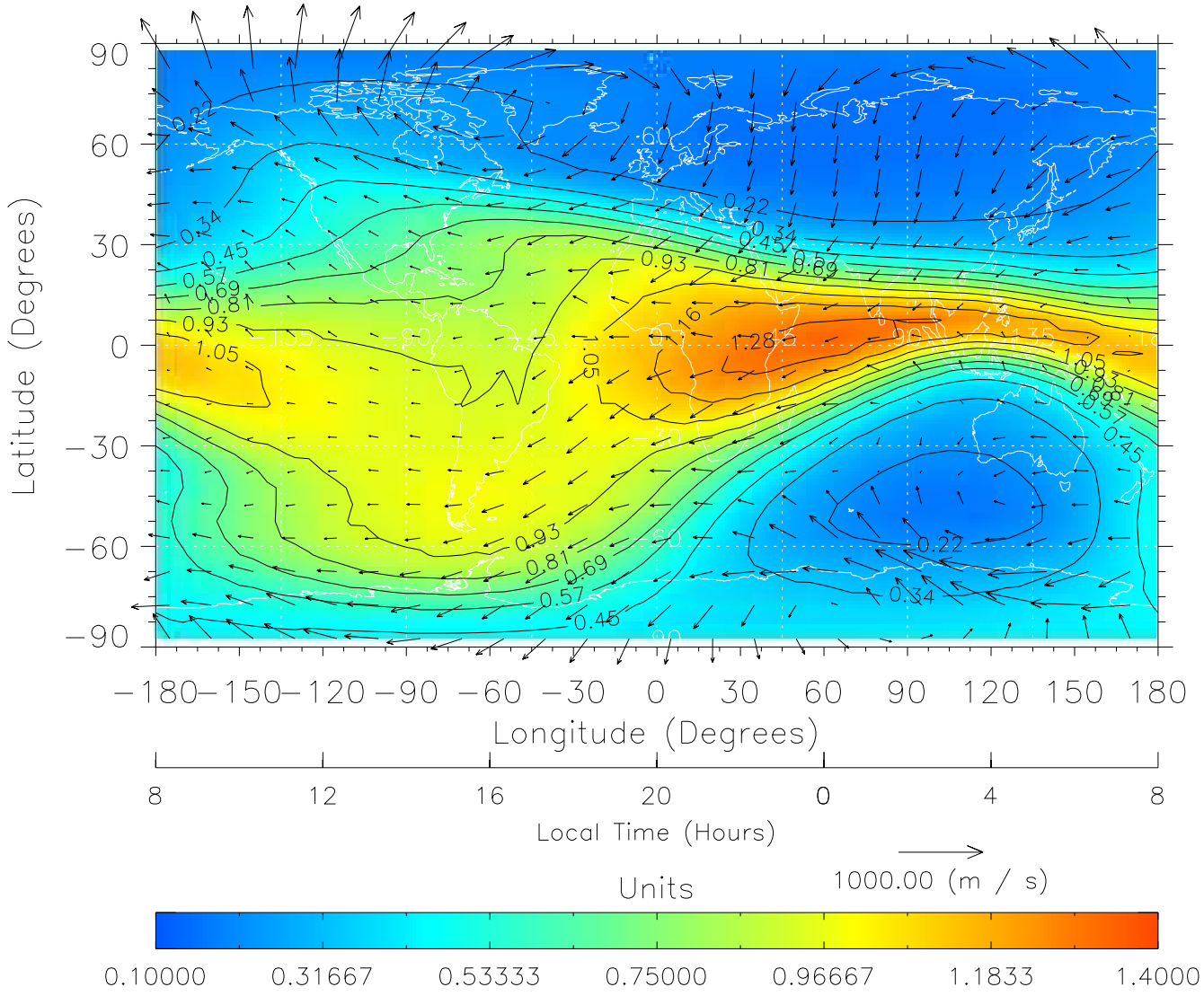
TIME-GCM MAP \Sigma O/N_2 with Neutral Wind vectors ZP = 2.00 UT = 20.00 DOY = 090
