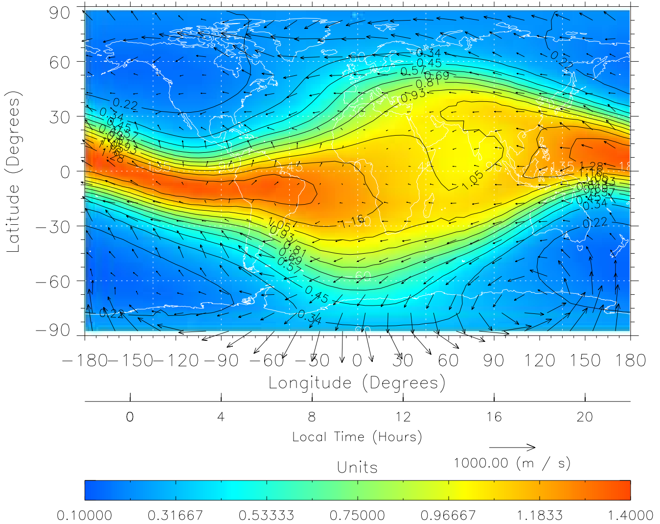
TIME-GCM MAP \Sigma O/N_2 with Neutral Wind vectors ZP = 2.00 UT = 10.00 DOY = 090
