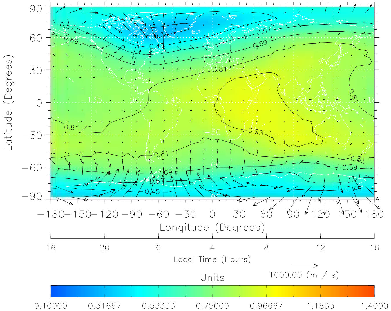
TIME-GCM MAP \Sigma O/N_2 with Neutral Wind vectors ZP = 2.00 UT = 4.00 DOY = 090
