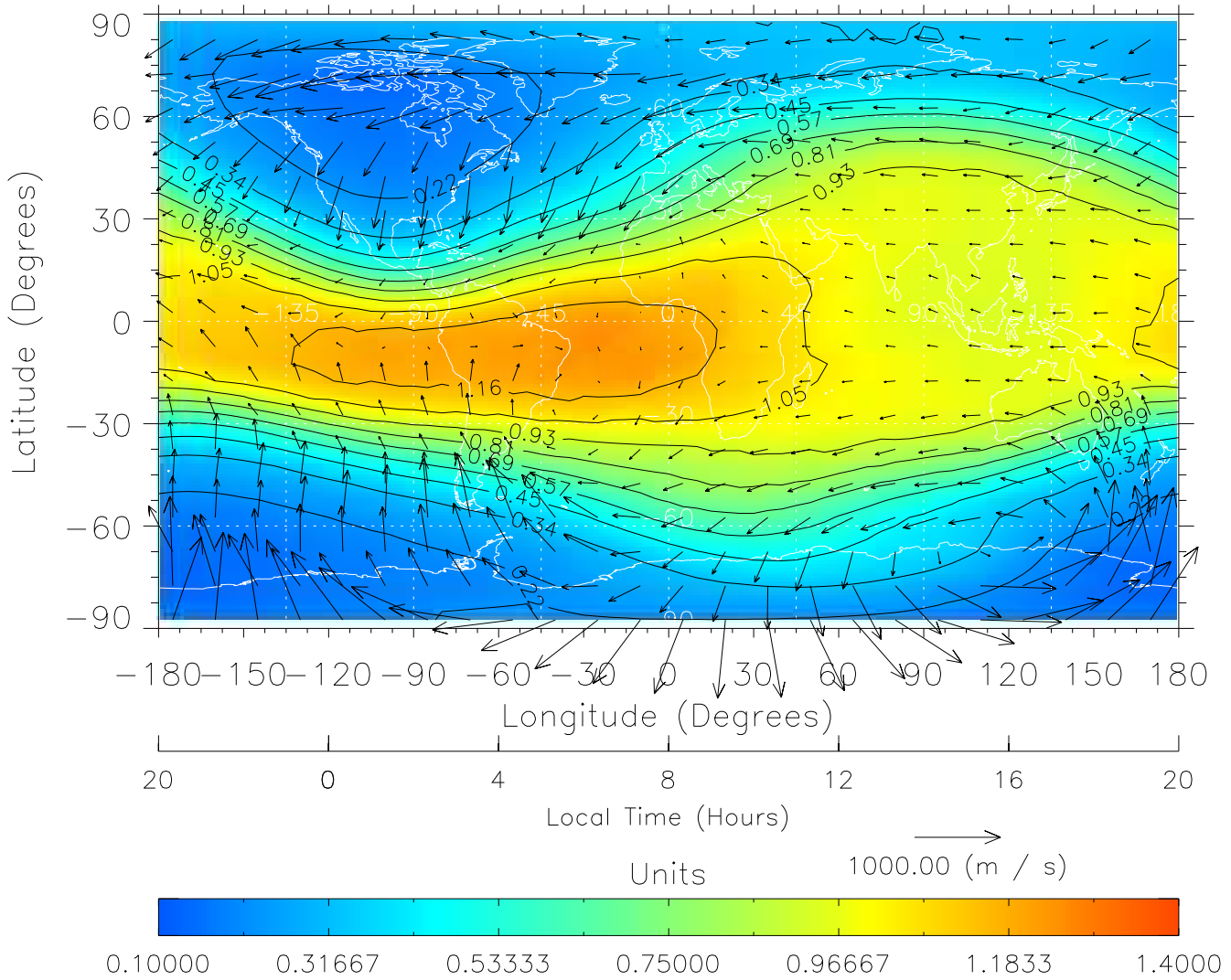
TIME-GCM MAP \Sigma O/N_2 with Neutral Wind vectors ZP = 2.00 UT = 8.00 DOY = 090
