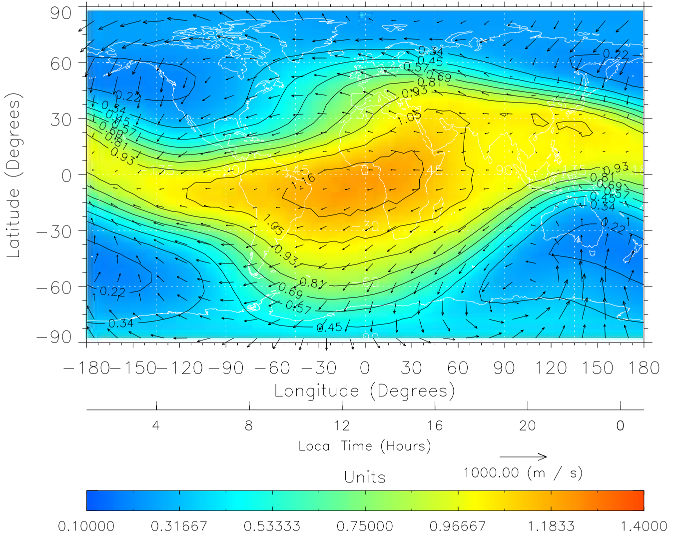
TIME-GCM MAP \Sigma O/N_2 with Neutral Wind vectors ZP = 2.00 UT = 13.00 DOY = 090
