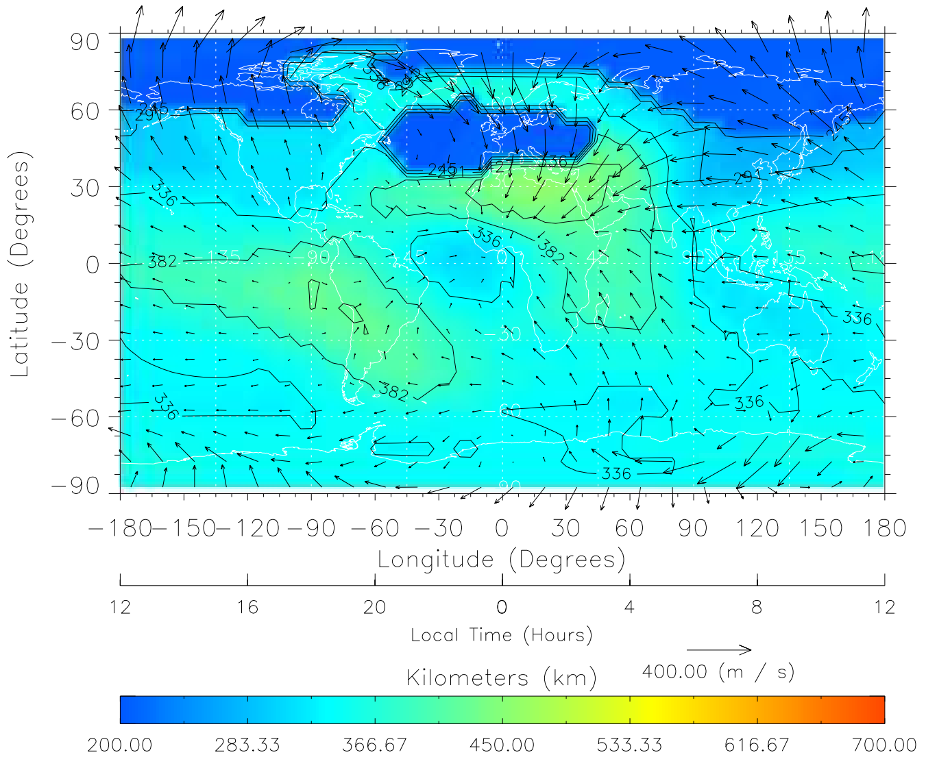
TIME-GCM MAP hmF2 with Neutral Wind vectors ZP = 2.00 UT = 0.00 DOY = 197
