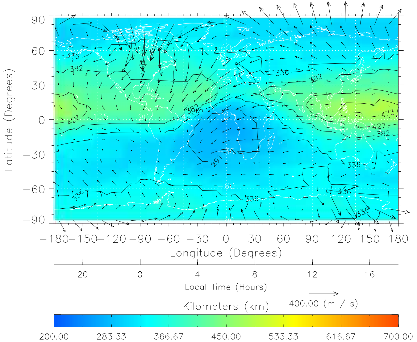
TIME-GCM MAP hmF2 with Neutral Wind vectors ZP = 2.00 UT = 6.00 DOY = 197
