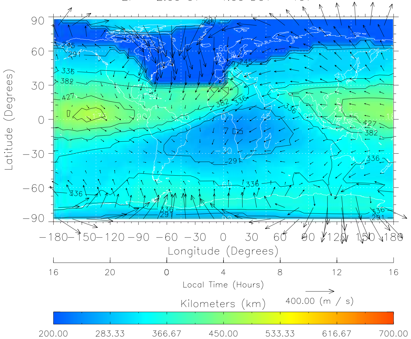
TIME-GCM MAP hmF2 with Neutral Wind vectors ZP = 2.00 UT = 4.00 DOY = 197
