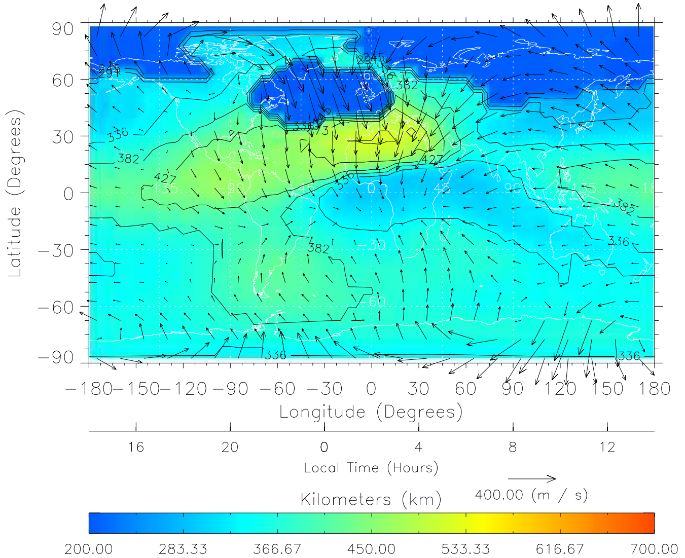
TIME-GCM MAP hmF2 with Neutral Wind vectors ZP = 2.00 UT = 2.00 DOY = 197
