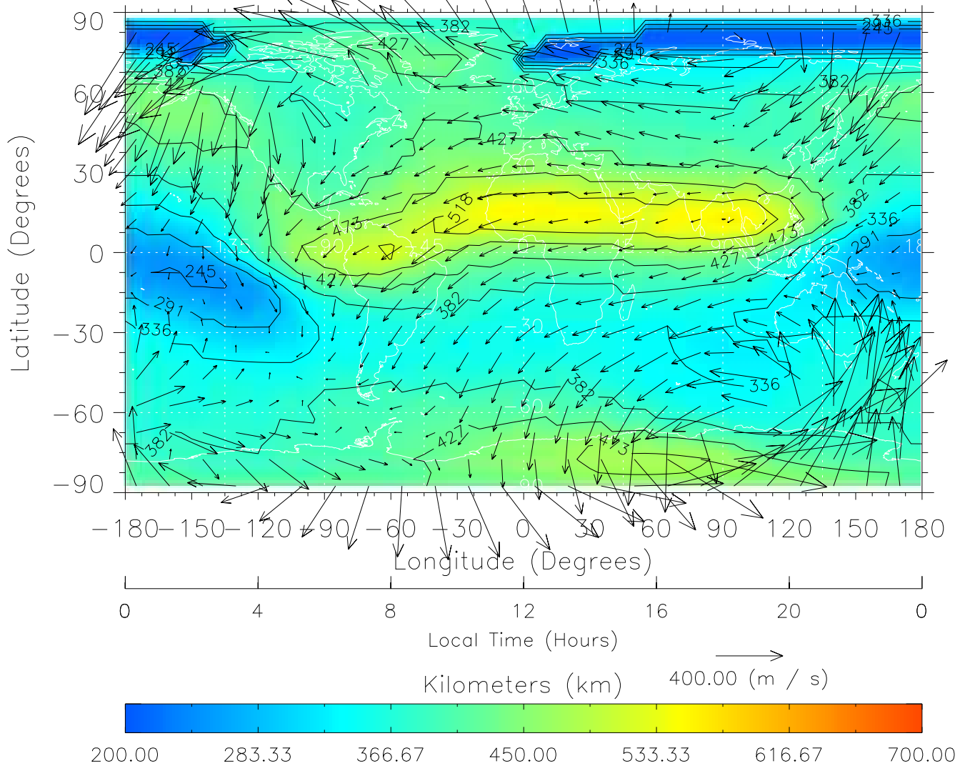
TIME-GCM MAP hmF2 with Neutral Wind vectors ZP = 2.00 UT = 12.00 DOY = 197
