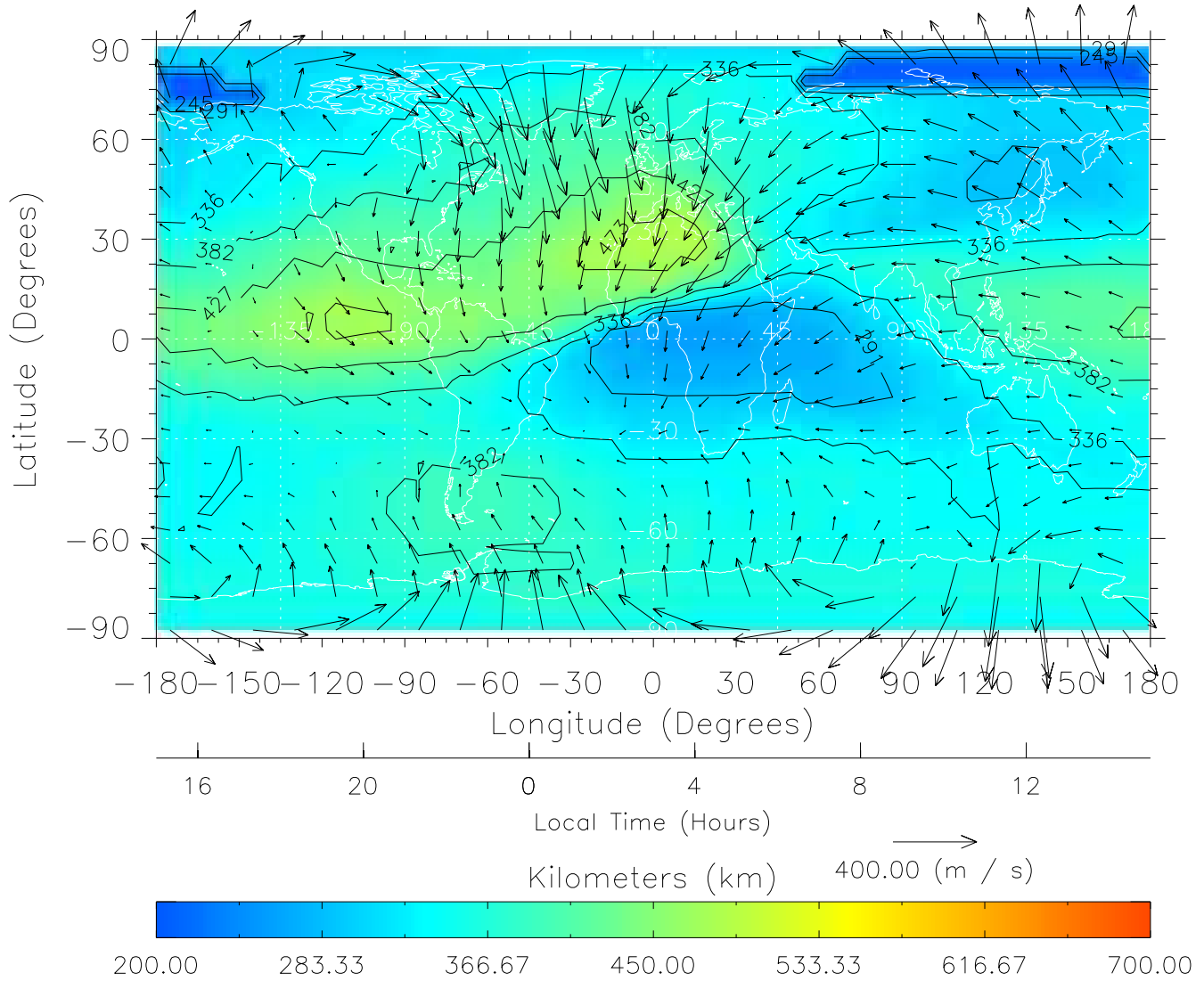
TIME-GCM MAP hmF2 with Neutral Wind vectors ZP = 2.00 UT = 3.00 DOY = 197
