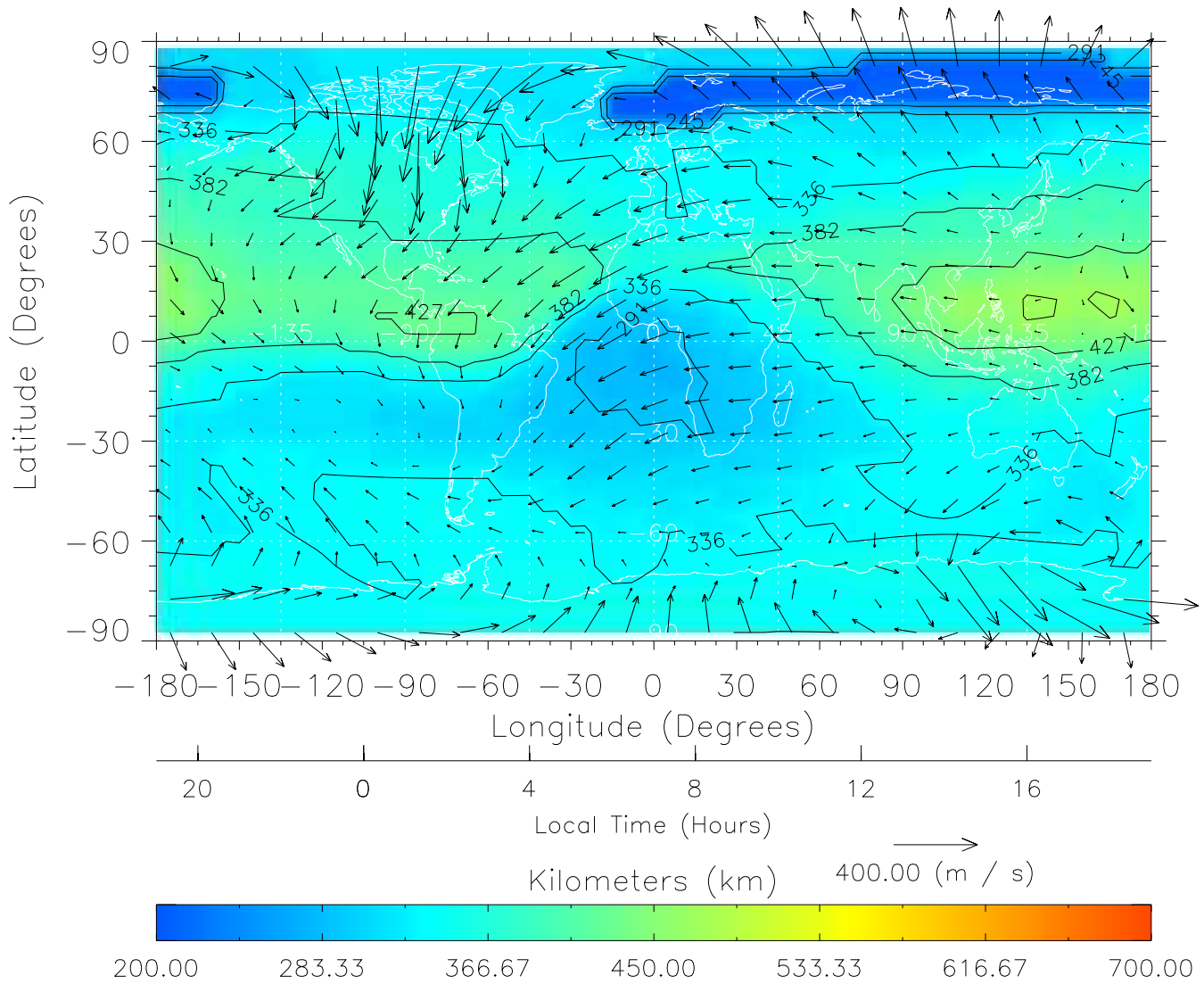
TIME-GCM MAP hmF2 with Neutral Wind vectors ZP = 2.00 UT = 7.00 DOY = 197
