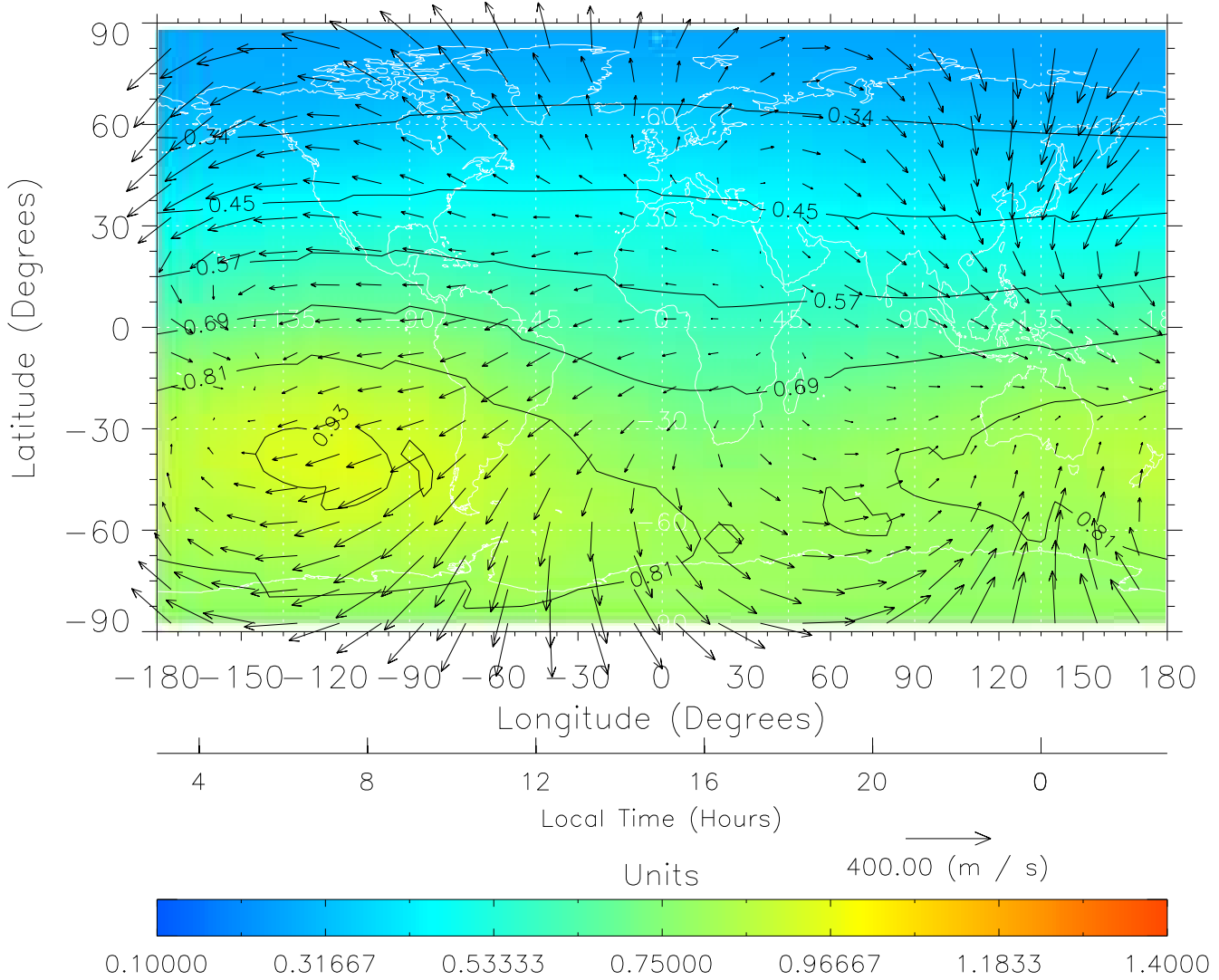
TIME-GCM MAP \Sigma O/N_2 with Neutral Wind vectors ZP = 2.00 UT = 15.00 DOY = 199
