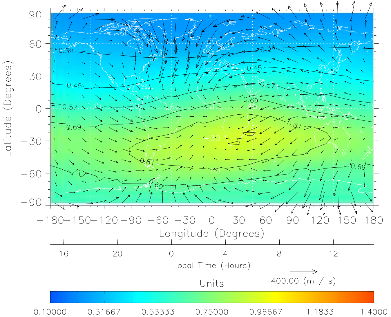
TIME-GCM MAP \Sigma O/N_2 with Neutral Wind vectors ZP = 2.00 UT = 3.00 DOY = 199
