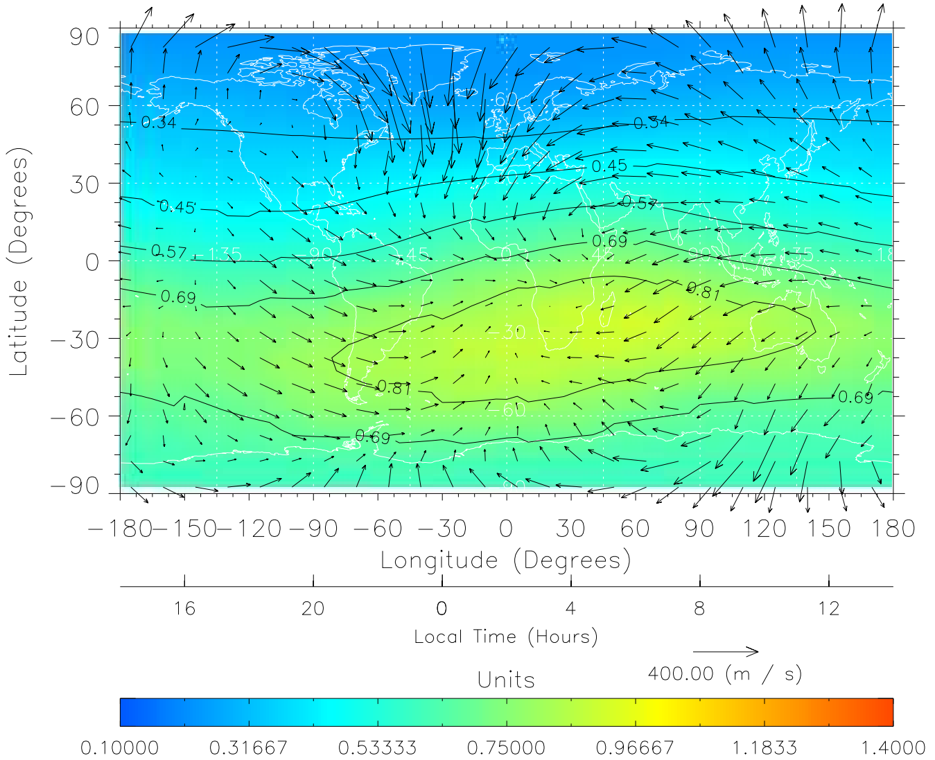
TIME-GCM MAP \Sigma O/N_2 with Neutral Wind vectors ZP = 2.00 UT = 2.00 DOY = 199
