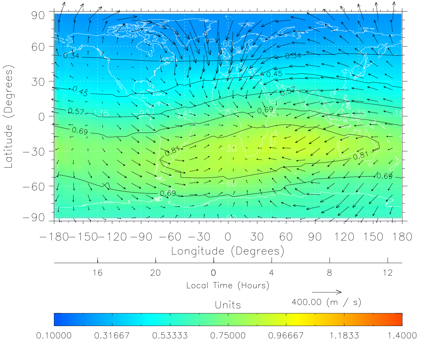
TIME-GCM MAP \Sigma O/N_2 with Neutral Wind vectors ZP = 2.00 UT = 1.00 DOY = 199
