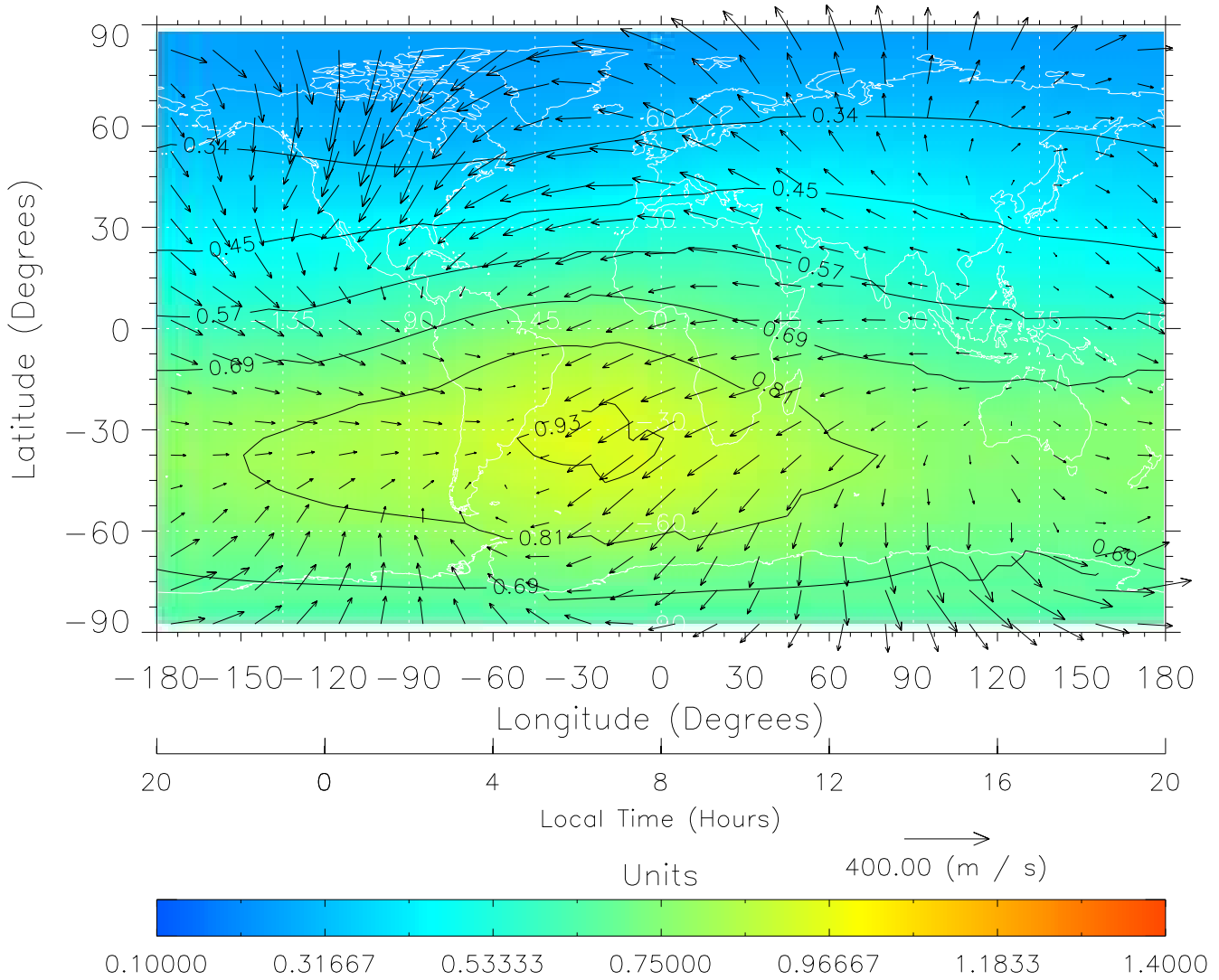
TIME-GCM MAP \Sigma O/N_2 with Neutral Wind vectors ZP = 2.00 UT = 8.00 DOY = 199
