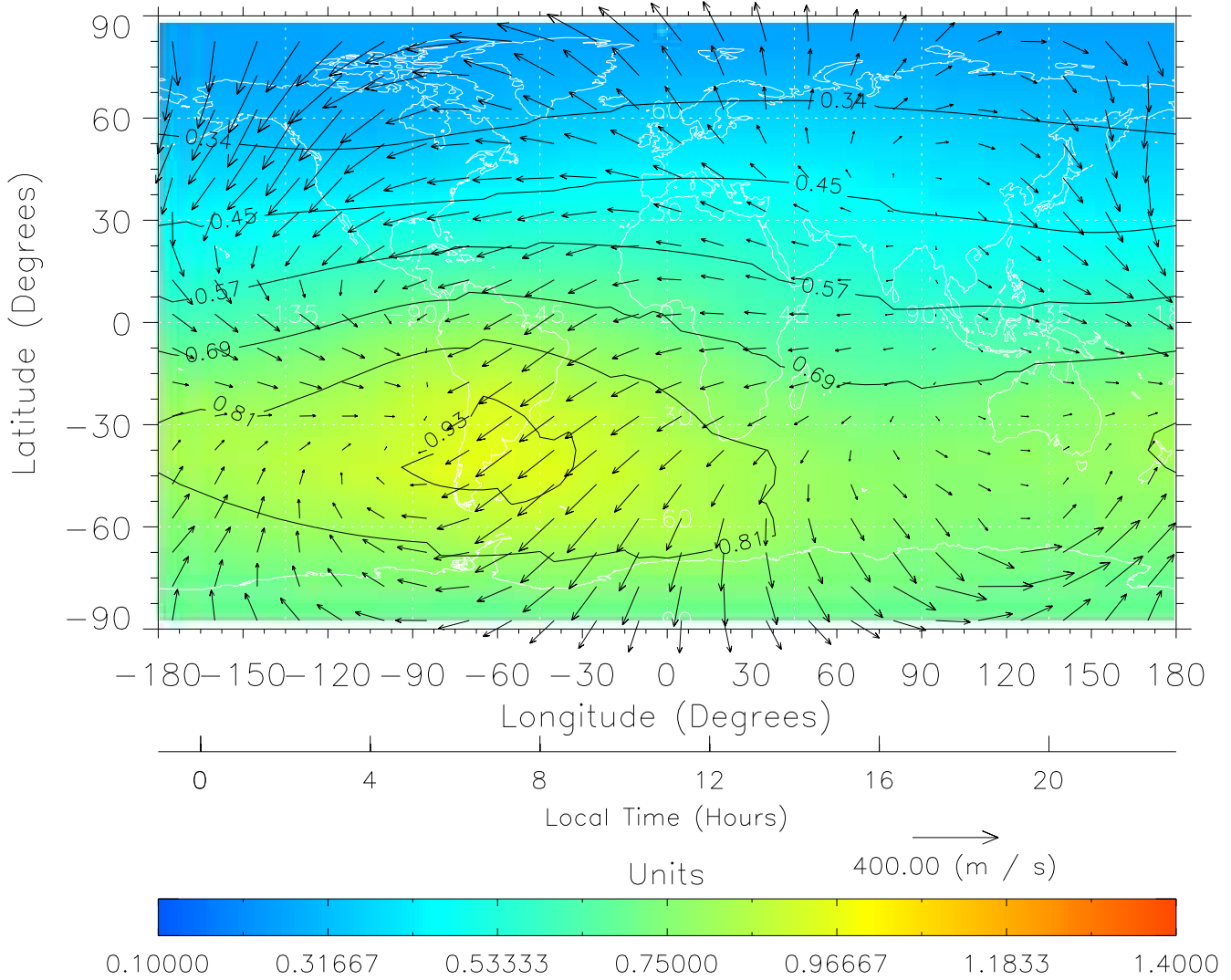
TIME-GCM MAP \Sigma O/N_2 with Neutral Wind vectors ZP = 2.00 UT = 11.00 DOY = 199
