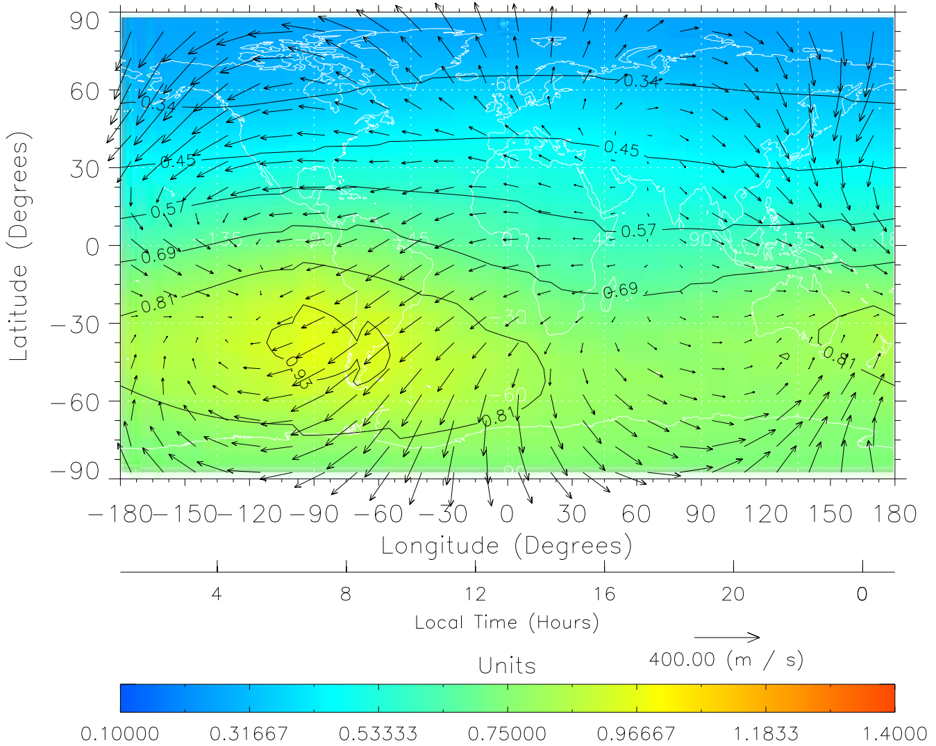
TIME-GCM MAP \Sigma O/N_2 with Neutral Wind vectors ZP = 2.00 UT = 13.00 DOY = 199
