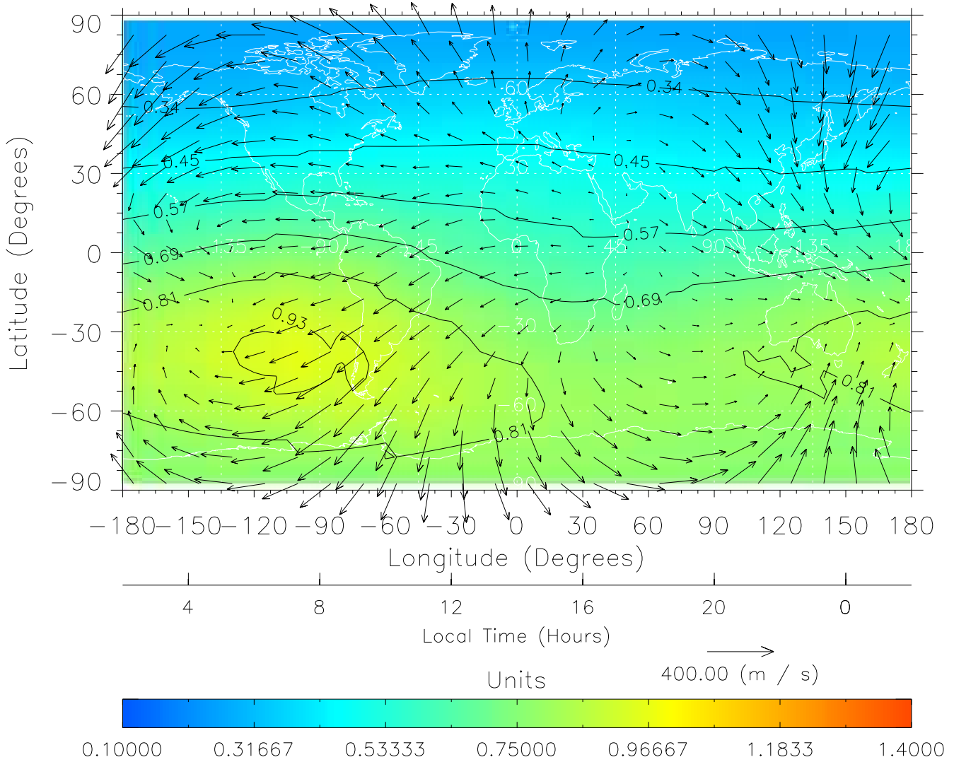
TIME-GCM MAP \Sigma O/N_2 with Neutral Wind vectors ZP = 2.00 UT = 14.00 DOY = 199
