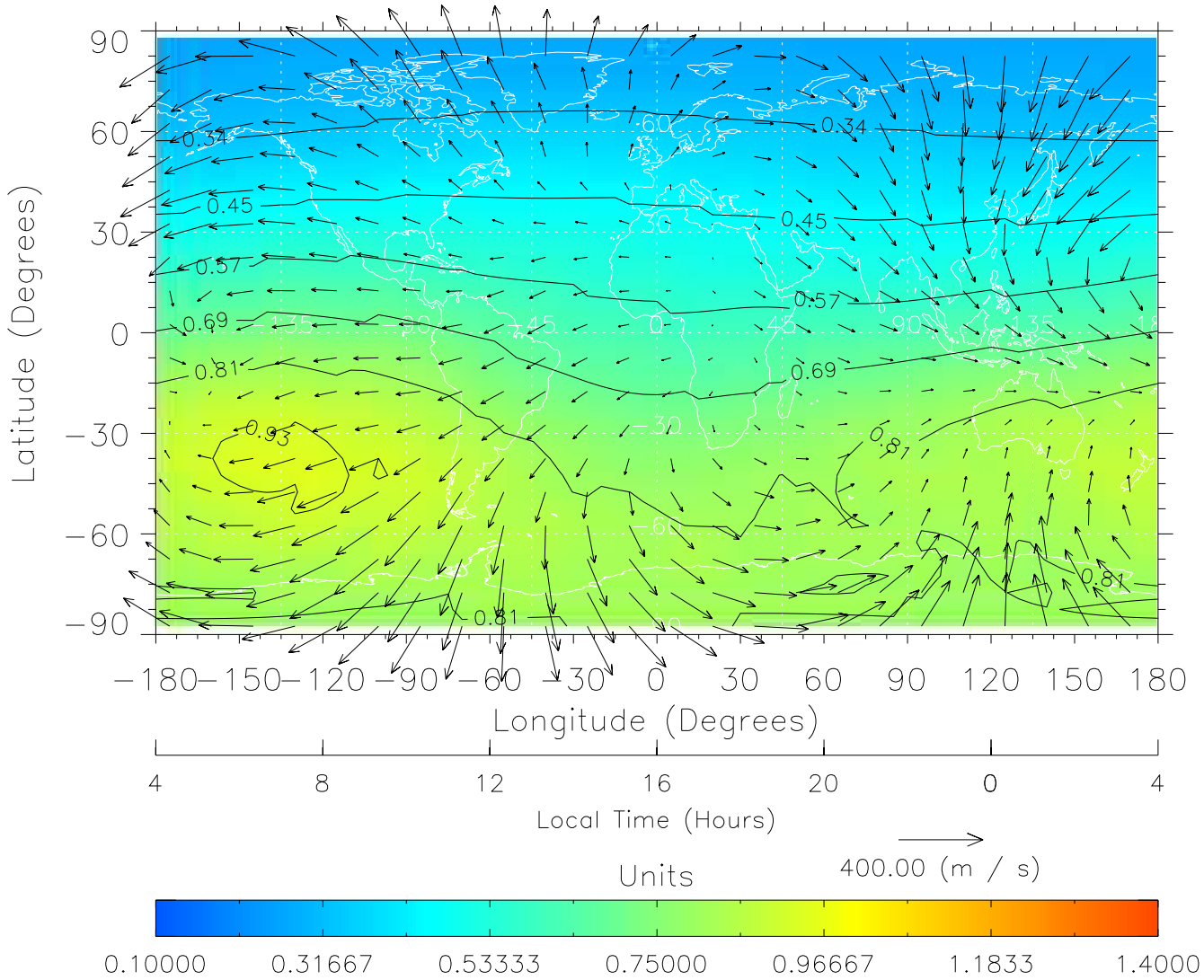
TIME-GCM MAP \Sigma O/N_2 with Neutral Wind vectors ZP = 2.00 UT = 16.00 DOY = 199
