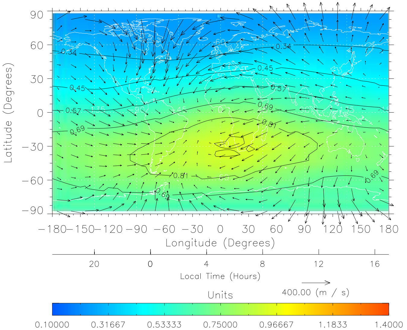
TIME-GCM MAP \Sigma O/N_2 with Neutral Wind vectors ZP = 2.00 UT = 5.00 DOY = 199
