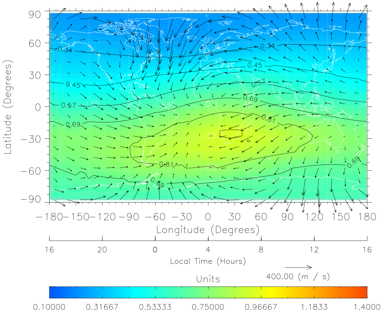
TIME-GCM MAP \Sigma O/N_2 with Neutral Wind vectors ZP = 2.00 UT = 4.00 DOY = 199
