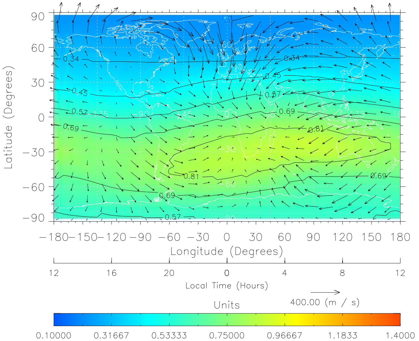
TIME-GCM MAP \Sigma O/N_2 with Neutral Wind vectors ZP = 2.00 UT = 0.00 DOY = 199
