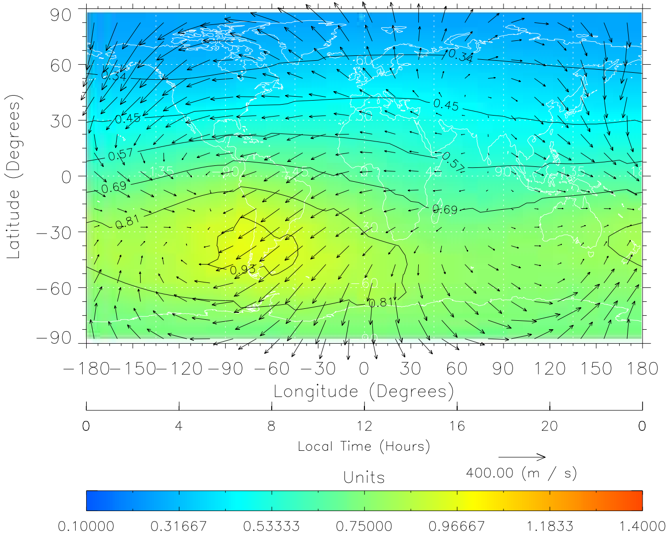
TIME-GCM MAP \Sigma O/N_2 with Neutral Wind vectors ZP = 2.00 UT = 12.00 DOY = 199
