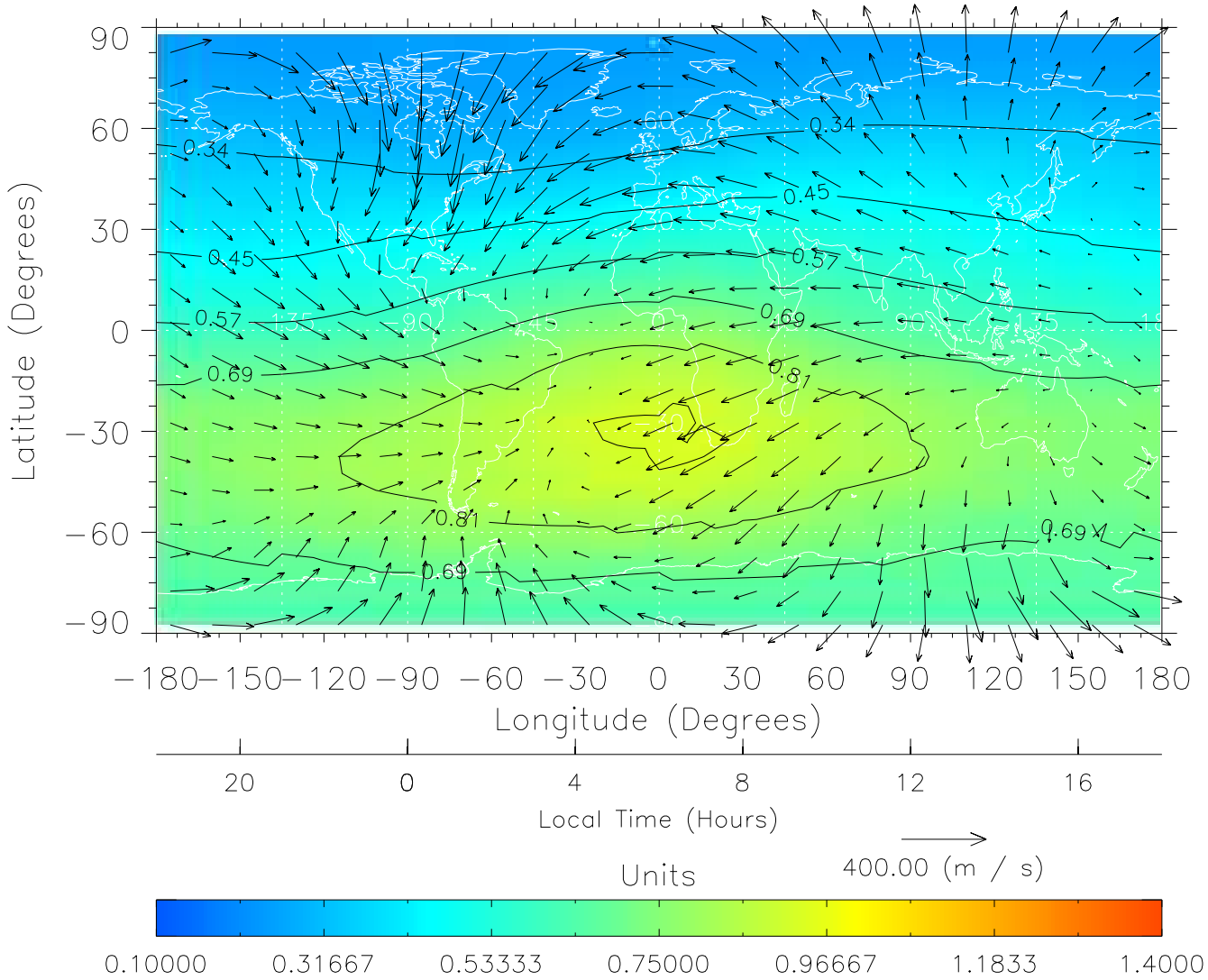
TIME-GCM MAP \Sigma O/N_2 with Neutral Wind vectors ZP = 2.00 UT = 6.00 DOY = 199
