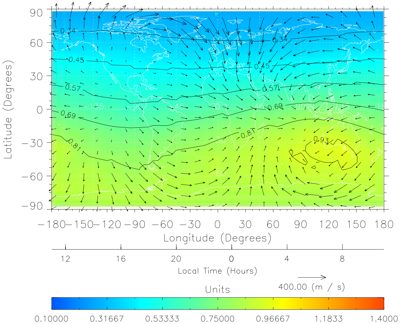
TIME-GCM MAP \Sigma O/N_2 with Neutral Wind vectors ZP = 2.00 UT = 23.00 DOY = 199
