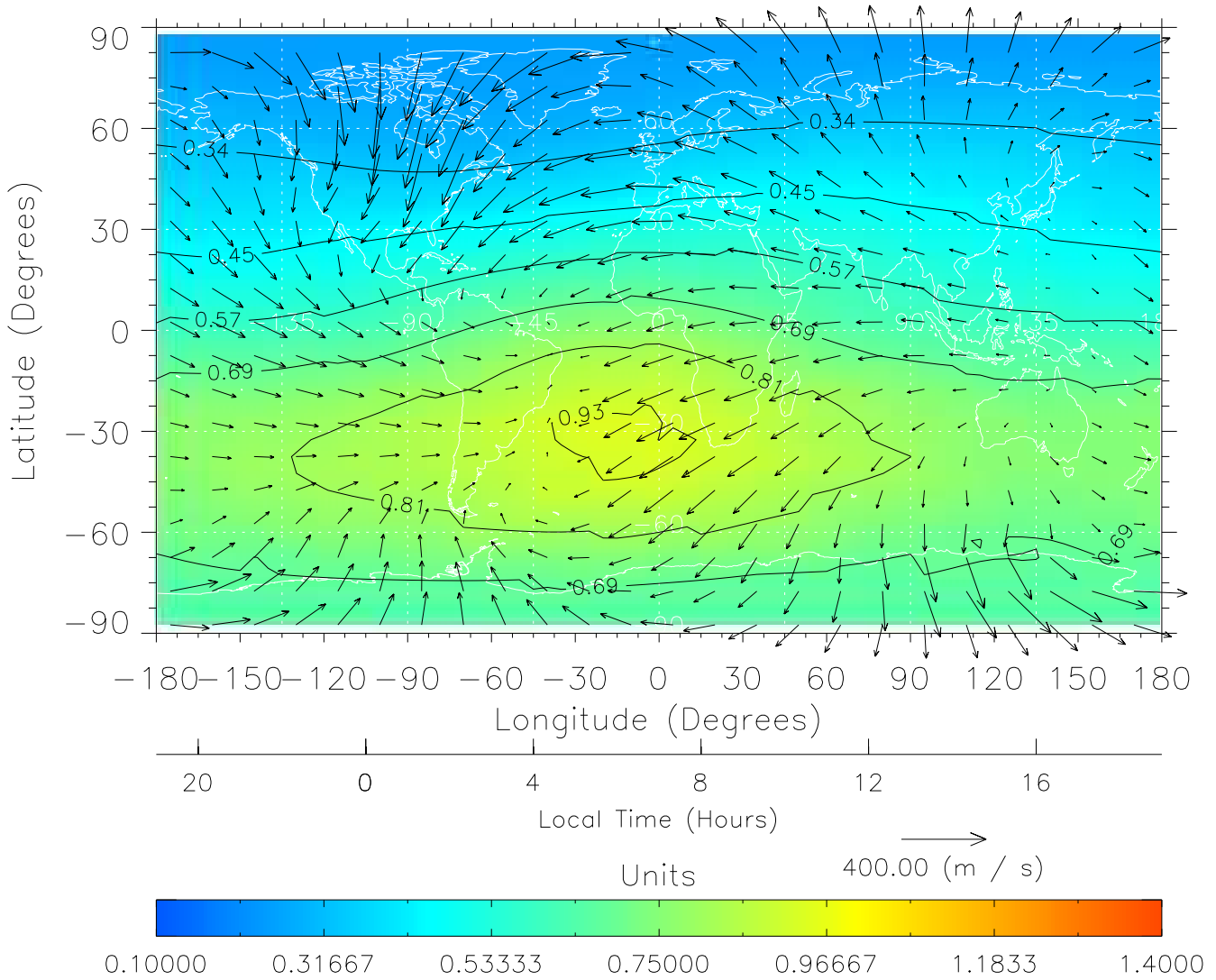
TIME-GCM MAP \Sigma O/N_2 with Neutral Wind vectors ZP = 2.00 UT = 7.00 DOY = 199
