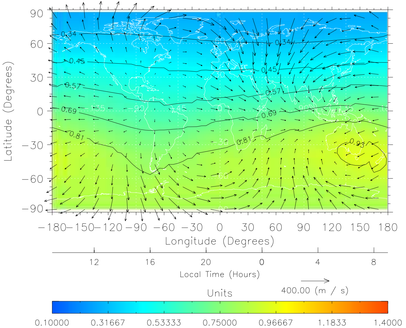
TIME-GCM MAP \Sigma O/N_2 with Neutral Wind vectors ZP = 2.00 UT = 21.00 DOY = 199
