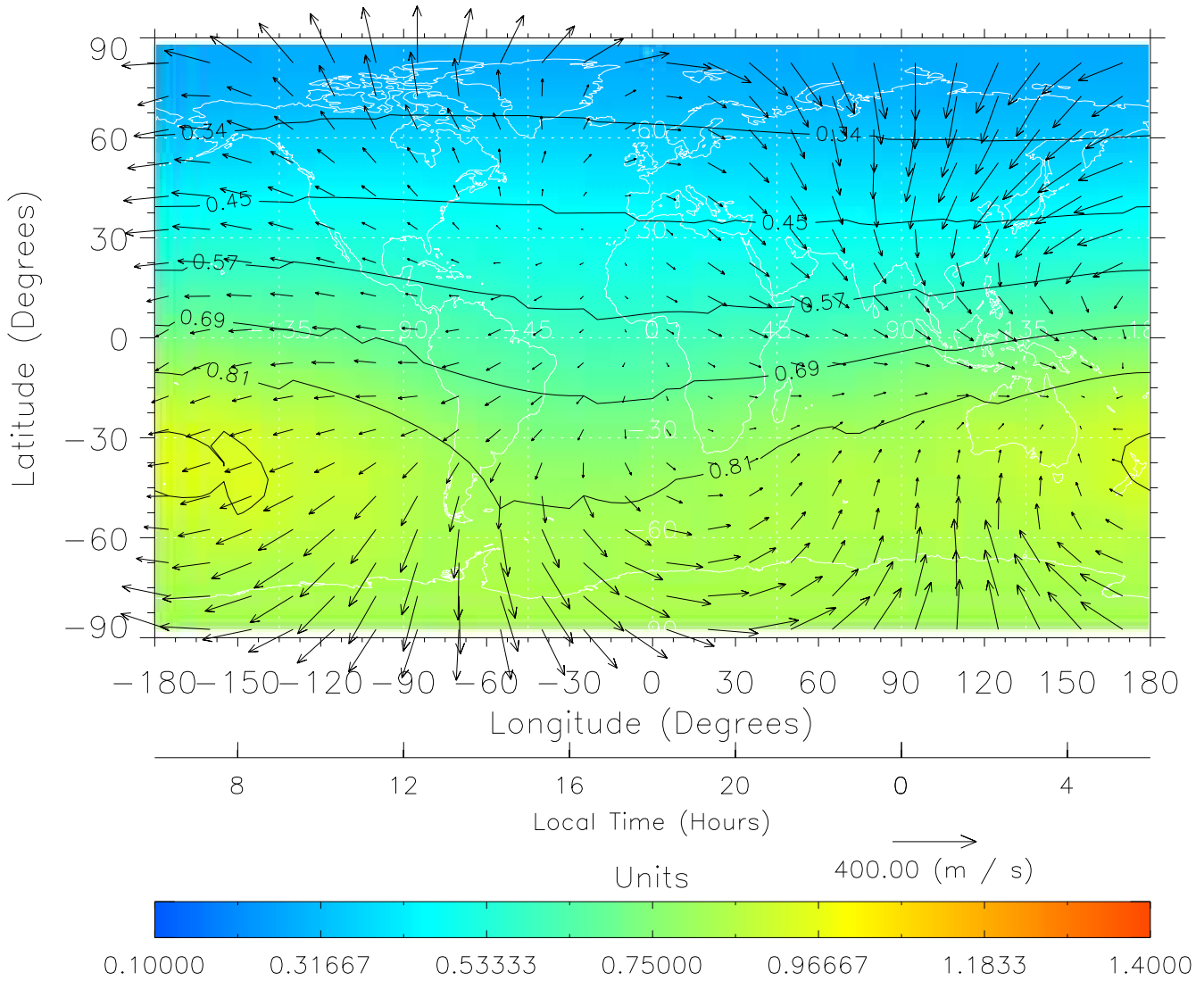
TIME-GCM MAP \Sigma O/N_2 with Neutral Wind vectors ZP = 2.00 UT = 18.00 DOY = 199
