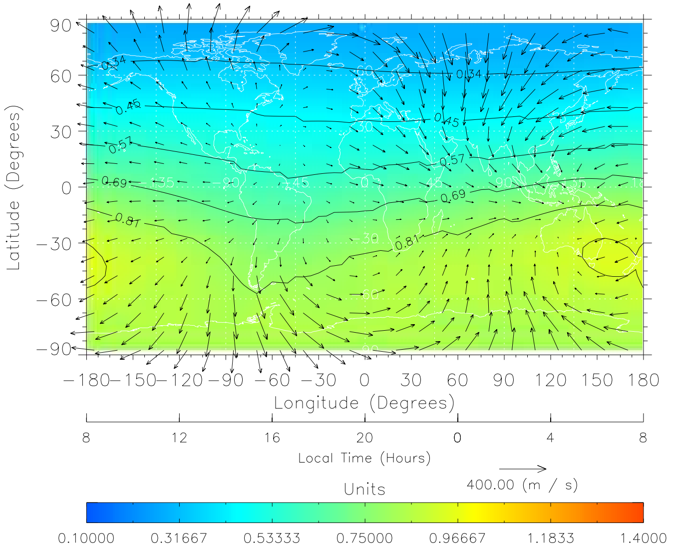
TIME-GCM MAP \Sigma O/N_2 with Neutral Wind vectors ZP = 2.00 UT = 20.00 DOY = 199
