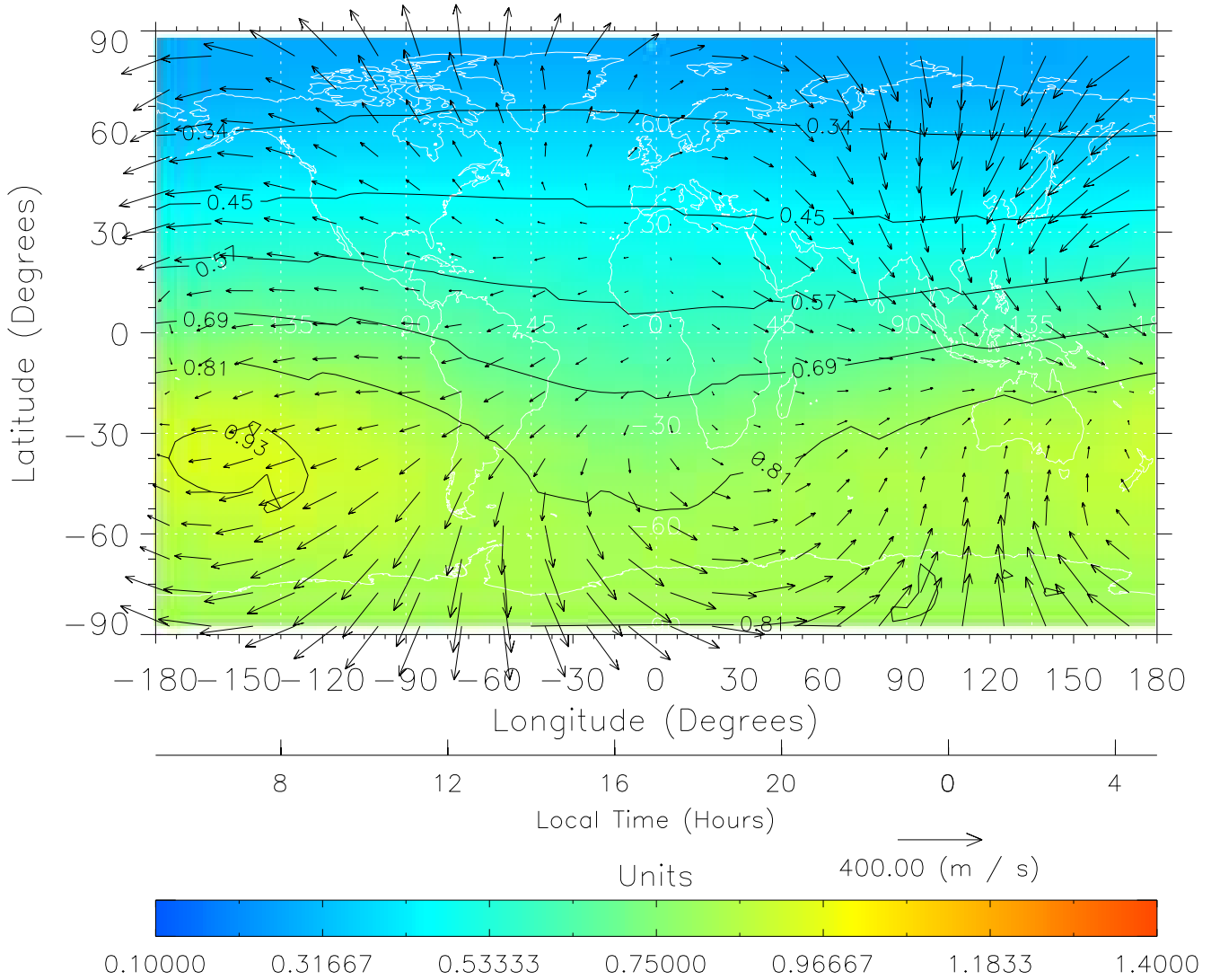
TIME-GCM MAP \Sigma O/N_2 with Neutral Wind vectors ZP = 2.00 UT = 17.00 DOY = 199
