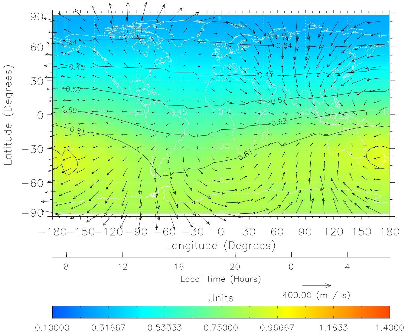
TIME-GCM MAP \Sigma O/N_2 with Neutral Wind vectors ZP = 2.00 UT = 19.00 DOY = 199
