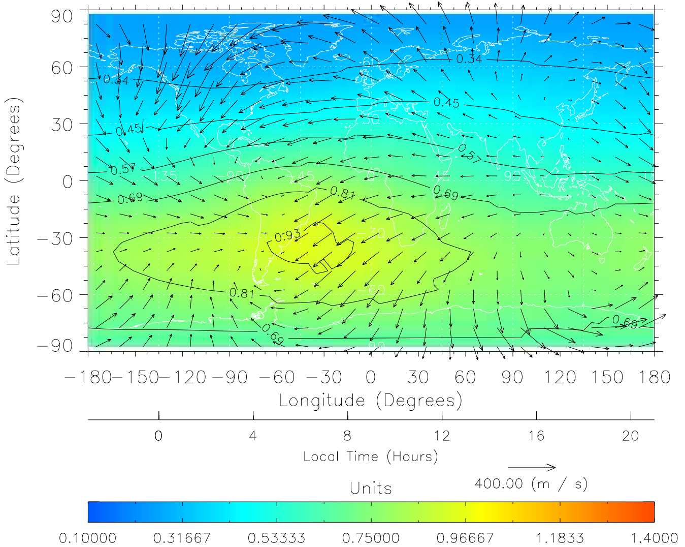
TIME-GCM MAP \Sigma O/N_2 with Neutral Wind vectors ZP = 2.00 UT = 9.00 DOY = 199
