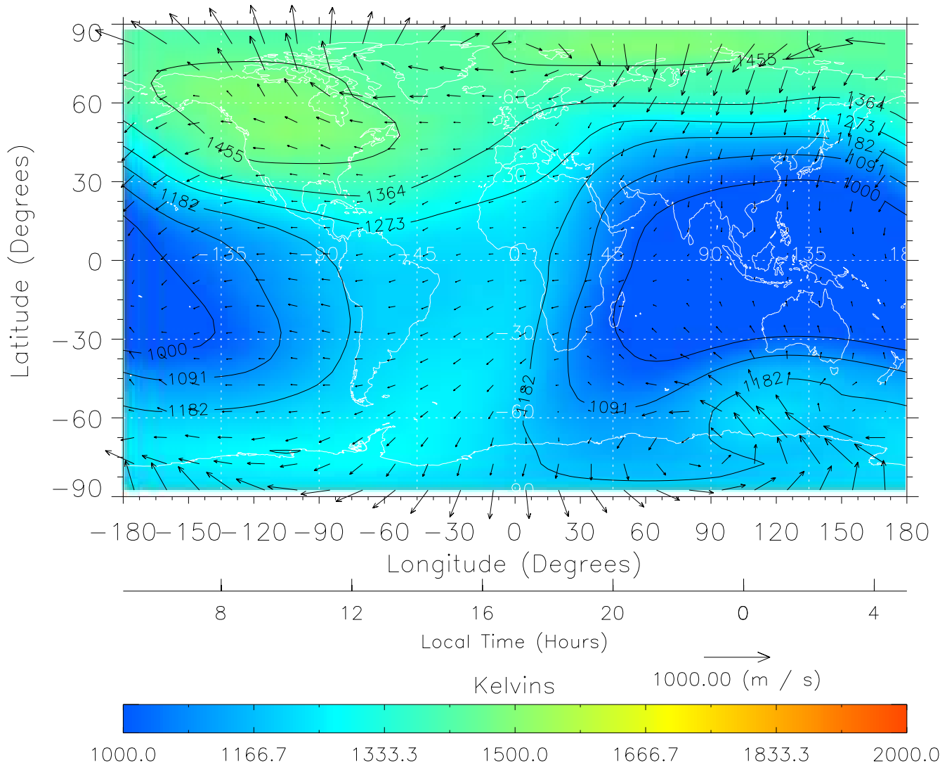
TIME-GCM MAP Temperature with Neutral Wind vectors ZP = 2.00 UT = 17.00 DOY = 110
