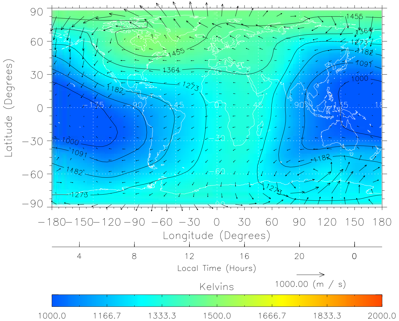
TIME-GCM MAP Temperature with Neutral Wind vectors ZP = 2.00 UT = 14.00 DOY = 108
