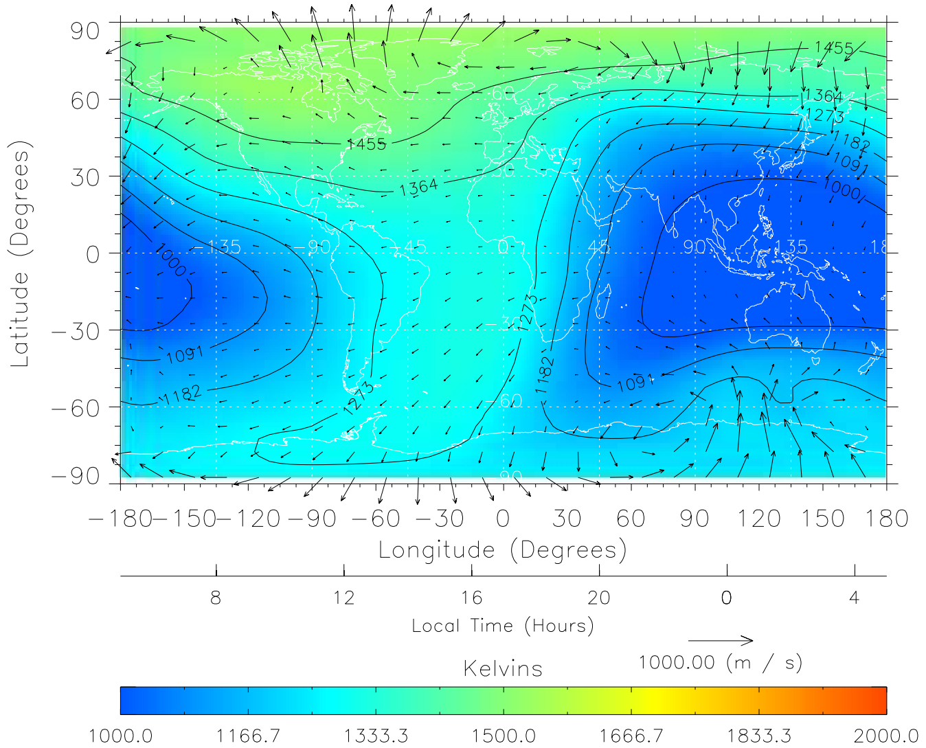
TIME-GCM MAP Temperature with Neutral Wind vectors ZP = 2.00 UT = 17.00 DOY = 108
