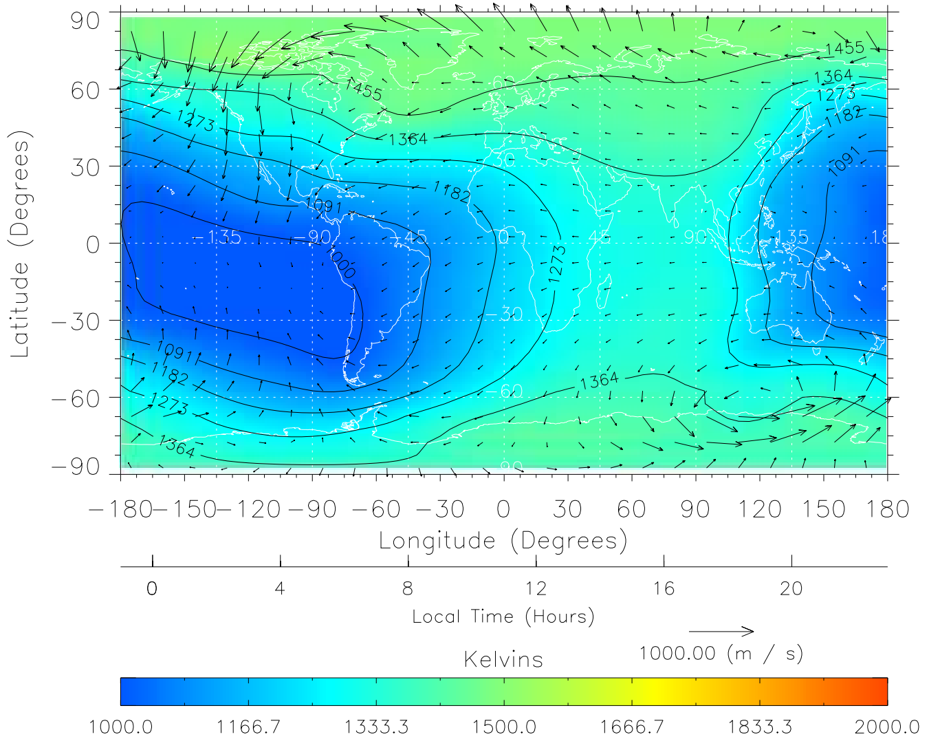
TIME-GCM MAP Temperature with Neutral Wind vectors ZP = 2.00 UT = 11.00 DOY = 108
