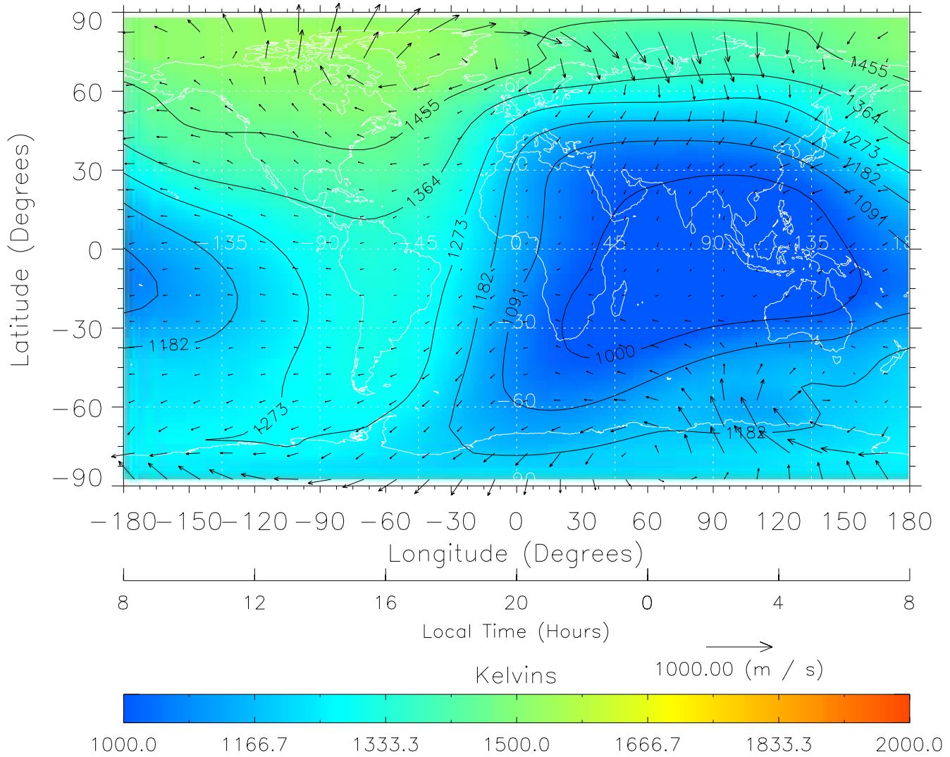
TIME-GCM MAP Temperature with Neutral Wind vectors ZP = 2.00 UT = 20.00 DOY = 108
