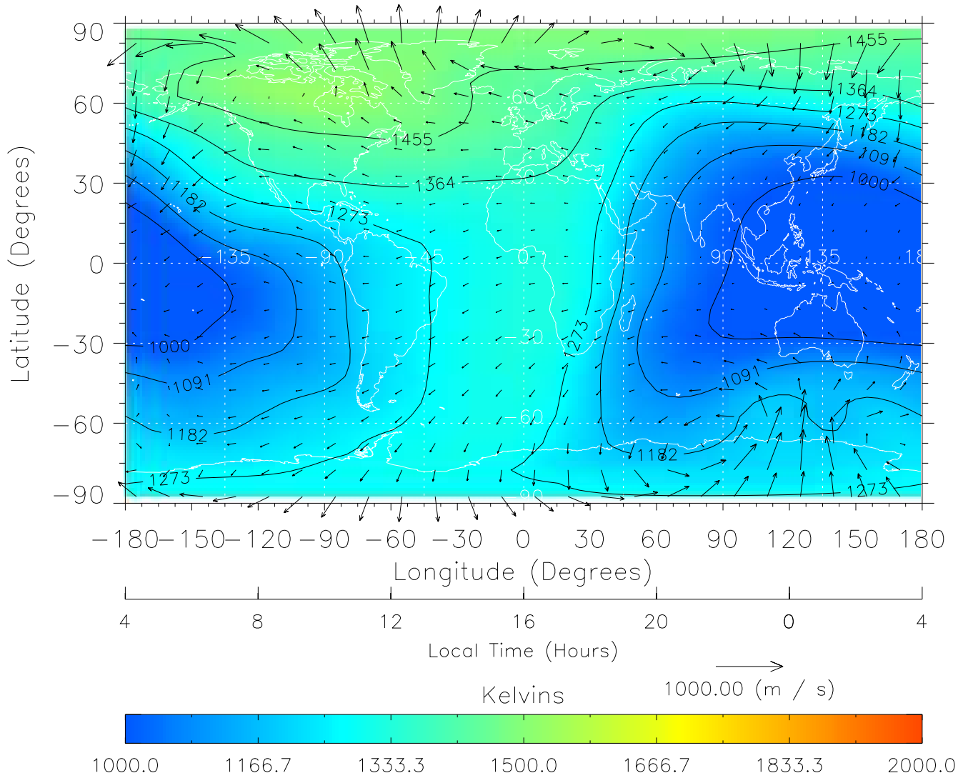
TIME-GCM MAP Temperature with Neutral Wind vectors ZP = 2.00 UT = 16.00 DOY = 108
