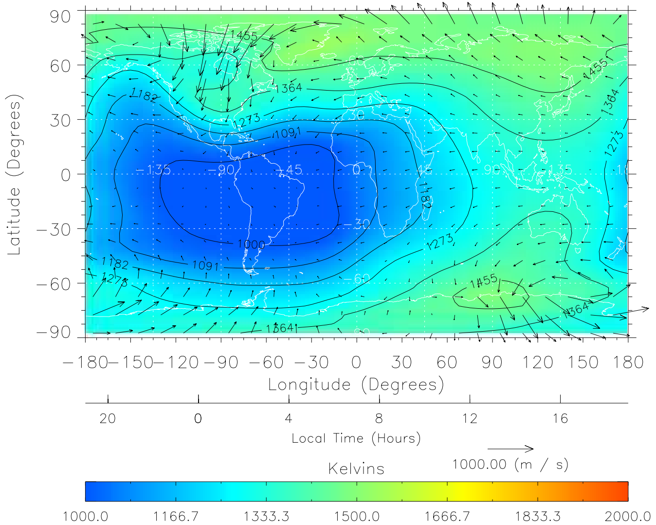
TIME-GCM MAP Temperature with Neutral Wind vectors ZP = 2.00 UT = 7.00 DOY = 108
