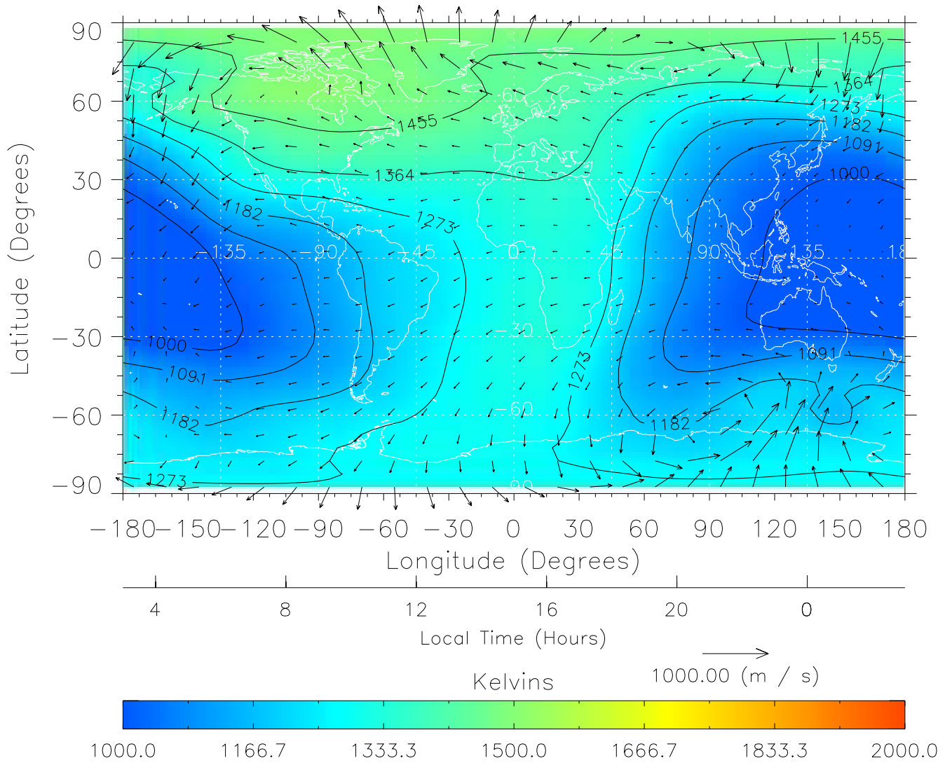
TIME-GCM MAP Temperature with Neutral Wind vectors ZP = 2.00 UT = 15.00 DOY = 108
