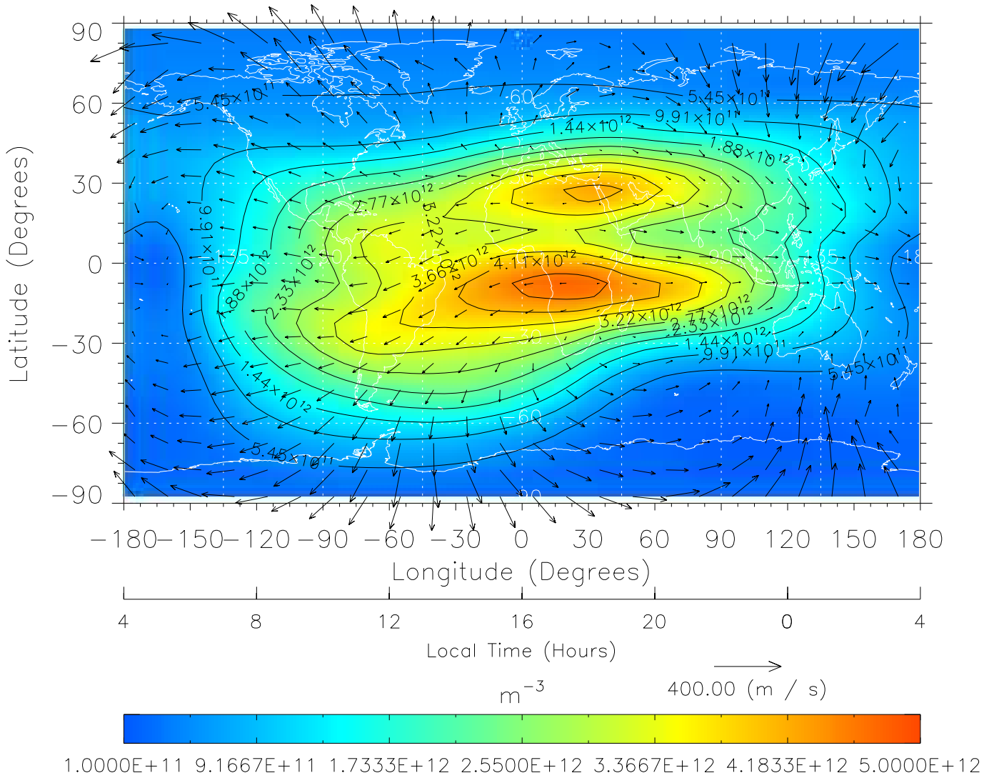
TIME-GCM MAP NmF2 with Neutral Wind vectors ZP = 2.00 UT = 16.00 DOY = 111
