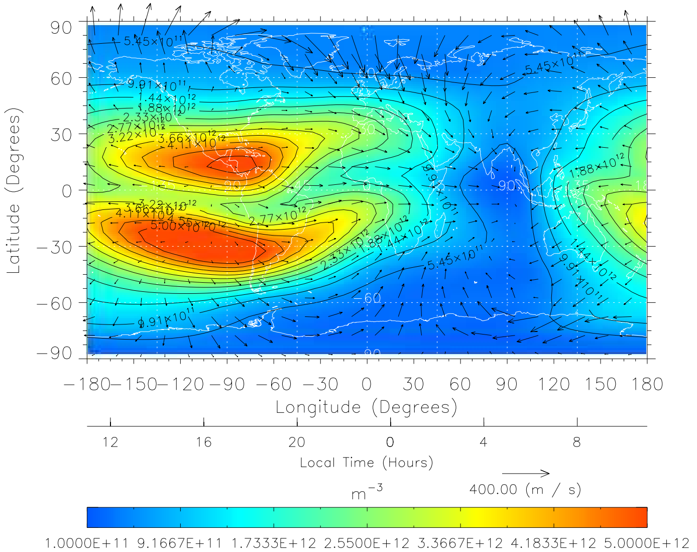
TIME-GCM MAP NmF2 with Neutral Wind vectors ZP = 2.00 UT = 23.00 DOY = 111
