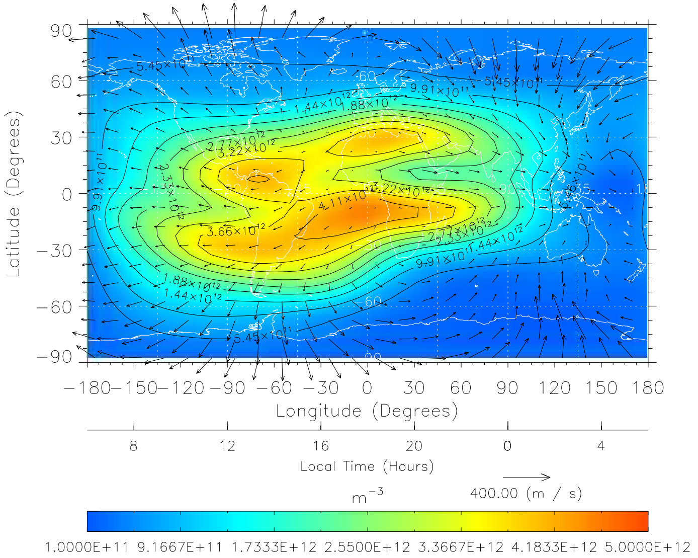
TIME-GCM MAP NmF2 with Neutral Wind vectors ZP = 2.00 UT = 18.00 DOY = 111
