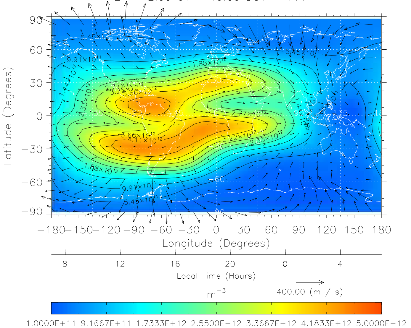
TIME-GCM MAP NmF2 with Neutral Wind vectors ZP = 2.00 UT = 19.00 DOY = 111
