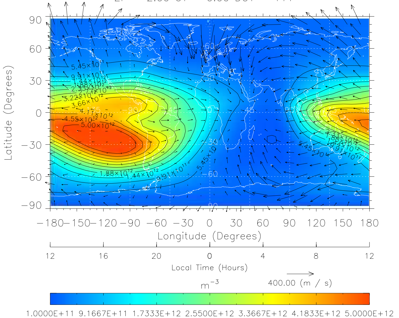
TIME-GCM MAP NmF2 with Neutral Wind vectors ZP = 2.00 UT = 0.00 DOY = 111
