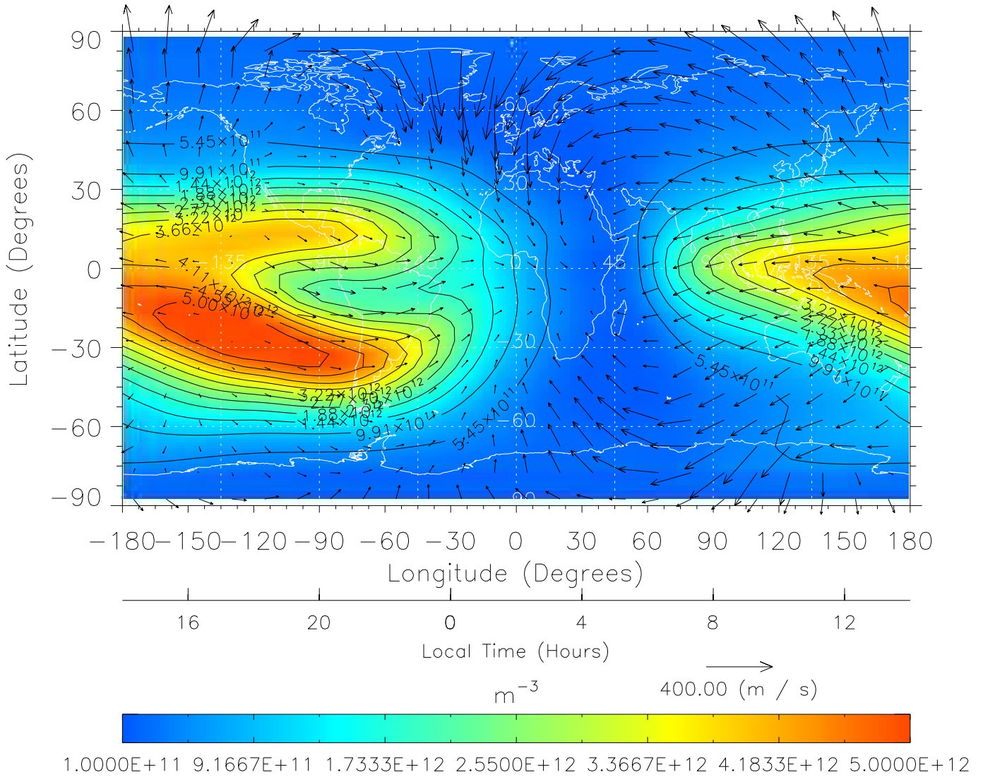
TIME-GCM MAP NmF2 with Neutral Wind vectors ZP = 2.00 UT = 2.00 DOY = 111
