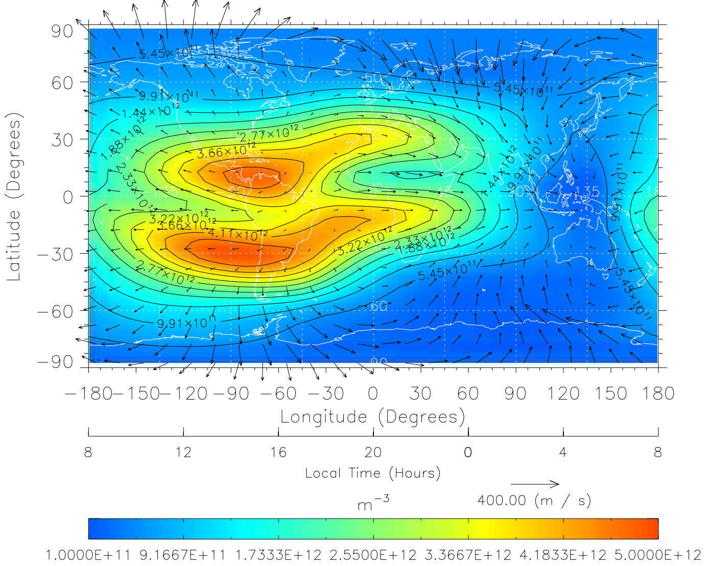
TIME-GCM MAP NmF2 with Neutral Wind vectors ZP = 2.00 UT = 20.00 DOY = 111
