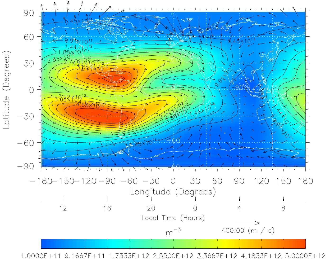
TIME-GCM MAP NmF2 with Neutral Wind vectors ZP = 2.00 UT = 22.00 DOY = 111
