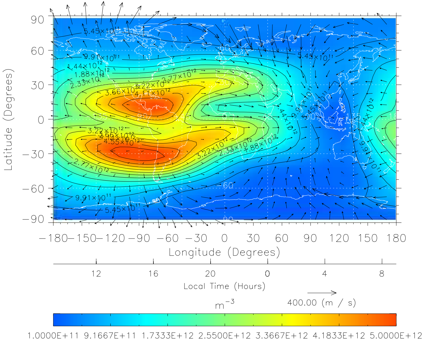
TIME-GCM MAP NmF2 with Neutral Wind vectors ZP = 2.00 UT = 21.00 DOY = 111
