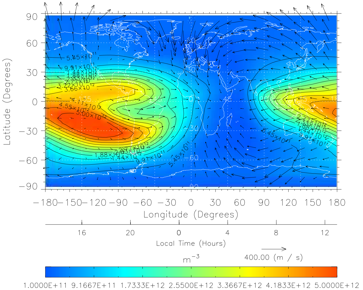
TIME-GCM MAP NmF2 with Neutral Wind vectors ZP = 2.00 UT = 1.00 DOY = 111
