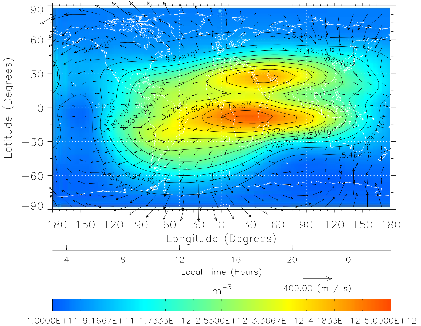
TIME-GCM MAP NmF2 with Neutral Wind vectors ZP = 2.00 UT = 15.00 DOY = 111
