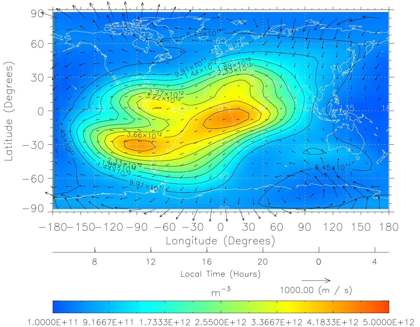
TIME-GCM MAP NmF2 with Neutral Wind vectors ZP = 2.00 UT = 17.00 DOY = 110
