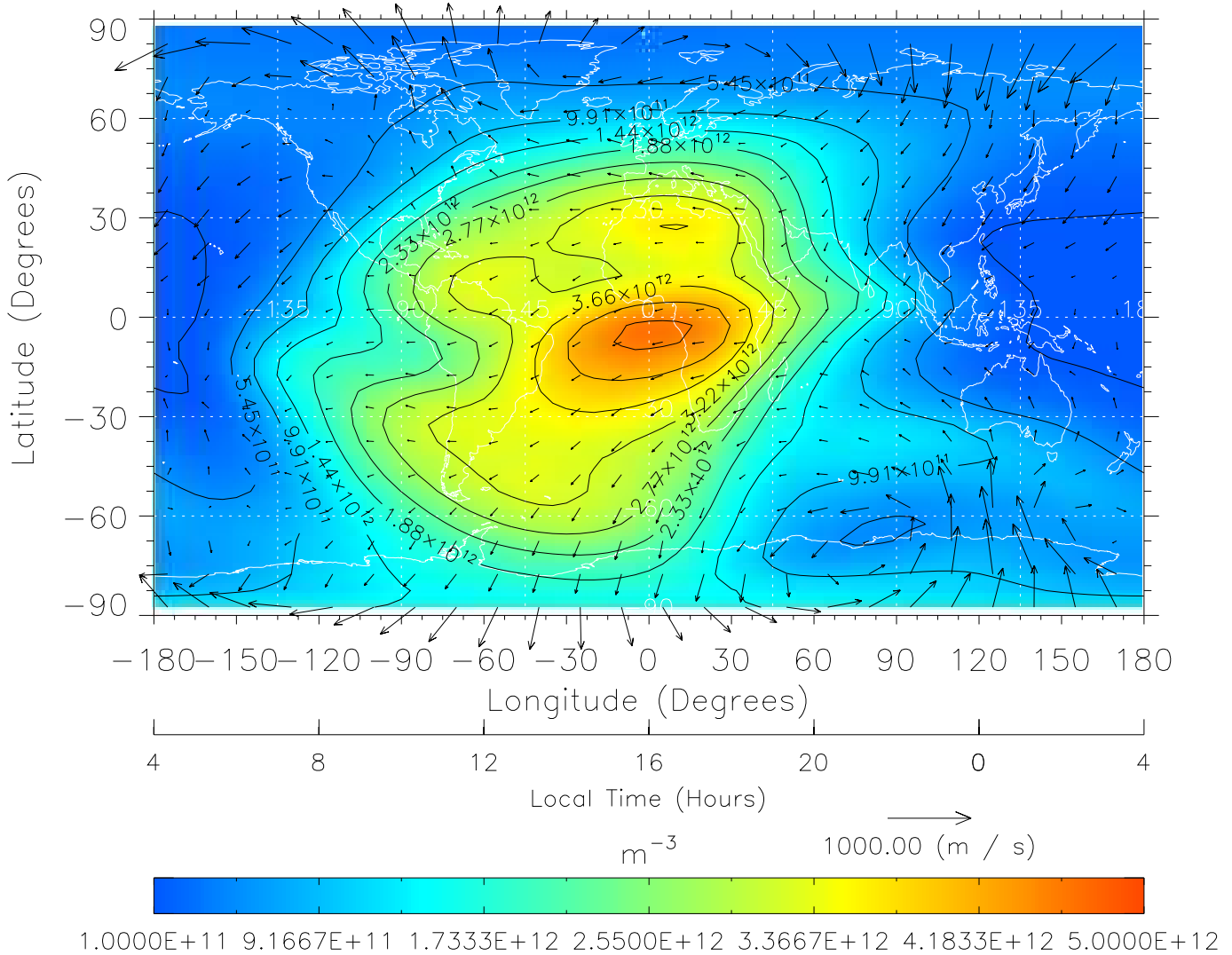
TIME-GCM MAP NmF2 with Neutral Wind vectors ZP = 2.00 UT = 16.00 DOY = 109
