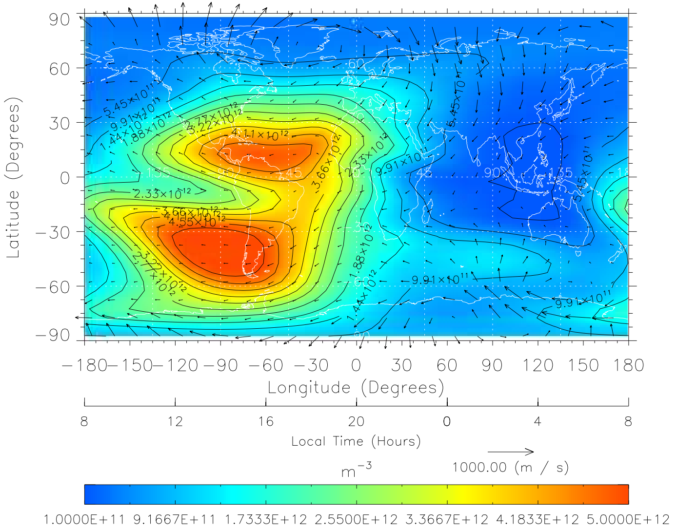
TIME-GCM MAP NmF2 with Neutral Wind vectors ZP = 2.00 UT = 20.00 DOY = 109
