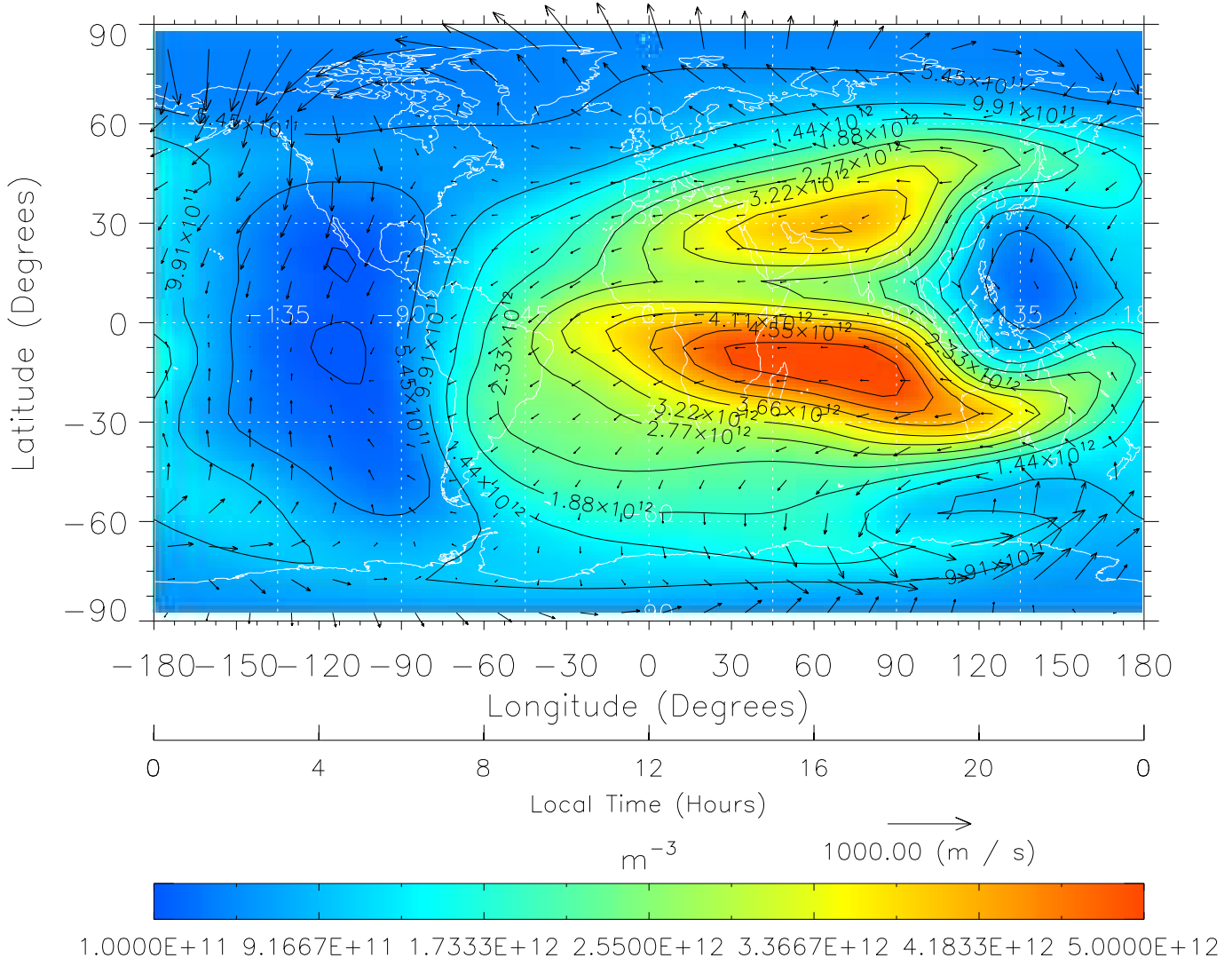
TIME-GCM MAP NmF2 with Neutral Wind vectors ZP = 2.00 UT = 12.00 DOY = 109
