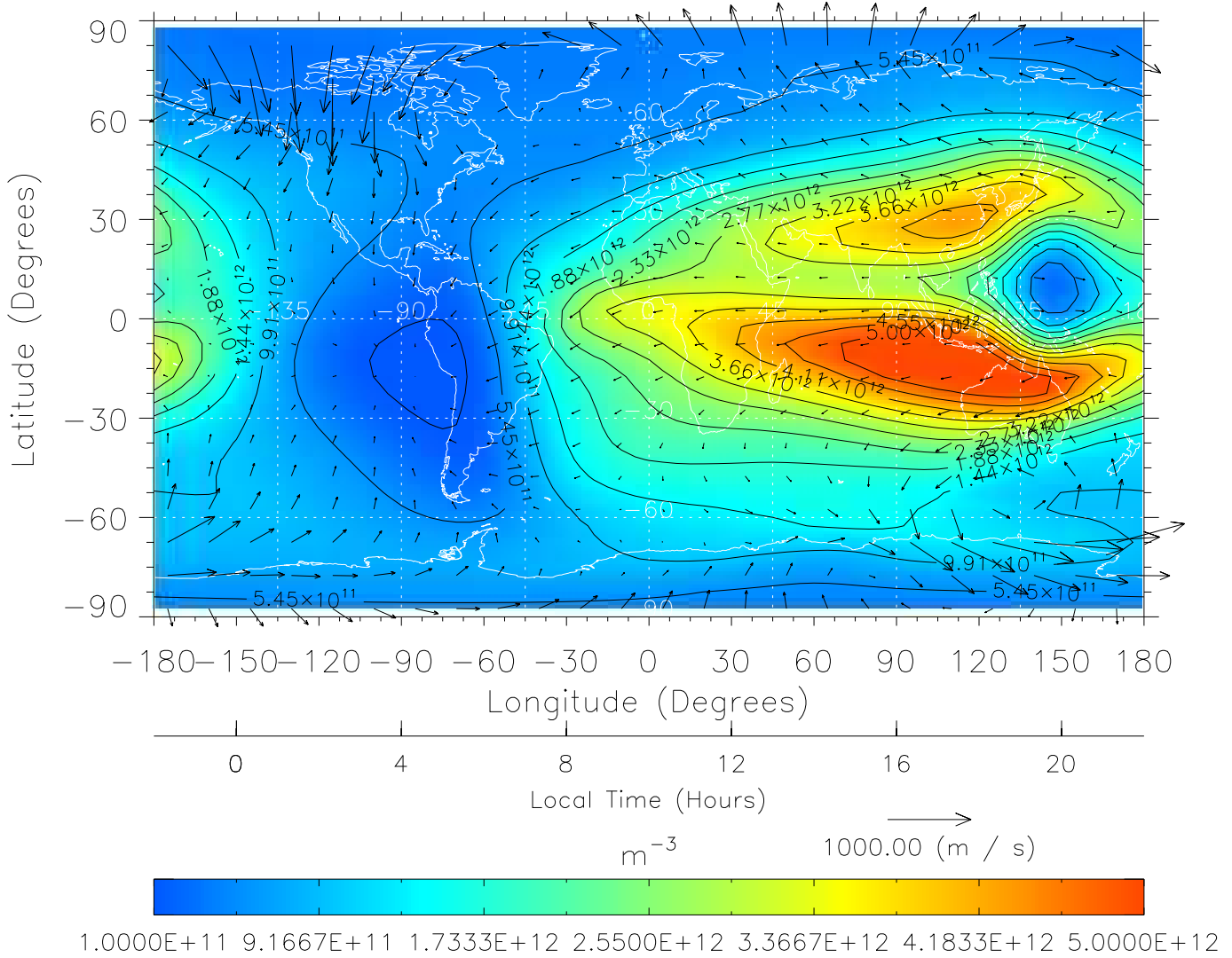
TIME-GCM MAP NmF2 with Neutral Wind vectors ZP = 2.00 UT = 10.00 DOY = 109
