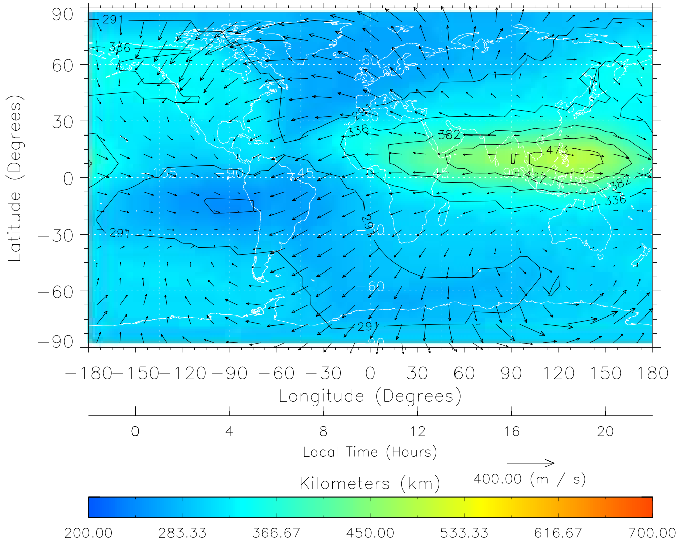
TIME-GCM MAP hmF2 with Neutral Wind vectors ZP = 2.00 UT = 10.00 DOY = 111
