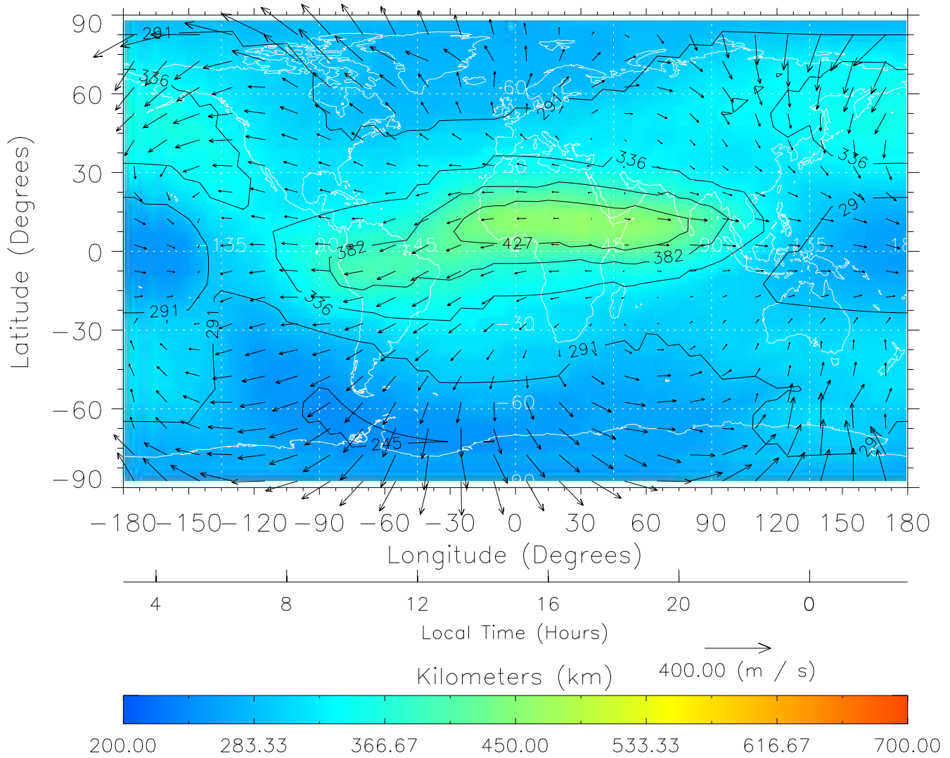
TIME-GCM MAP hmF2 with Neutral Wind vectors ZP = 2.00 UT = 15.00 DOY = 111
