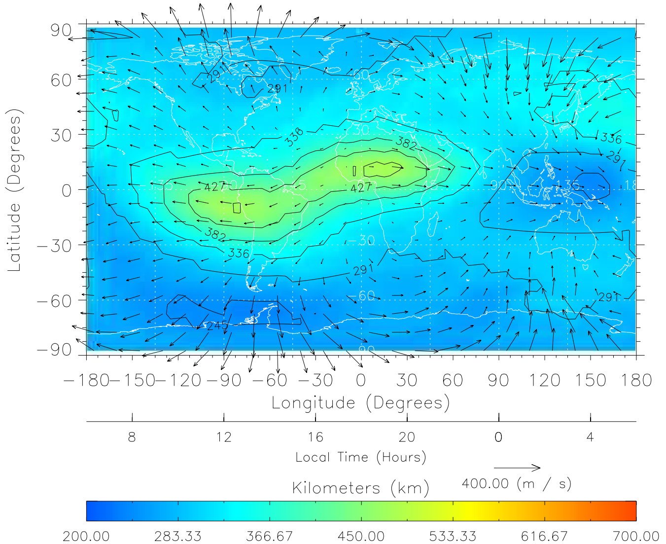
TIME-GCM MAP hmF2 with Neutral Wind vectors ZP = 2.00 UT = 18.00 DOY = 111
