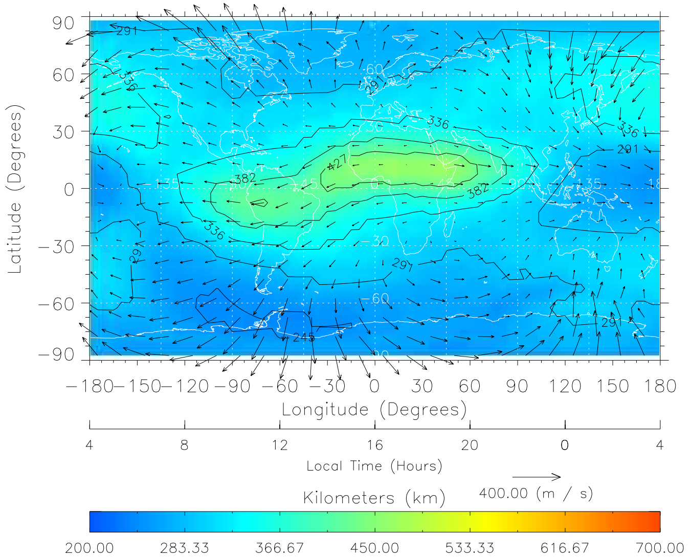
TIME-GCM MAP hmF2 with Neutral Wind vectors ZP = 2.00 UT = 16.00 DOY = 111
