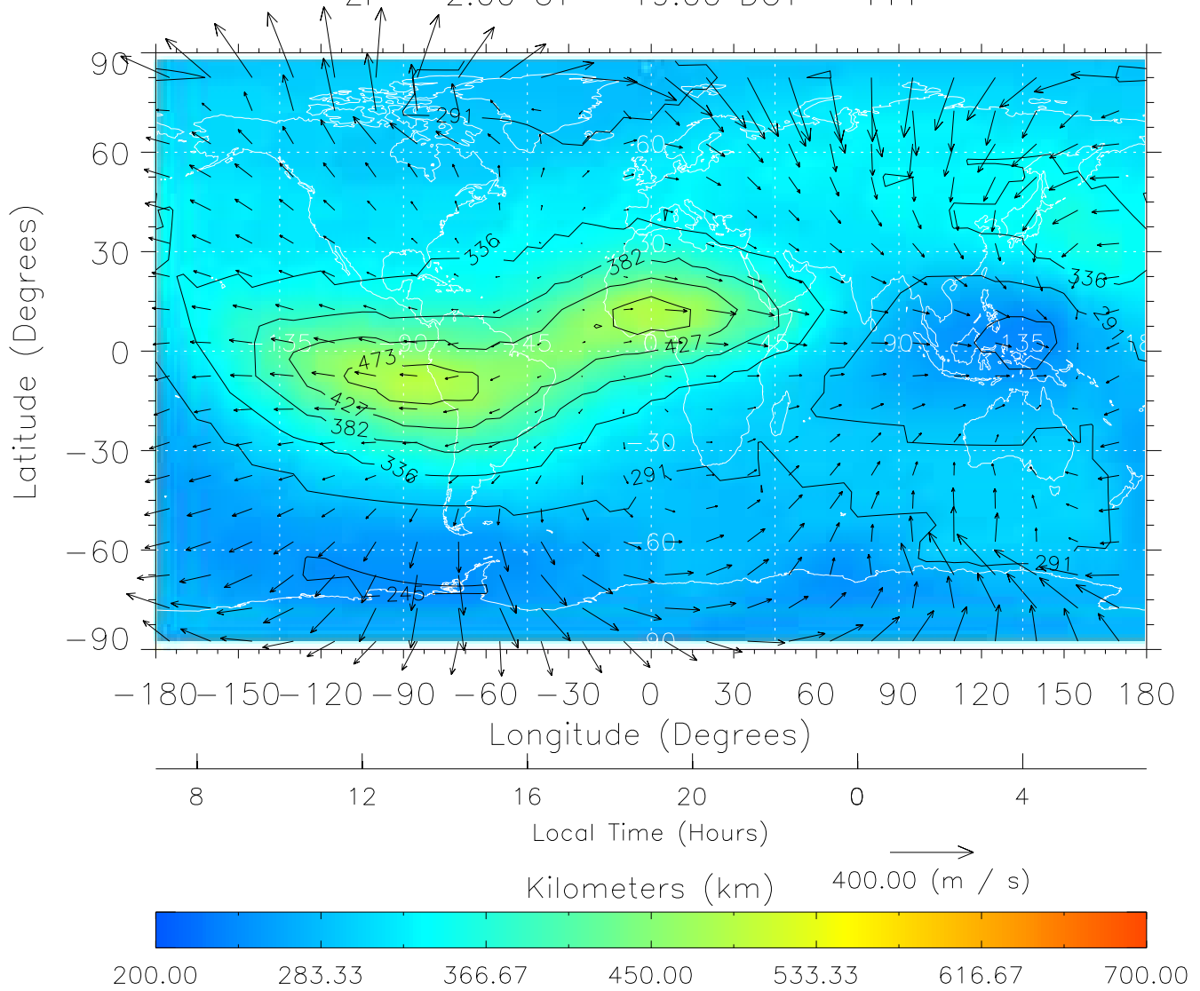
TIME-GCM MAP hmF2 with Neutral Wind vectors ZP = 2.00 UT = 19.00 DOY = 111
