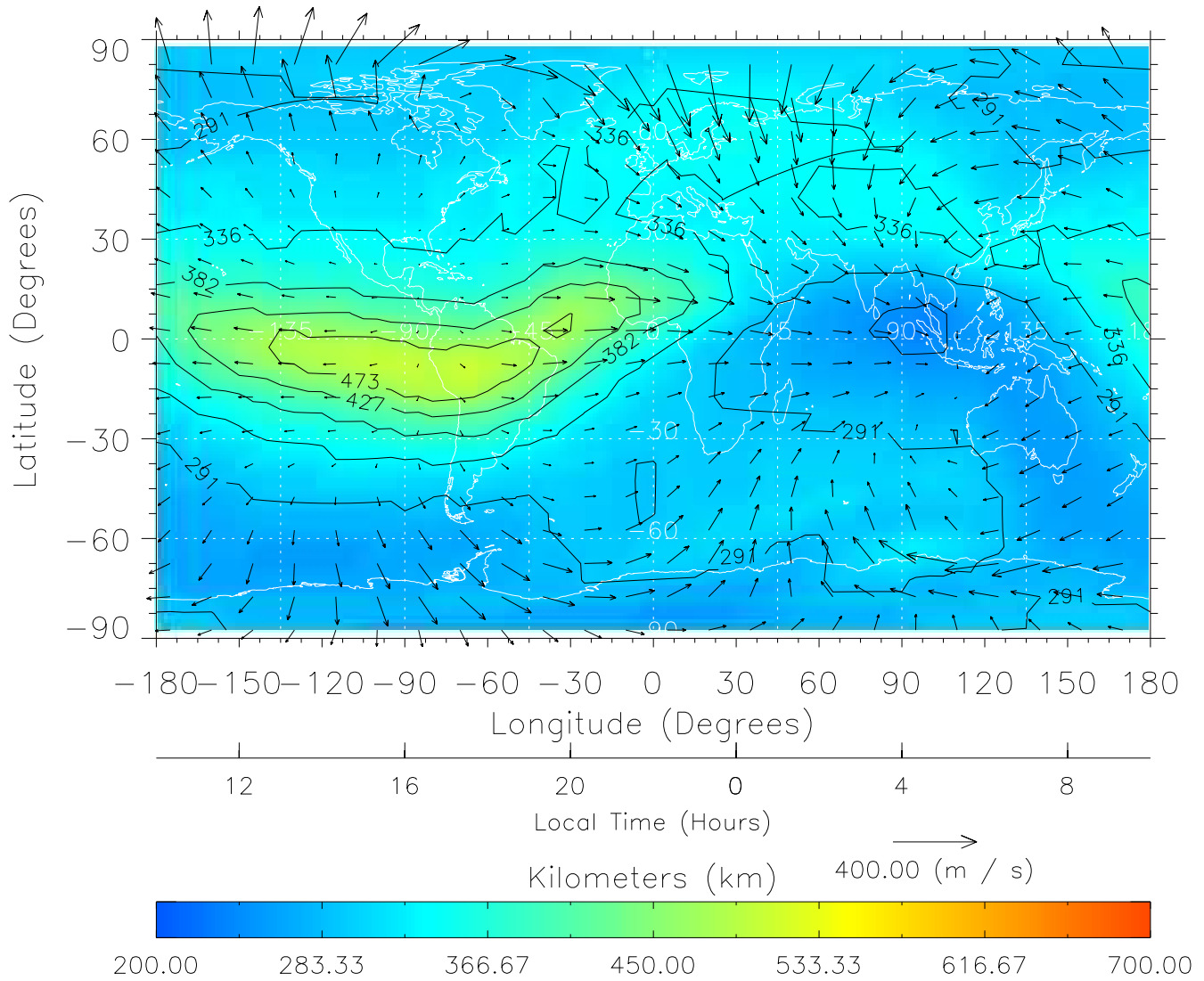
TIME-GCM MAP hmF2 with Neutral Wind vectors ZP = 2.00 UT = 22.00 DOY = 111
