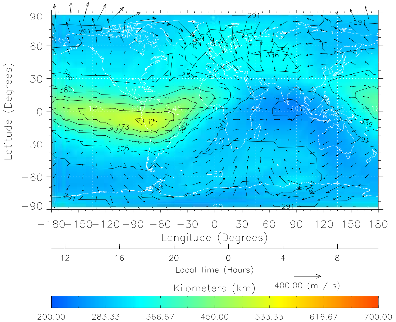
TIME-GCM MAP hmF2 with Neutral Wind vectors ZP = 2.00 UT = 23.00 DOY = 111
