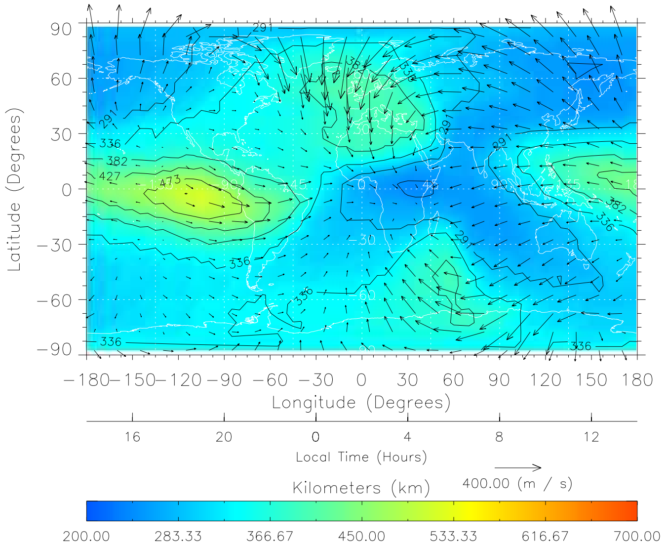
TIME-GCM MAP hmF2 with Neutral Wind vectors ZP = 2.00 UT = 2.00 DOY = 111
