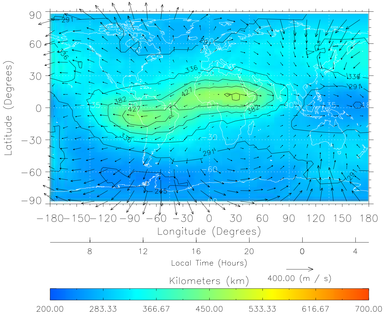
TIME-GCM MAP hmF2 with Neutral Wind vectors ZP = 2.00 UT = 17.00 DOY = 111
