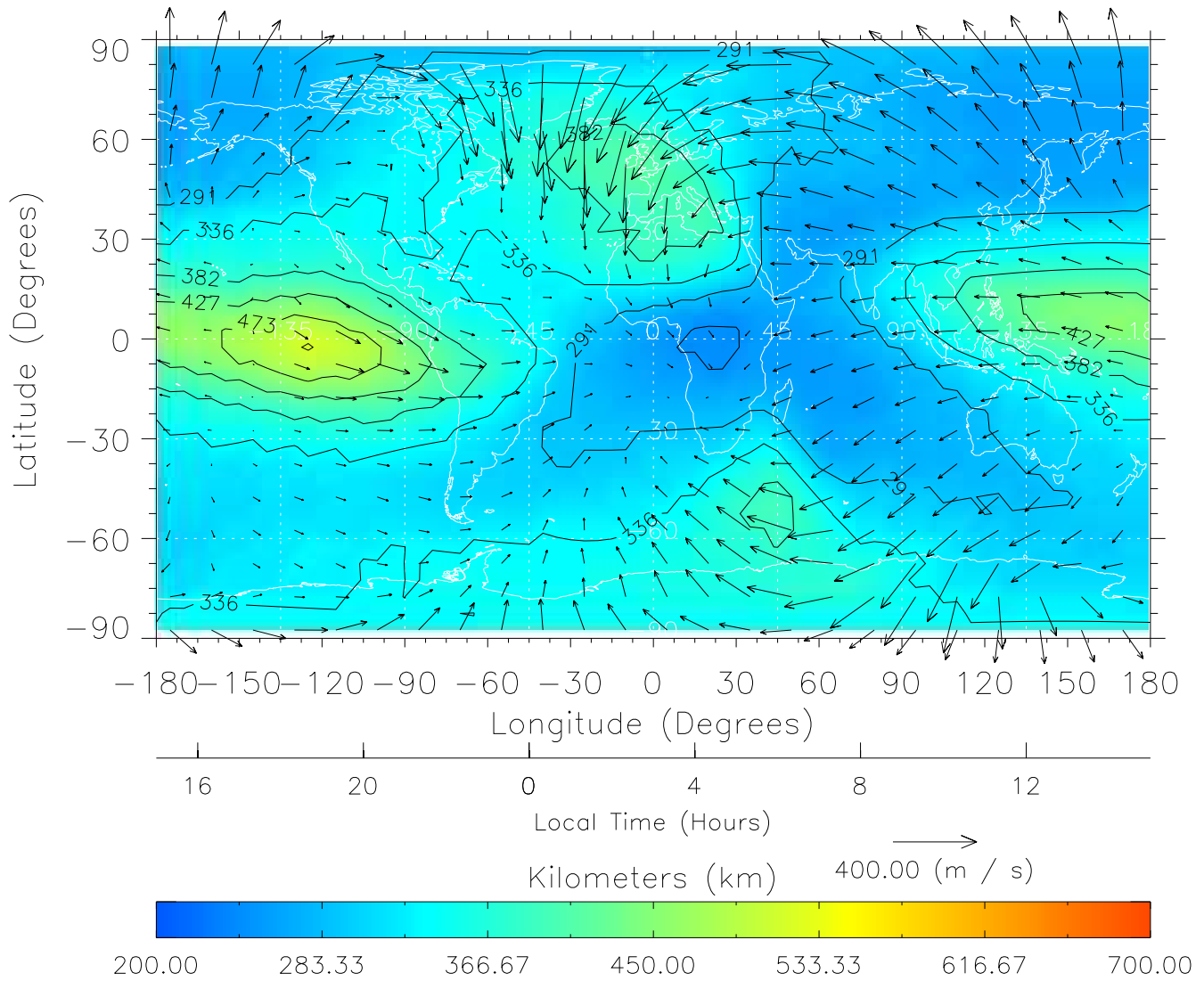
TIME-GCM MAP hmF2 with Neutral Wind vectors ZP = 2.00 UT = 3.00 DOY = 111
