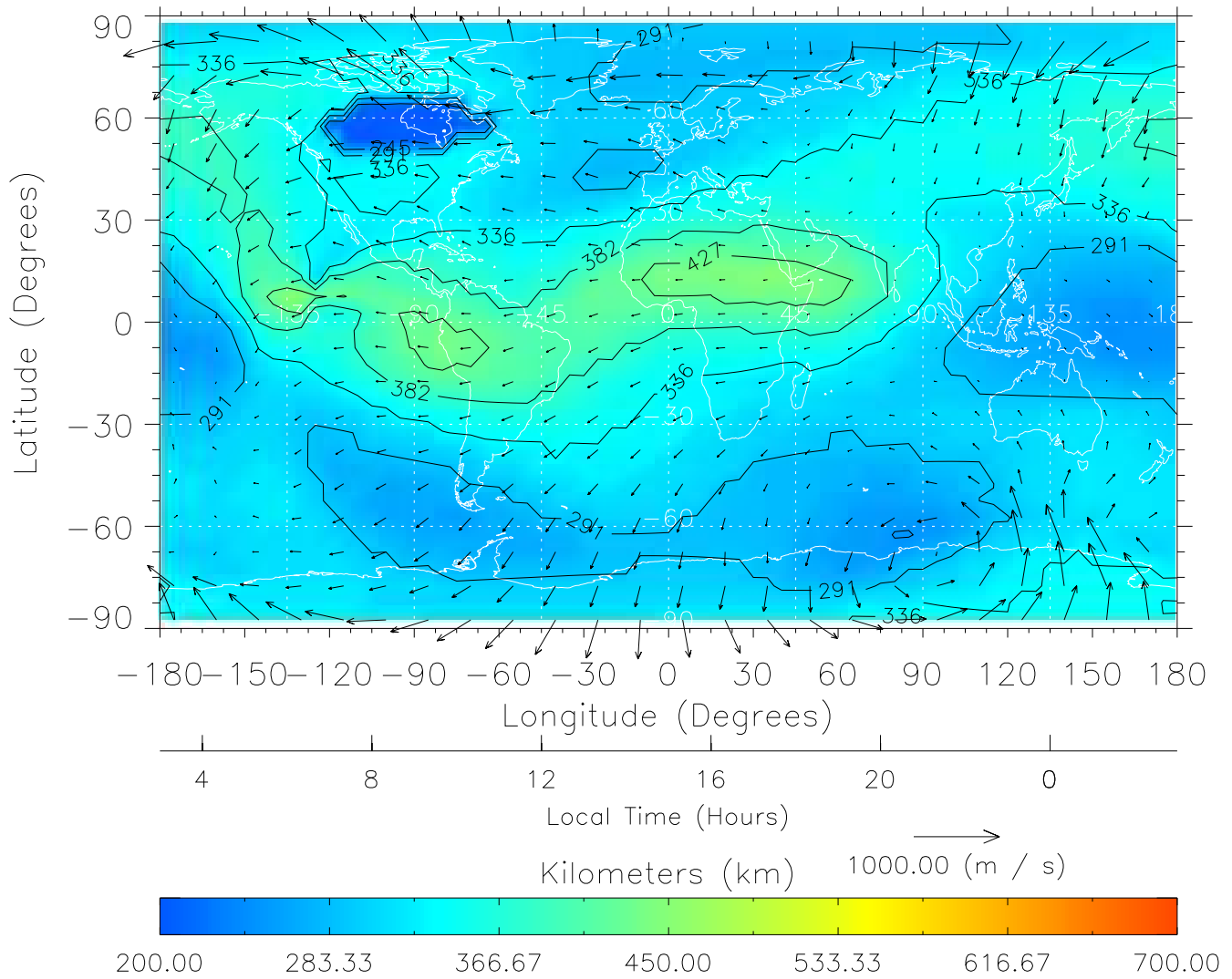
TIME-GCM MAP hmF2 with Neutral Wind vectors ZP = 2.00 UT = 15.00 DOY = 110
