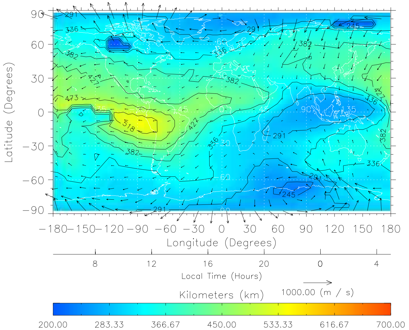
TIME-GCM MAP hmF2 with Neutral Wind vectors ZP = 2.00 UT = 17.00 DOY = 110
