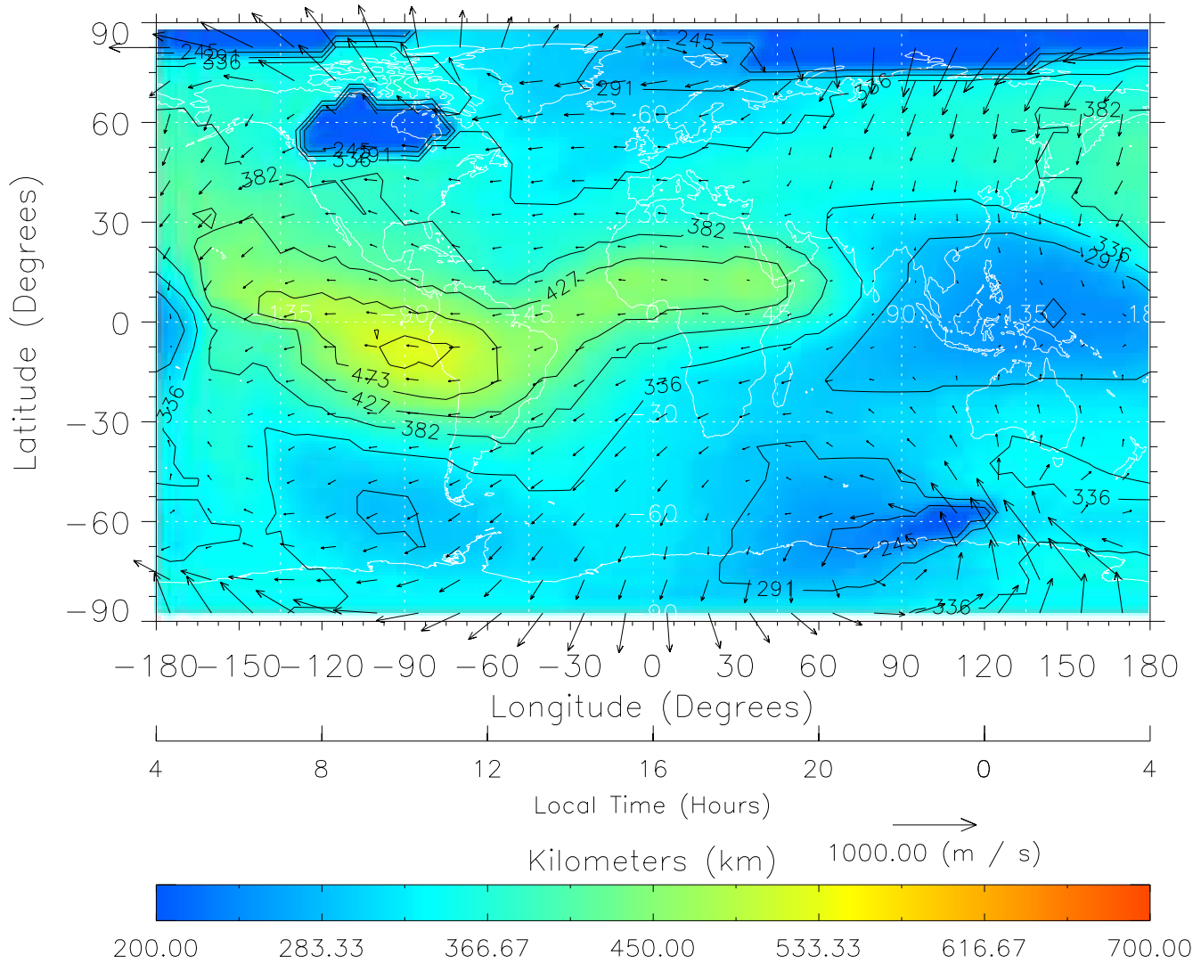
TIME-GCM MAP hmF2 with Neutral Wind vectors ZP = 2.00 UT = 16.00 DOY = 110
