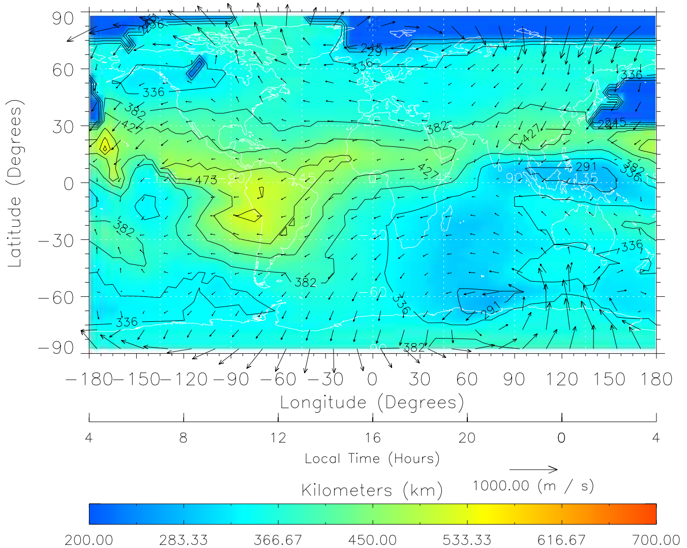
TIME-GCM MAP hmF2 with Neutral Wind vectors ZP = 2.00 UT = 16.00 DOY = 109
