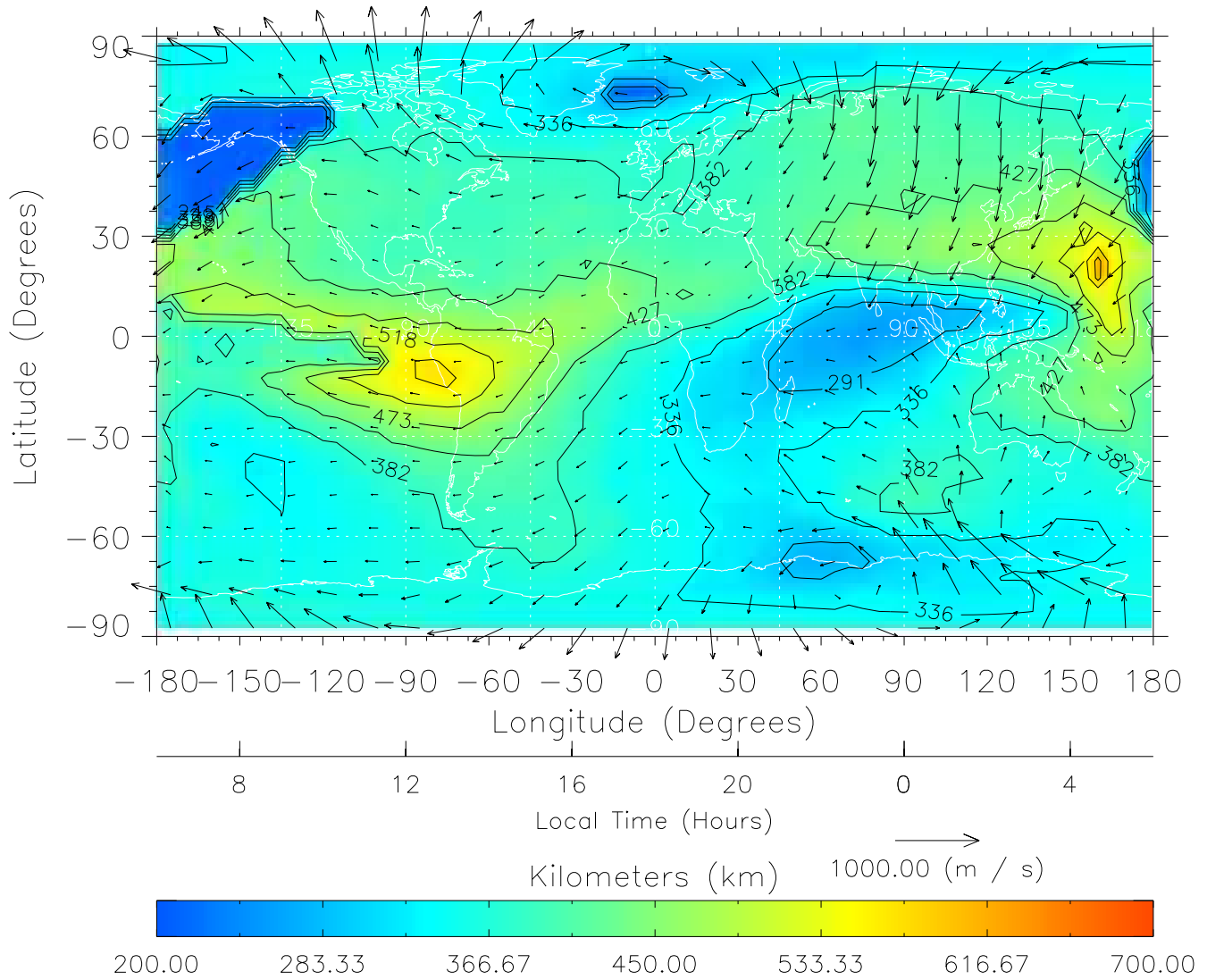
TIME-GCM MAP hmF2 with Neutral Wind vectors ZP = 2.00 UT = 18.00 DOY = 109
