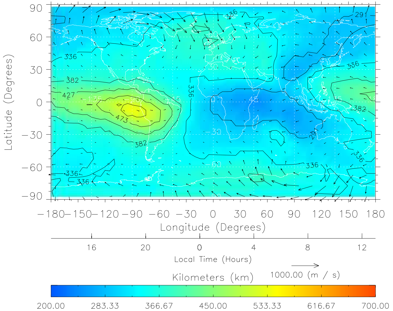
TIME-GCM MAP hmF2 with Neutral Wind vectors ZP = 2.00 UT = 1.00 DOY = 109
