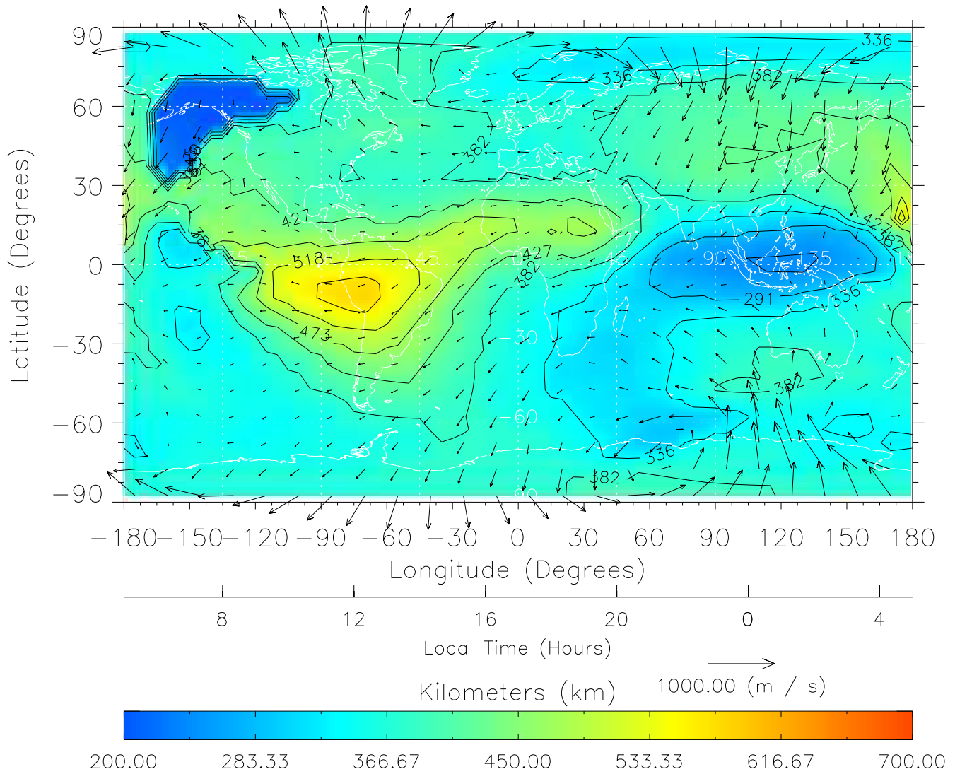
TIME-GCM MAP hmF2 with Neutral Wind vectors ZP = 2.00 UT = 17.00 DOY = 109
