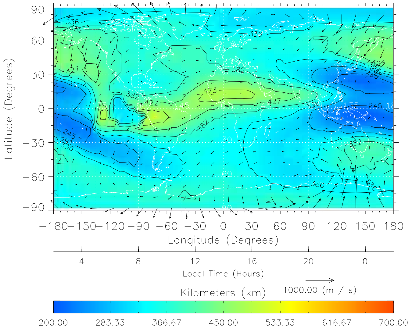
TIME-GCM MAP hmF2 with Neutral Wind vectors ZP = 2.00 UT = 14.00 DOY = 109
