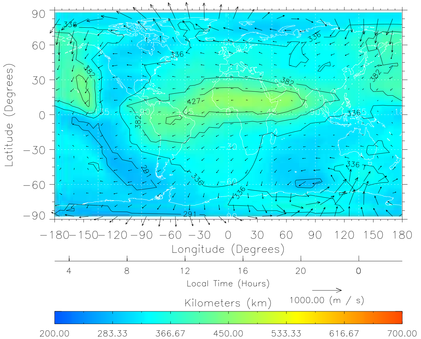
TIME-GCM MAP hmF2 with Neutral Wind vectors ZP = 2.00 UT = 15.00 DOY = 108
