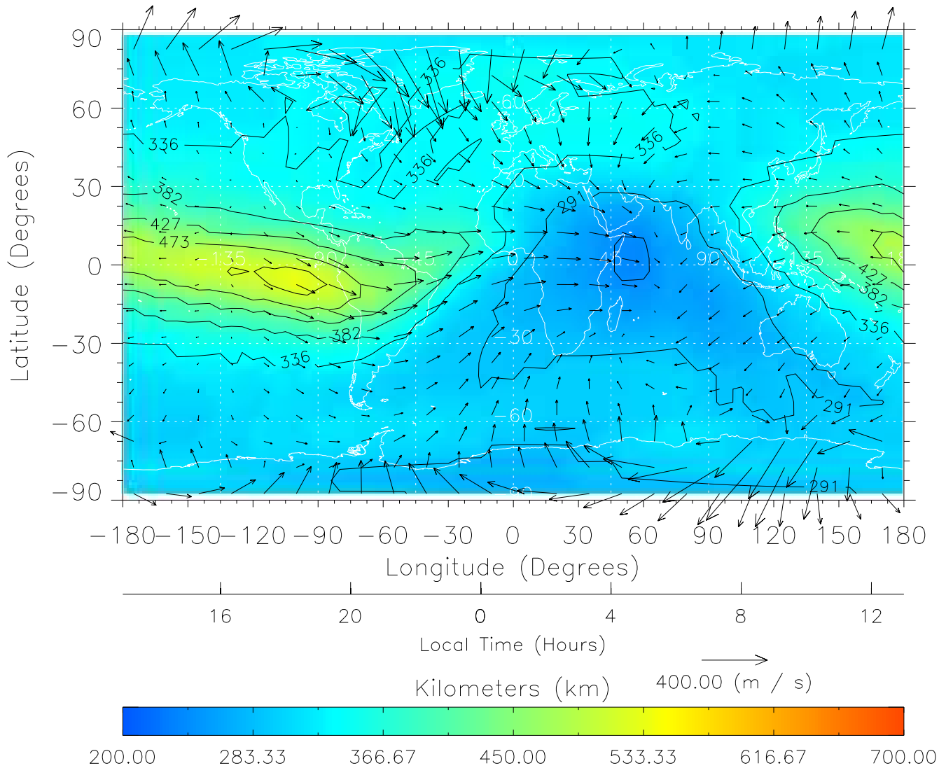
TIME-GCM MAP hmF2 with Neutral Wind vectors ZP = 2.00 UT = 1.00 DOY = 107
