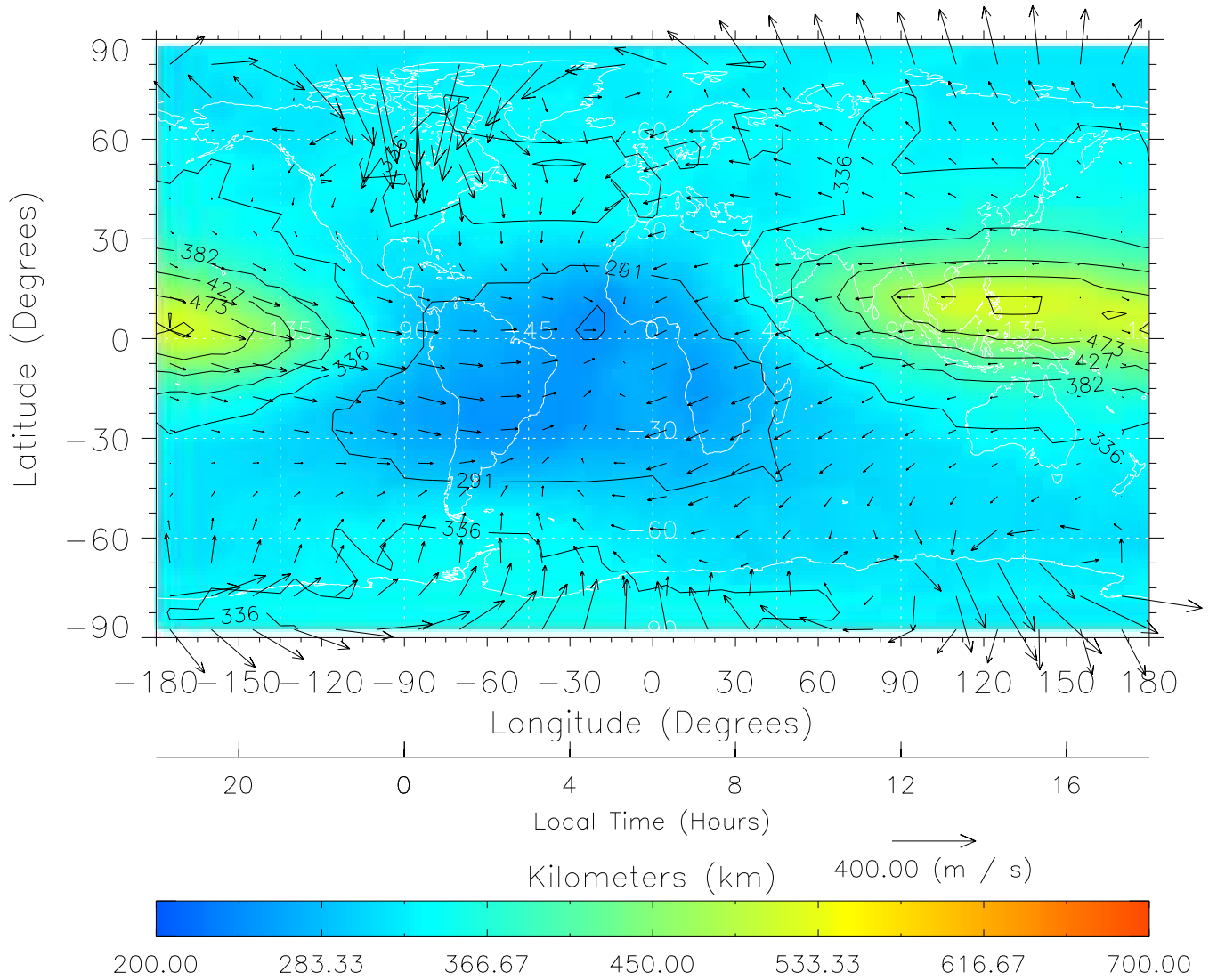
TIME-GCM MAP hmF2 with Neutral Wind vectors ZP = 2.00 UT = 6.00 DOY = 107
