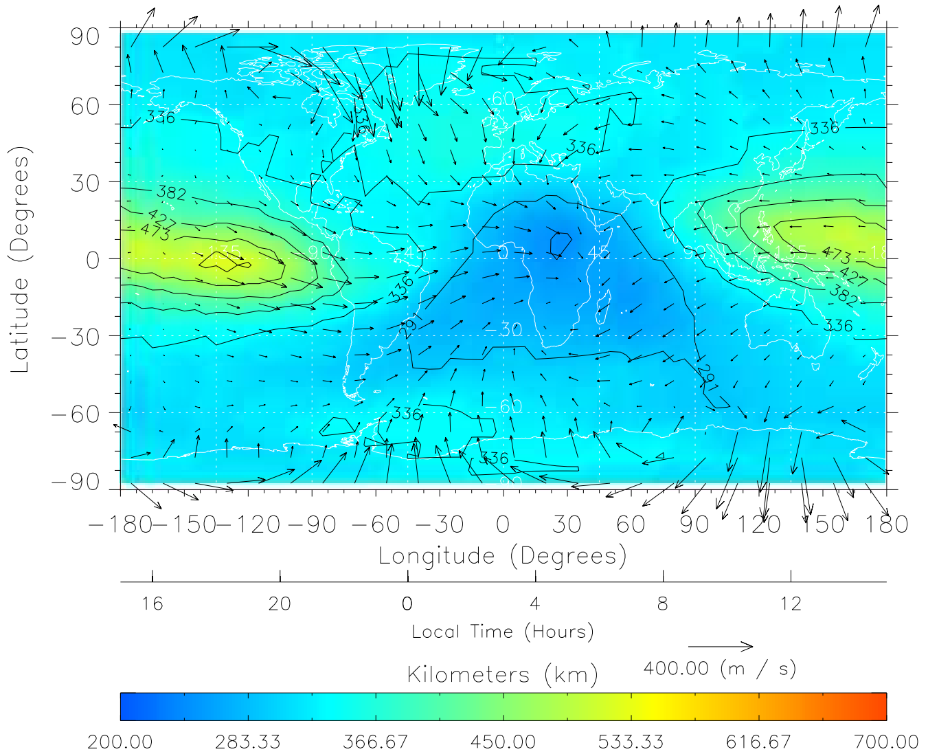
TIME-GCM MAP hmF2 with Neutral Wind vectors ZP = 2.00 UT = 3.00 DOY = 107
