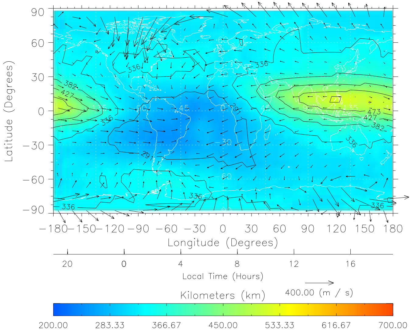
TIME-GCM MAP hmF2 with Neutral Wind vectors ZP = 2.00 UT = 7.00 DOY = 107
