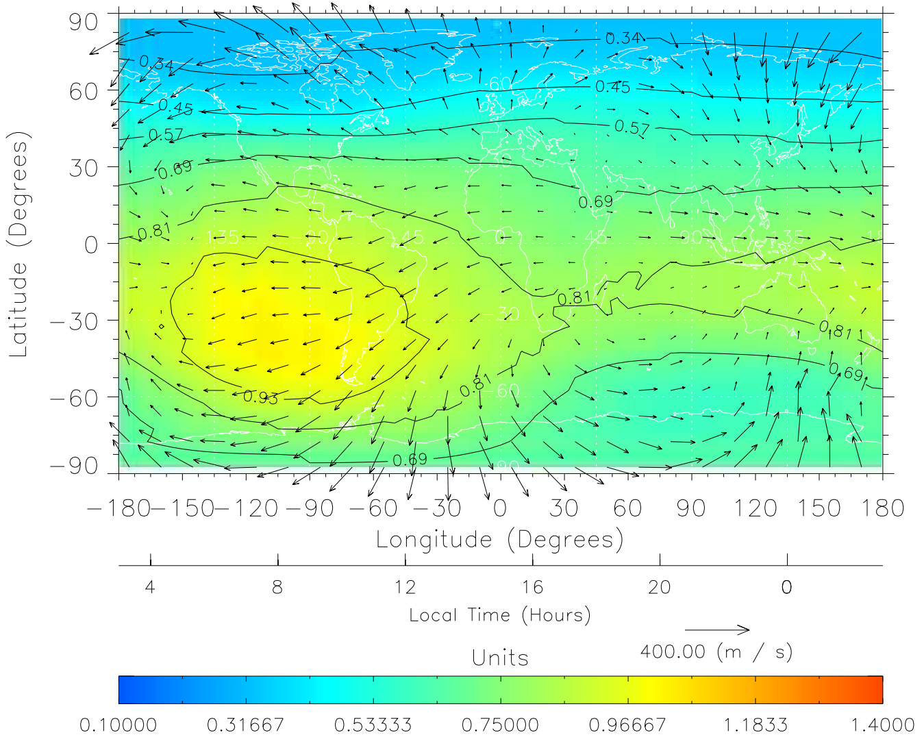
TIME-GCM MAP \Sigma O/N_2 with Neutral Wind vectors ZP = 2.00 UT = 15.00 DOY = 111
