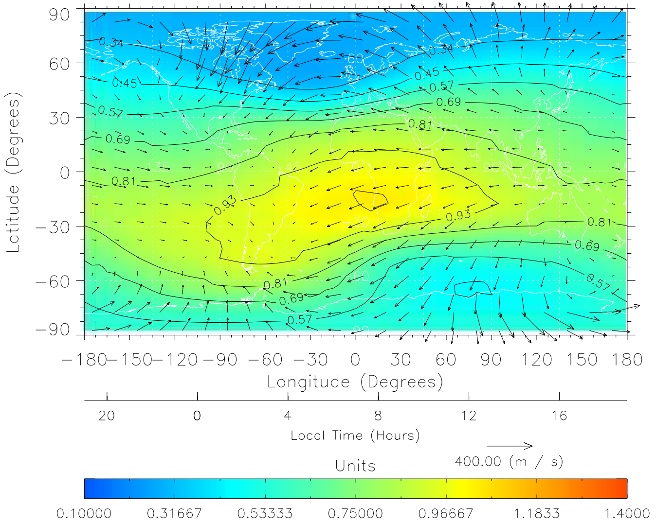
TIME-GCM MAP \Sigma O/N_2 with Neutral Wind vectors ZP = 2.00 UT = 7.00 DOY = 111
