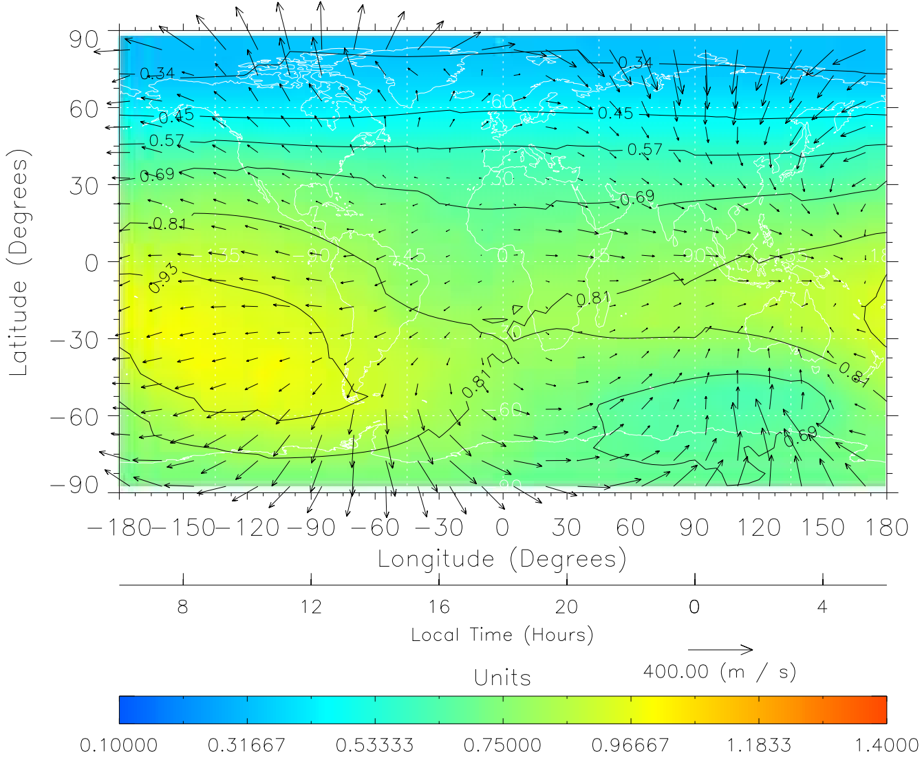
TIME-GCM MAP \Sigma O/N_2 with Neutral Wind vectors ZP = 2.00 UT = 18.00 DOY = 111
