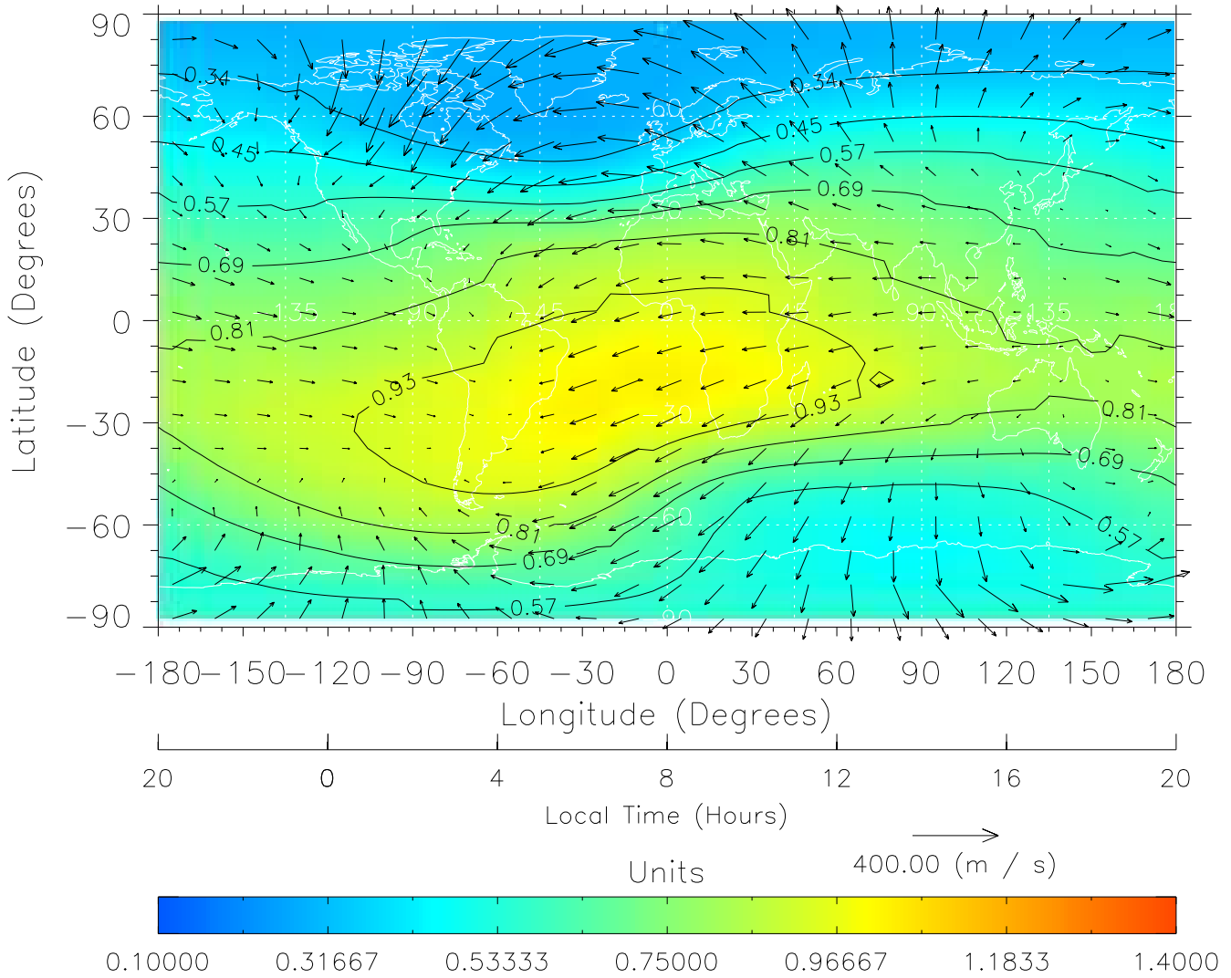
TIME-GCM MAP \Sigma O/N_2 with Neutral Wind vectors ZP = 2.00 UT = 8.00 DOY = 111
