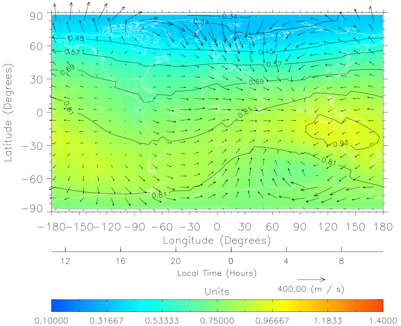
TIME-GCM MAP \Sigma O/N_2 with Neutral Wind vectors ZP = 2.00 UT = 23.00 DOY = 111
