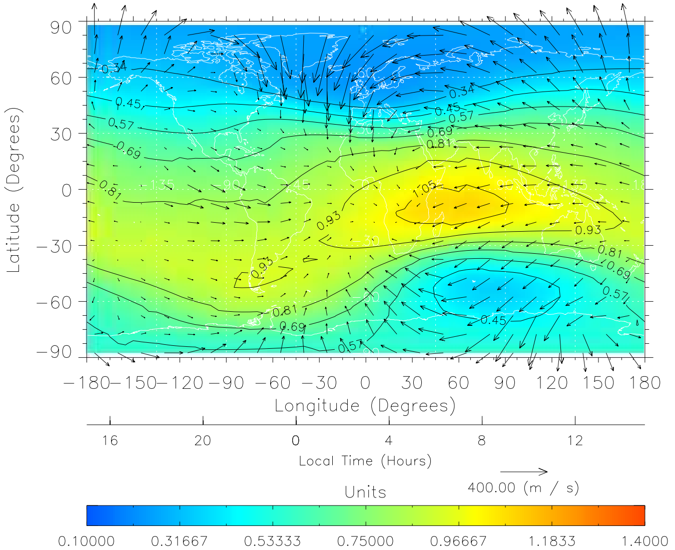
TIME-GCM MAP \Sigma O/N_2 with Neutral Wind vectors ZP = 2.00 UT = 3.00 DOY = 111
