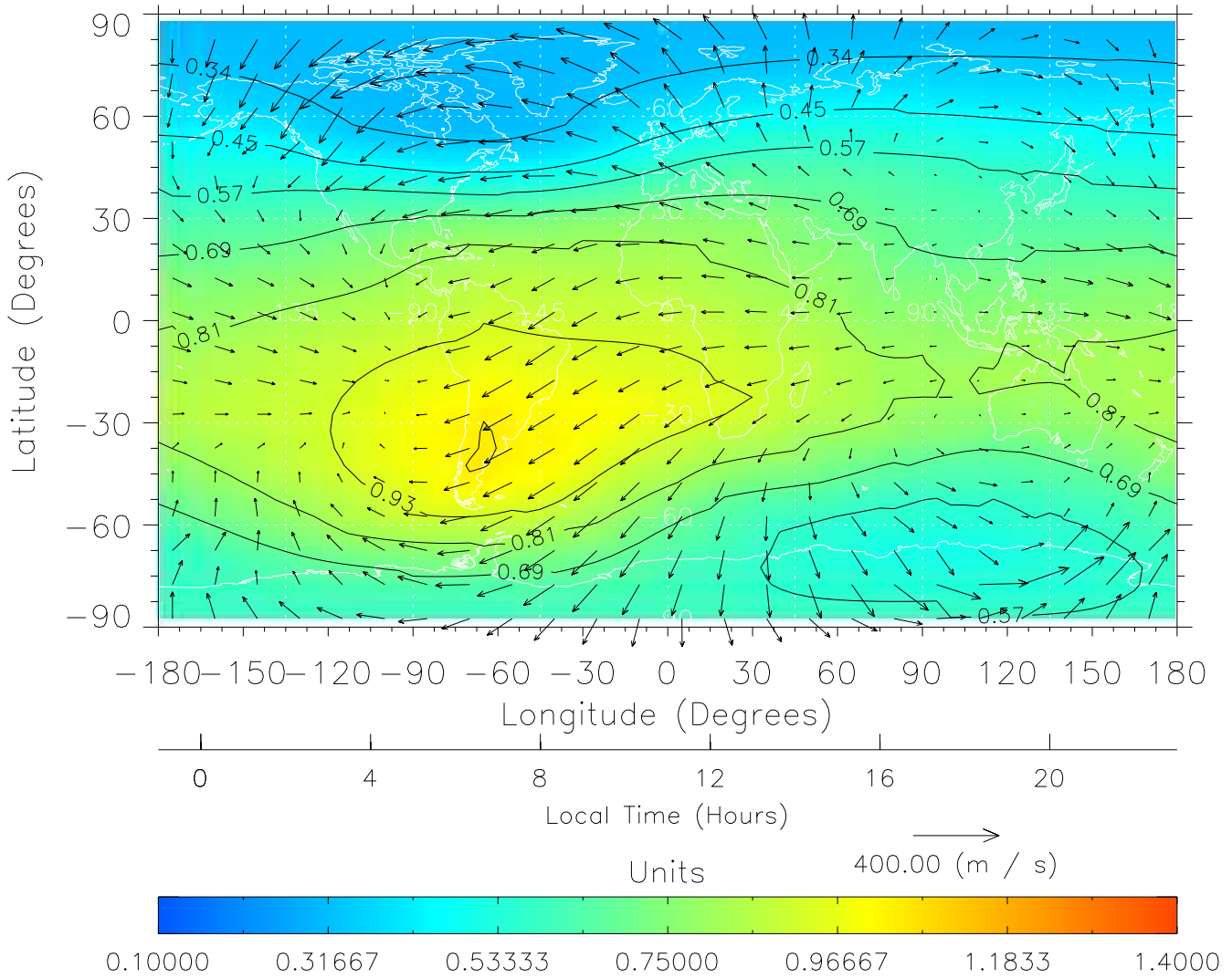
TIME-GCM MAP \Sigma O/N_2 with Neutral Wind vectors ZP = 2.00 UT = 11.00 DOY = 111
