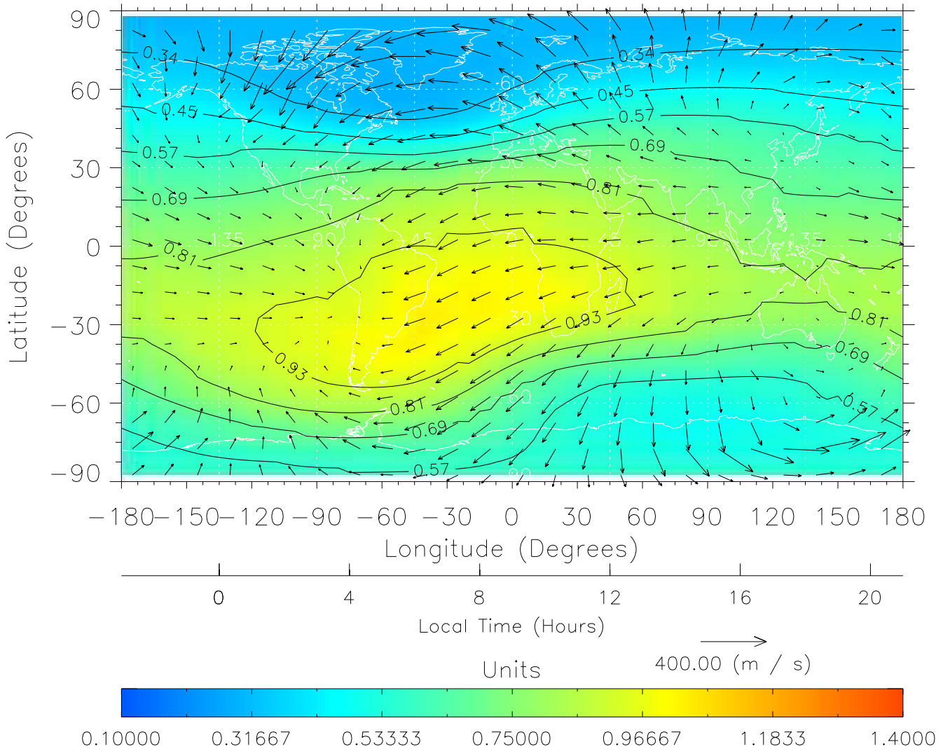
TIME-GCM MAP \Sigma O/N_2 with Neutral Wind vectors ZP = 2.00 UT = 9.00 DOY = 111
