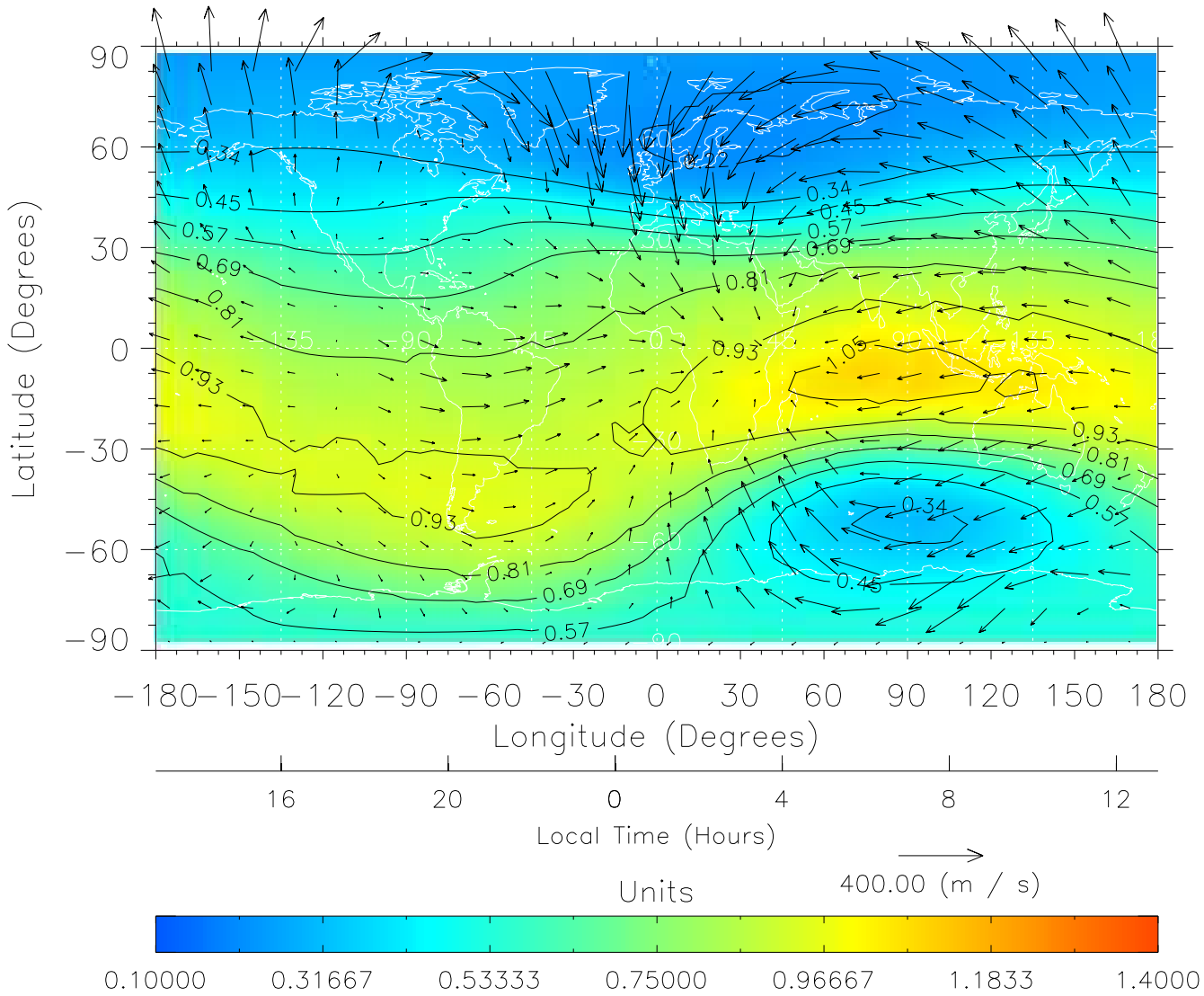
TIME-GCM MAP \Sigma O/N_2 with Neutral Wind vectors ZP = 2.00 UT = 1.00 DOY = 111
