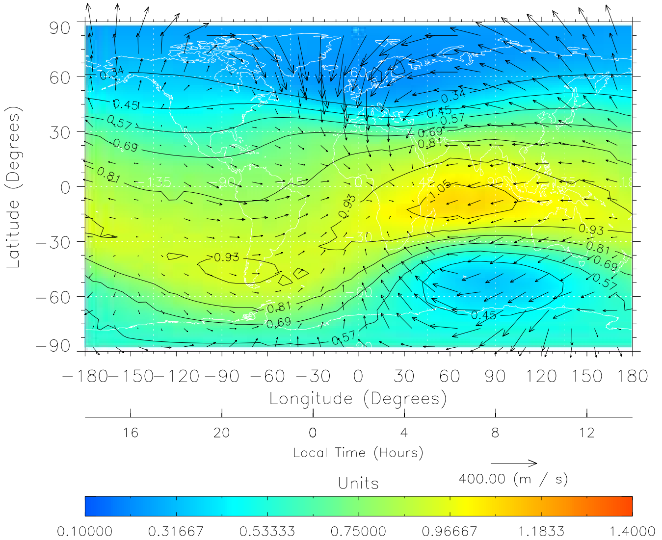
TIME-GCM MAP \Sigma O/N_2 with Neutral Wind vectors ZP = 2.00 UT = 2.00 DOY = 111
