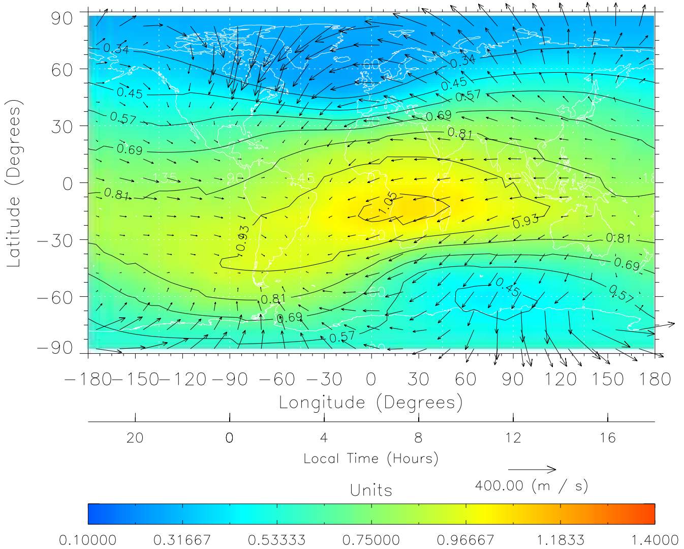
TIME-GCM MAP \Sigma O/N_2 with Neutral Wind vectors ZP = 2.00 UT = 6.00 DOY = 111
