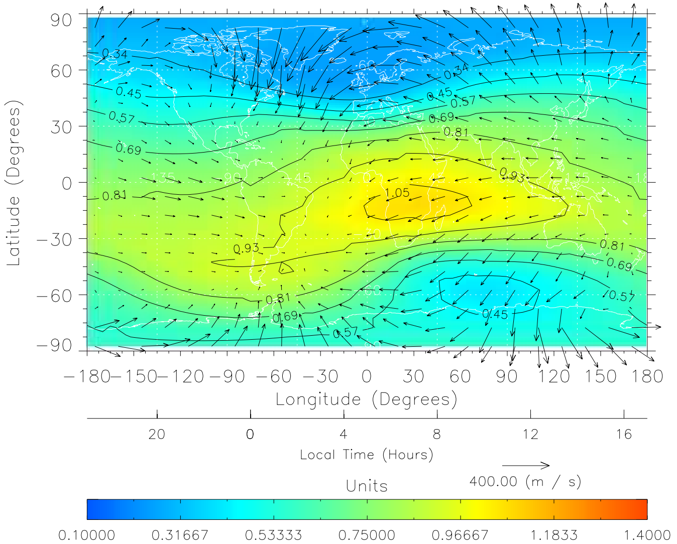
TIME-GCM MAP \Sigma O/N_2 with Neutral Wind vectors ZP = 2.00 UT = 5.00 DOY = 111
