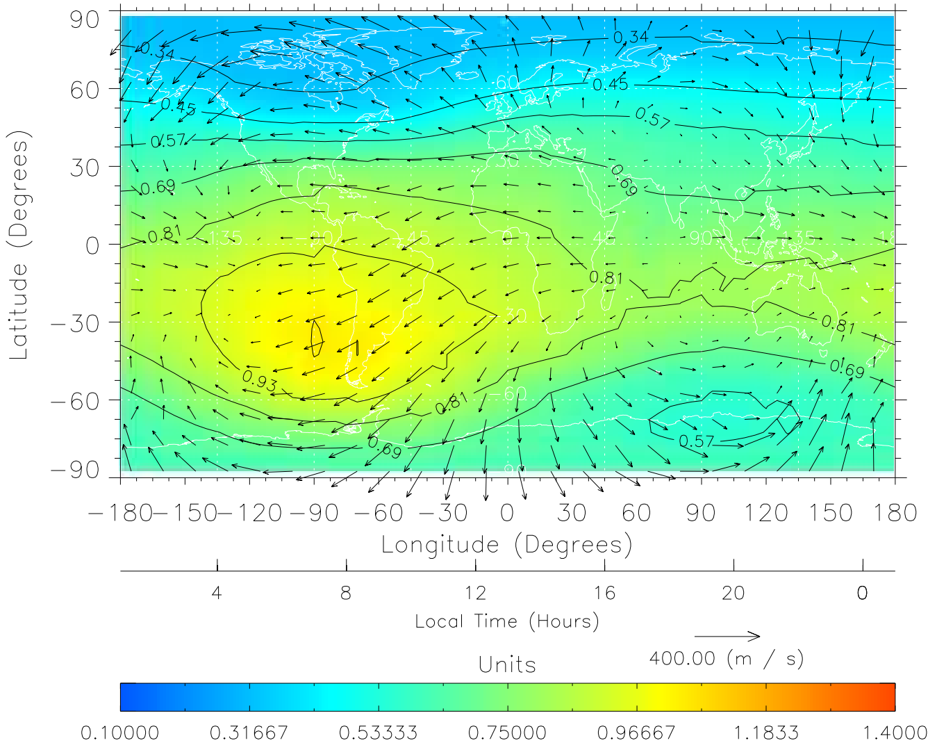
TIME-GCM MAP \Sigma O/N_2 with Neutral Wind vectors ZP = 2.00 UT = 13.00 DOY = 111
