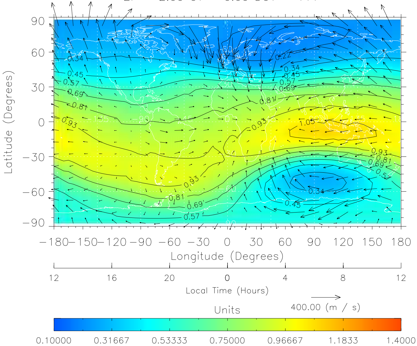
TIME-GCM MAP \Sigma O/N_2 with Neutral Wind vectors ZP = 2.00 UT = 0.00 DOY = 111
