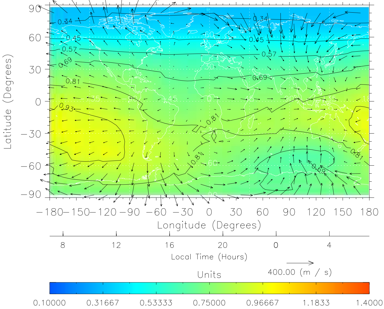
TIME-GCM MAP \Sigma O/N_2 with Neutral Wind vectors ZP = 2.00 UT = 19.00 DOY = 111
