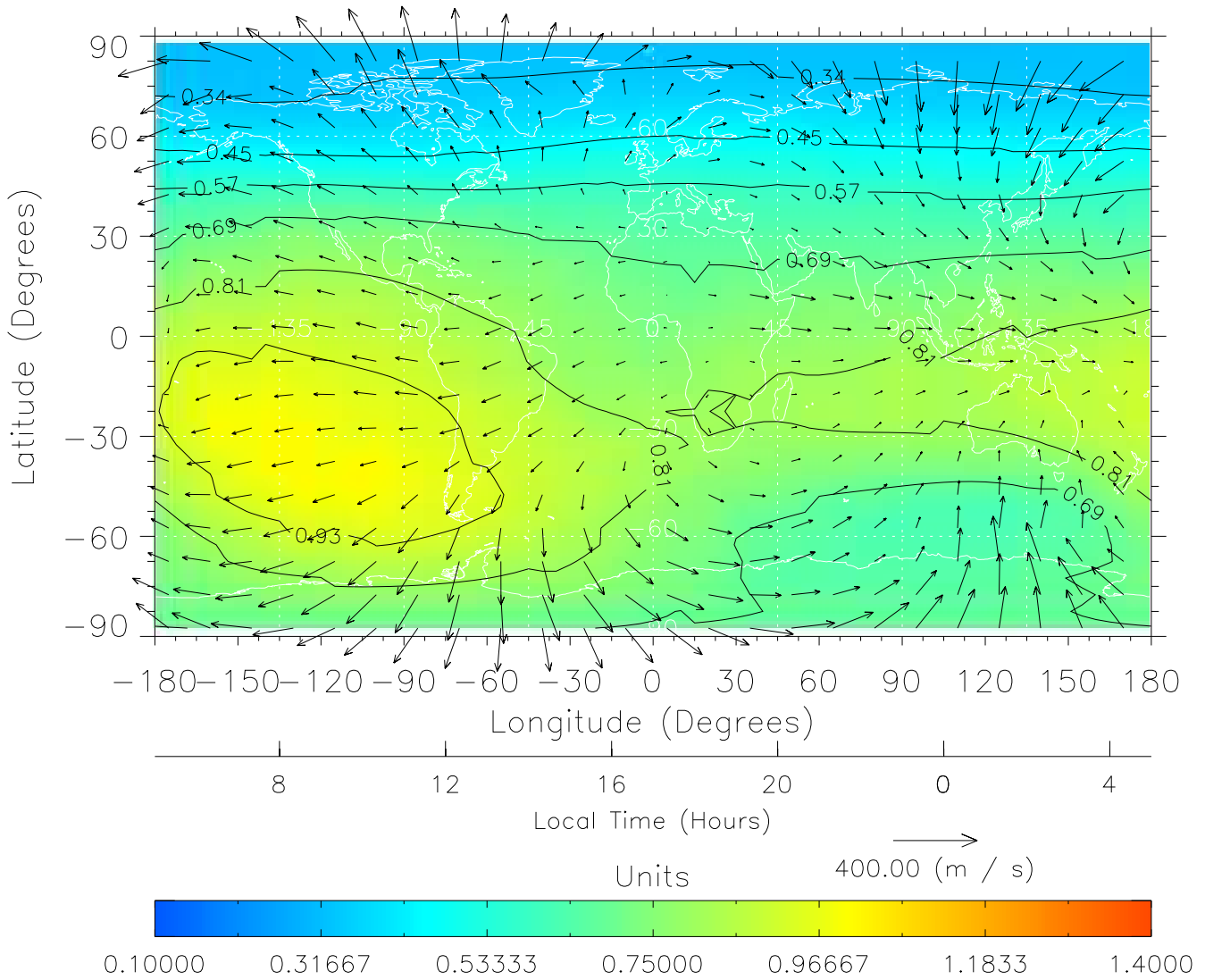
TIME-GCM MAP \Sigma O/N_2 with Neutral Wind vectors ZP = 2.00 UT = 17.00 DOY = 111
