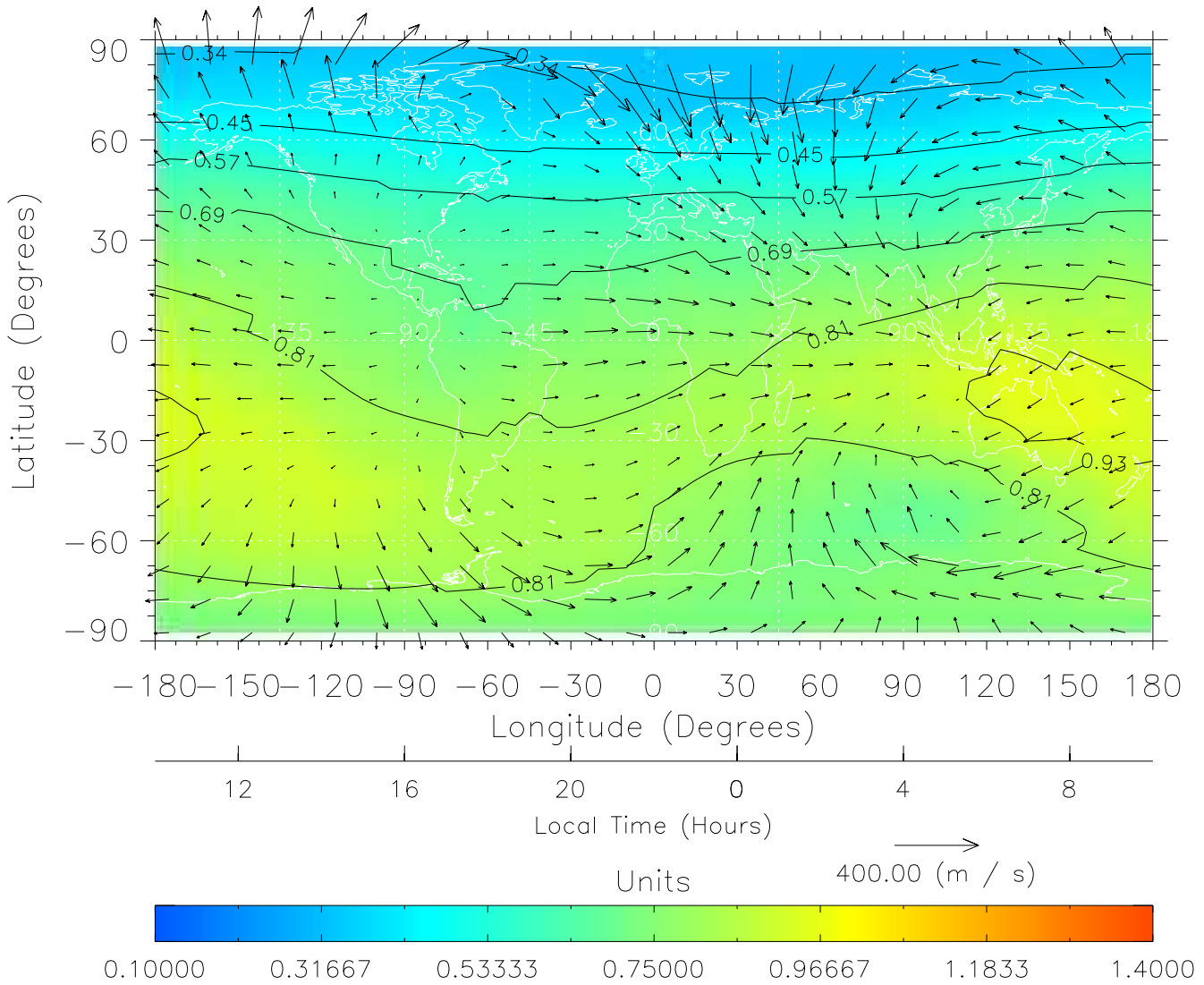
TIME-GCM MAP \Sigma O/N_2 with Neutral Wind vectors ZP = 2.00 UT = 22.00 DOY = 111
