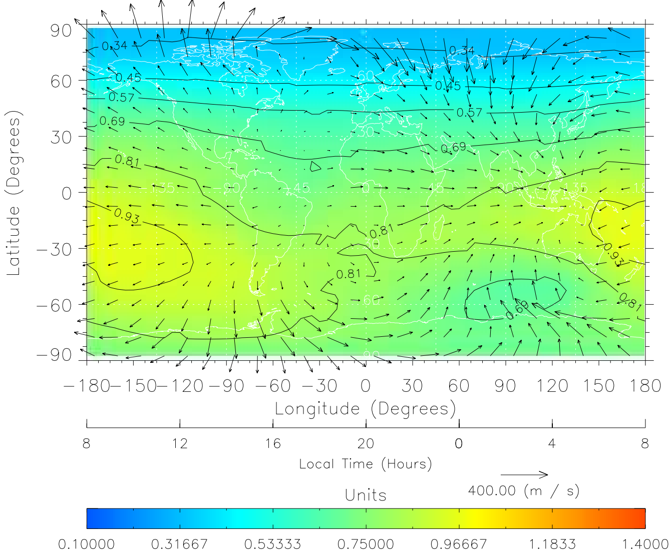
TIME-GCM MAP \Sigma O/N_2 with Neutral Wind vectors ZP = 2.00 UT = 20.00 DOY = 111
