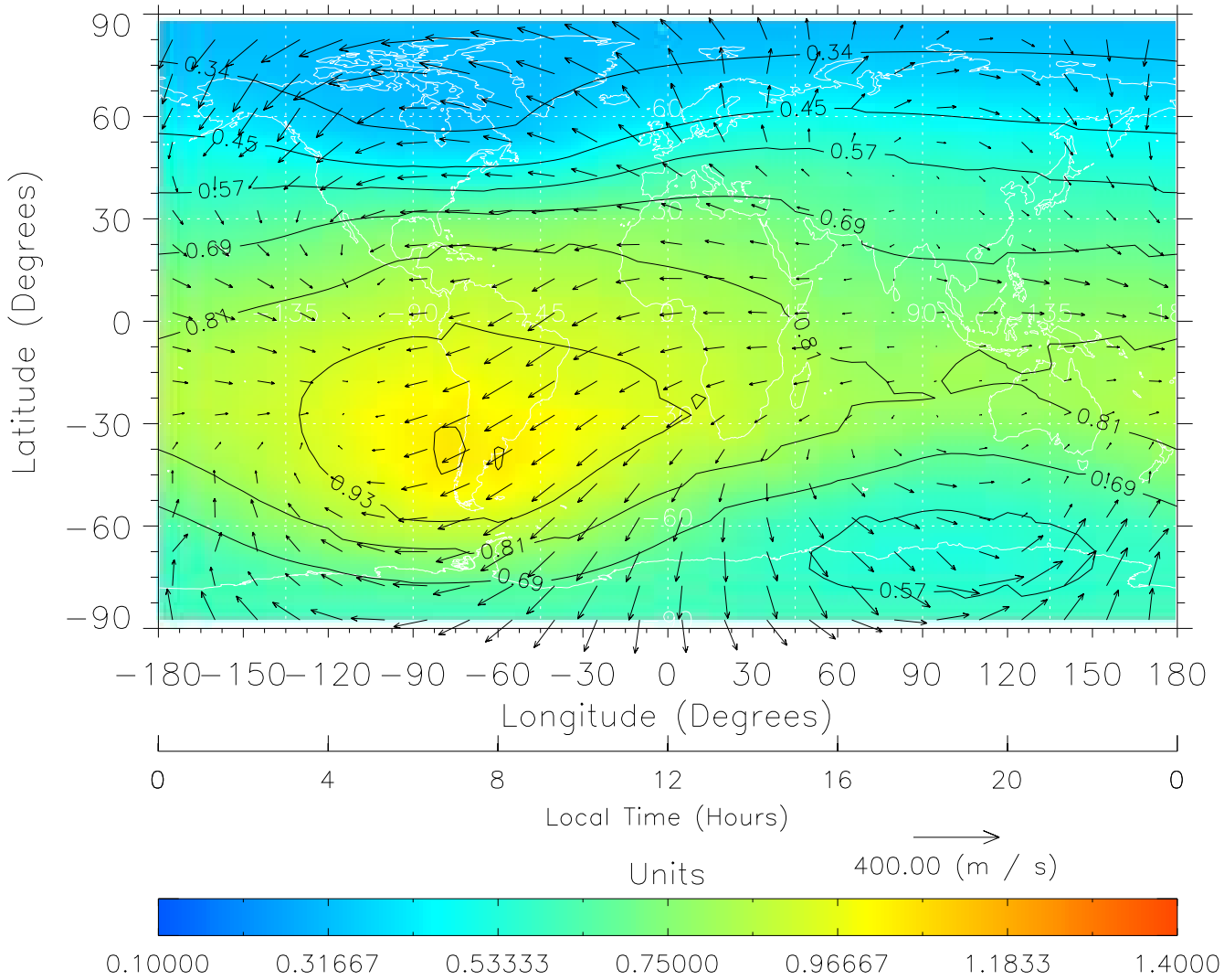
TIME-GCM MAP \Sigma O/N_2 with Neutral Wind vectors ZP = 2.00 UT = 12.00 DOY = 111
