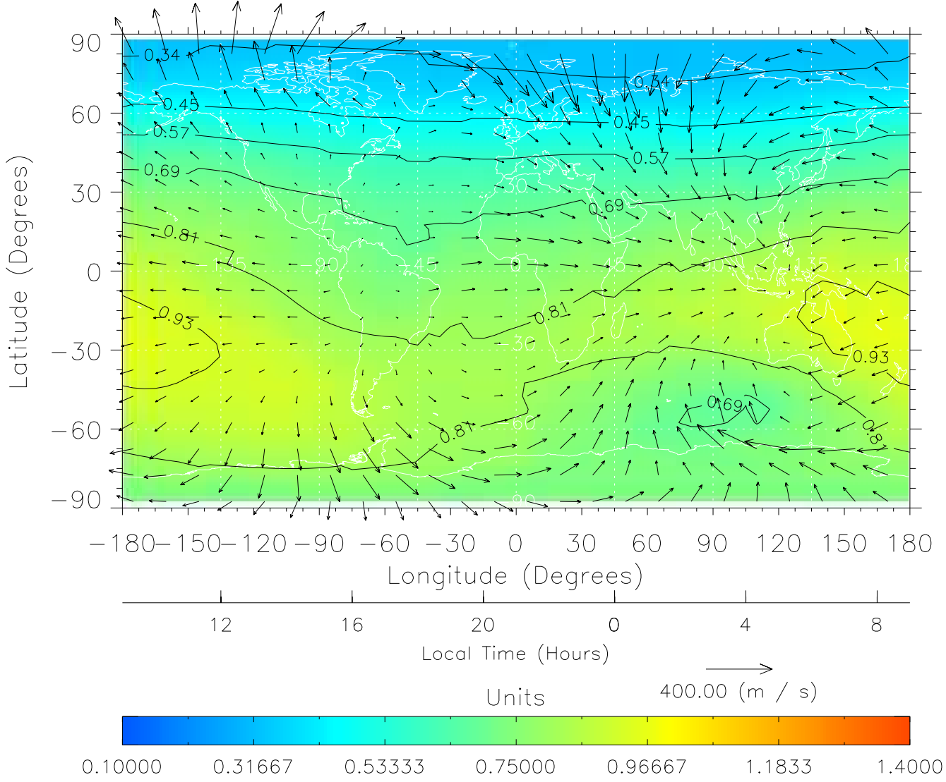
TIME-GCM MAP \Sigma O/N_2 with Neutral Wind vectors ZP = 2.00 UT = 21.00 DOY = 111
