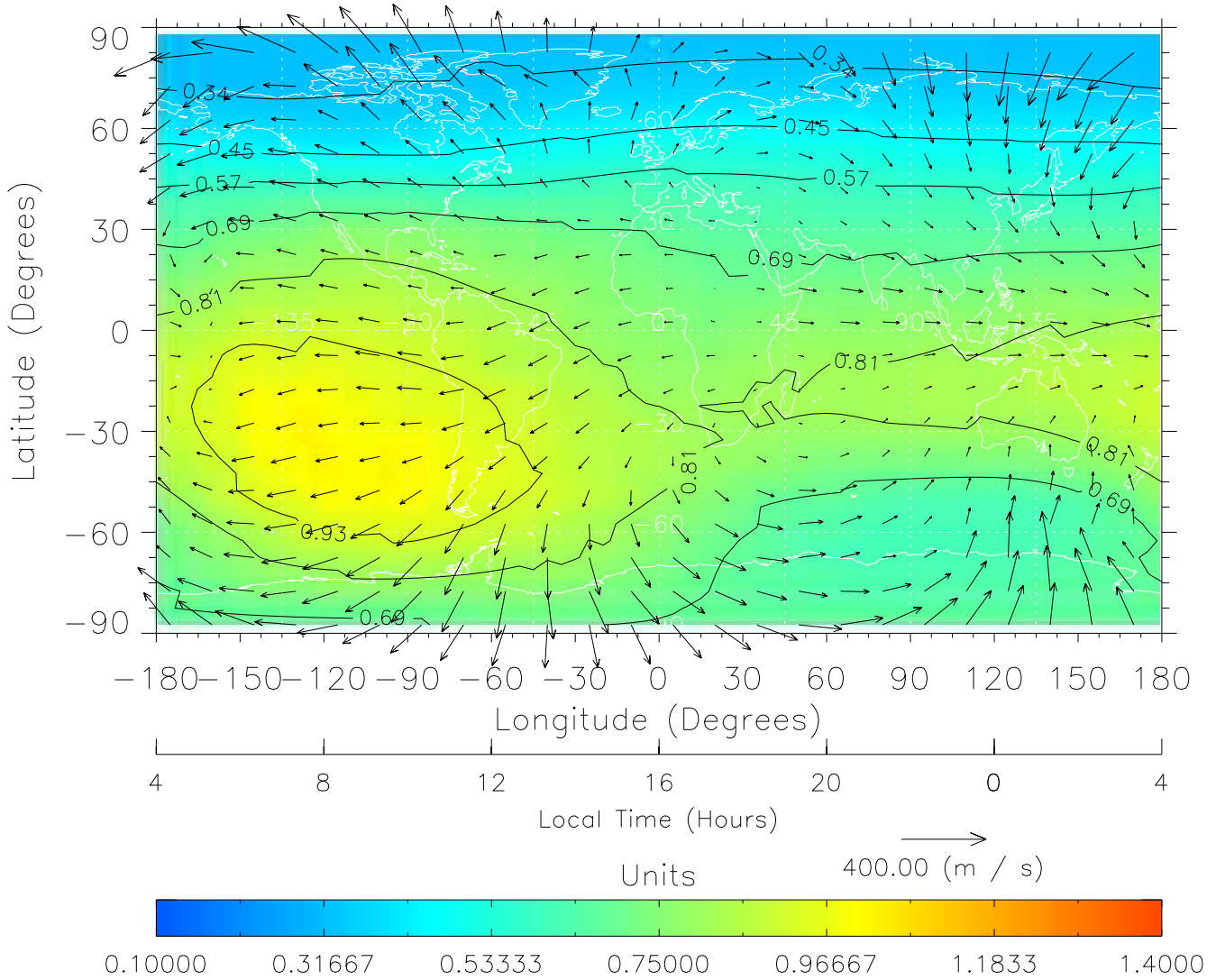
TIME-GCM MAP \Sigma O/N_2 with Neutral Wind vectors ZP = 2.00 UT = 16.00 DOY = 111
