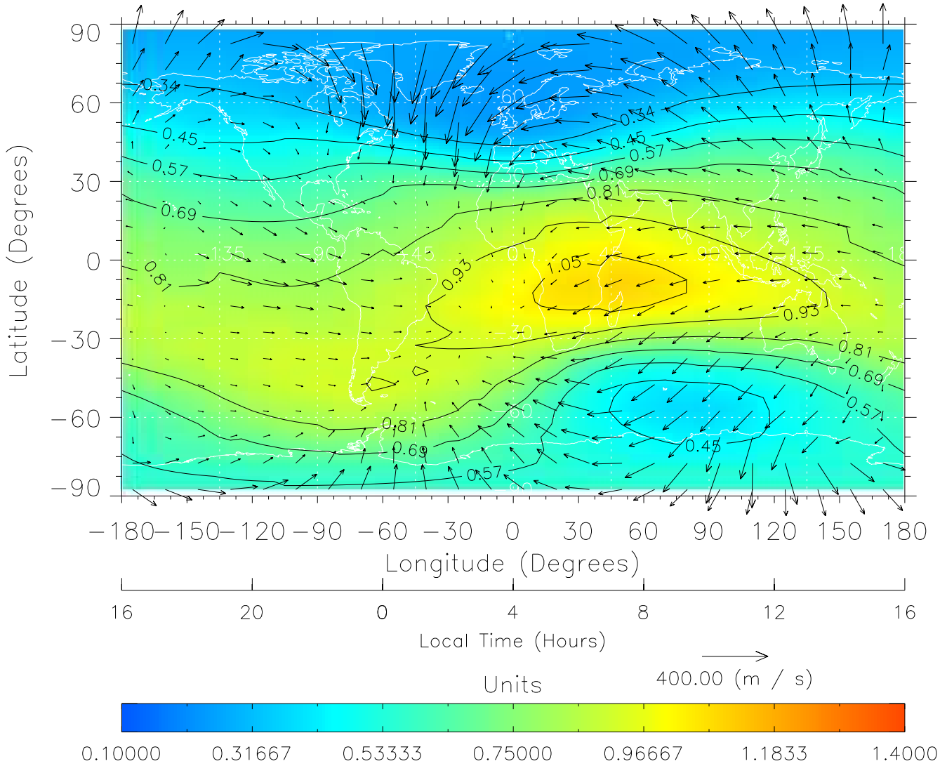
TIME-GCM MAP \Sigma O/N_2 with Neutral Wind vectors ZP = 2.00 UT = 4.00 DOY = 111
